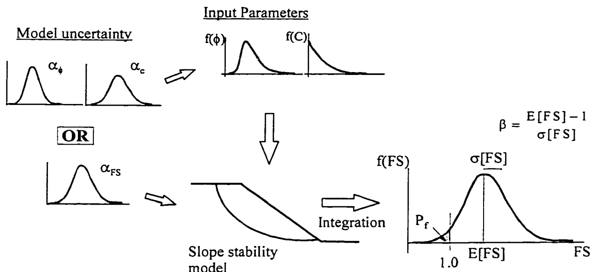
Figure 4–2 Concept of probabilistic analysis
