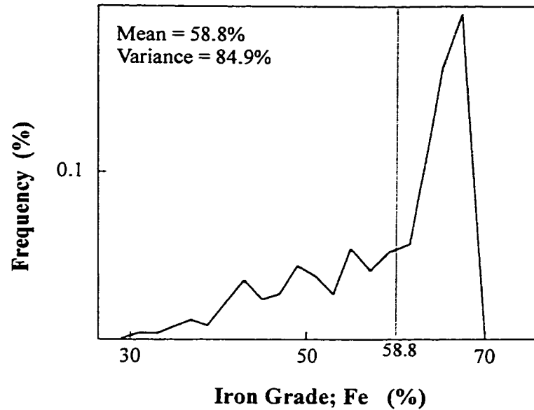
Figure 3–2 Histogram of iron grades; global ore (modified from Journel & Huijbregts, 1978)
