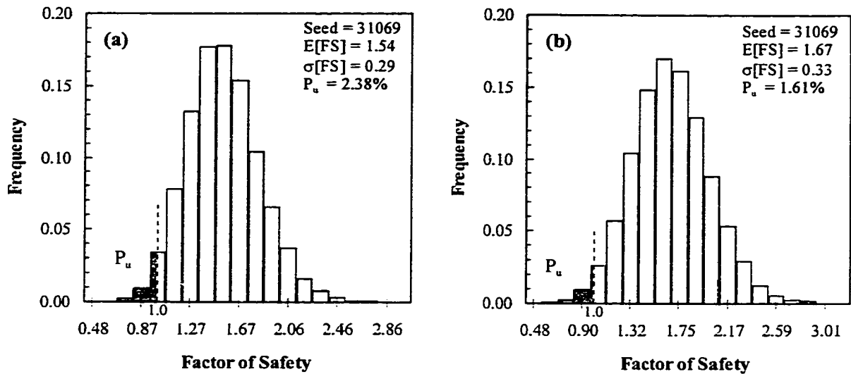
Figure 6–17 Histograms of the factor of safety, Design 2 – Proposed Methodology: a) Deep failure; b) Shallow failure
