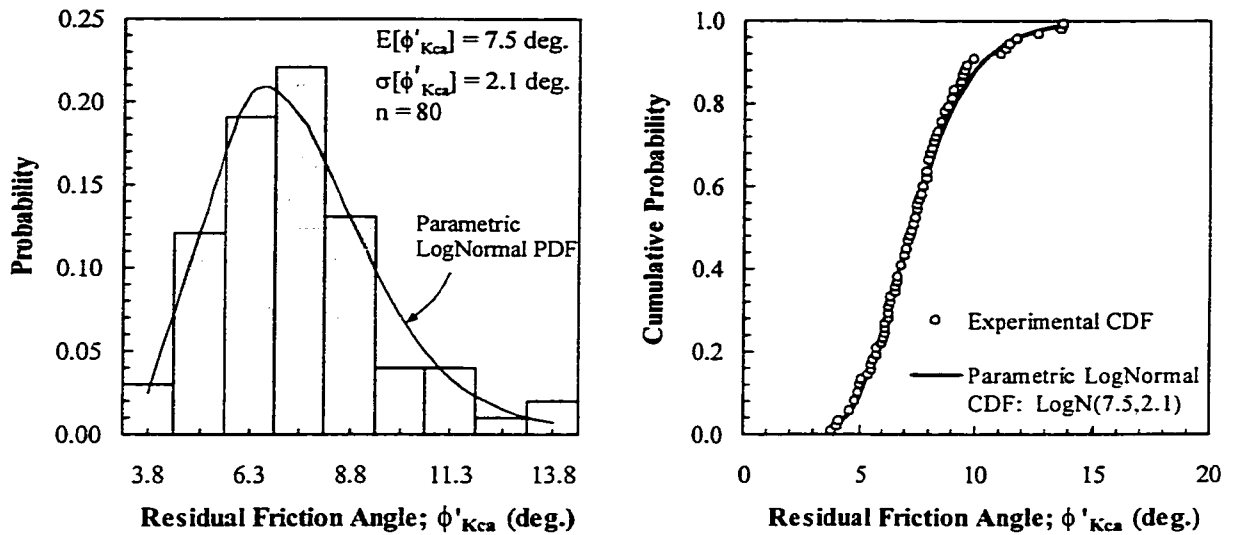
Figure 7-4 Probability histogram and cumulative distribution function of the residual friction angle of the Kca unit
