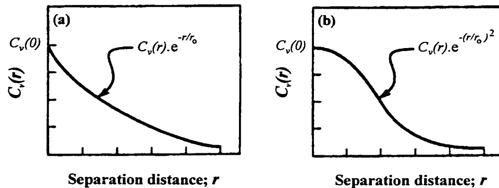
Figure 3–7 Autocovariance functions: a) Exponential; b) Gaussian (modified from DeGroot and Baecher, 1993)
