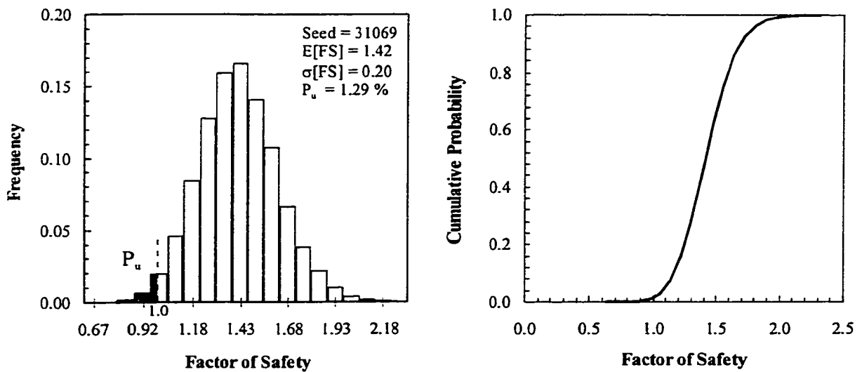
Figure 9–9 Histogram and CDF of the factor of safety, Muar Embankment (H=3.3m) – Proposed Methodology
