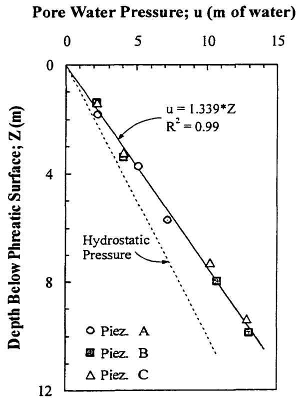
Figure 8-6 Pore pressure versus depth below phreatic surface
