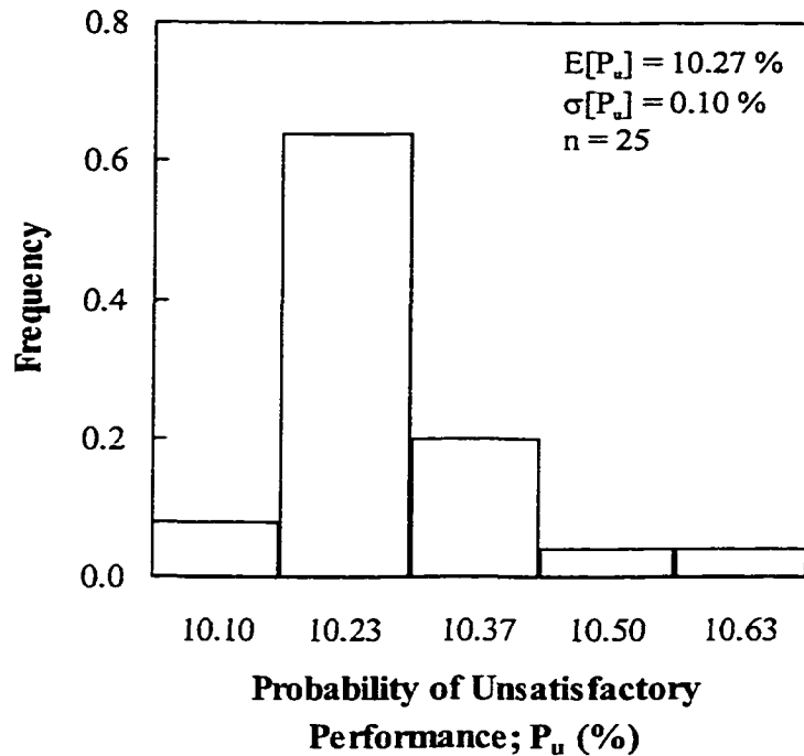
Figure 11-30 Histogram of the probability of unsatisfactory performance, Ching Cheung Road (acceptable slope) – Naïve Analysis
