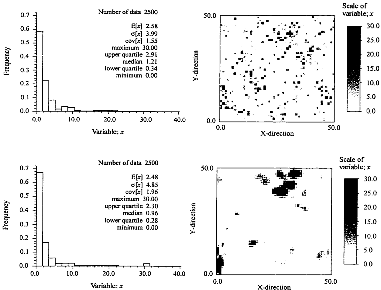
Figure 3–3 A highly erratic spatial structure (upper right) and a highly continuous structure (lower right), both with similar histograms
