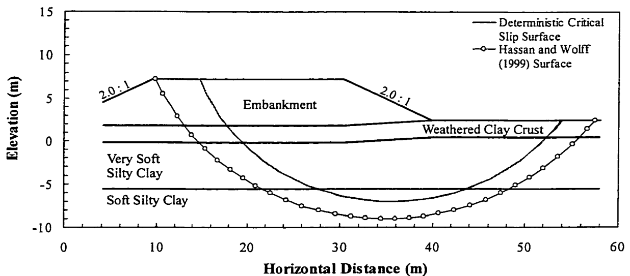
Figure 9-1 Geometry before failure and soil stratigraphy of Muar trial embankment
