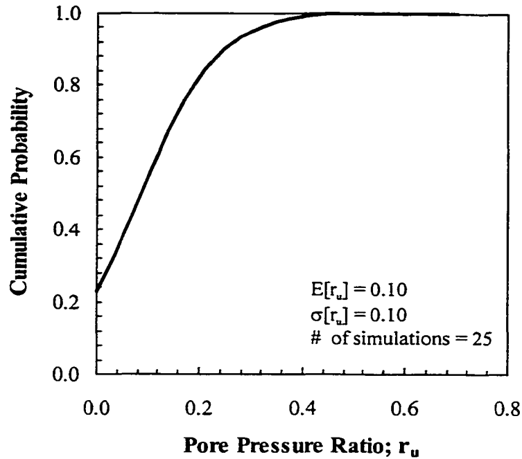
Figure 11-33 Probability distribution of pore pressure ratio at failure – Shek Kip Mei landslide
