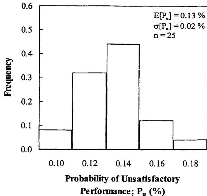
Figure 11-29 Histogram of the probability of unsatisfactory performance, Ching Cheung Road (acceptable slope) – Proposed Methodology
