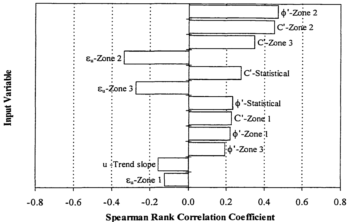
Figure 8–10 Sensitivity analysis results, Lodalen slide (2h:1v) – Proposed Methodology
