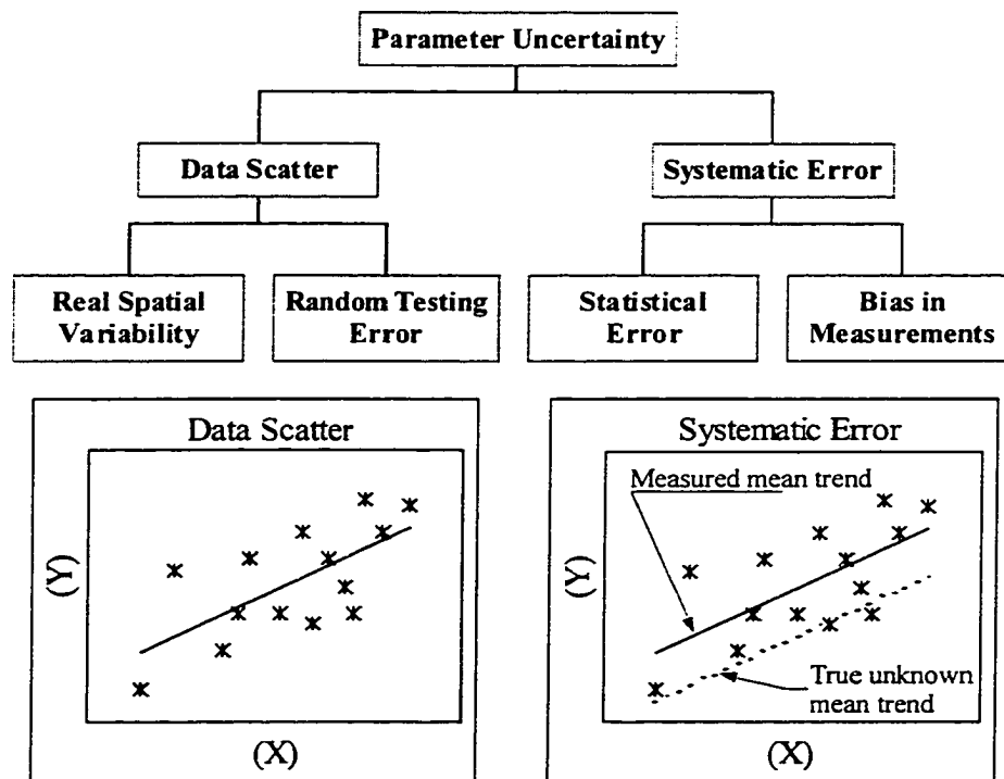
Figure 3–1 Sources of parameter uncertainty (modified from Baecher, 1987)
