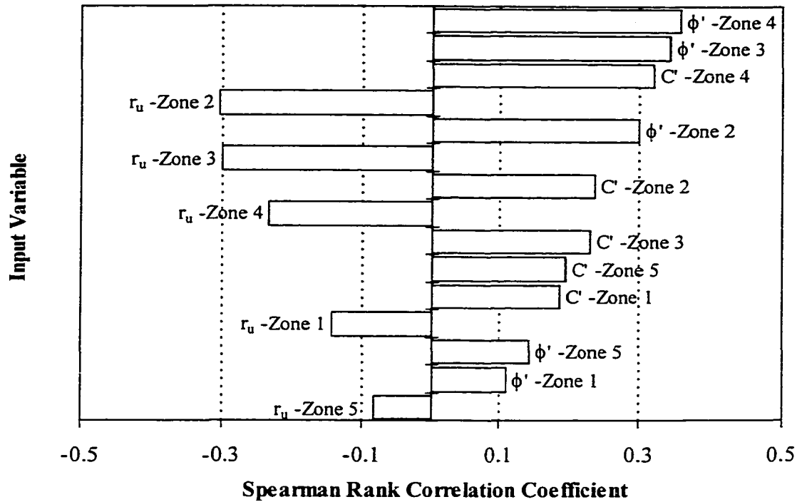
Figure 11-35 Sensitivity analysis results, Shek Kip Mei slope (acceptable design) – Proposed Methodology
