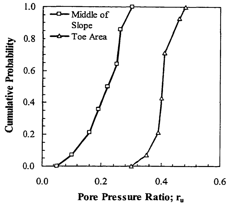
Figure 7-12 CDF of the pore pressure ratio in the Pgs layer, March 1994
