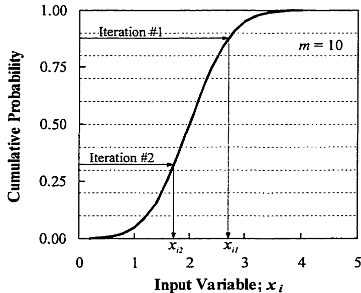
Figure 5–13 Latin Hypercube sampling with 10 iterations
