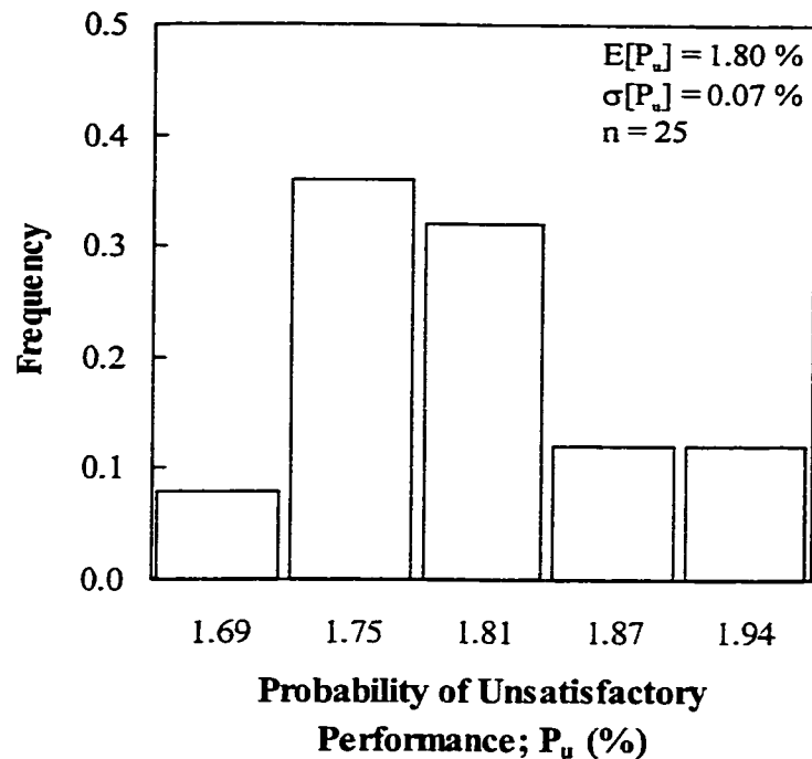
Figure 9–14 Histogram of the probability of unsatisfactory performance, Muar Embankment (H=3.3m) – Naïve Analysis
