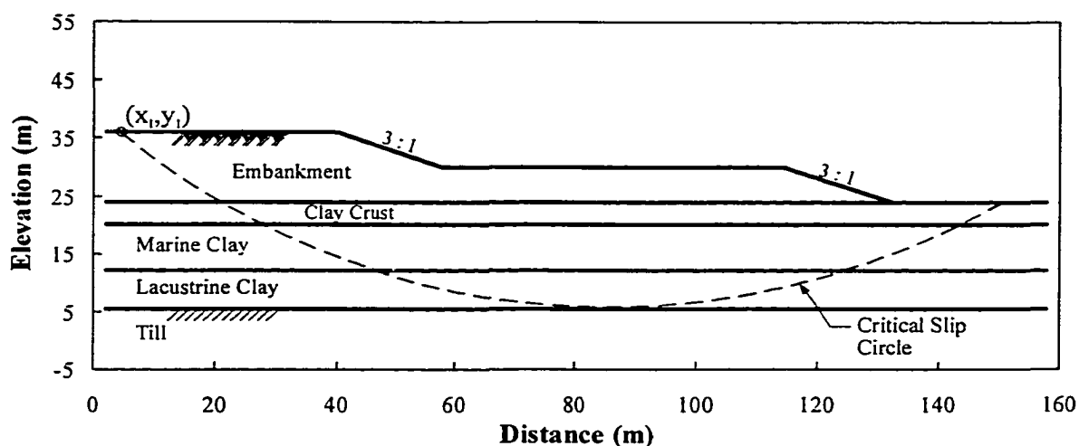
Figure 6-1 Geometry and stratigraphy of James Bay dykes; Design 1 (H = 12m)
