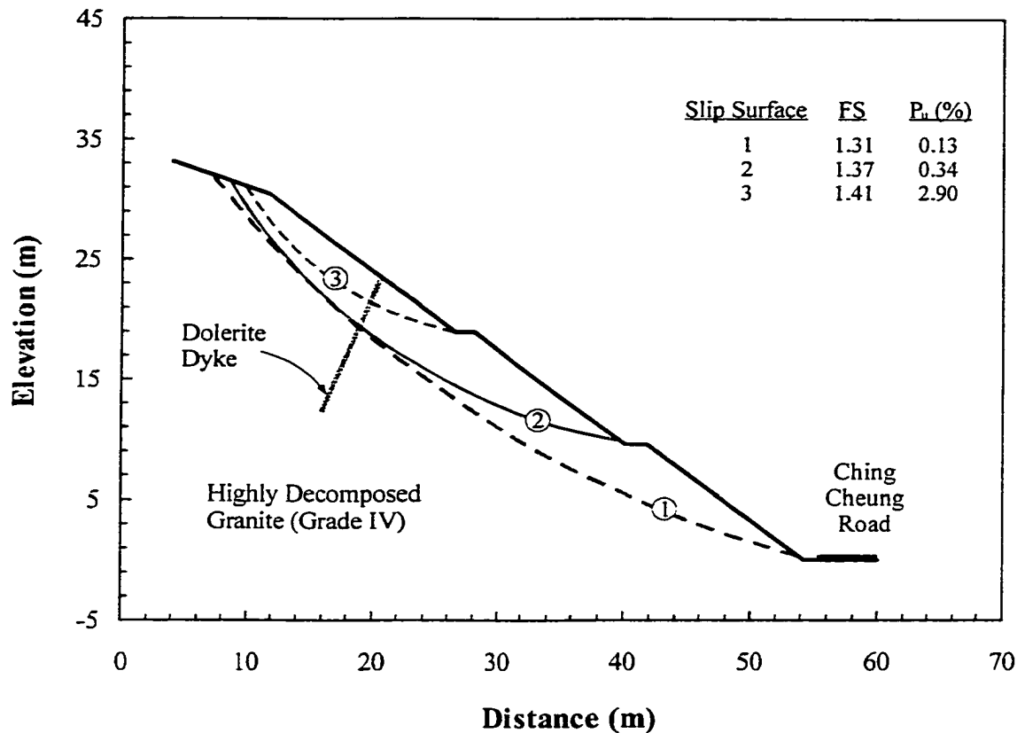
Figure 11-40 Effect of scale of failure on probability of unsatisfactory performance and factor of safety – Ching Cheung Road (acceptable design)
