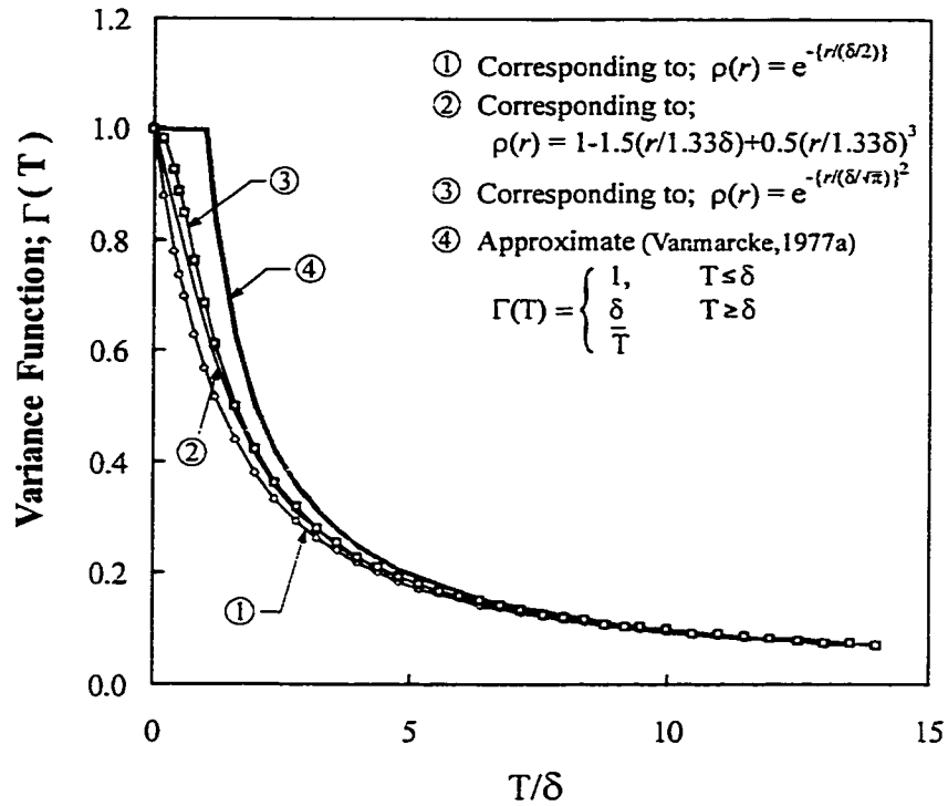
Figure 5-4 Variance function versus the averaging interval T normalized with respect to the scale of fluctuation \delta for various autocorrelation models
