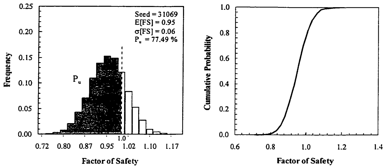
Figure 8–8 Histogram and CDF of the factor of safety, Lodalen slide (2h:1v) – Proposed Methodology
