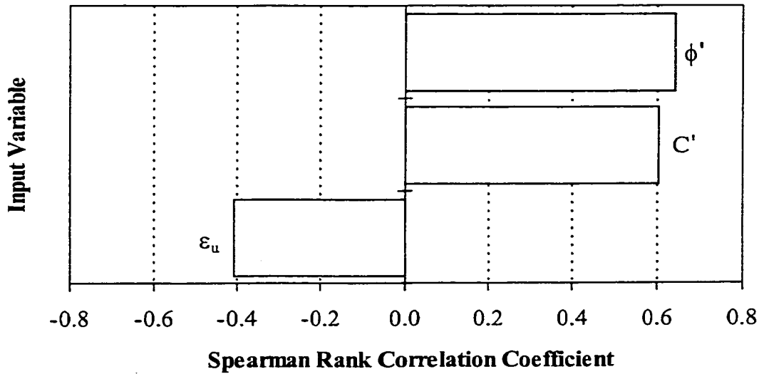
Figure 8-16 Sensitivity analysis results, Lodalen slope (4h:1v) – Naïve analysis
