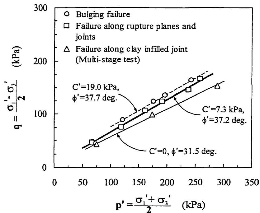
Figure 11-7 p'-q plot of the consolidated undrained (single stage) and consolidated drained triaxial tests, Cho Yiu slide
