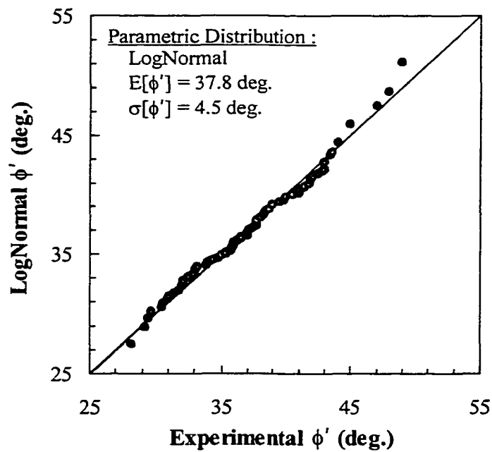
Figure 11-3 Q-Q plot of the effective friction angle of the granitic soils of Hong Kong (HDG and CDG)
