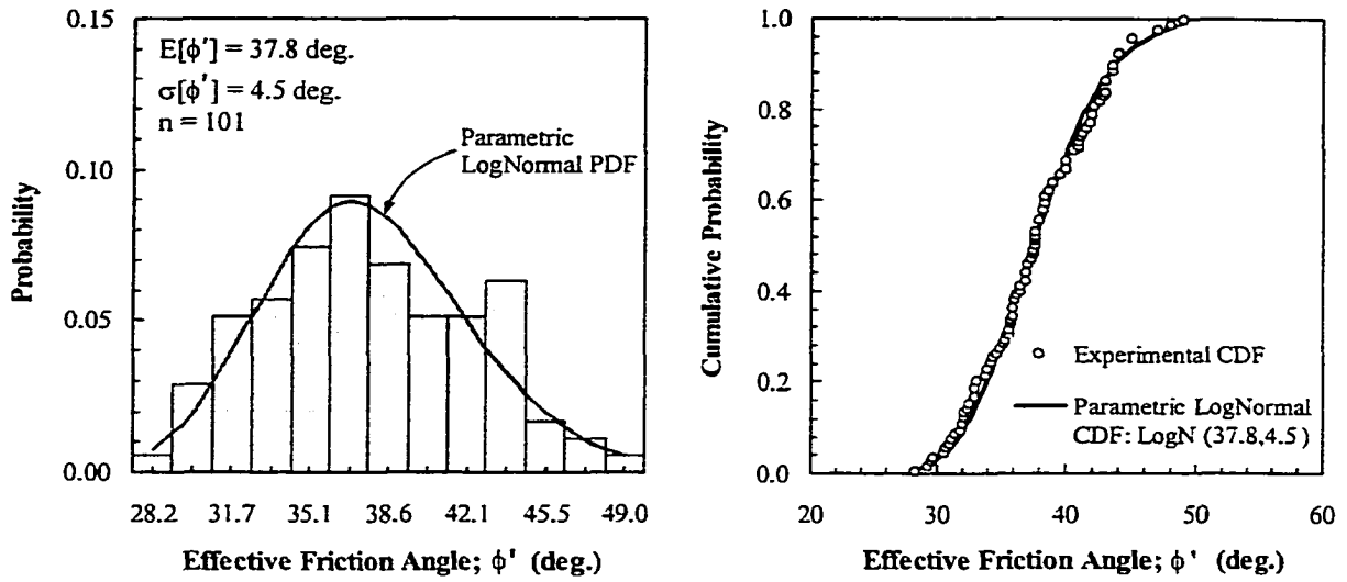
Figure 11-2 Probability histogram and CDF of the effective friction angle of the granitic soils (HDG and CDG) of Hong Kong
