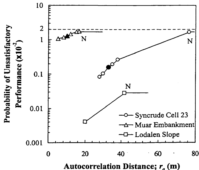
Figure 12-3 Effect of autocorrelation distance on probability of unsatisfactory performance, Safe Slopes - Soil formations exhibiting continuous spatial variability (solid symbols refer to the analyses based on the most likely r_o values, letter N refers to naïve analysis)
