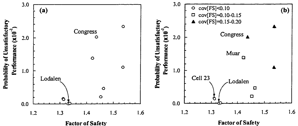
Figure 12–9 Probability of unsatisfactory performance versus factor of safety; Safe Slopes – Proposed Methodology (data are grouped by the coefficient of variation of the factor of safety in the right plot)
