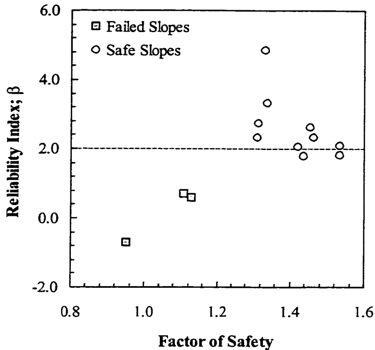
Figure 12-6 Reliability Index versus factor of safety – Proposed Methodology
