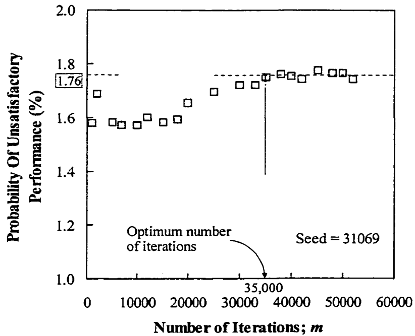
Figure 6-4 Estimating optimum number of iterations for James Bay Design 2
