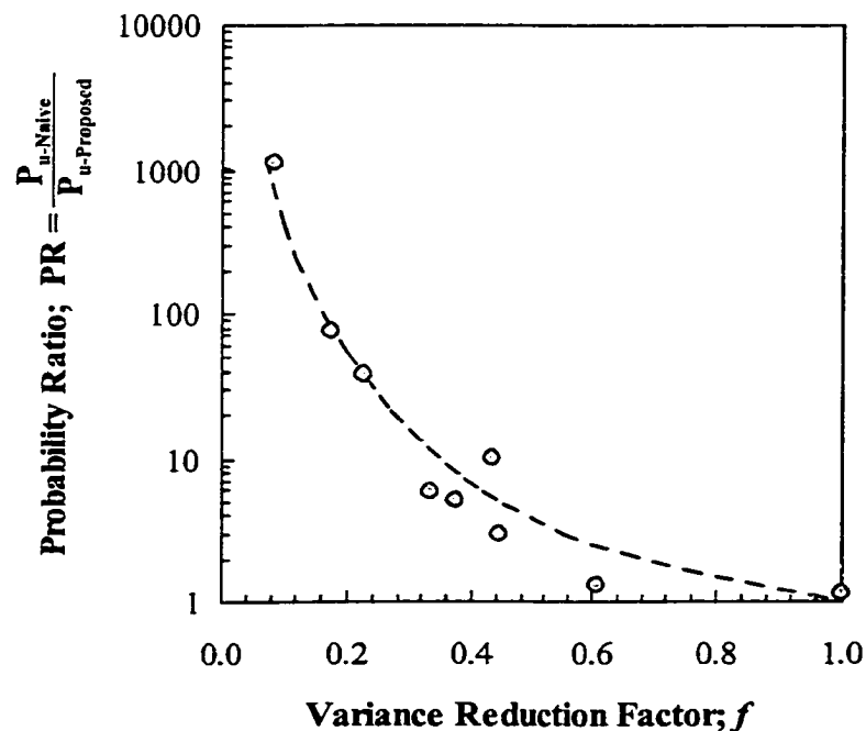
Figure 12–2 Probability ratio versus variance reduction factor
