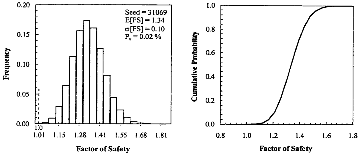
Figure 11–18 Histogram and CDF of the factor of safety, Tsing Yi: 1 slope (acceptable design) – Proposed Methodology
