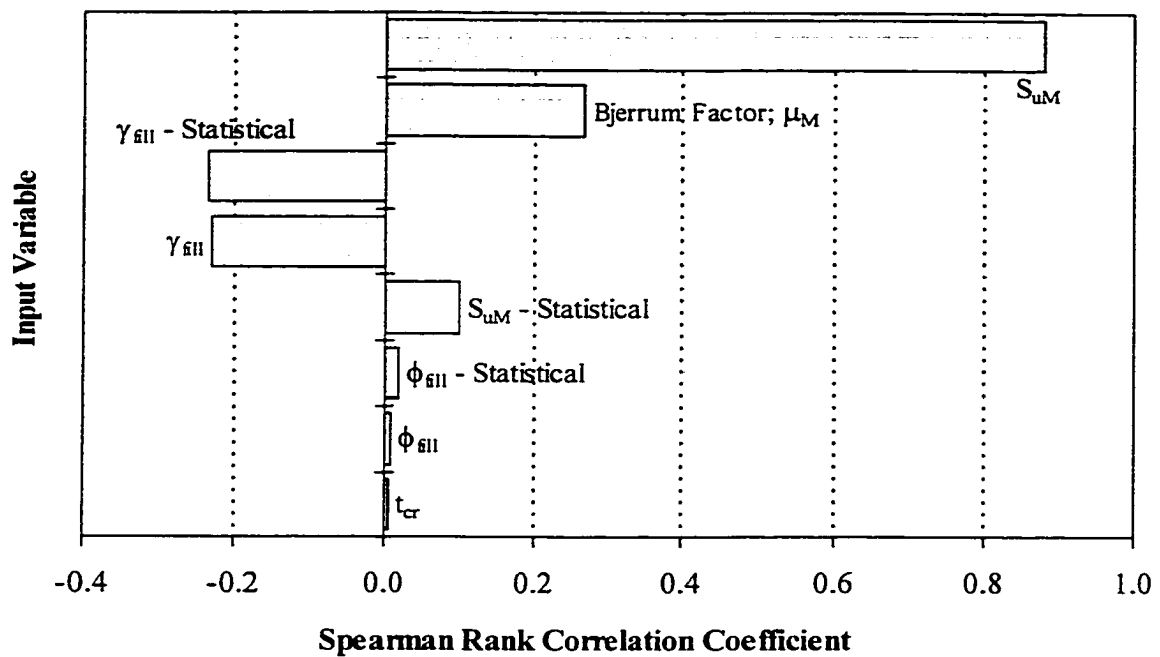
Figure 6–20 Sensitivity analysis results, Design 2 (shallow failure) – Proposed Methodology
