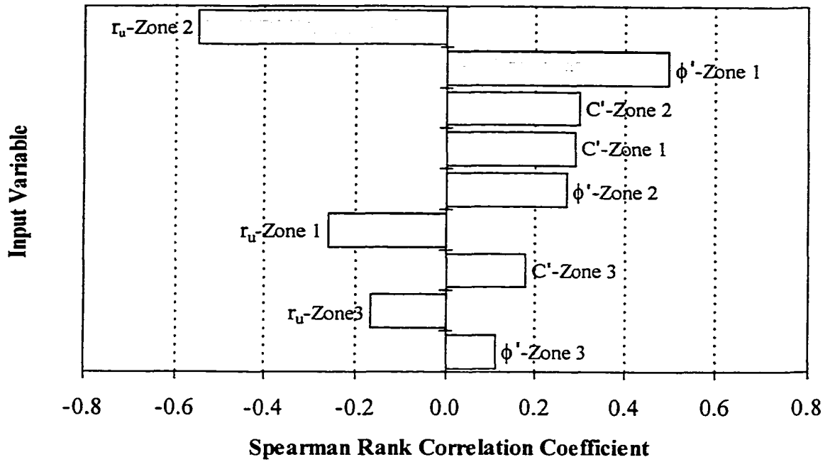
Figure 11-11 Sensitivity analysis results, Cho Yiu slope (acceptable design)
