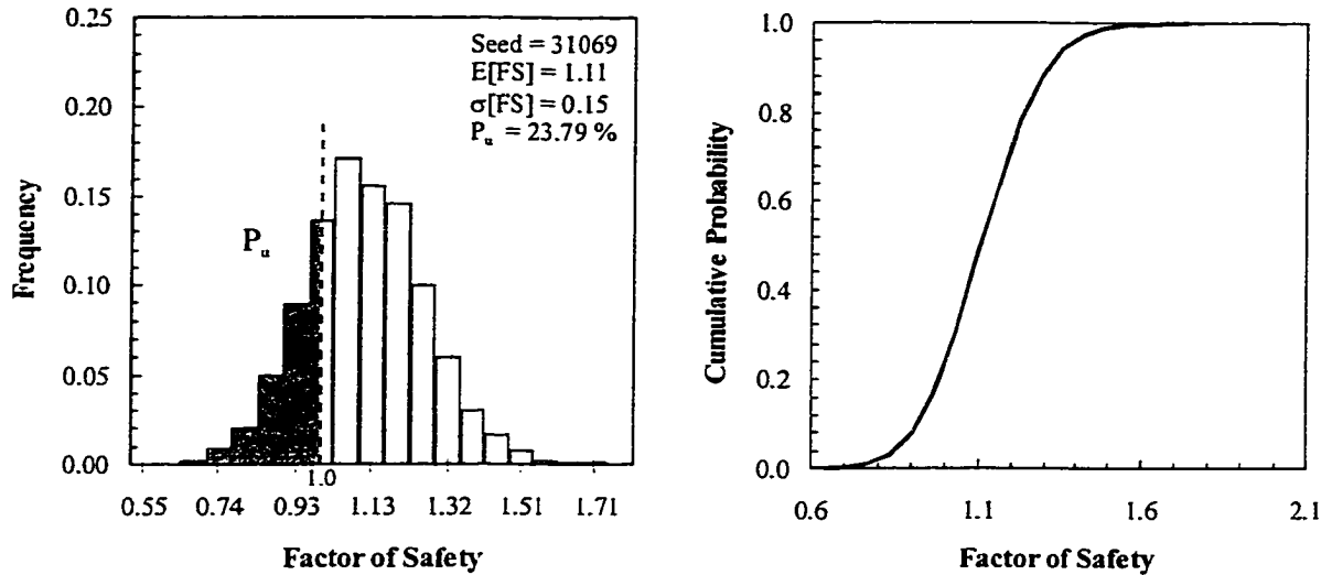
Figure 9–6 Histogram and CDF of the factor of safety, Muar Embankment (H=4.7m) – Proposed Methodology
