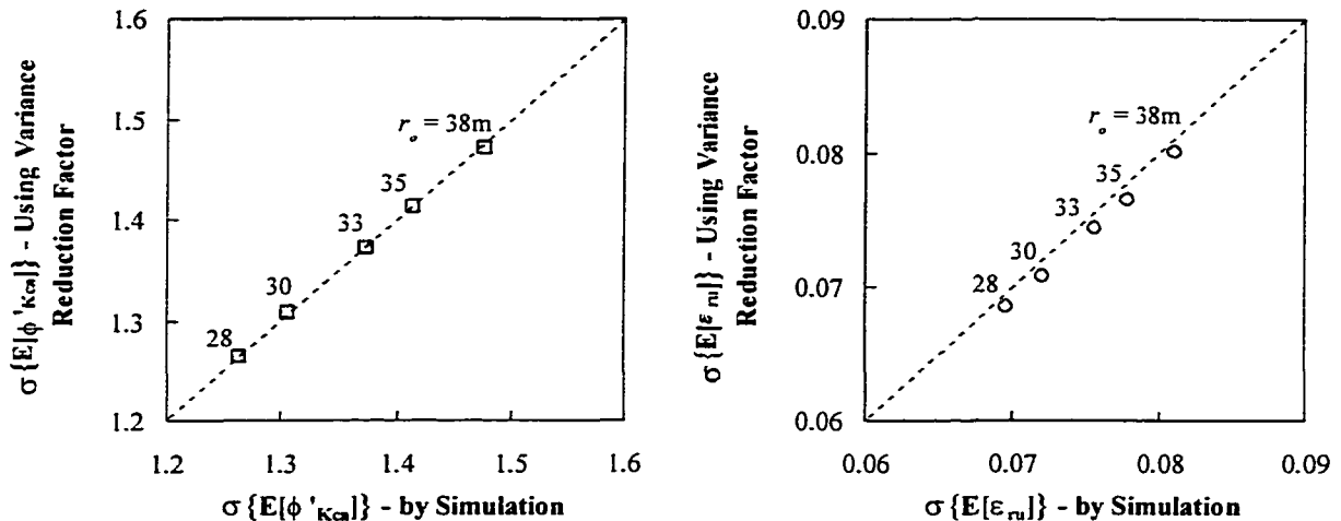
Figure 7–19 Comparing the estimates of the variances of the average friction angle and the average residual pore pressure ratio using Monte Carlo simulation and the variance reduction factor
