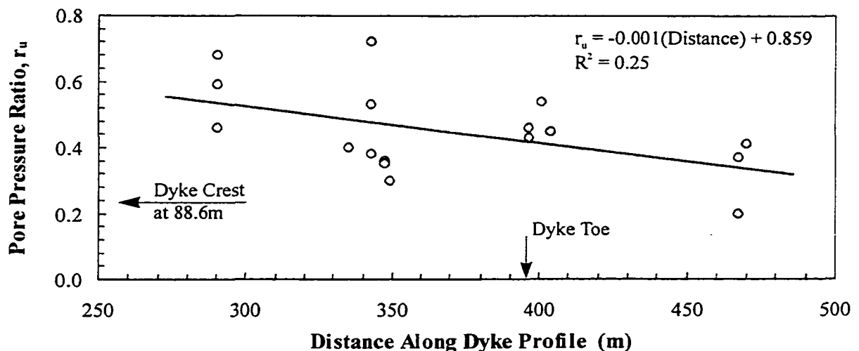
Figure 7-8 Profile of pore pressure ratio in the Kca layer along dyke cross-section, March 1994
