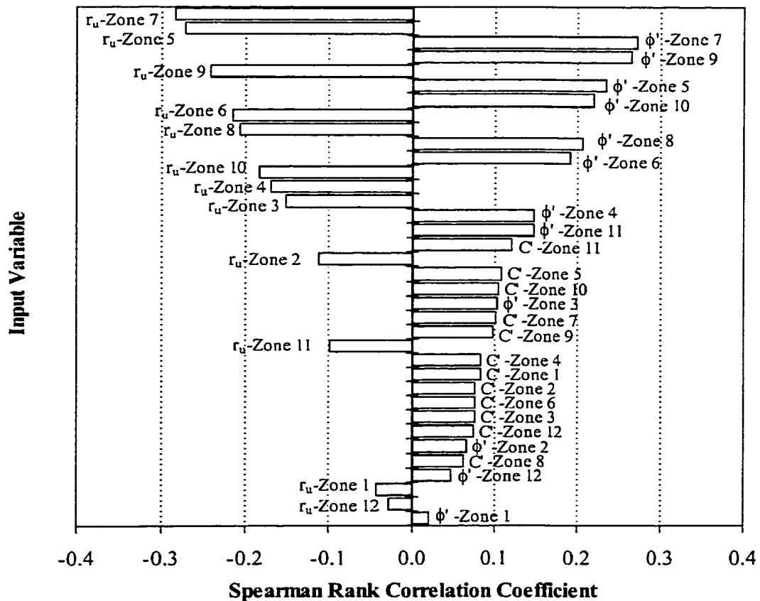
Figure 11–19 Sensitivity analysis results, Tsing Yi: 1 slope (acceptable design) – Proposed Methodology
