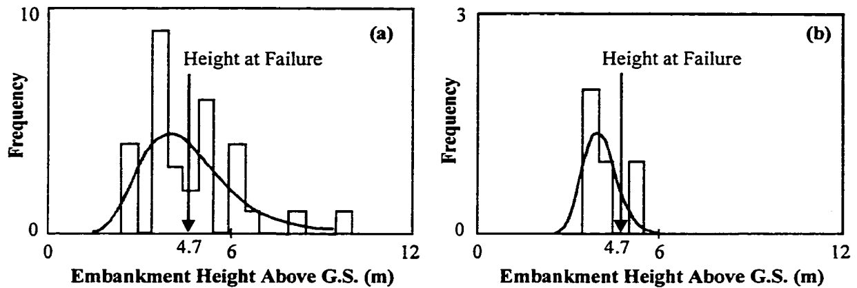
Figure 4-1 Muar Embankment : histograms of embankment height predictions; a) all 30 participants, b) four experts (modified from Kay, 1993)
