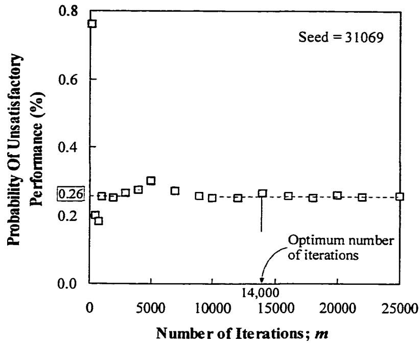
Figure 6-3 Estimating optimum number of iterations for James Bay Design 1
