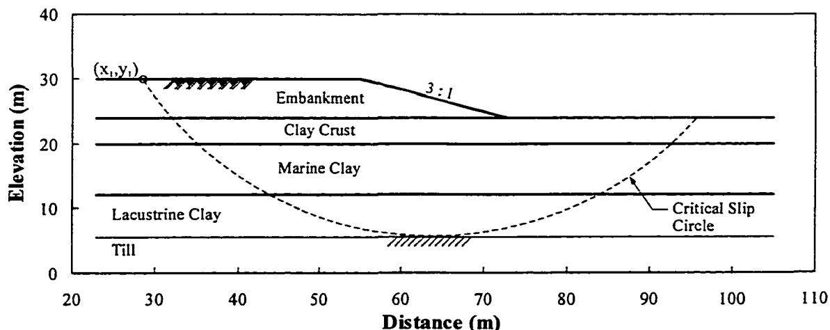
Figure 6-2 Geometry and stratigraphy of James Bay dykes; Design 2 (H = 6m)
