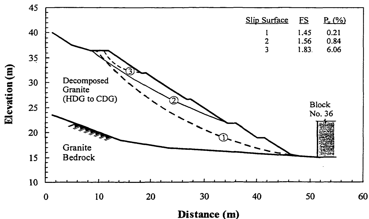
Figure 11-41 Effect of scale of failure on probability of unsatisfactory performance and factor of safety – Shek Kip Mei slope (acceptable design)
