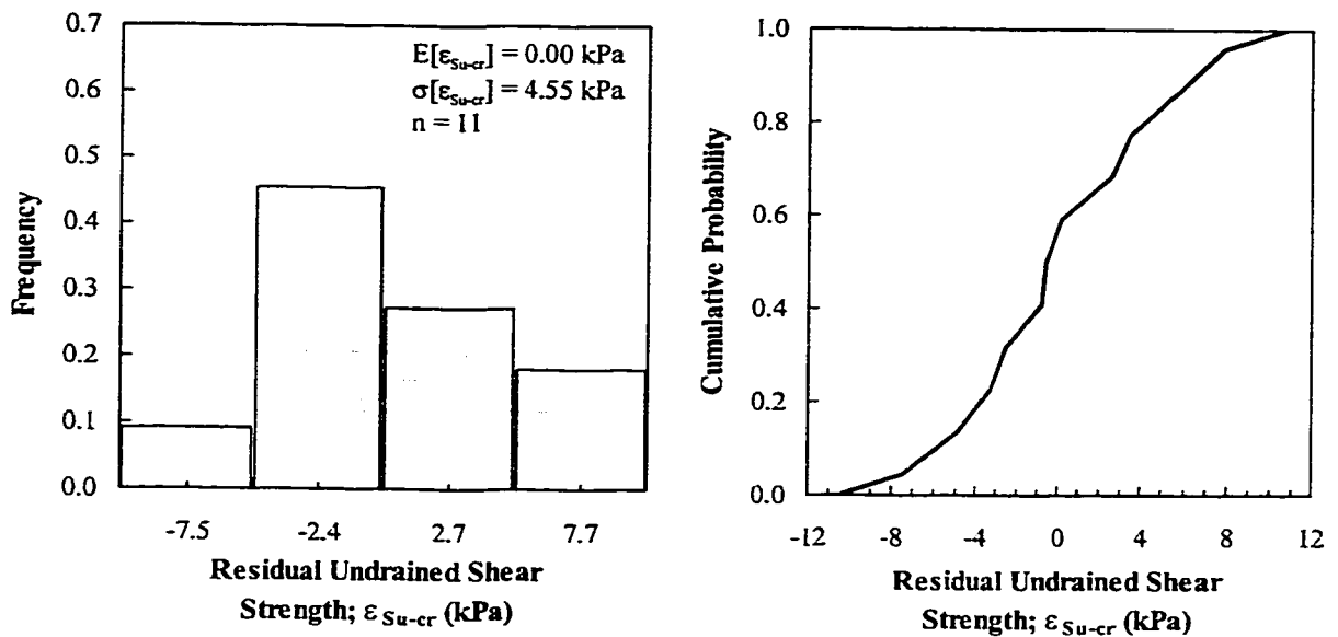
Figure 9–3 Histogram and CDF of the residuals of the undrained shear strength of the weathered clay crust
