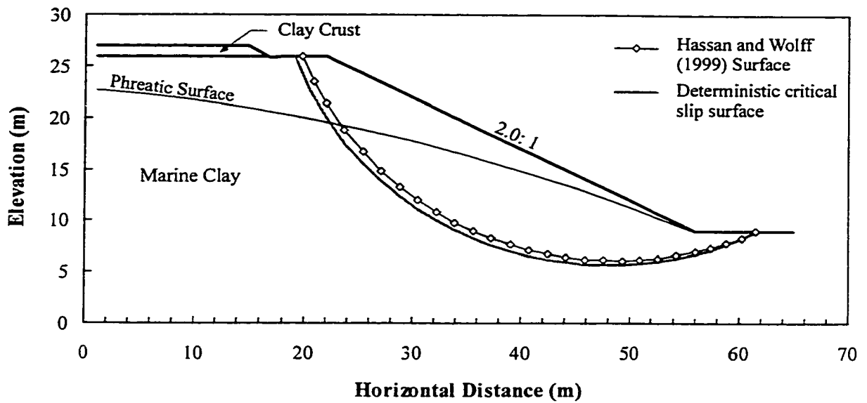
Figure 8-1 Cross-section and stratigraphy of Lodalen slide
