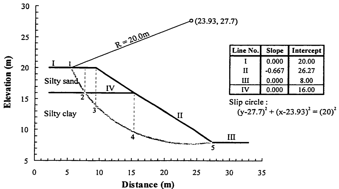
Figure 5-7 Modeling geometry, stratigraphy and slip surface
