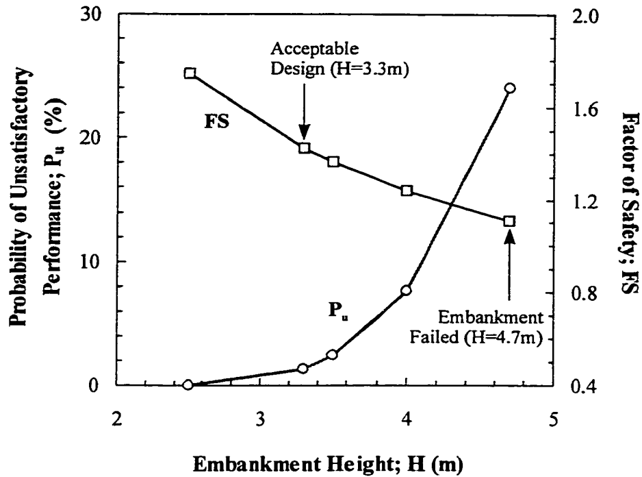
Figure 9–8 Variation of the probability of unsatisfactory performance and the factor of safety with embankment height, Muar Embankment – Proposed Methodology
