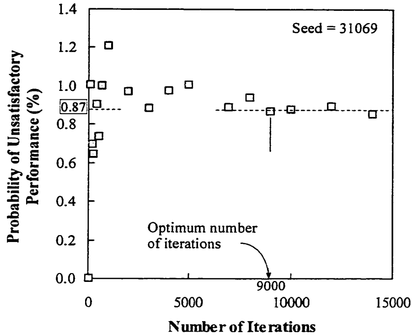
Figure 5–14 Optimum number of iterations for estimating probability of unsatisfactory performance
