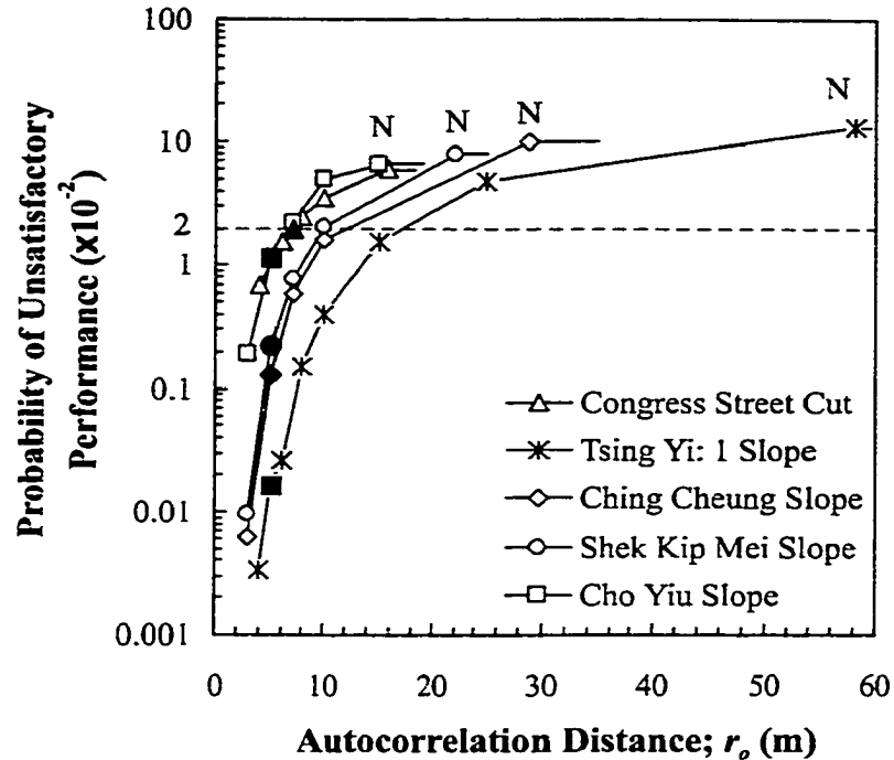
Figure 12-4 Effect of autocorrelation distance on probability of unsatisfactory performance, Safe Slopes - Soil formations exhibiting erratic spatial variability (solid symbols refer to the analyses based on the most likely r_o values, letter N refers to naïve analysis)
