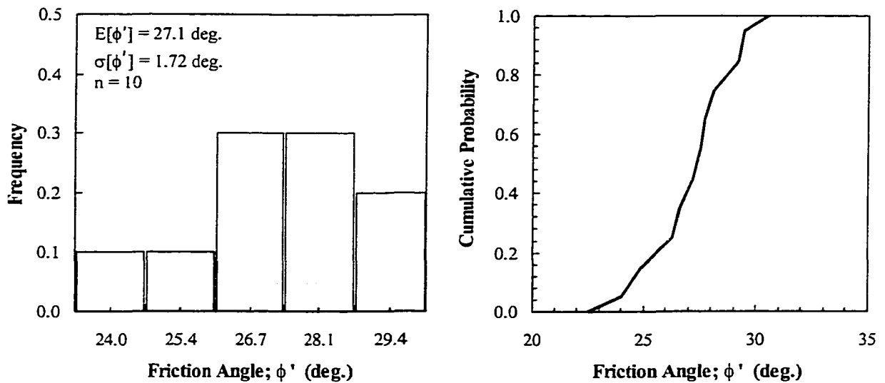
Figure 8–3 Histogram and CDF of the friction angle of the marine clay
