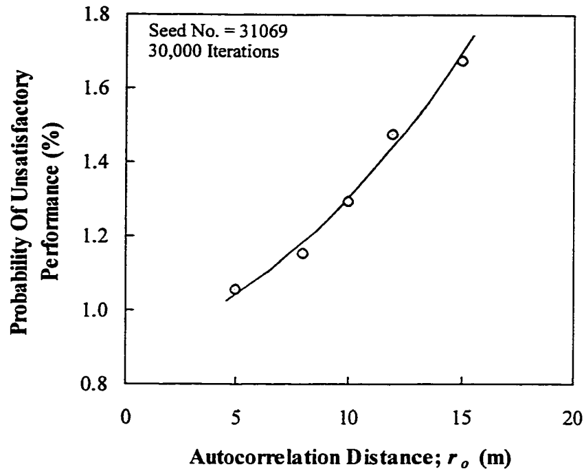
Figure 9–13 Variation of the probability of unsatisfactory performance with the autocorrelation distance, Muar Embankment (H=3.3m)
