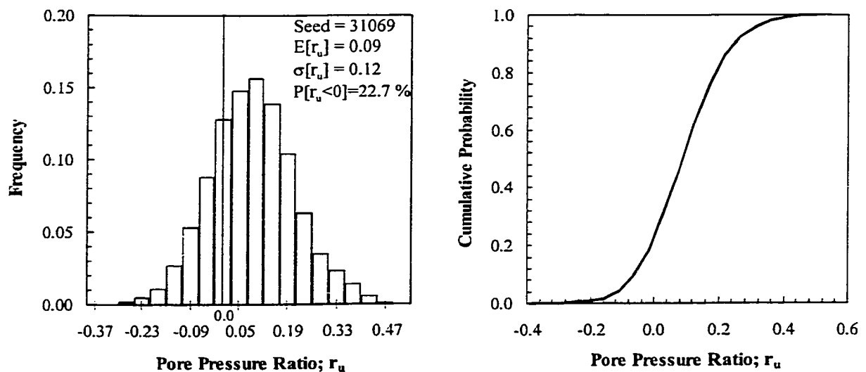
Figure 11–32 Histogram and CDF of the pore pressure ratio at failure – Shek Kip Mei landslide
