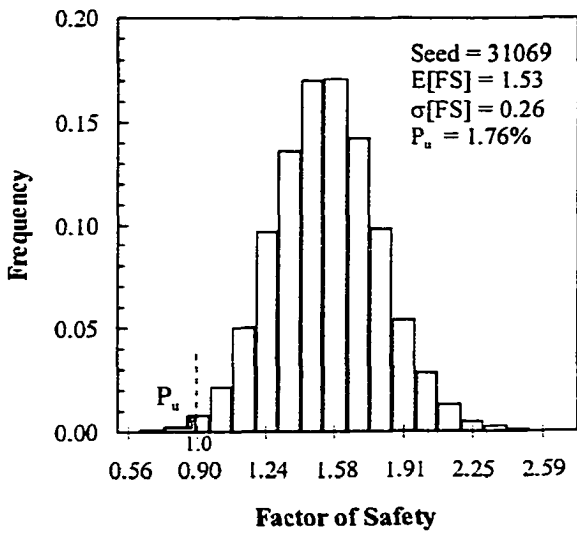
Figure 6-6 Histogram and CDF of the factor of safety, Design 2
