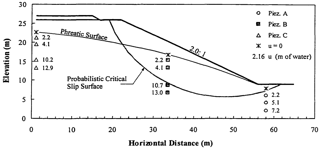
Figure 8-5 Piezometers and pore pressure measurements – Lodalen slide
