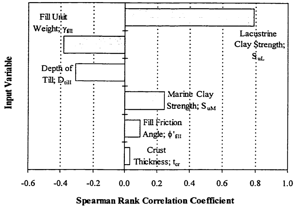
Figure 6-8 Sensitivity analysis results, Design 1
