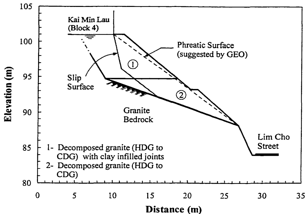
Figure 11–6 Geometry, stratigraphy and slip surface of the Cho Yiu landslide
