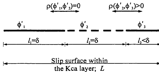
Figure 7–18 Estimating the spatial average of \phi'_{Kca} along the slip surface
