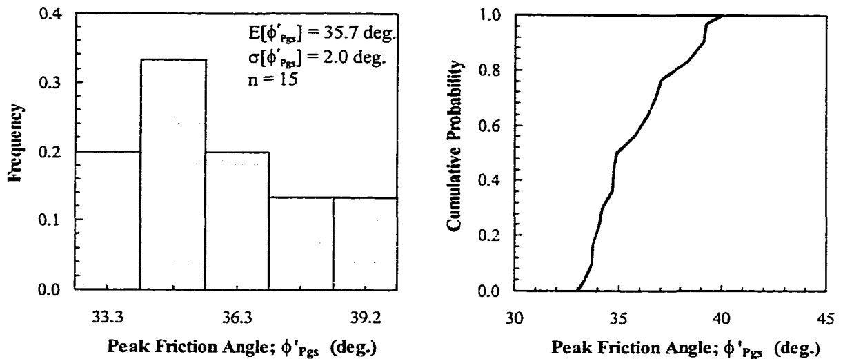
Figure 7-6 Histogram and CDF of the peak friction angle of the sandy till (Pgs) layer
