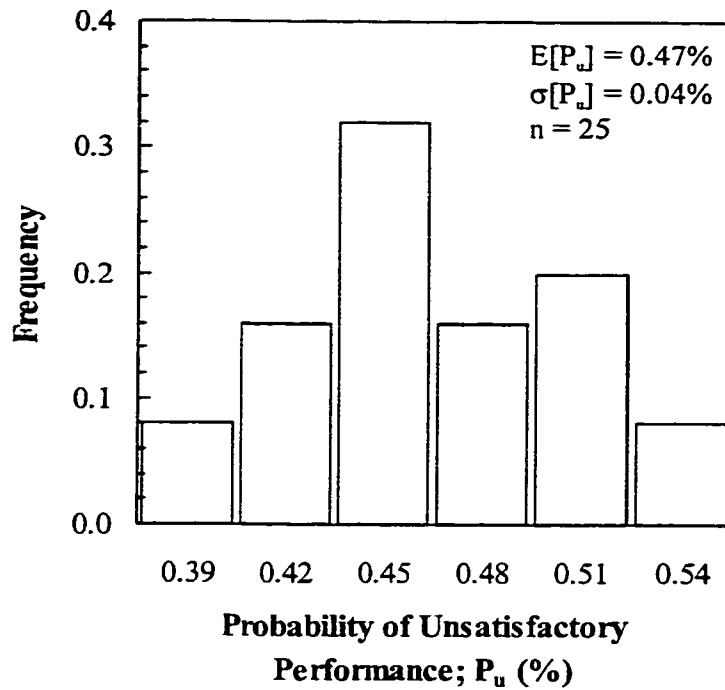
Figure 6-13 Histogram of the probability of unsatisfactory performance; Proposed Methodology; Design 1
