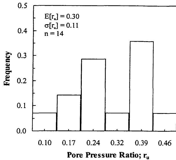
Figure 7-10 Histogram of pore pressure ratio in the sandy till, Pgs, in March 1994
