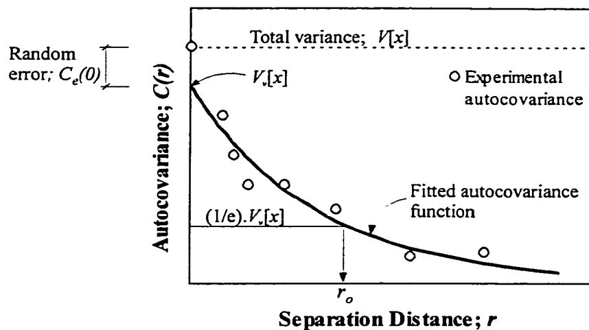
Figure 3–10 Method of Moments: estimating random error variance, C_e(0) , and autocorrelation distance, r_o
