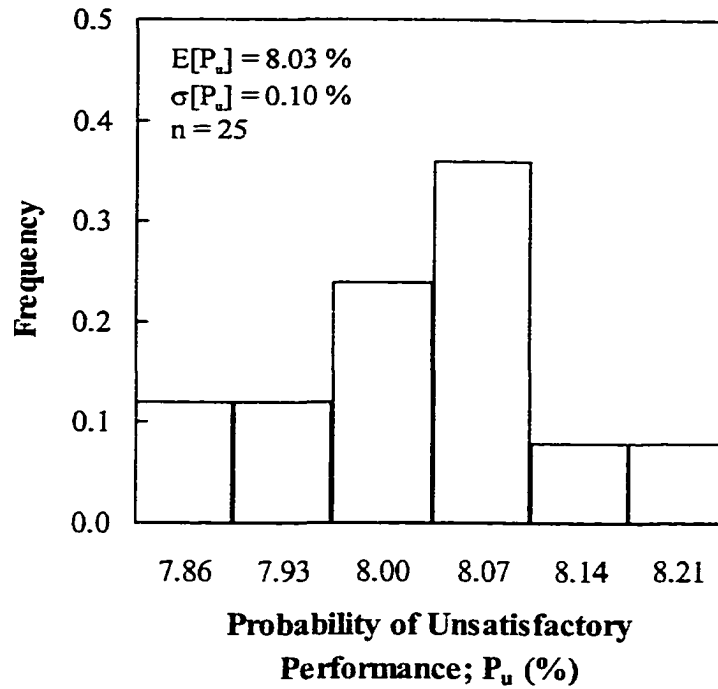
Figure 11-38 Histogram of the probability of unsatisfactory performance, Shek Kip Mei slope (acceptable design) – Naïve Analysis
