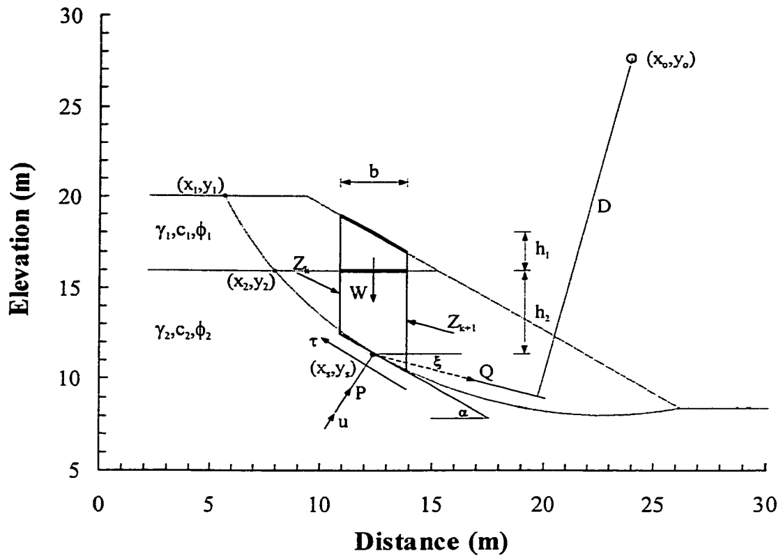
Figure 5-10 Notations and symbols used in stability analysis
