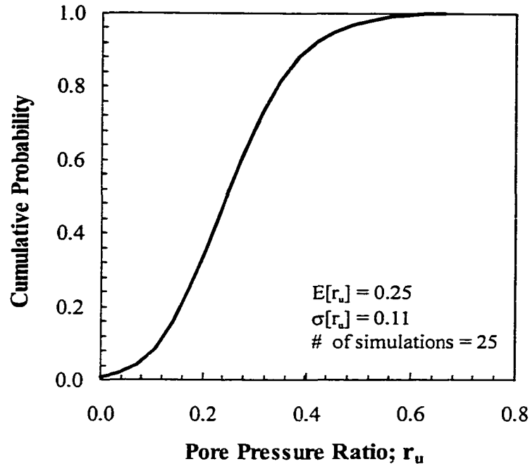
Figure 11–9 Probability distribution of pore pressure ratio at failure – Cho Yiu landslide
