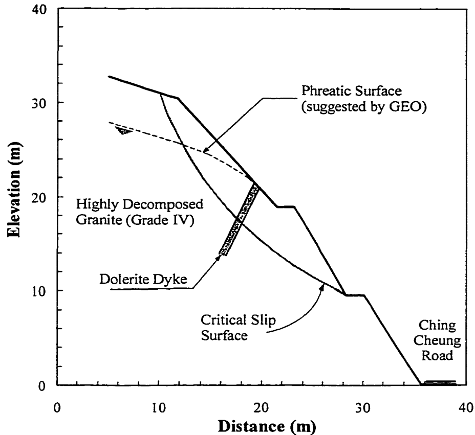
Figure 11-23 Cross-section and stratigraphy of Ching Cheung Road landslide
