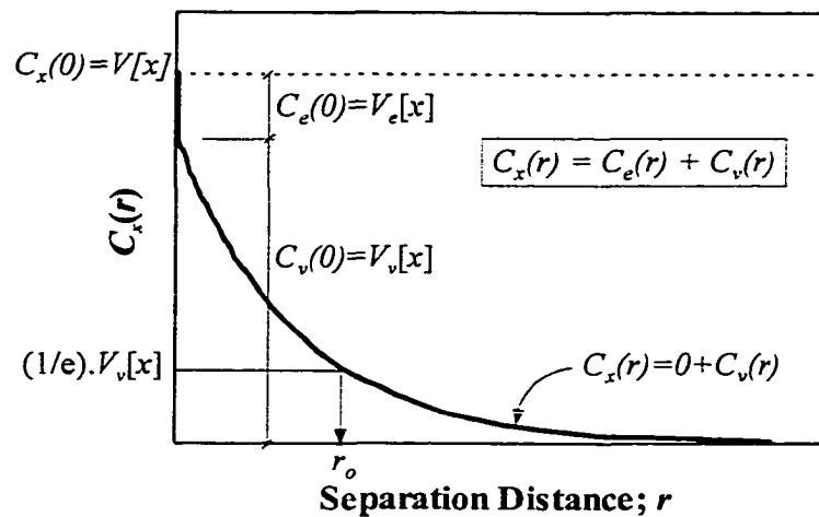
Figure 3–6 Components of autocovariance function
