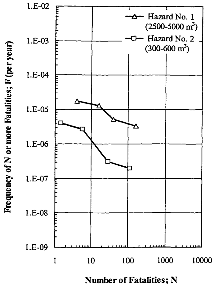
Figure 13-2 Calculated F-N curves for Hazards Nos. 1 and 2 - Shek Kip Mei slope
