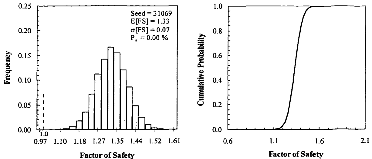
Figure 8–13 Histogram and CDF of the factor of safety, Lodalen slope (4h:1v) – Proposed Methodology
