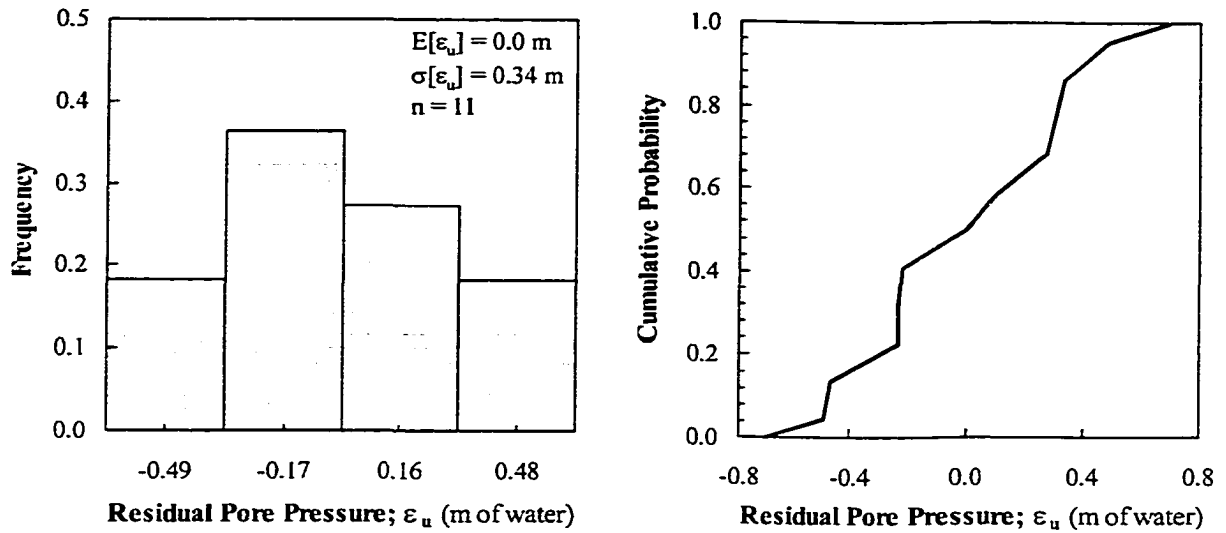
Figure 8–7 Histogram and CDF of the residual pore pressure – Lodalen slide
