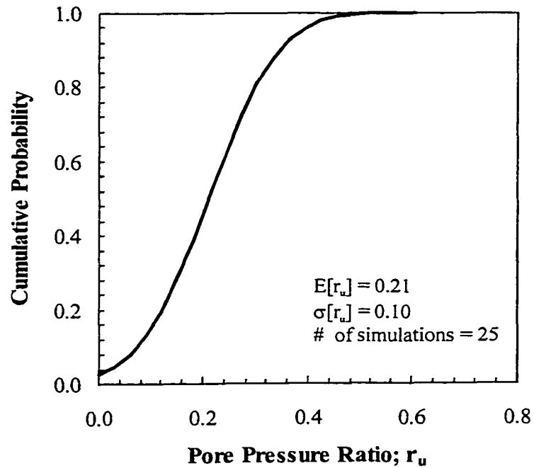
Figure 11-17 Probability distribution of pore pressure ratio at failure – Tsing Yi: 1 landslide
