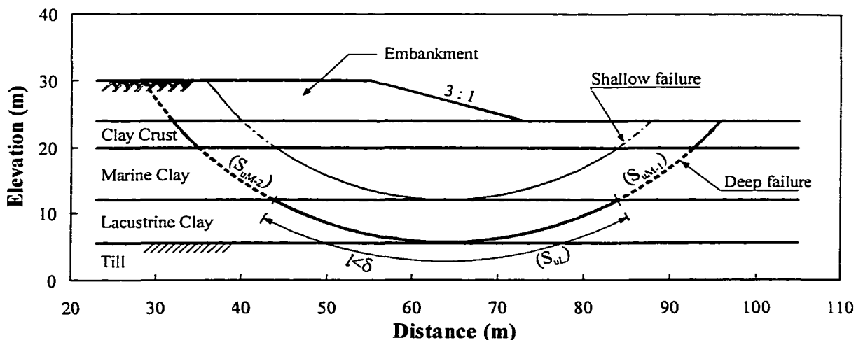
Figure 6–16 Critical slip circles and spatial averaging – Design 2
