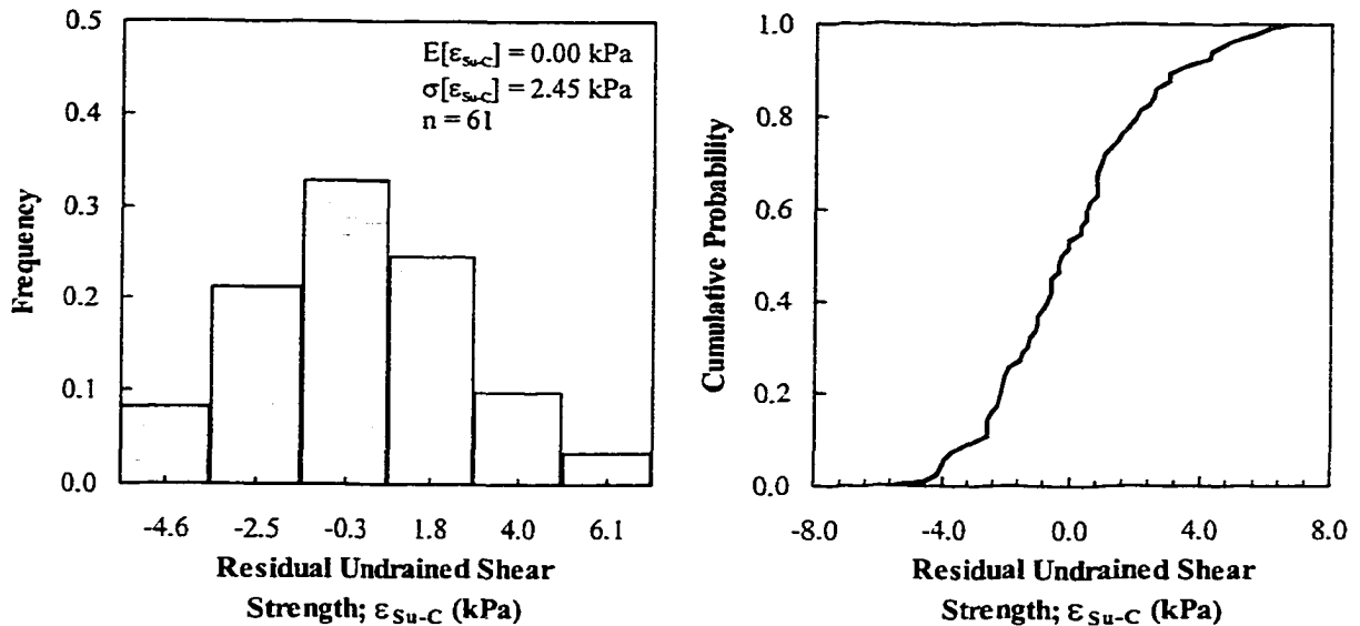
Figure 9-4 Histogram and CDF of the residuals of the undrained shear strength of the silty clay layers
