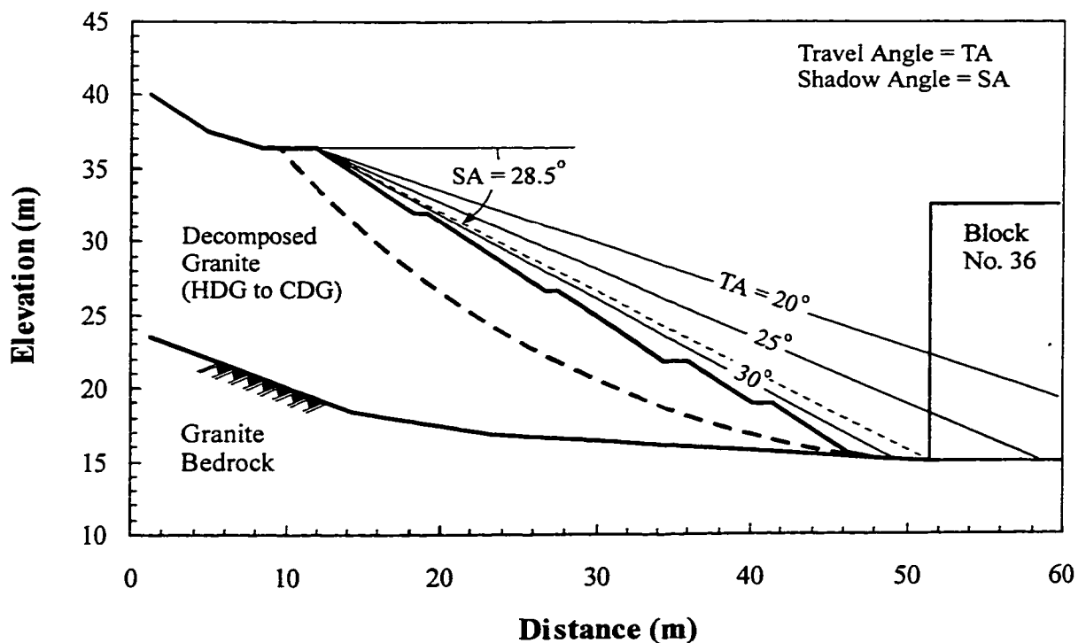
Figure 13-1 Limits of landslide debris run-outs for Hazard No. 1 relative to the location of Block 36
