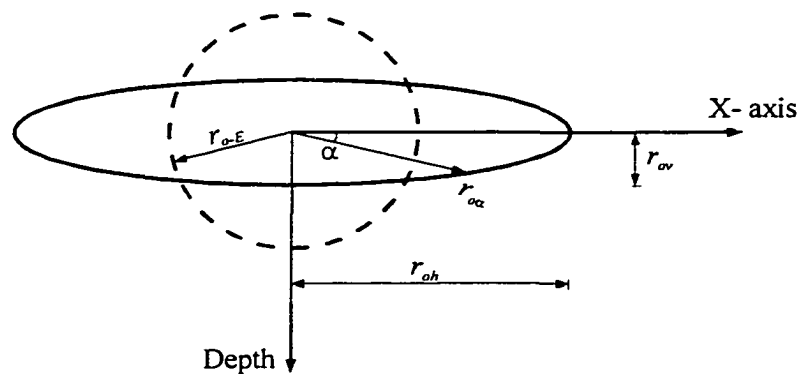
Figure 5-5 Estimation of an approximate isotropic autocorrelation distance for an anisotropic random field
