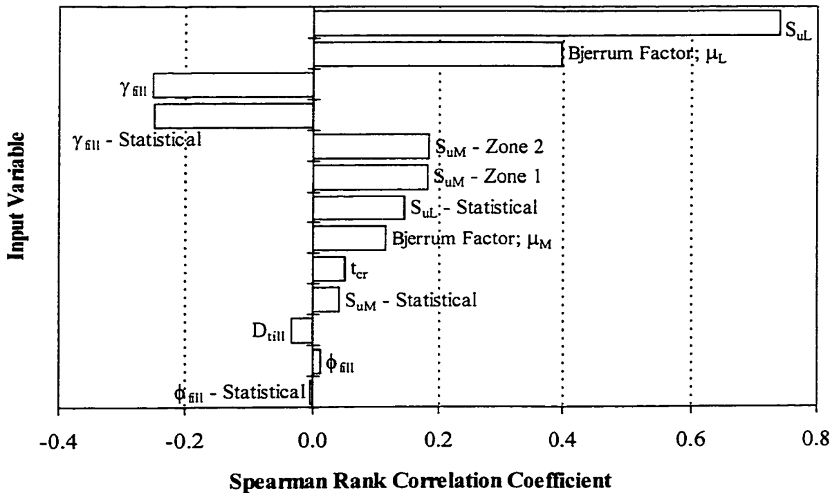
Figure 6–19 Sensitivity analysis results, Design 2 (deep failure) – Proposed Methodology
