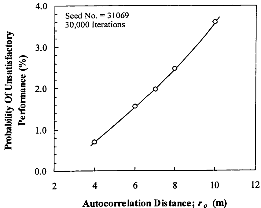
Figure 10–8 Variation of the probability of unsatisfactory performance with the autocorrelation distance, Congress Street Cut (2.5:1)
