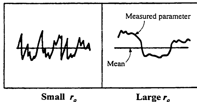
Figure 3–8 Influence of autocorrelation distance on soil variability, both plots have the same horizontal scale
