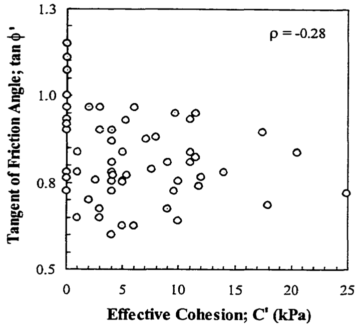
Figure 11-5 Scatter plot of tangent of friction angle and effective cohesion, Hong Kong granitic soils (HDG and CDG)
