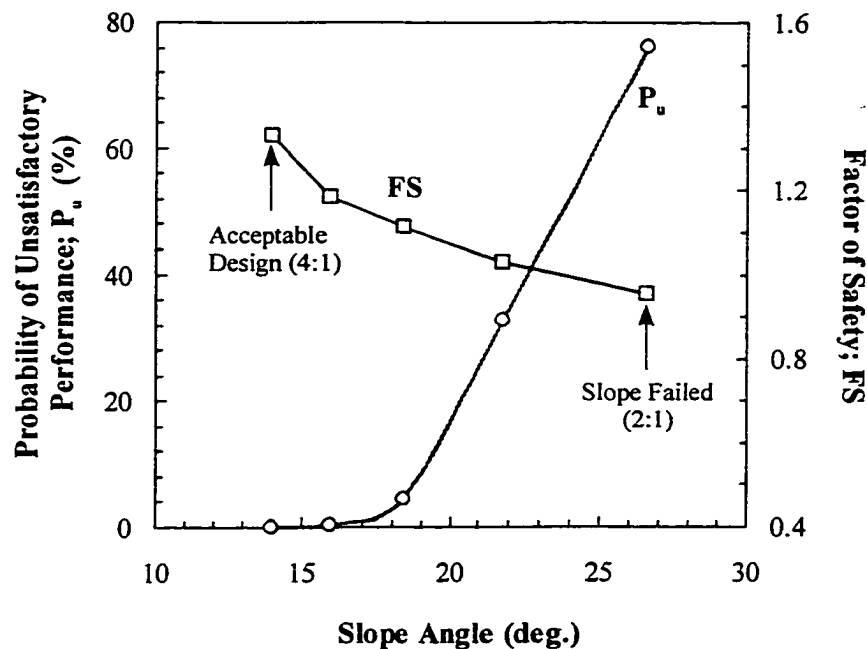
Figure 8–12 Variation of the probability of unsatisfactory performance and the factor of safety with the slope angle, Lodalen slope – Proposed Methodology
