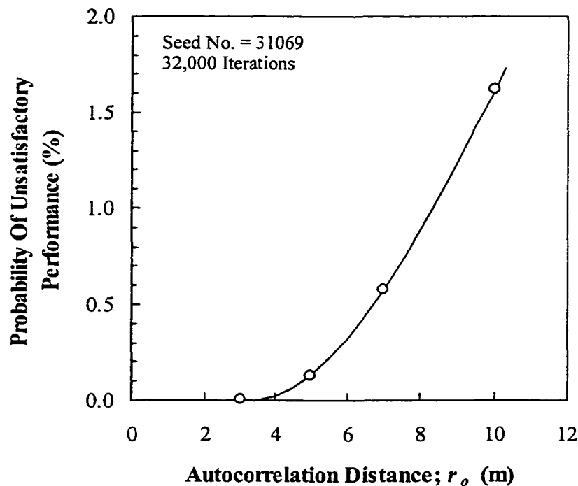
Figure 11–28 Variation of the probability of unsatisfactory performance with the autocorrelation distance, Ching Cheung Road (acceptable design)
