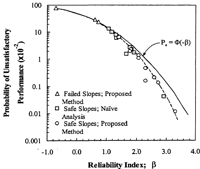
Figure 12–8 Relationship between probability of unsatisfactory performance and reliability index
