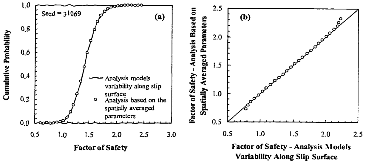
Figure 9–12 Comparison of the factor of safety from the analysis modeling soil variability along slip surface and that based on the spatially averaged parameters, Muar Embankment; a) Probability distribution functions, b) Q-Q plot
