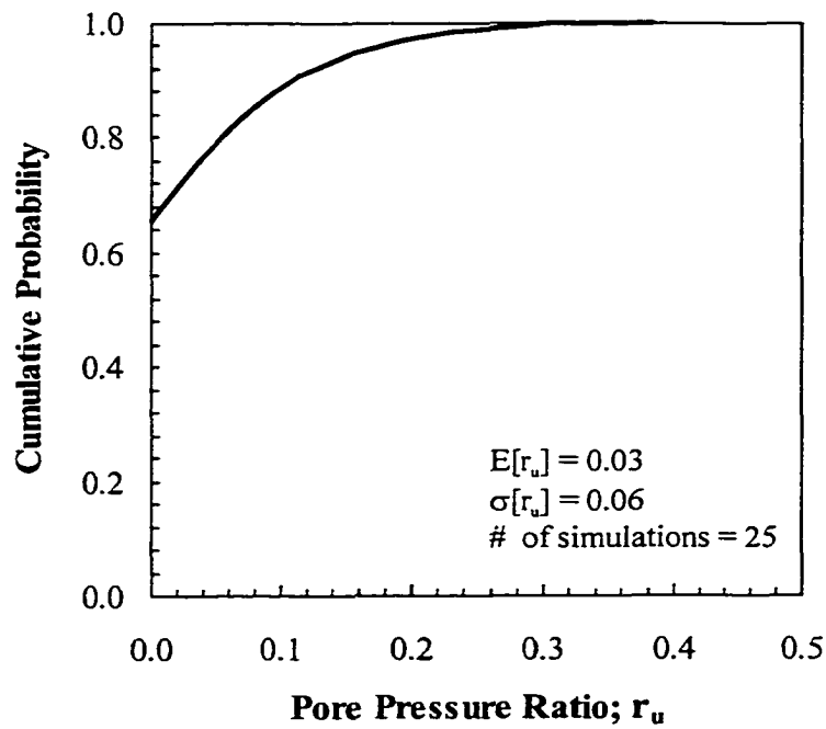
Figure 11-25 Probability distribution of pore pressure ratio at failure – Ching Cheung Road landslide
