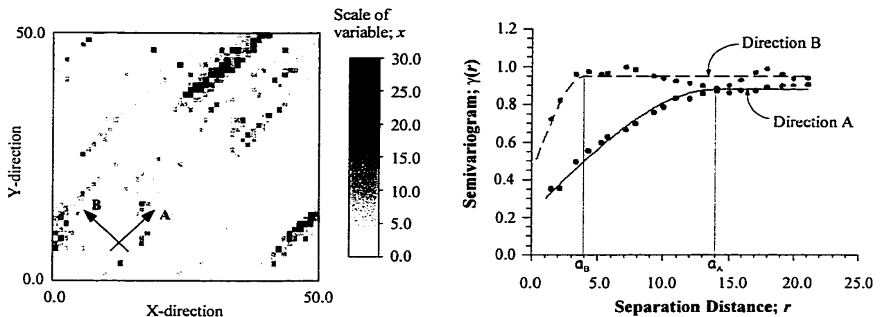
Figure 3–12 Spatial structures in different directions for anisotropic data generated using GSLIB software (Deutsch and Journel, 1998)
