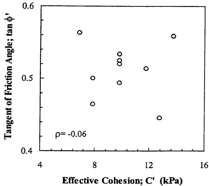
Figure 8–4 Scatter plot of C' and \tan \phi'
