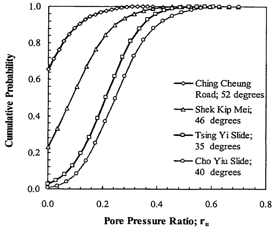
Figure 11-42 Comparison between probability distributions of the pore pressure ratios at failure for all the analyzed case studies
