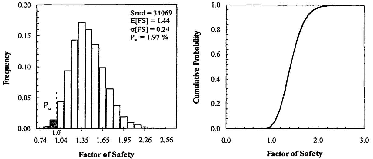
Figure 10-5 Histogram and CDF of the factor of safety, Congress Street Cut (2.5:1) – Proposed Methodology
