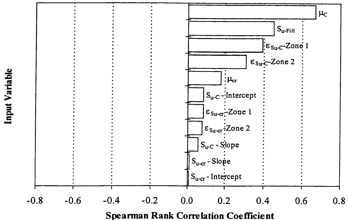
Figure 9–11 Sensitivity analysis results, Muar Embankment (H=3.3m) – Proposed Methodology
