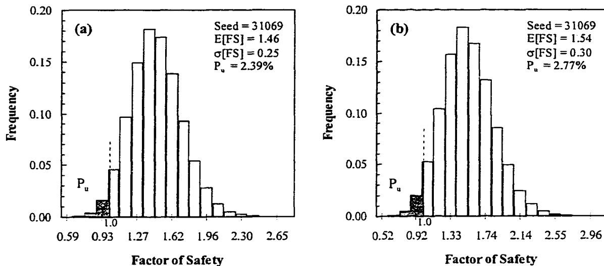
Figure 6-21 Histograms of the factor of safety – Naïve analysis : a) Design 1; b) Design 2
