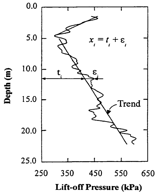
Figure 3-4 Model of spatial variability; Dilatometer lift-off pressure at the University of Massachusetts-Amherst National Geotechnical Experimental Test Site (modified from DeGroot, 1996)
