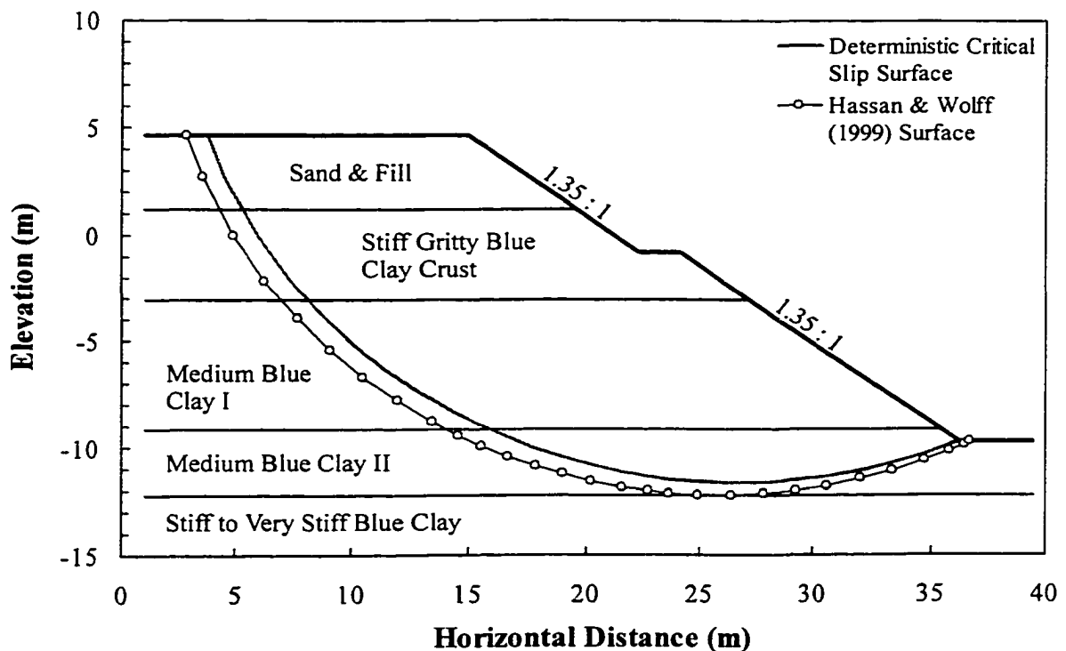
Figure 10-1 Geometry and soil stratigraphy of the Congress Street open cut
