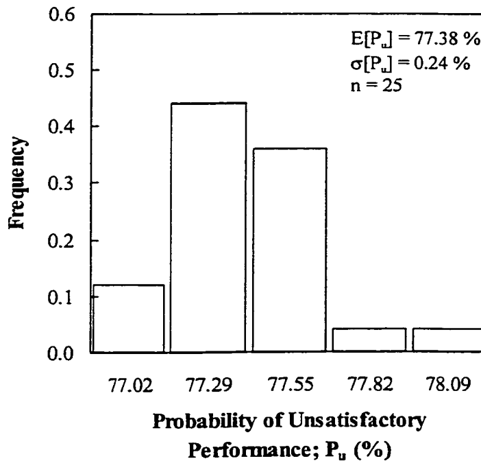
Figure 8–9 Histogram of the probability of unsatisfactory performance; Lodalen slide (2h:1v) – Proposed methodology
