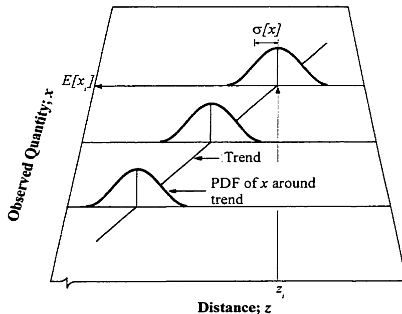
Figure 3-5 Model of soil variability (modified from Neter et al., 1990)
