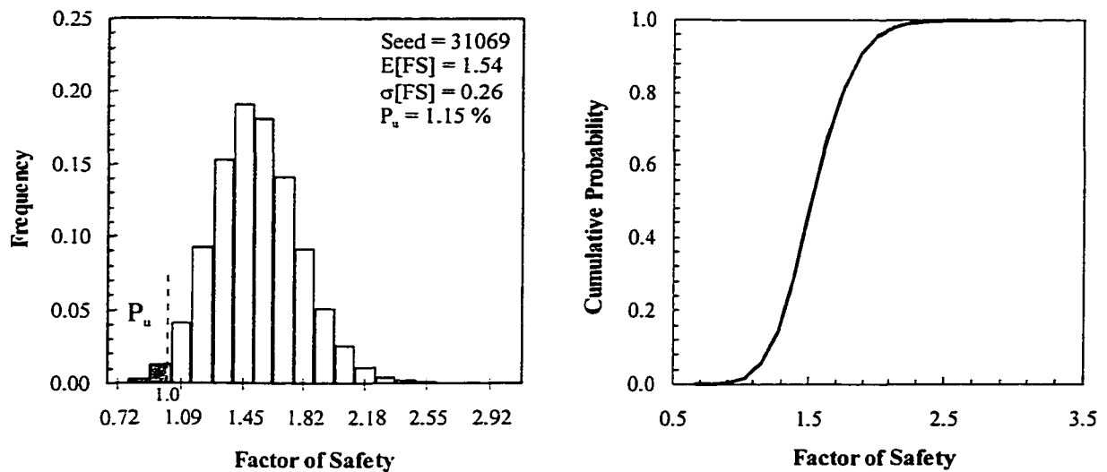
Figure 11–10 Histogram and CDF of the factor of safety, Cho Yiu slope (acceptable design) – Proposed Methodology
