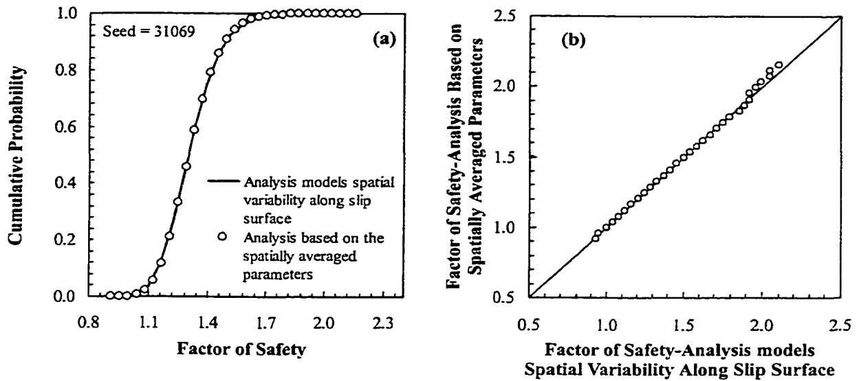
Figure 7-20 Comparison of the CDFs of the factor of safety from the analysis modeling spatial variability along slip surface and that based on the spatially averaged parameters – Cell 23; a) Probability distribution functions, b) Q-Q plot
