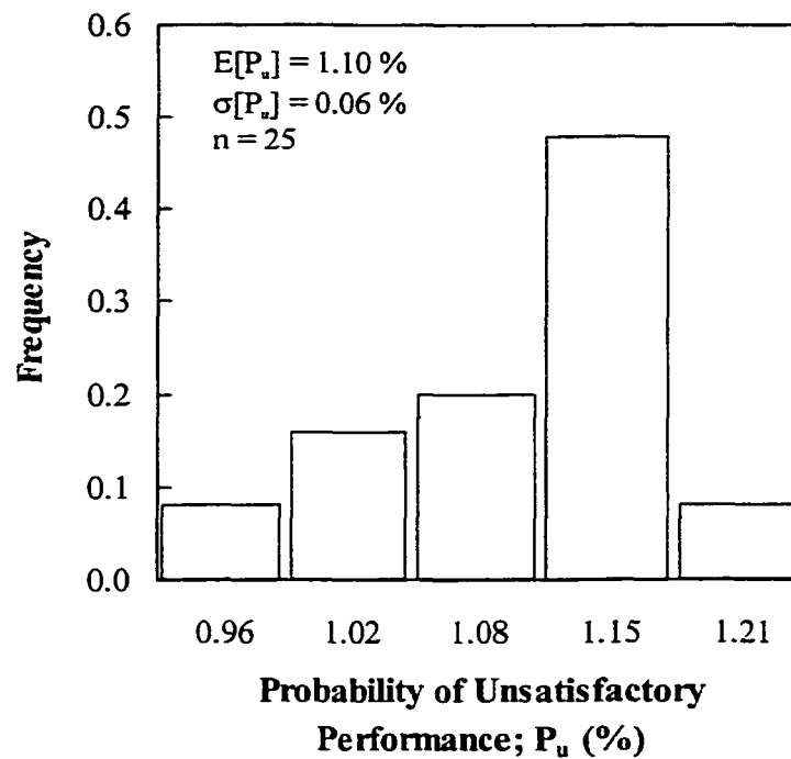
Figure 11–13 Histogram of the probability of unsatisfactory performance, Cho Yiu slope (acceptable design) – Proposed Methodology
