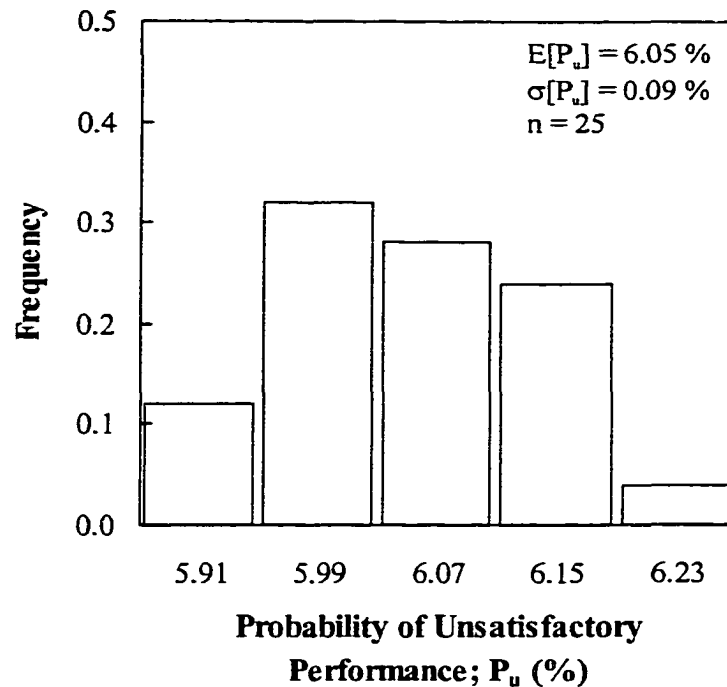
Figure 10-9 Histogram of the probability of unsatisfactory performance, Congress Street Cut (2.5:1) – Naïve Analysis
