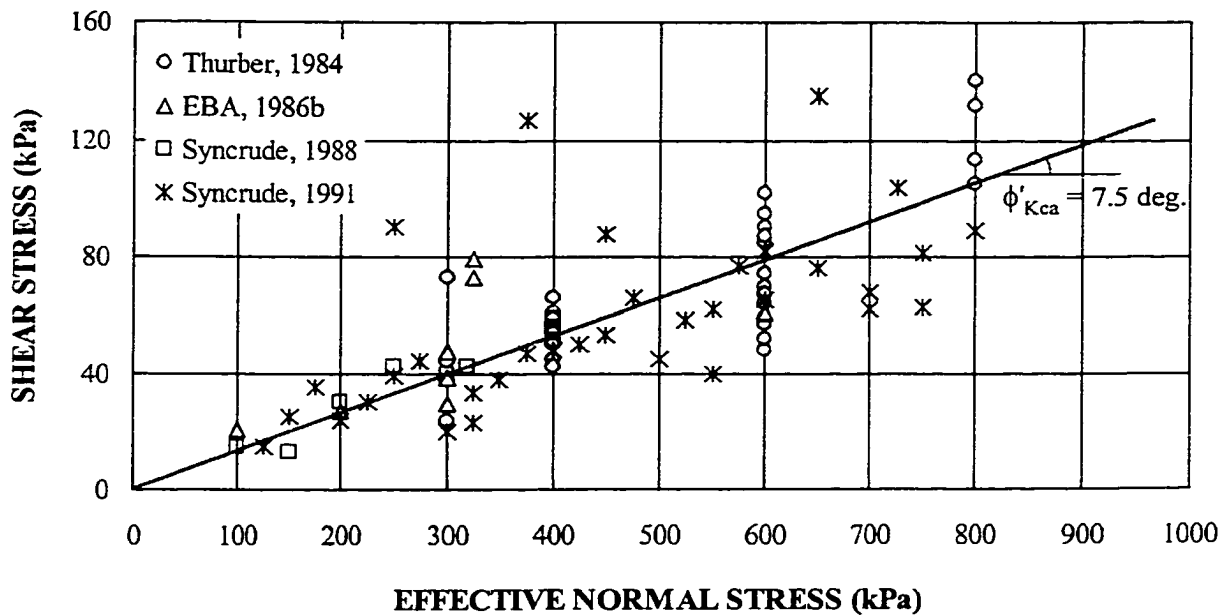
Figure 7-3 Shear box results for the residual strength of the Kca material
