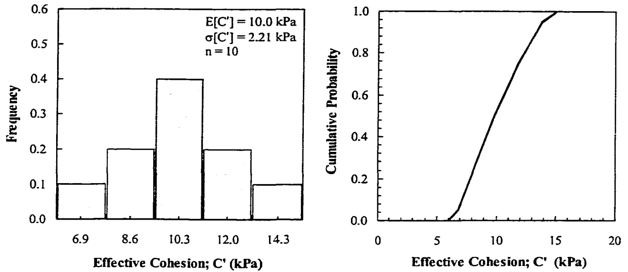
Figure 8–2 Histogram and CDF of the effective cohesion of the marine clay
