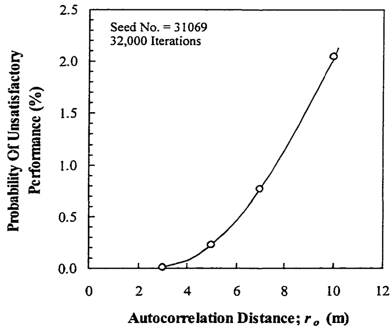
Figure 11-36 Variation of the probability of unsatisfactory performance with the autocorrelation distance, Shek Kip Mei slope (acceptable design)
