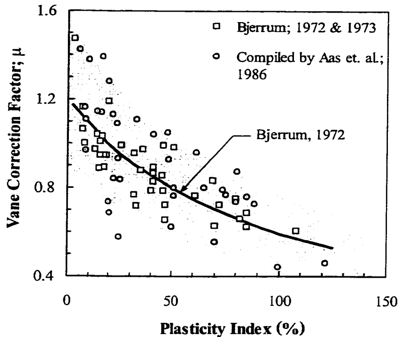
Figure 9-5 Bjerrum’s vane correction factor
