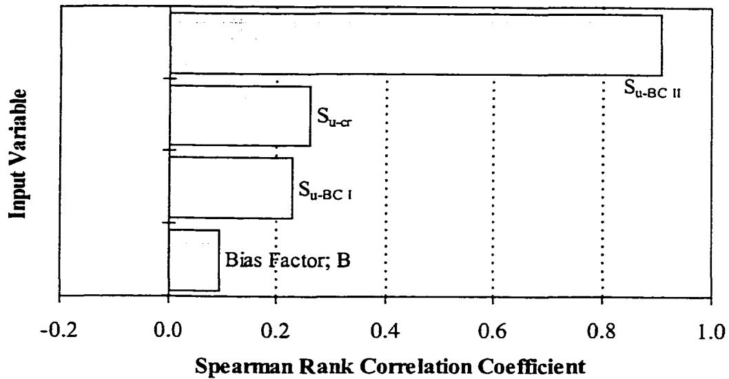
Figure 10–10 Sensitivity analysis results, Congress Street Cut (2.5:1) – Naïve analysis
