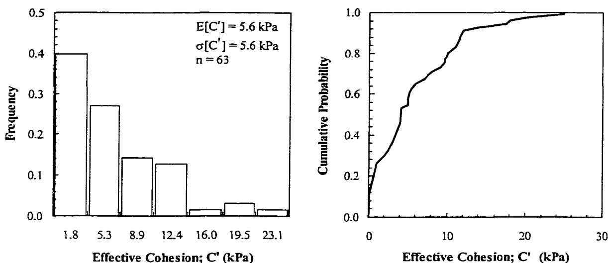
Figure 11–4 Histogram and CDF of the effective cohesion of the granitic soils of Hong Kong (HDG and CDG)
