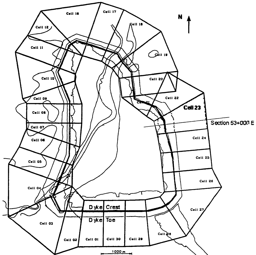
Figure 7-1 Plan of the tailings pond dyke (modified from Nicol, 1994)
