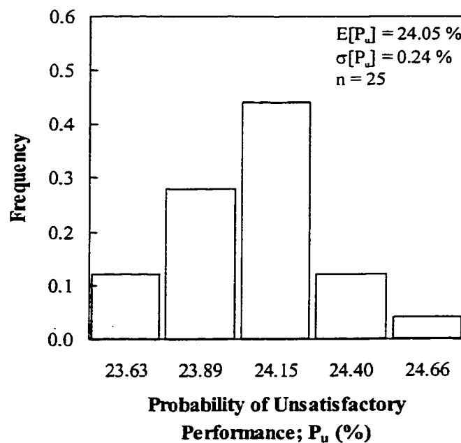
Figure 9–7 Histogram of the probability of unsatisfactory performance, Muar Embankment (H=4.7m) – Proposed Methodology
