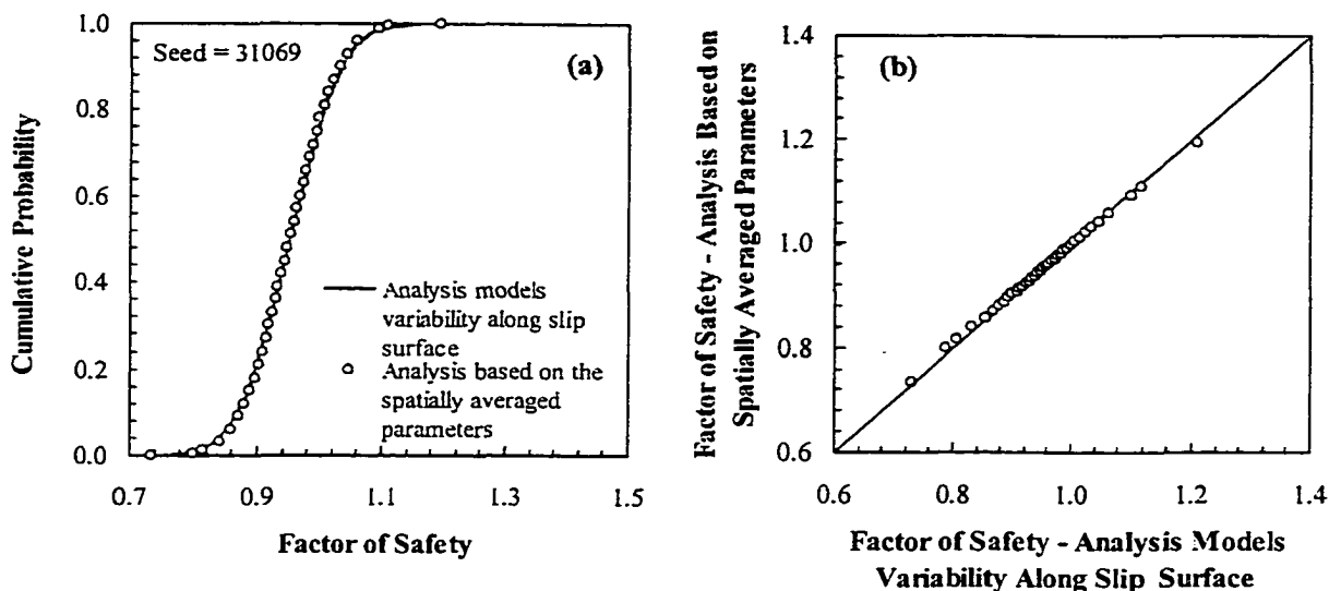
Figure 8–11 Comparison of the factor of safety from the analysis modeling variability along the slip surface that based on the spatially averaged parameters, Lodalen slide; a) Probability distribution functions, b) Q-Q plot
