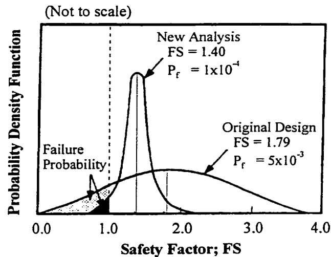
Figure 4–3 Probabilistic analysis of a pile foundation (modified from Lacasse & Nadim, 1996)
