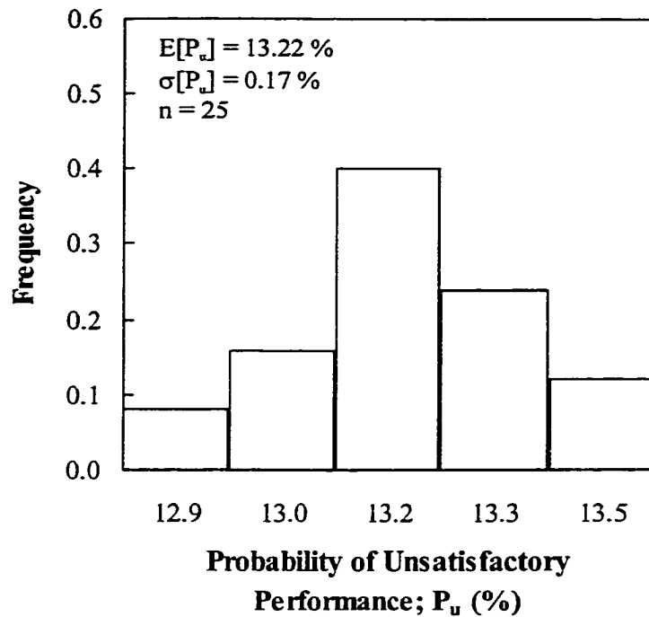
Figure 11-22 Histogram of the probability of unsatisfactory performance, Tsing Yi: 1 slope (acceptable design) – Naïve Analysis
