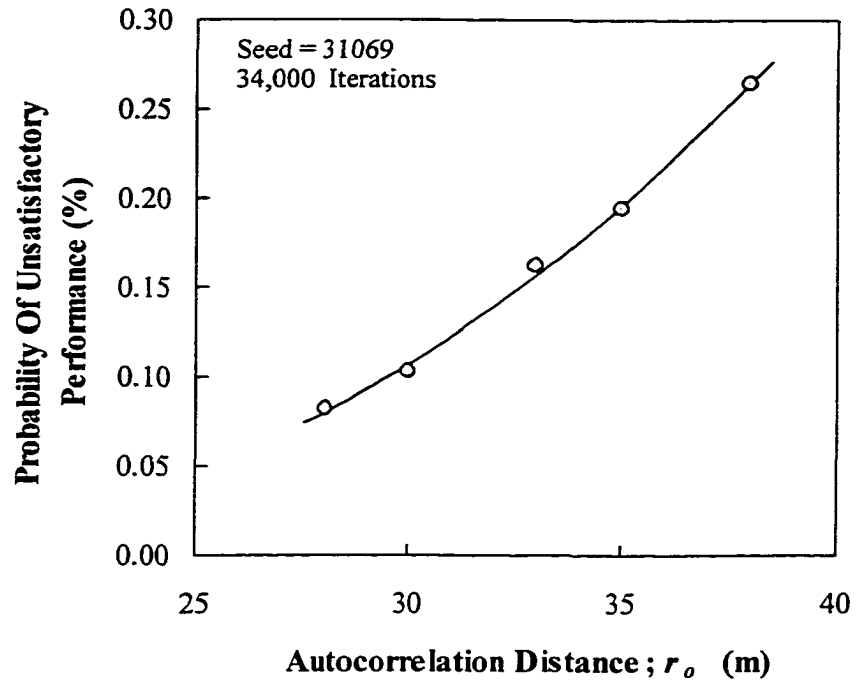
Figure 7-21 Probability of unsatisfactory performance versus autocorrelation distance
