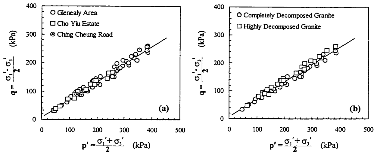
Figure 11-1 p' - q plots of triaxial tests on granitic soils; a) Based on location, b) Based on weathering grade
