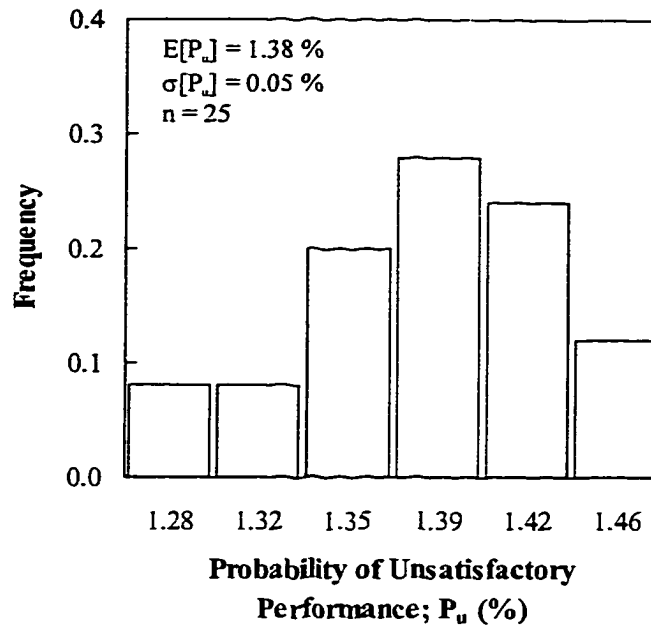
Figure 9–10 Histogram of the probability of unsatisfactory performance, Muar Embankment (H=3.3m) – Proposed Methodology
