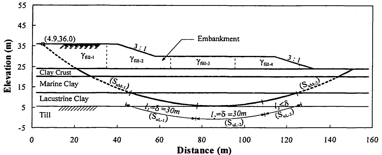
Figure 6-10 Proposed approach to account for spatial averaging, Design 1
