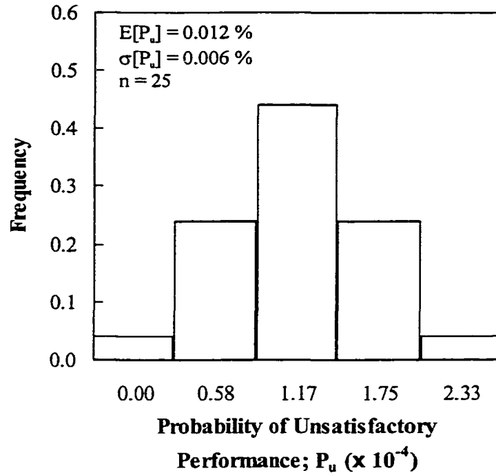
Figure 11-21 Histogram of the probability of unsatisfactory performance, Tsing Yi: 1 slope (acceptable design) – Proposed Methodology
