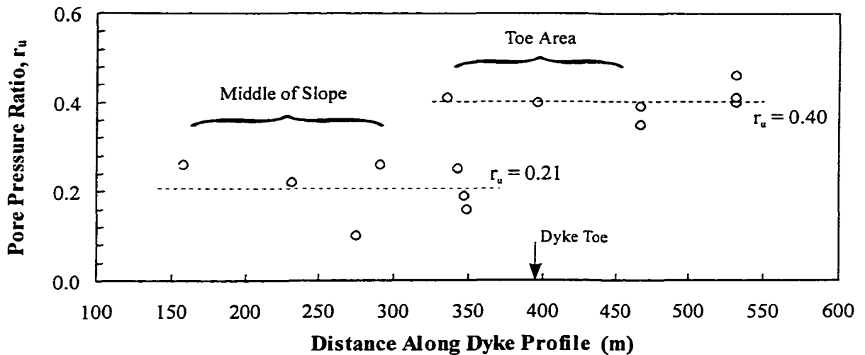
Figure 7-11 Profile of pore pressure ratio in the Pgs layer along dyke cross-section, March 1994
