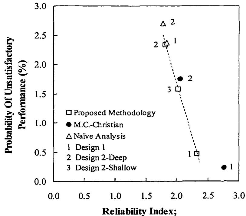
Figure 6–23 Reliability index versus probability of unsatisfactory performance – James Bay dykes
