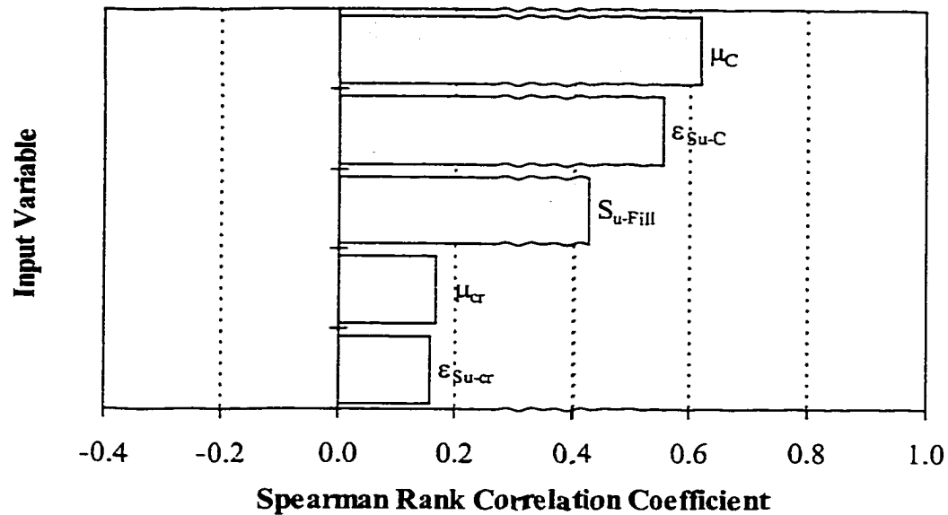
Figure 9-15 Sensitivity analysis results, Muar Embankment (H=3.3m) – Naïve Analysis
