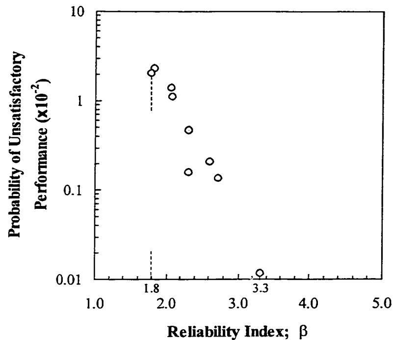
Figure 12-7 Probability of unsatisfactory performance versus reliability index; Safe Slope – Proposed Methodology
