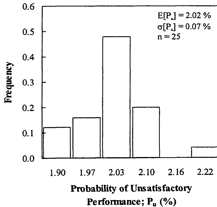
Figure 10-6 Histogram of the probability of unsatisfactory performance, Congress Street Cut (2.5:1) – Proposed Methodology
