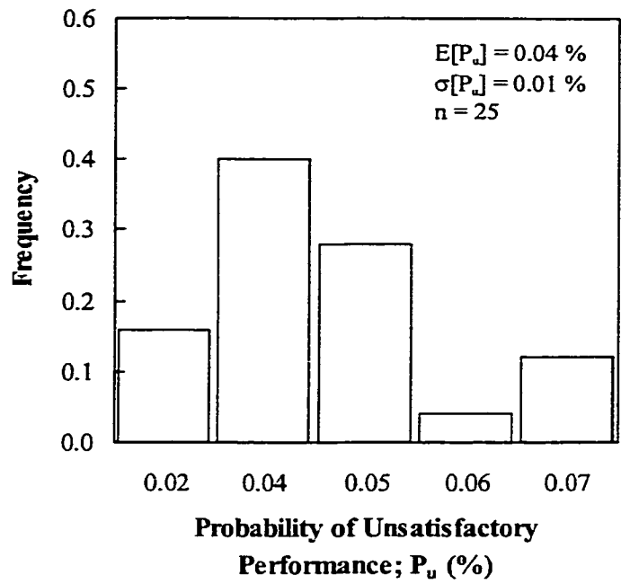
Figure 8-15 Histogram of the probability of unsatisfactory performance, Lodalen slope (4h:1v) – Naïve analysis
