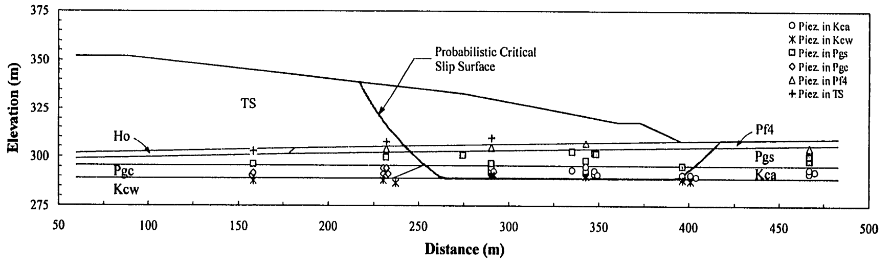
Figure 7-7 Locations of piezometer tips, Section 53+000E – Cell23
