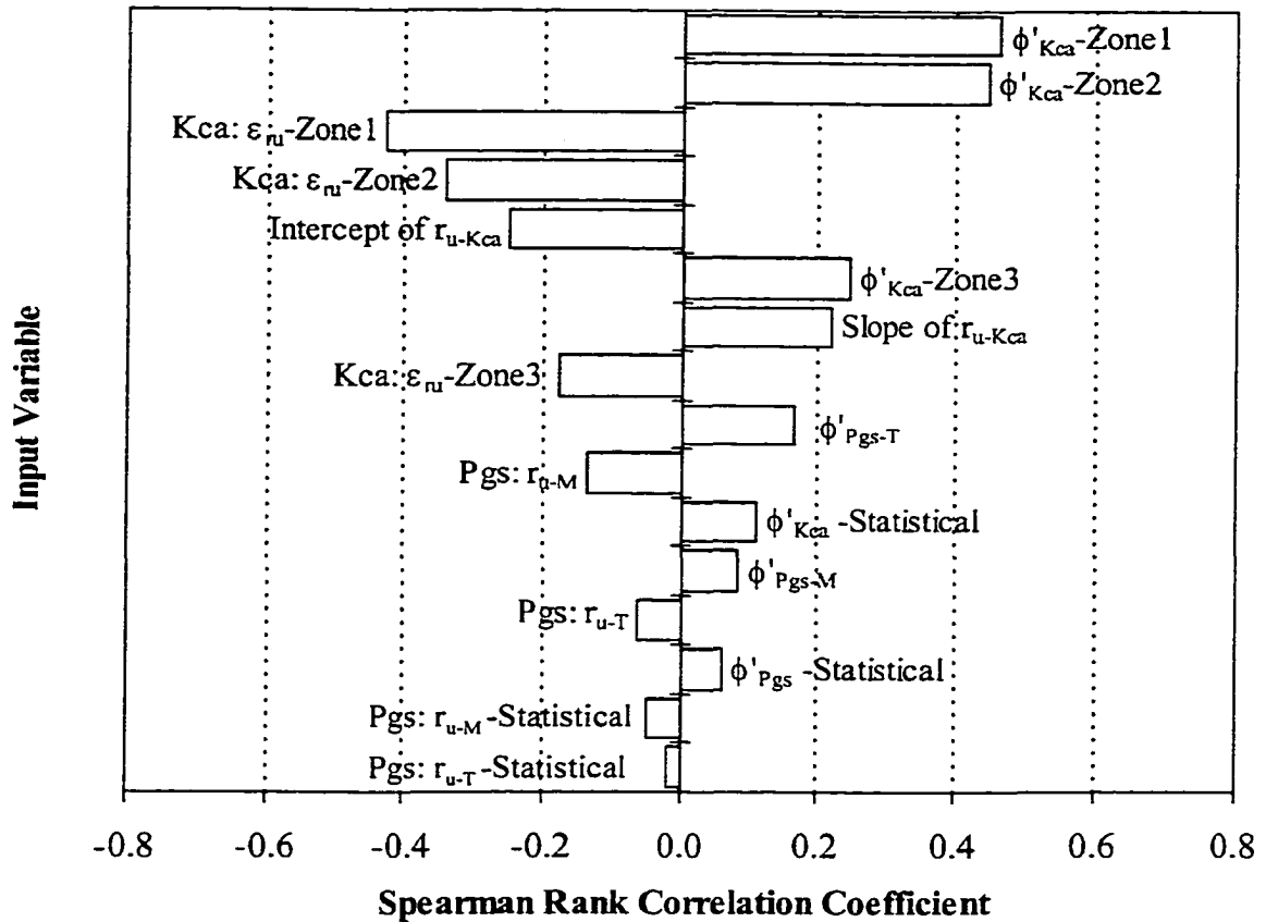
Figure 7–16 Sensitivity analysis results, Cell 23 – Proposed Methodology
