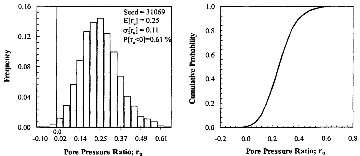
Figure 11–8 Histogram and CDF of the pore pressure ratio at failure – Cho Yiu landslide
