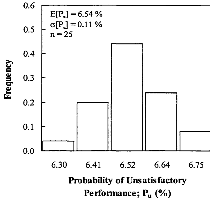
Figure 11–14 Histogram of the probability of unsatisfactory performance, Cho Yiu slope (acceptable design) – Naïve Analysis
