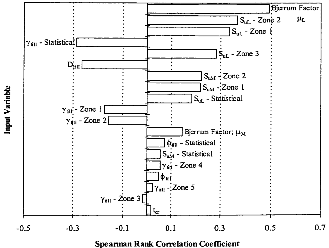
Figure 6-15 Sensitivity analysis results – Proposed Methodology; Design 1
