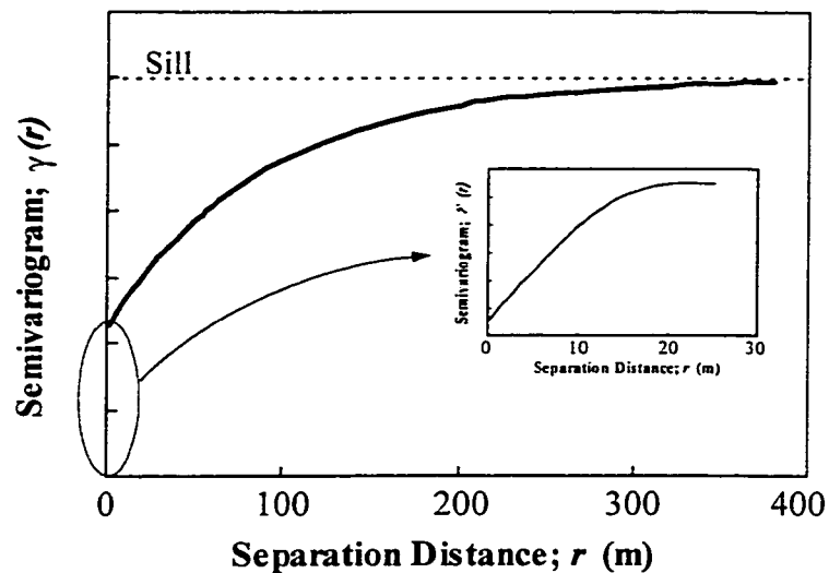
Figure 3–13 Effect of scale of observations on observed variability
