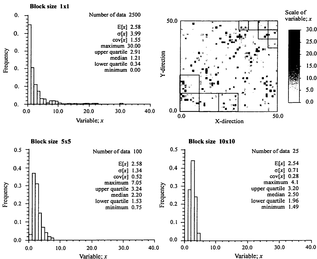
Figure 3–11 Variance reduction due to spatial averaging over blocks of sizes 1x1, 5x5 and 10x10
