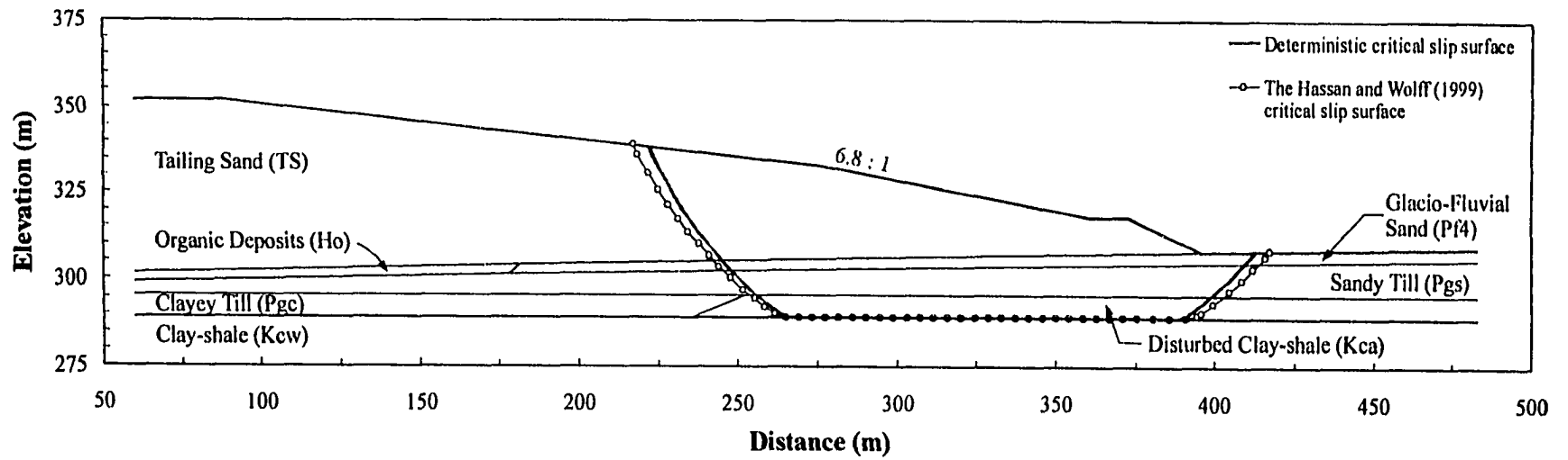
Figure 7-2 Geometry and soil stratigraphy at Section 53+000E - Cell 23
