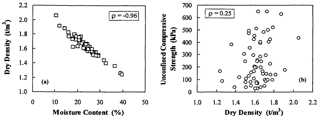
Figure 3–14 Scatter plot for detecting correlation between soil properties (data from Holtz and Krizek, 1972); a) Strong negative correlation, b) Weak positive correlation
