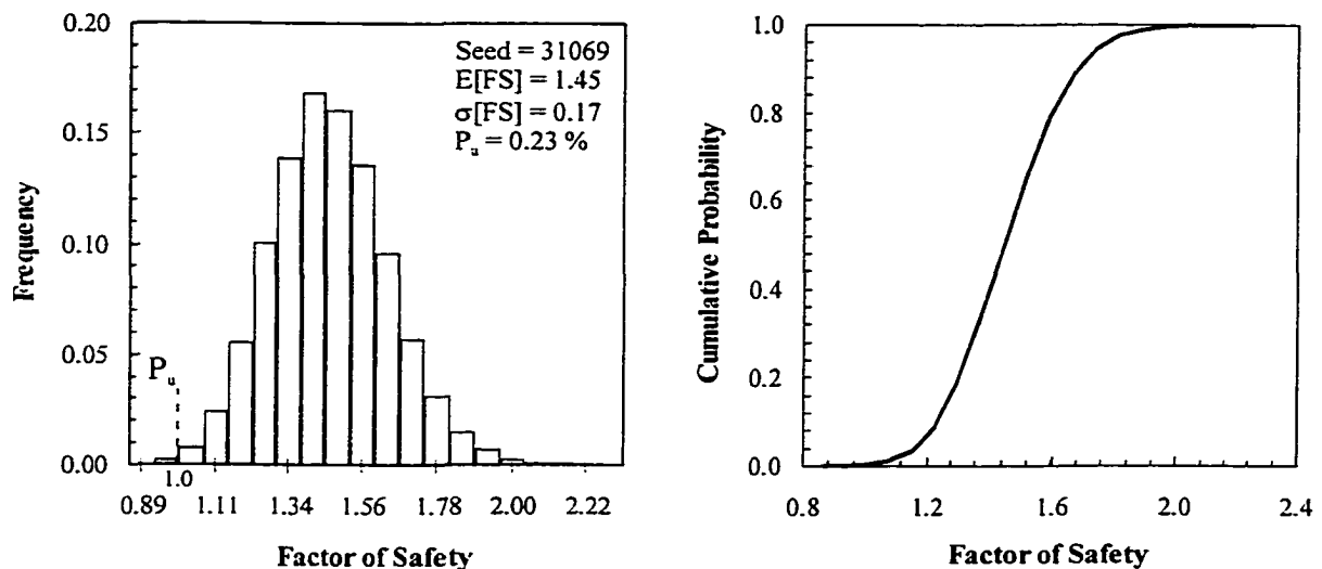
Figure 11–34 Histogram and CDF of the factor of safety, Shek Kip Mei slope (acceptable design) – Proposed Methodology
