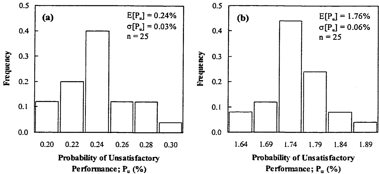
Figure 6-7 Histogram of the probability of unsatisfactory performance: a) Design 1; b) Design 2
