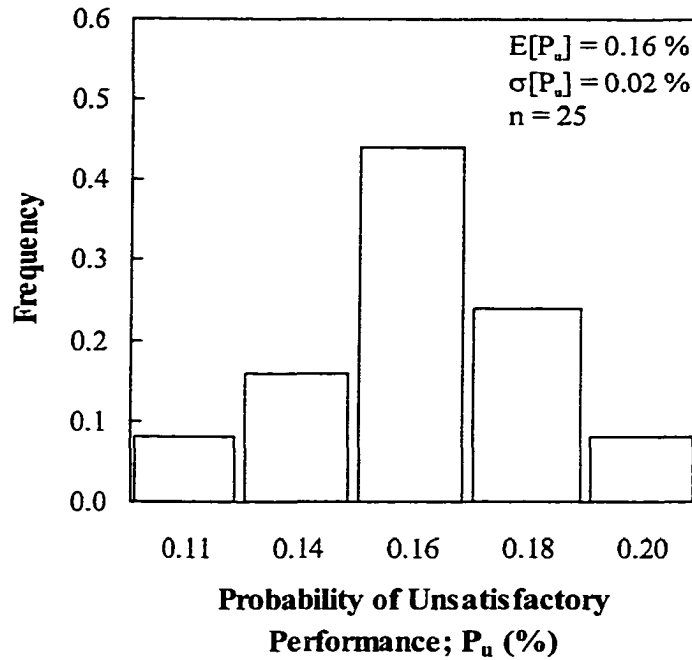
Figure 7–17 Histogram of the probability of unsatisfactory performance – Cell 23
