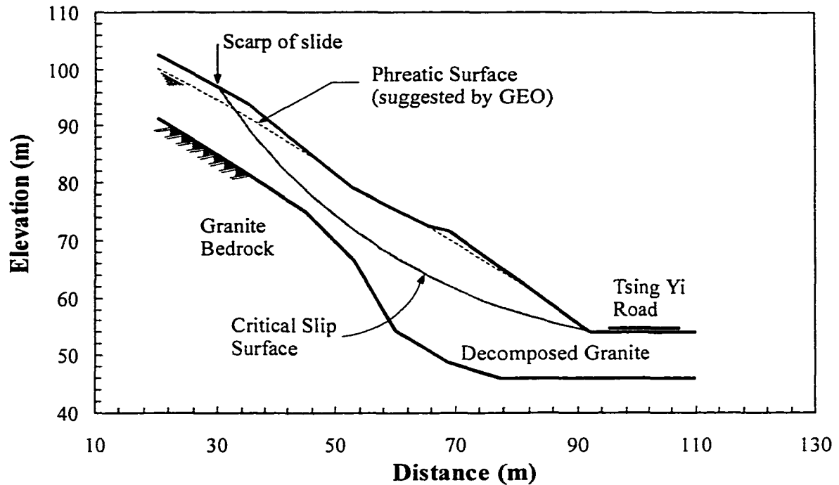
Figure 11-15 Cross-section and stratigraphy of Tsing Yi: 1 slide
