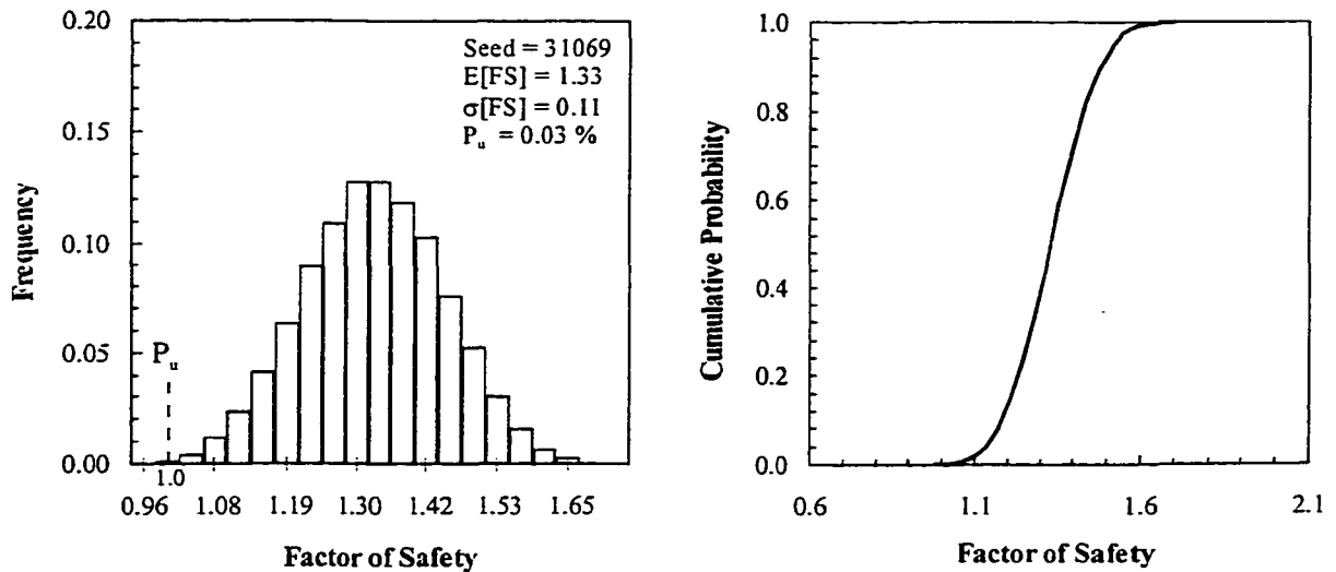
Figure 8–14 Histogram and CDF of the factor of safety; Lodalen slope (4h:1v) – Naïve analysis
