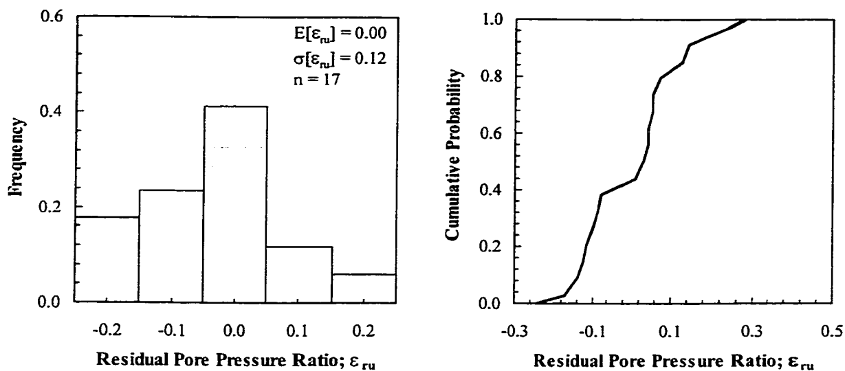
Figure 7-9 Histogram and CDF of the residual pore pressure ratio of the Kca unit
