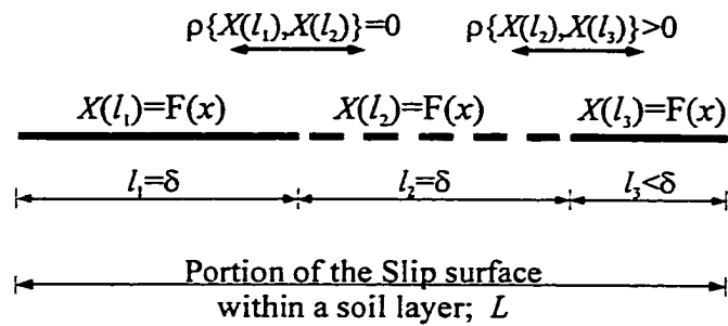
Figure 5–6 Modeling variability of an input parameter along the failure surface
