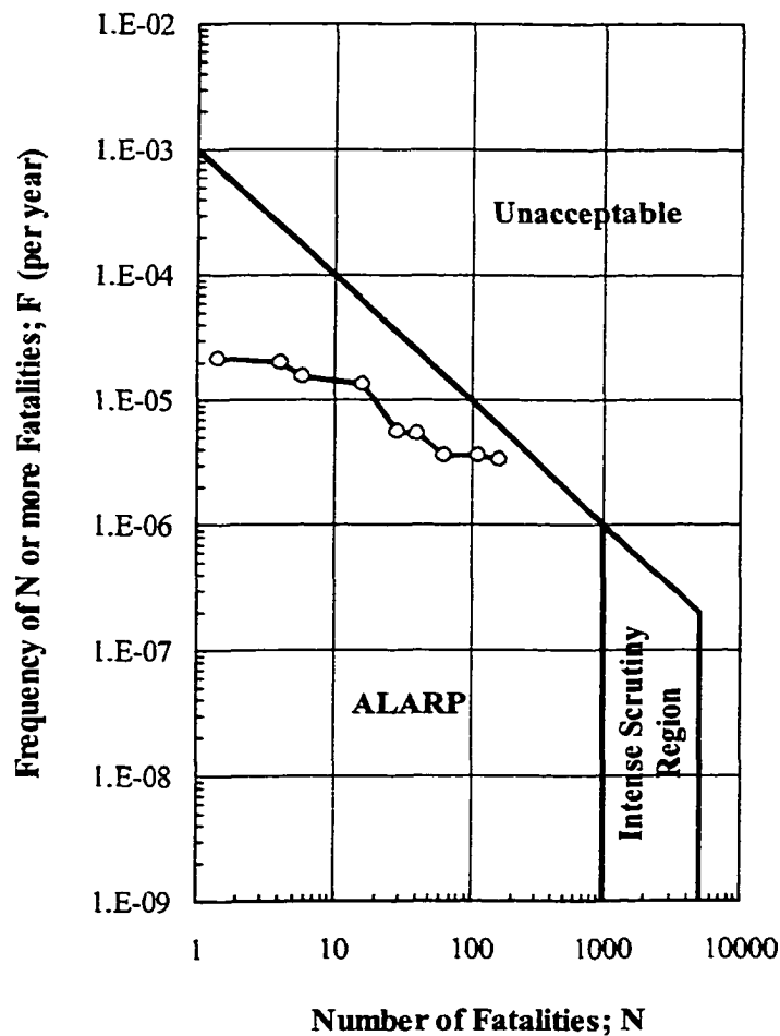
Figure 13-3 Calculated F-N curve for sliding failure of Shek Kip Mei slope and the ERM (1999) risk acceptance criteria
