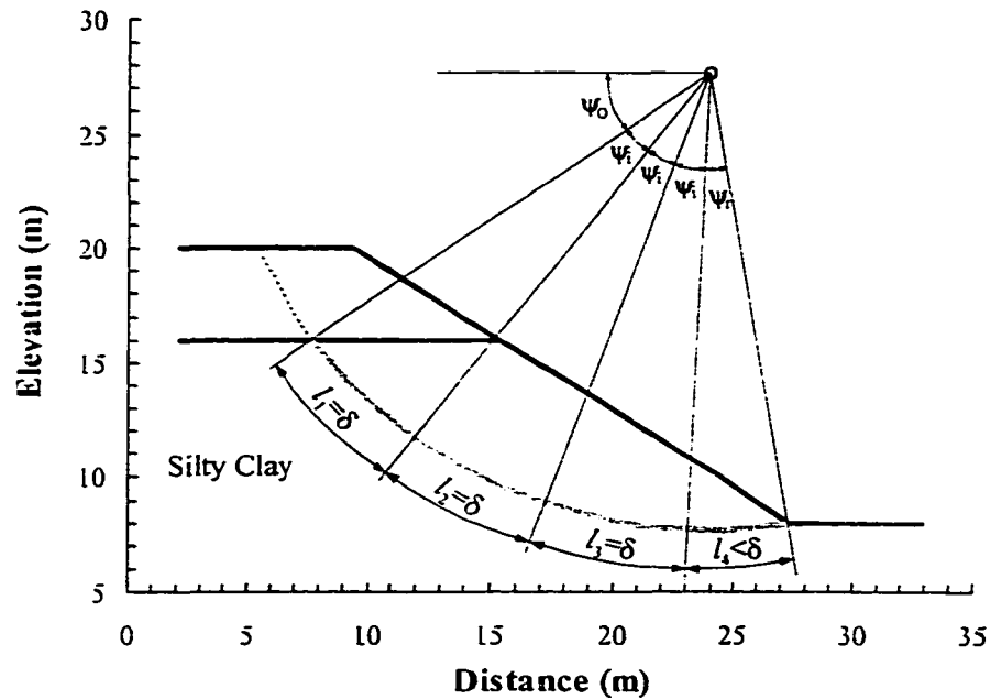
Figure 5-9 Accounting for spatial variability in the spreadsheet model
