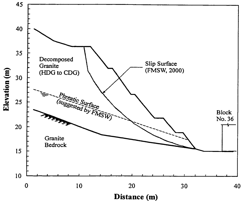
Figure 11-31 Geometry and stratigraphy of Shek Kip Mei Estate landslide, Northern Slope
