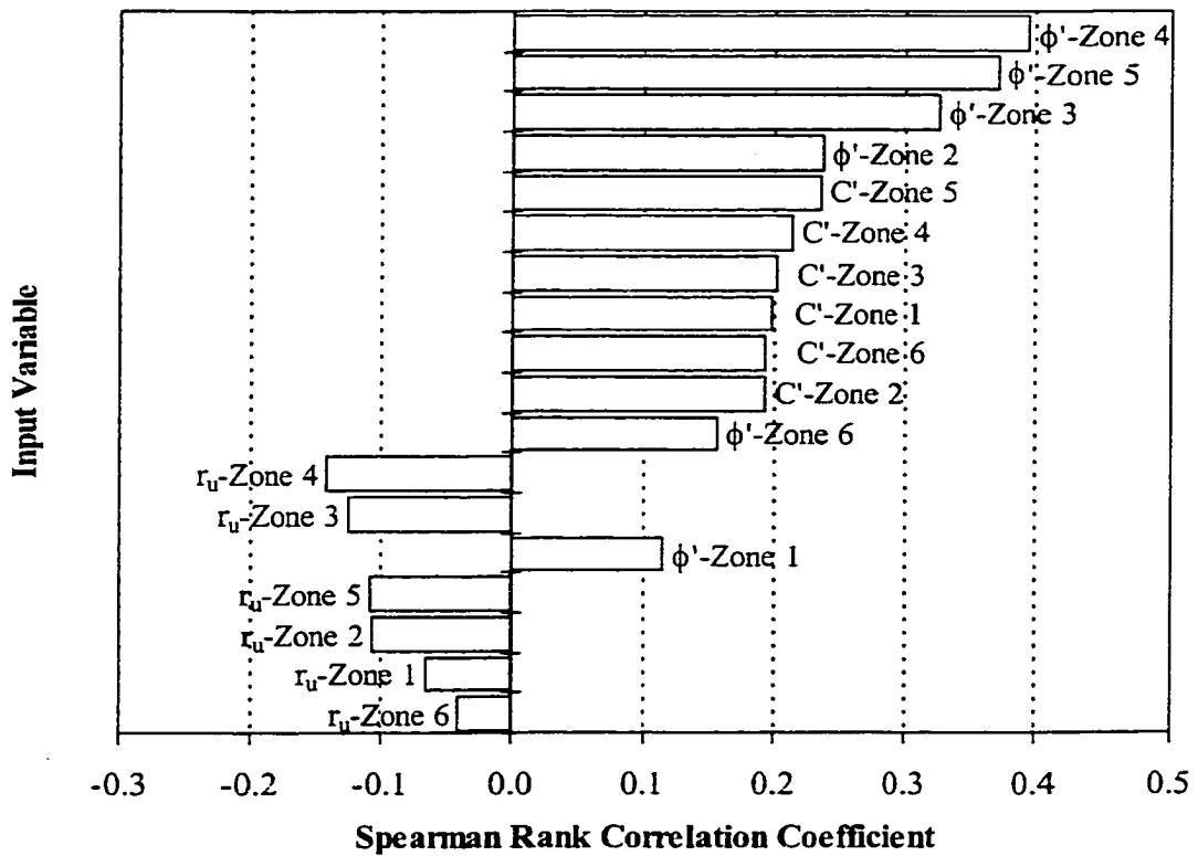
Figure 11–27 Sensitivity analysis results, Ching Cheung Road (acceptable slope) – Proposed Methodology
