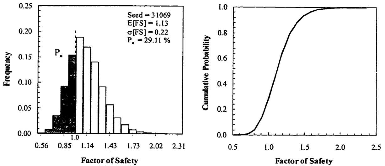
Figure 10-2 Histogram and CDF of the factor of safety, Congress Street Cut (1.35:1) – Proposed Methodology
