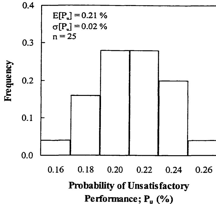
Figure 11-37 Histogram of the probability of unsatisfactory performance, Shek Kip Mei slope (acceptable design) – Proposed Methodology
