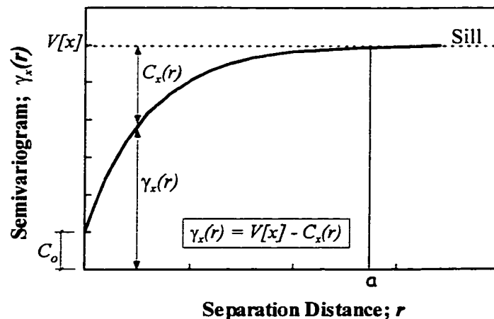
Figure 3–9 Elements of semivariogram function for a stationary condition
