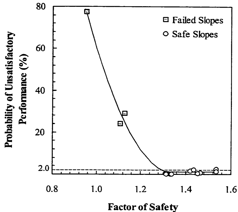
Figure 12-5 Probability of Unsatisfactory performance versus factor of safety for the safe and failed slopes – Proposed Methodology
