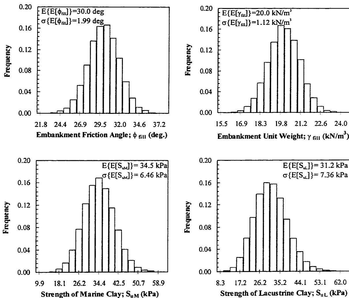
Figure 6–14 Histograms of the average soil parameters – Proposed Methodology; Design 1
