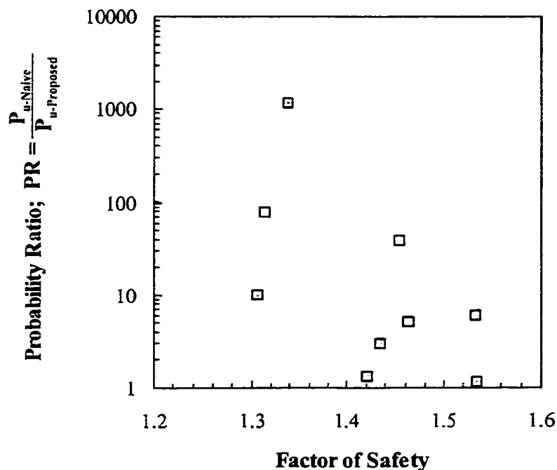
Figure 12–1 Probability ratio versus factor of safety for safe slopes
