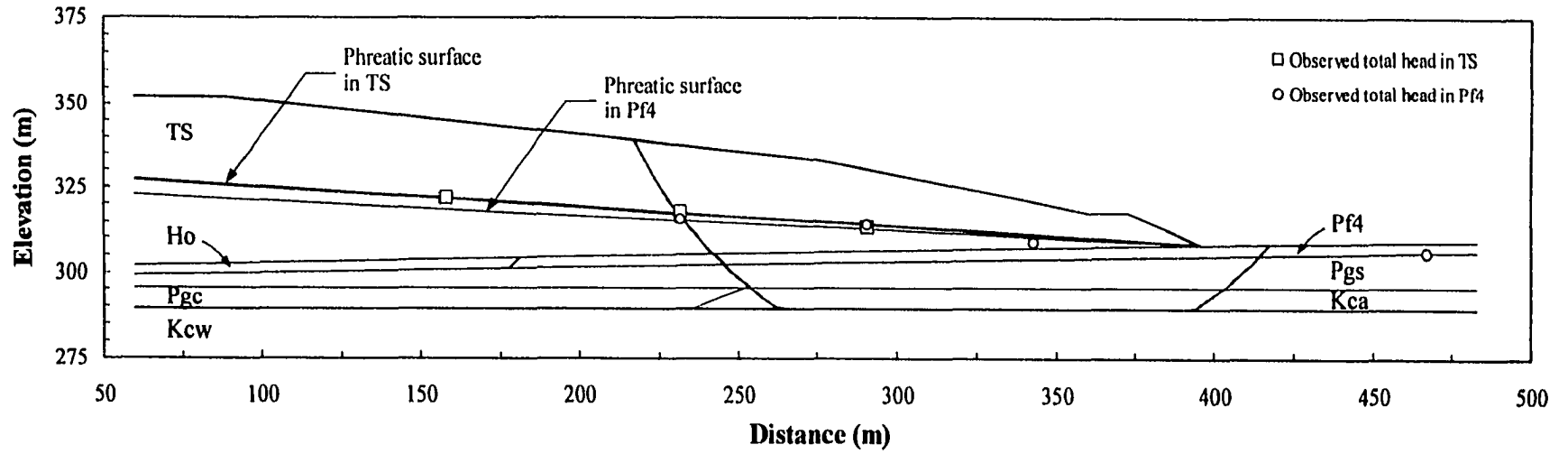
Figure 7-13 Phreatic surfaces in the tailing sand and the glacio-fluvial sand, March 1994
