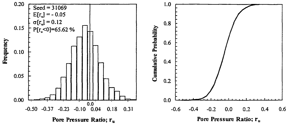
Figure 11-24 Histogram and CDF of pore pressure ratio at failure – Ching Cheung Road landslide
