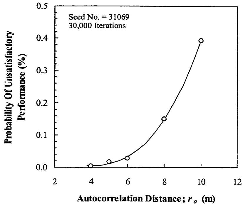
Figure 11–20 Variation of the probability of unsatisfactory performance with the autocorrelation distance, Tsing Yi: 1 slope (acceptable design)
