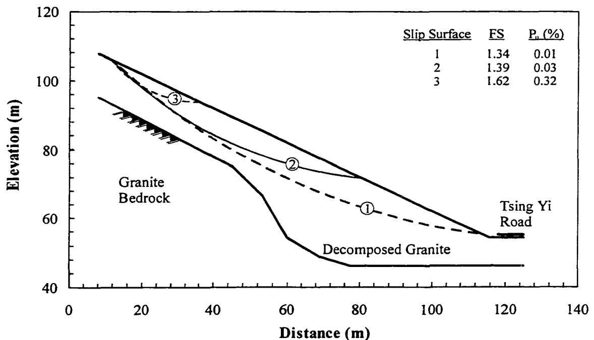
Figure 11-39 Effect of scale of failure on probability of unsatisfactory performance and factor of safety - Tsing Yi: 1 slope (acceptable design)
