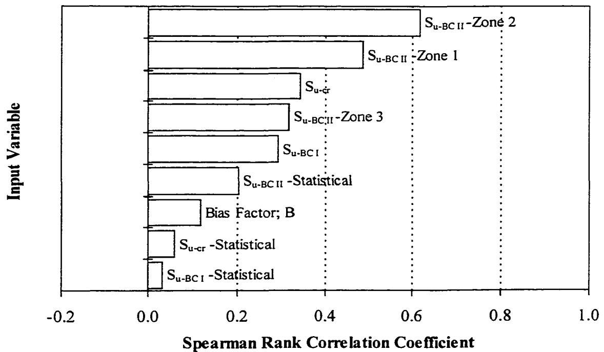
Figure 10–7 Sensitivity analysis results, Congress Street Cut (2.5:1) – Proposed Methodology
