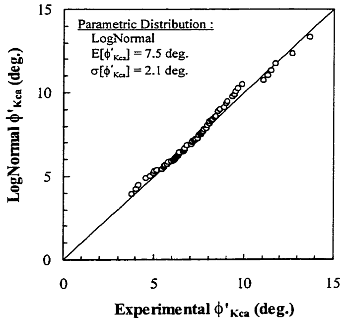
Figure 7-5 Q-Q plot of the experimental residual friction angle of the Kca unit and a parametric LogNormal distribution
