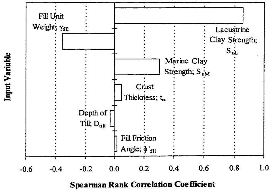
Figure 6-9 Sensitivity analysis results, Design 2
