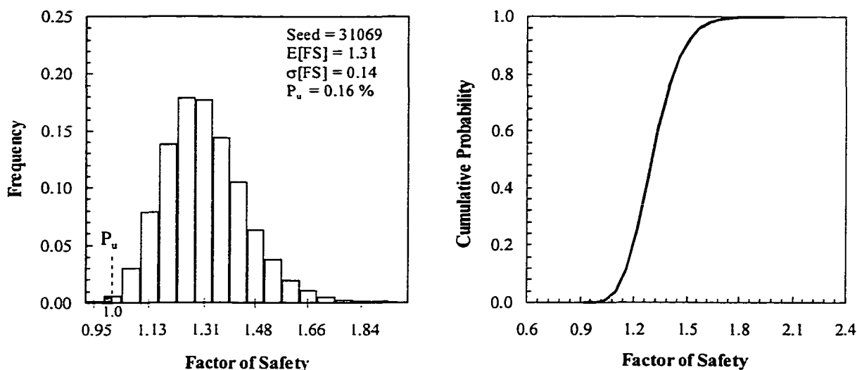
Figure 7–15 Histogram and CDF of the factor of safety, Cell 23 – Proposed methodology
