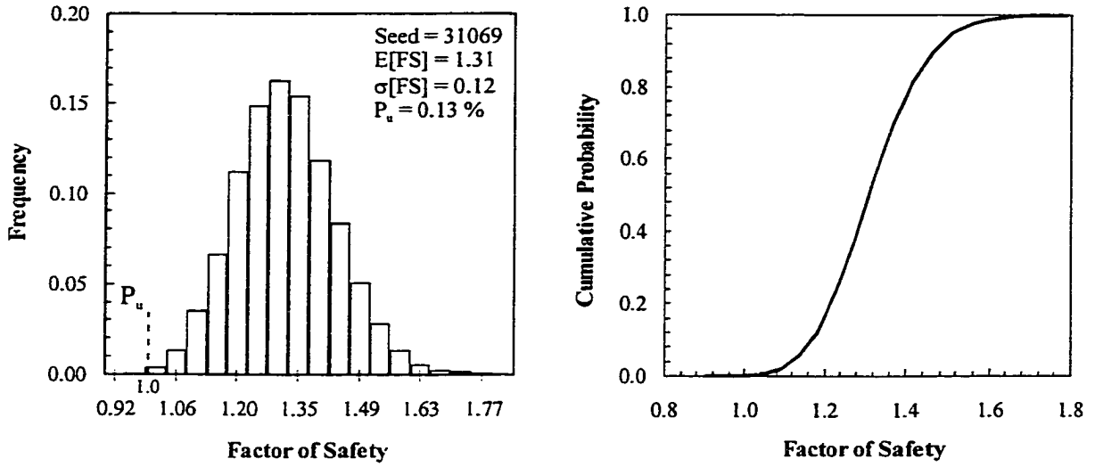
Figure 11–26 Histogram and CDF of the factor of safety, Ching Cheung Road (acceptable slope) – Proposed Methodology
