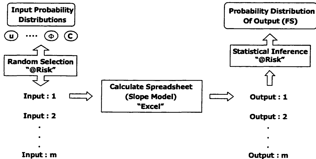
Figure 5–1 Monte Carlo simulation procedure using "Excel" and "@Risk" software
