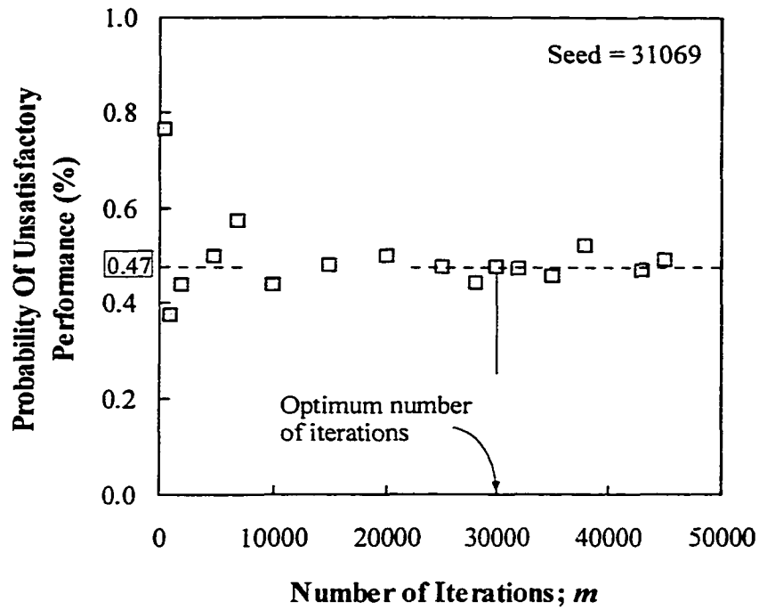
Figure 6-11 Optimum number of iterations - Proposed Methodology; Design 1
