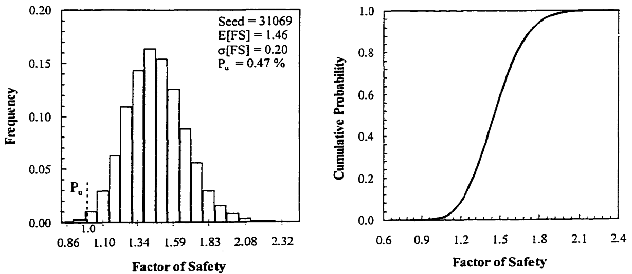
Figure 6-12 Histogram and CDF of the factor of safety –Proposed Methodology; Design 1
