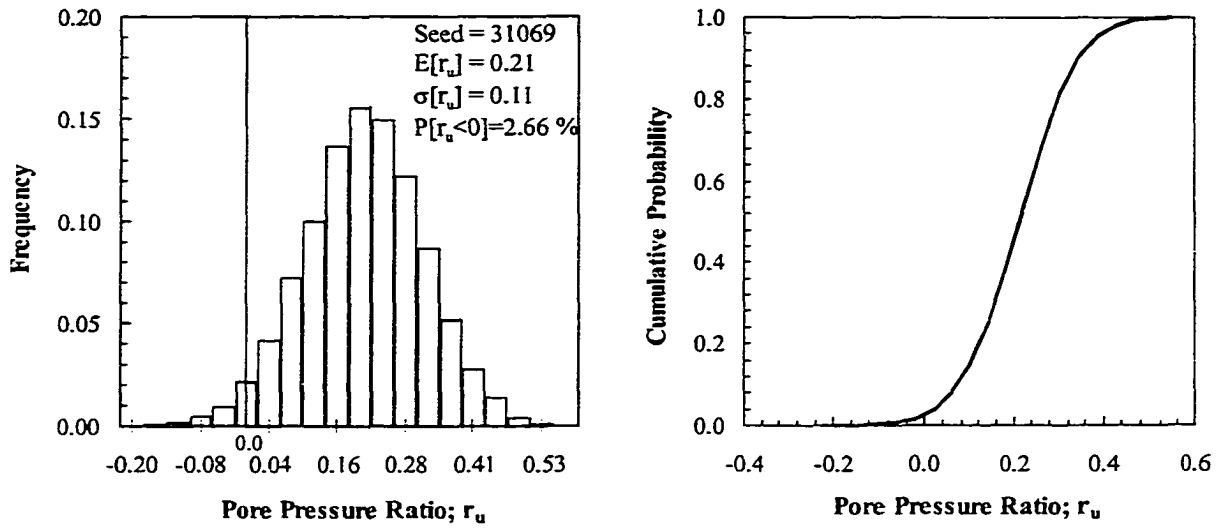
Figure 11-16 Histogram and CDF of the pore pressure ratio at failure – Tsing Yi: 1 landslide
