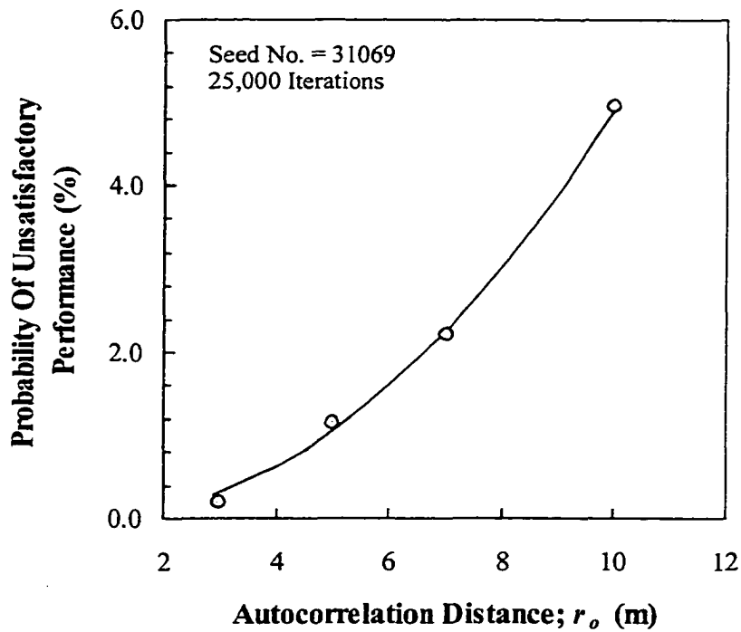
Figure 11-12 Variation of the probability of unsatisfactory performance with the autocorrelation distance, Cho Yiu slope (acceptable design)
