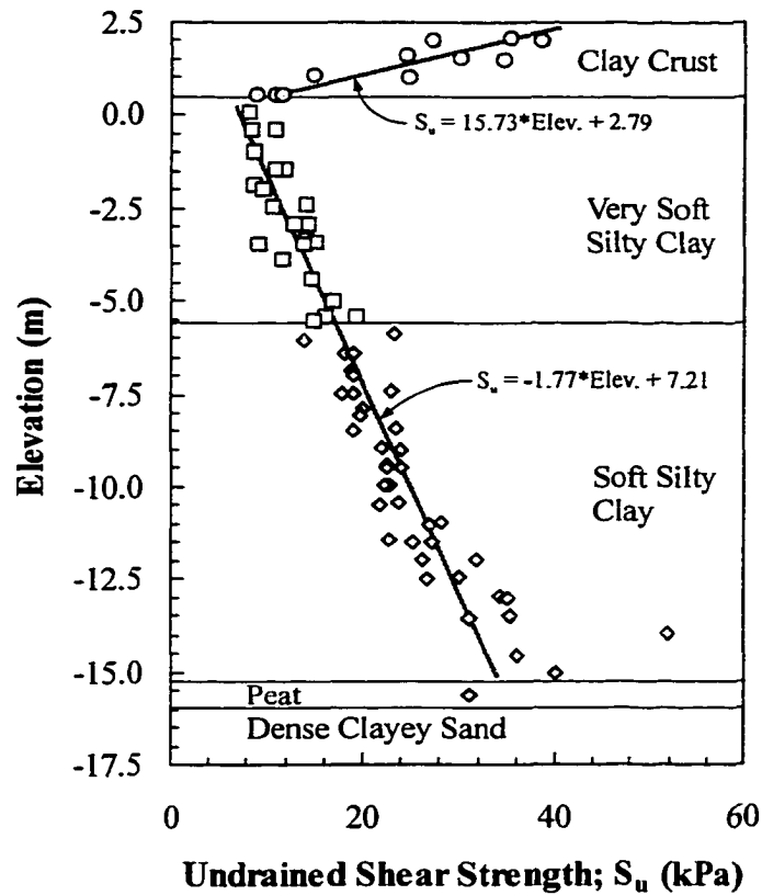
Figure 9–2 Profile of field vane shear strength
