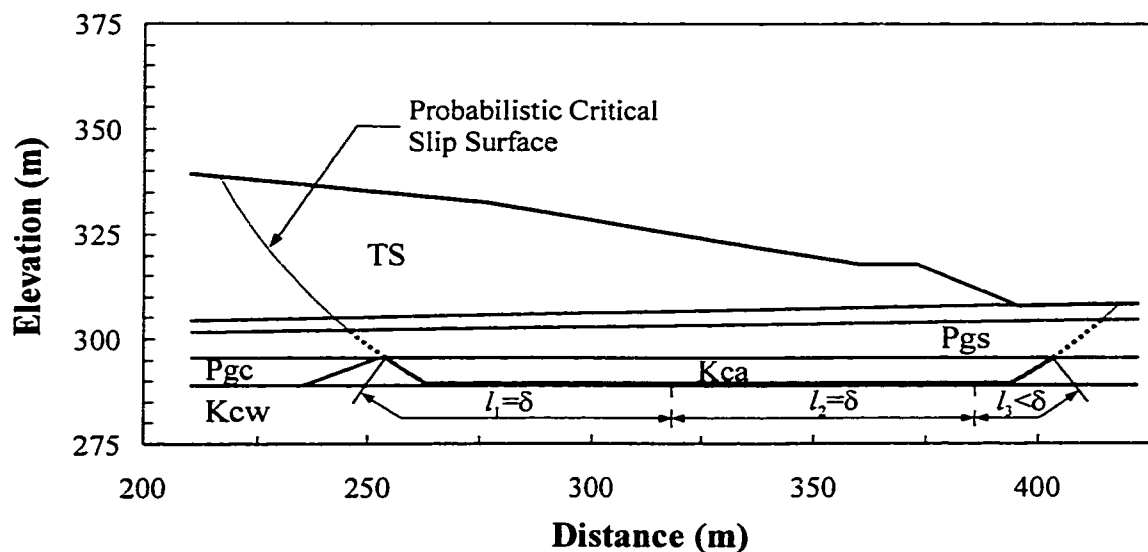
Figure 7-14 Accounting for spatial variability along the slip surface by the variability of local averages over segments of the surface
