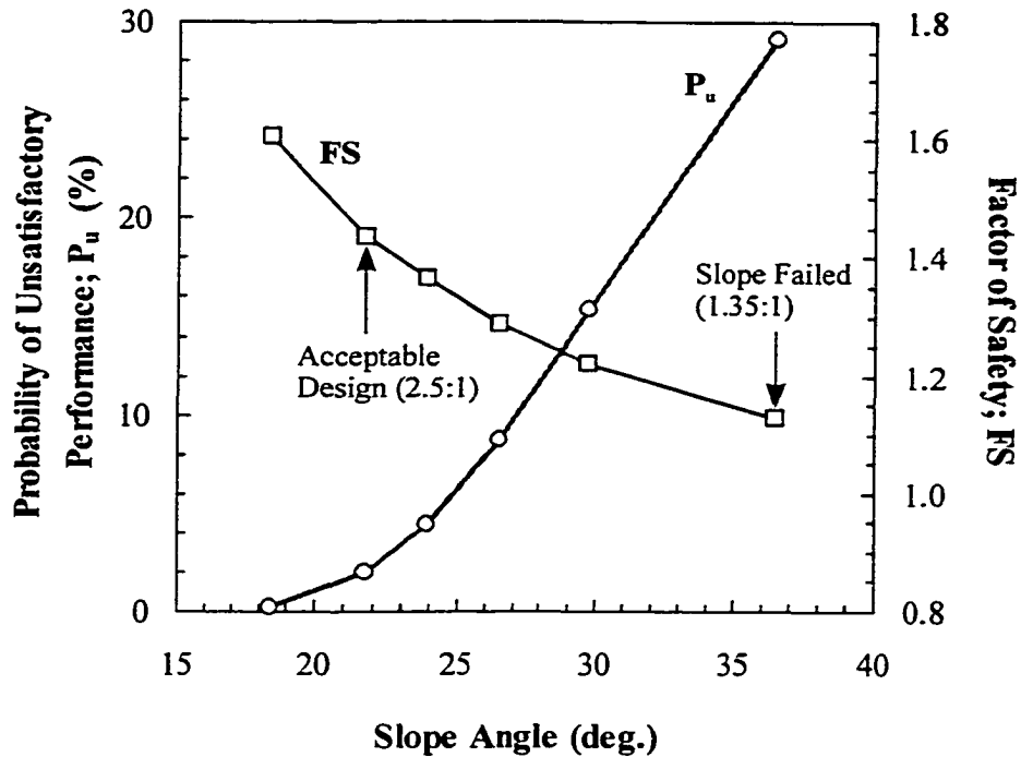
Figure 10-4 Variation of the probability of unsatisfactory performance and the factor of safety with the slope angle, Congress Street Cut – Proposed Methodology
