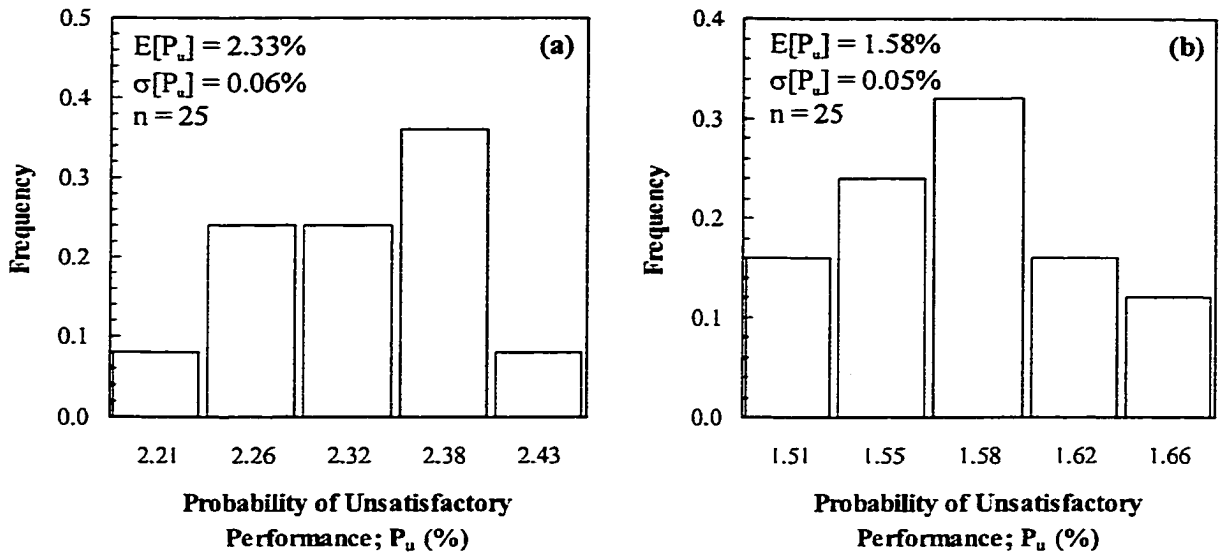
Figure 6–18 Histograms of the probability of unsatisfactory performance, Design 2 – Proposed Methodology; a) Deep failure; b) Shallow failure
