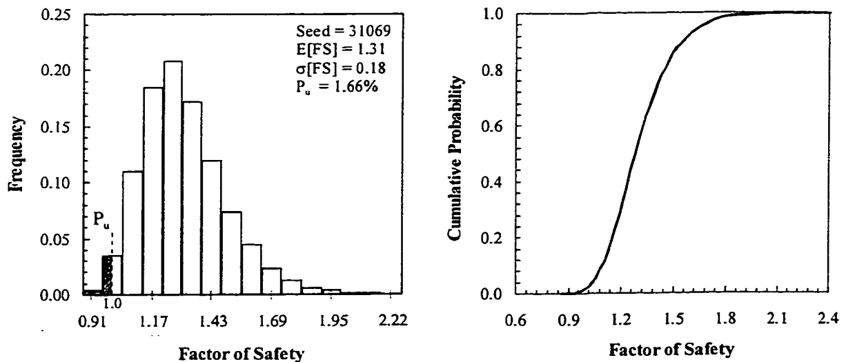
Figure 7-22 Histogram and CDF of the factor of safety, Cell 23 – Naïve analysis
