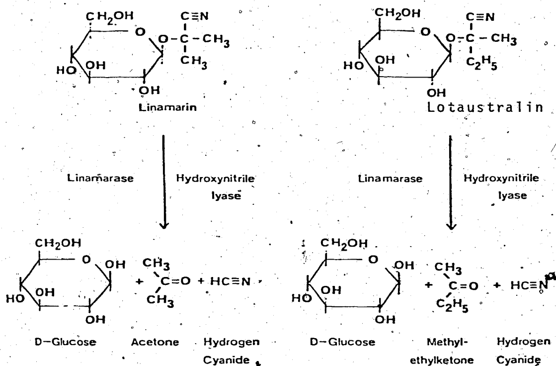
Fig. 1. The structures and hydrolytic products of the cyanogenic glucosides of cassava, linamarin and lotaustralin.
