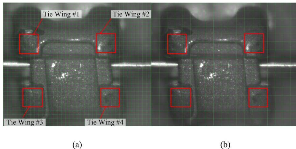
Fig 10: Bracket images showing image subsets (a) 64 \times 64 pixel subsets (b) 128 \times 128 pixel subsets.
