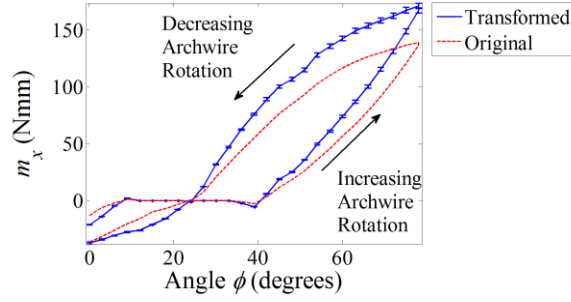
Fig 8: Load cell transformation showing transformed and measured m_x as well as effect of increasing and decreasing archwire rotation. Error bars are shown to demonstrate the uncertainty in the m_{xbracket} measurement.
