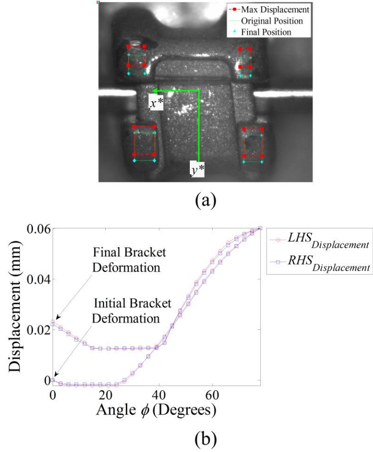
Fig 12: Tracking of bracket tie wings. (a) Bracket in original position shown by solid lines, square boxes showing maximum tie wing displacement and diamonds showing final tie wing position after applied torque has been removed. (b) Plot of bracket tie wing deformation measured using digital image correlation showing initial and final deformation of the left hand and right hand side of the bracket tie wings.
