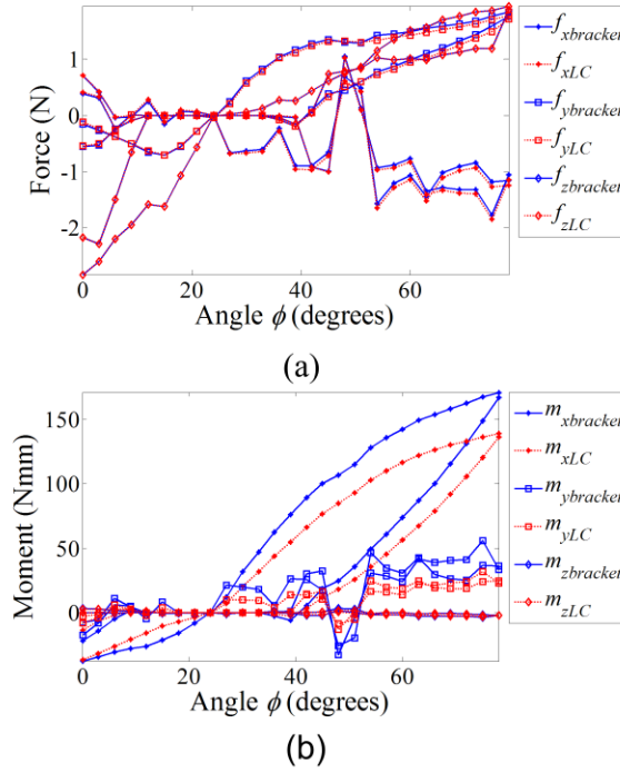
Fig 7: Load cell transformation showing transformed and measured forces and moments . (a) transformed and measured force ( f_x, f_y, f_z ). (b) transformed and measured moments ( m_x, m_y, m_z ).
