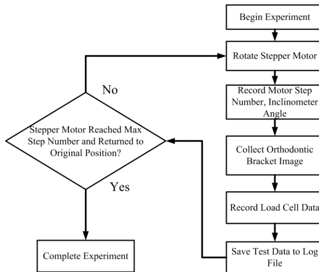
Fig 4: Flowchart of Orthodontic Torque Simulator operation.
