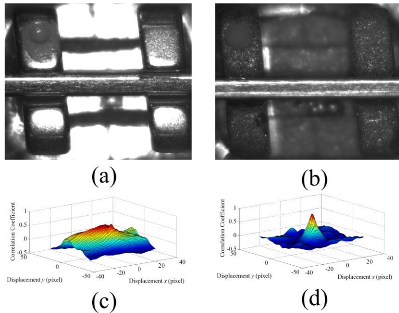
Fig 11: Preparation of orthodontic brackets (a) Bracket without micro-etching (b) Bracket with micro-etching. (c) Correlation peak for bracket without micro- etching (d) Correlation peak for bracket with micro- etching.
