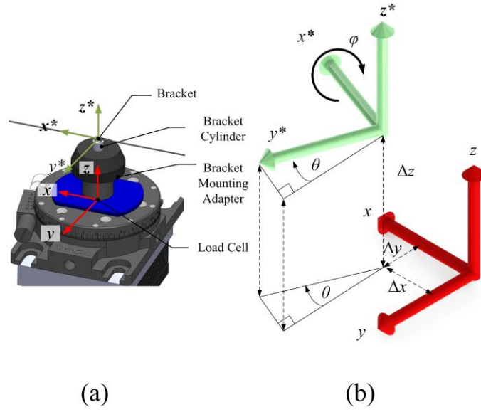
Fig 3: Load cell and bracket coordinate systems. (a) Offset of orthodontic bracket from load cell (b) Coordinate system transformation showing displacement, rotation about the z axis and the angle \phi indicating the direction of archwire rotation.
