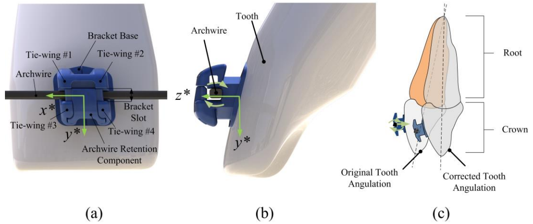
Fig 1: Self-ligating orthodontic bracket components (a) Top view of bracket showing tie wings, archwire and bracket base (b) Side view of bracket showing the angle of the bracket slot (prescription). Archwire rotation occurs about the x^* axis of the bracket coordinate system. (c) Control of tooth angulations using archwire rotation.
