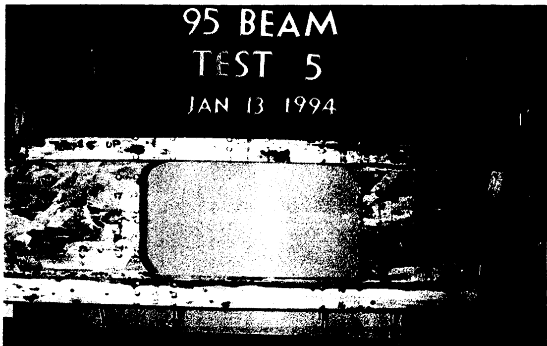
Figure 5.31. Web/flange connection failure in specimen 9.5dT5
