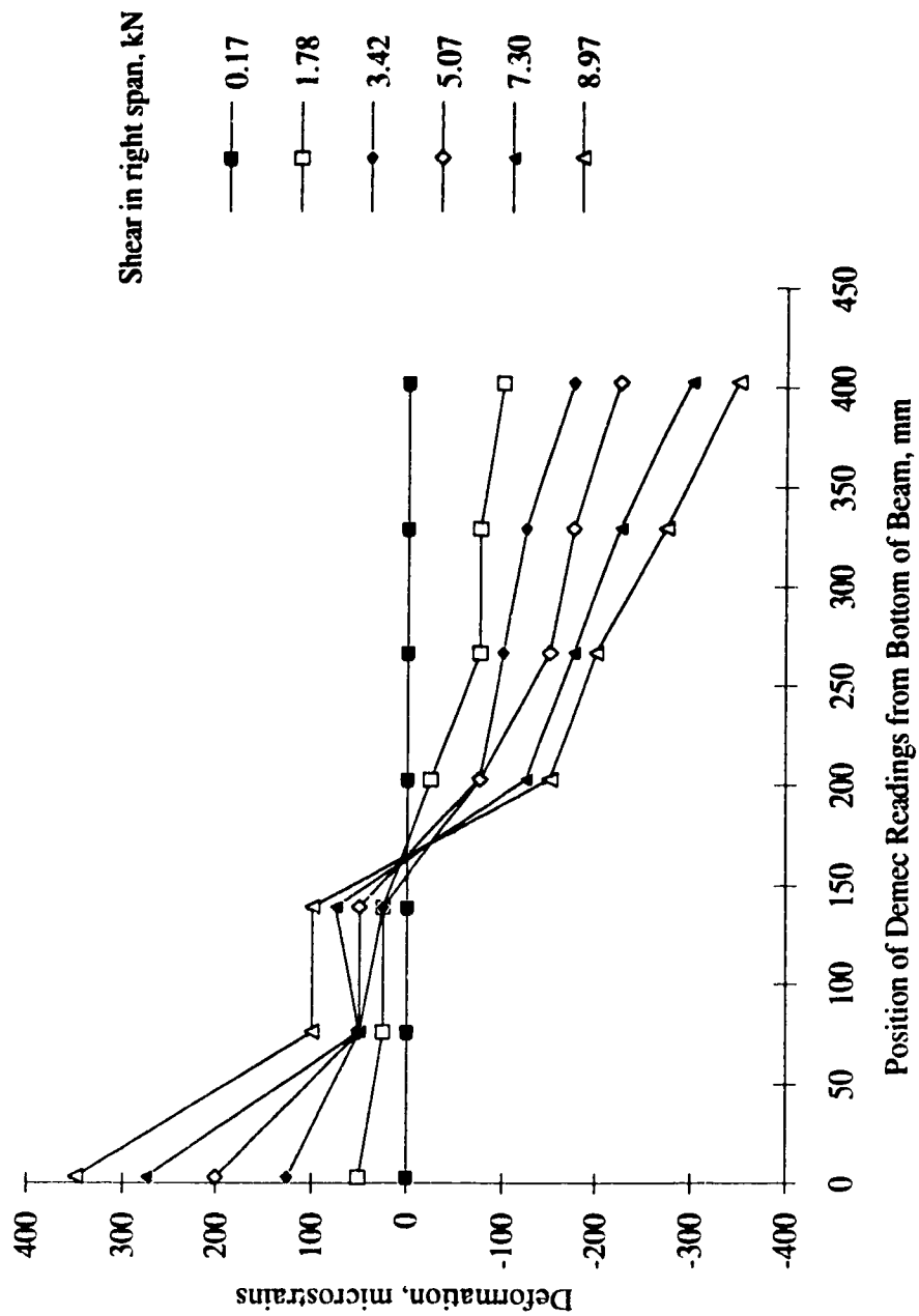
Figure 5.24. Longitudinal strain distribution of specimen 16dTT1 at 520 mm from right reaction
