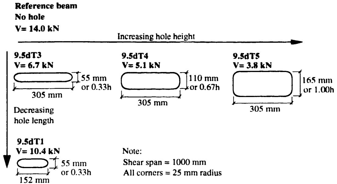
Figure 5.7. Effect of hole size in 241 mm beams
