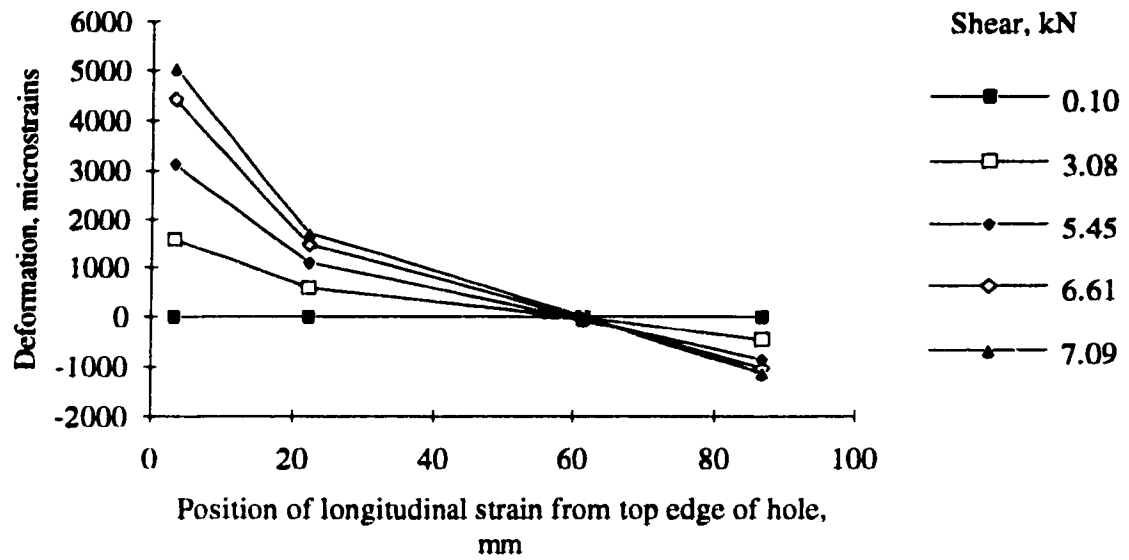
16dT2, Longitudinal demec readings at bottom right of hole
