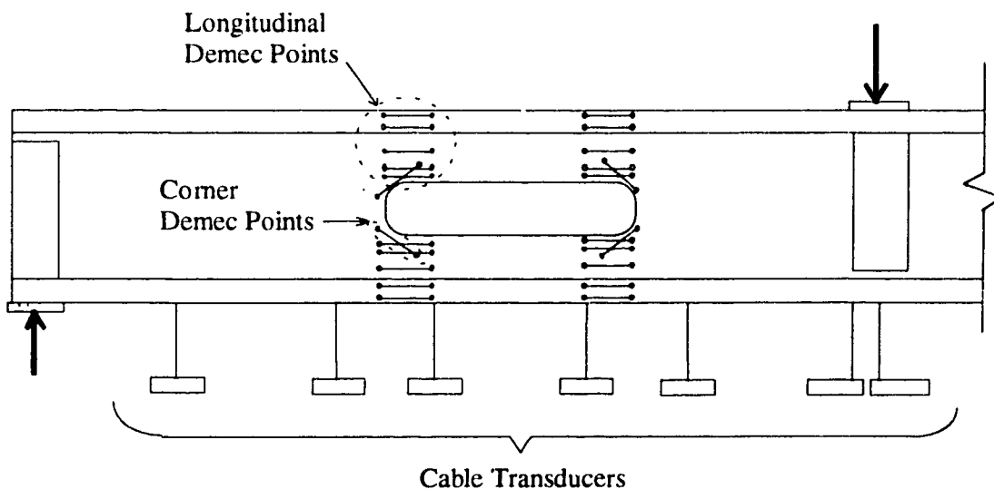
Figure 3.4. Instrumentation
