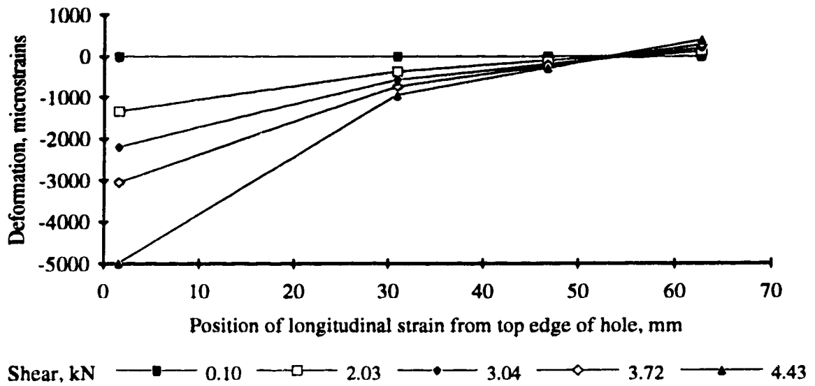
9.5dT4, Longitudinal demec readings at bottom left of hole
