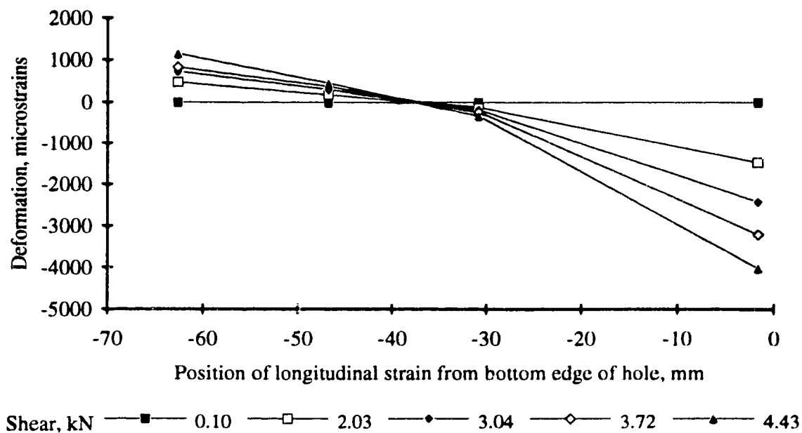
Figure 5.15. Longitudinal strain at the right section of the hole in specimen 9.5dT4
