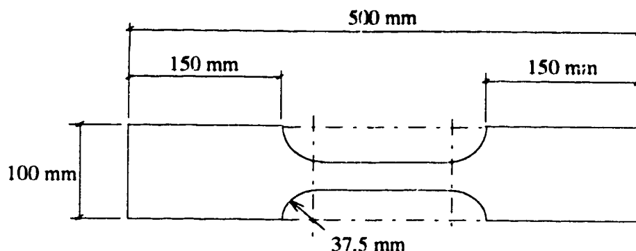
Figure 4.2. OSB tension coupon with face strands perpendicular to load
