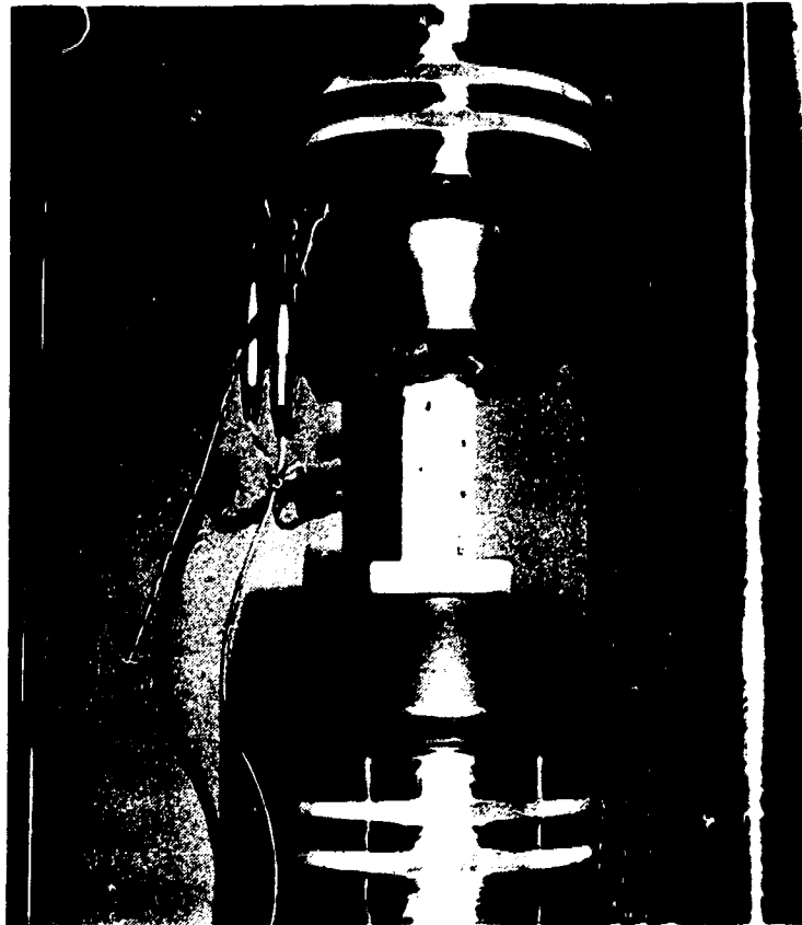
Figure 4.4. Chord compression test
