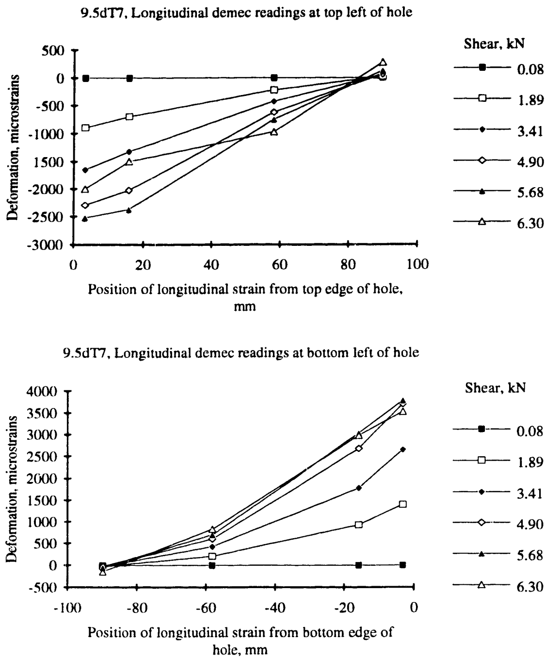
Figure 5.18. Longitudinal strain at the left section of the hole in specimen 9.5dT7
