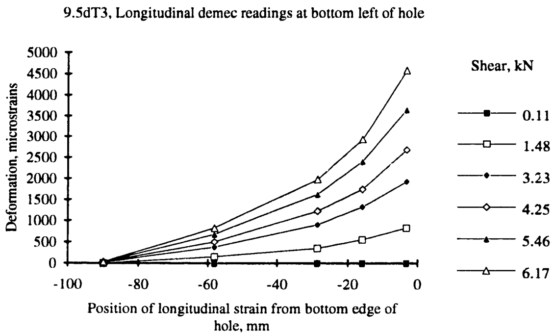
Figure 5.12. Longitudinal strain at the left section of the hole of specimen 9.5dT3
