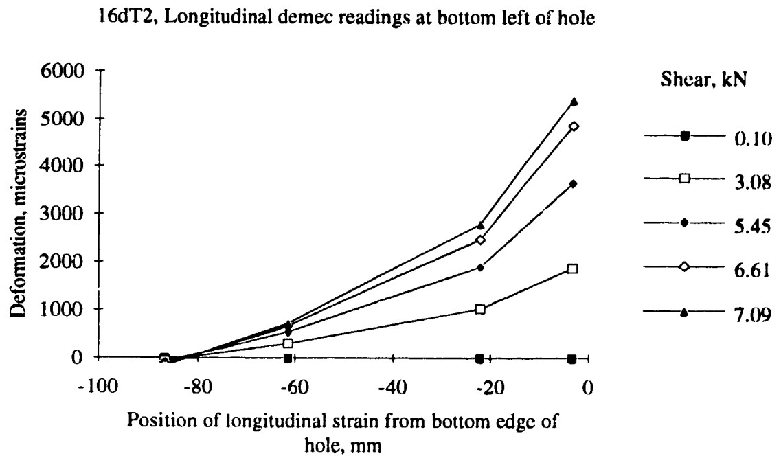
Figure 5.25. Longitudinal strain at the left section of the hole in specimen 16dT2
