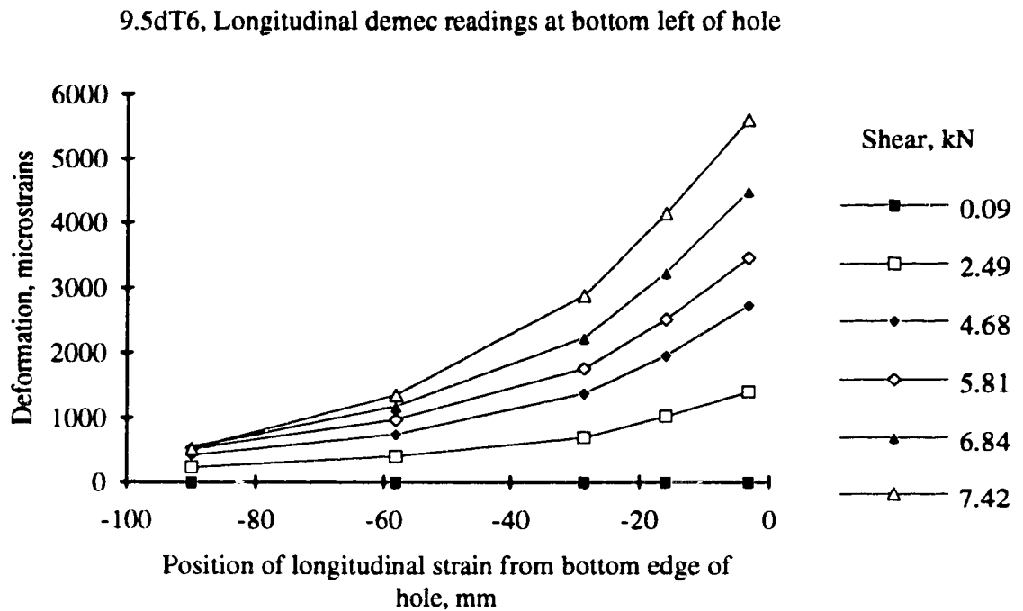
Figure 5.16. Longitudinal strain at the left section of the hole in specimen 9.5dT6
