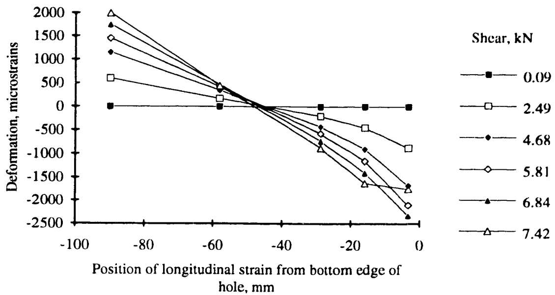
Figure 5.17. Longitudinal strain at the right section of the hole in specimen 9.5dT6
