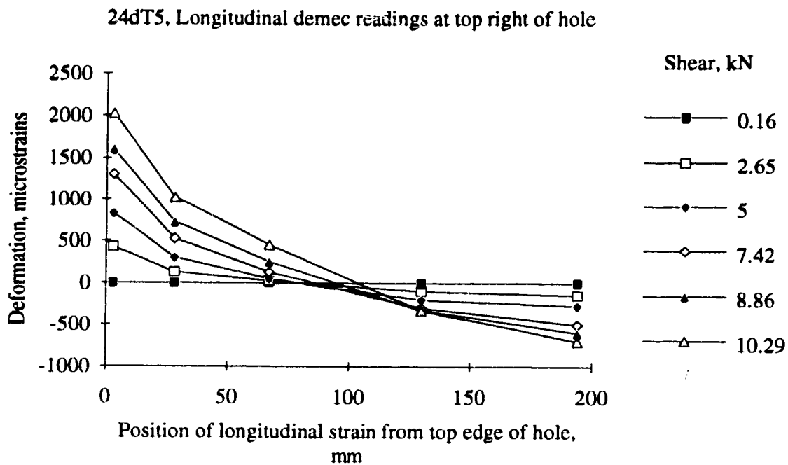
Figure 5.30. Longitudinal strains at the top right and bottom left corners of specimen 24dT5
