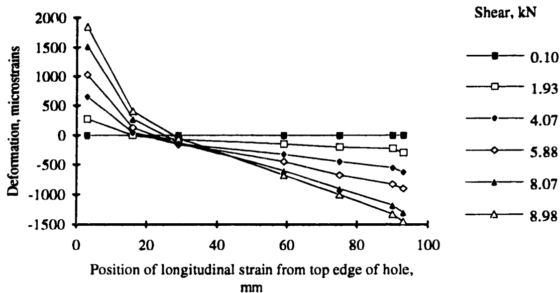
9.5dT1, Longitudinal demec readings at top right of hole
