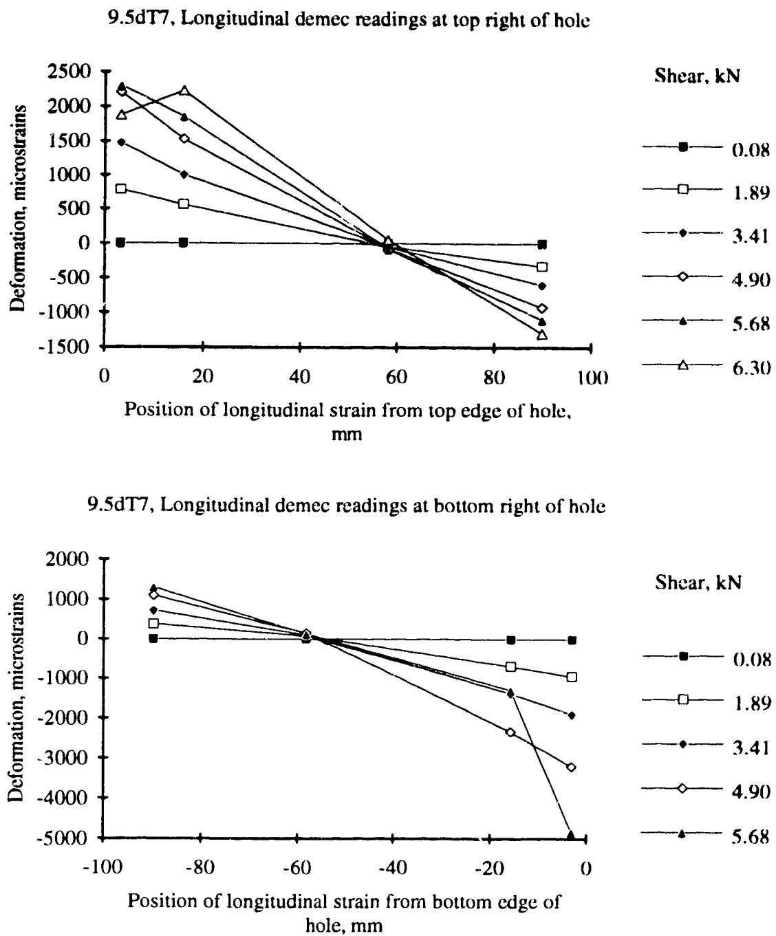
Figure 5.19. Longitudinal strain at the right section of the hole in specimen 9.5dT7
