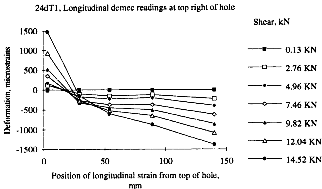
Figure 5.28. Longitudinal strains at the top right and bottom left corners of specimen 24dT1
