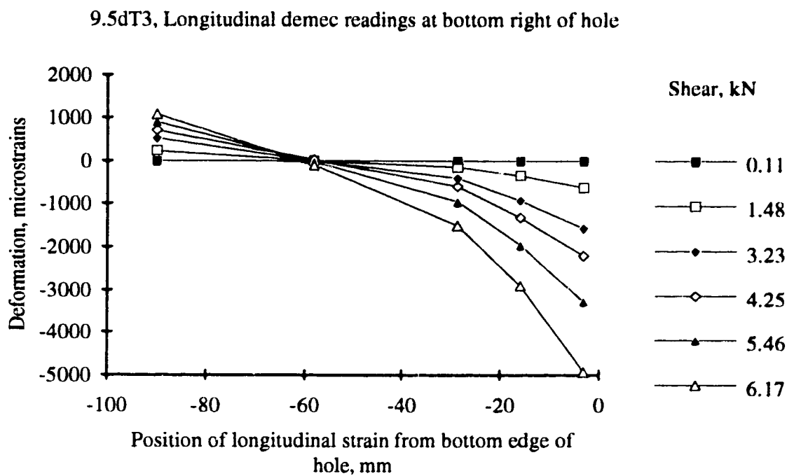
Figure 5.13. Longitudinal strain at the right section of the hole of specimen 9.5dT3
