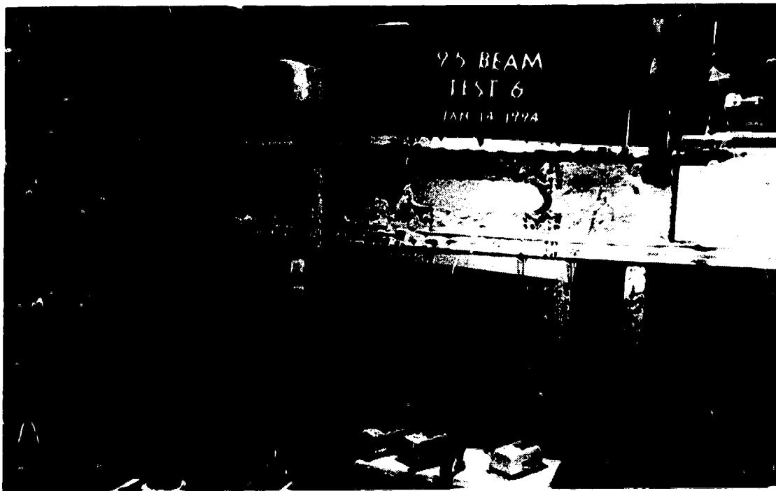
Figure 5.37. Vierendeel truss action exhibited in specimen 9.5dT6
