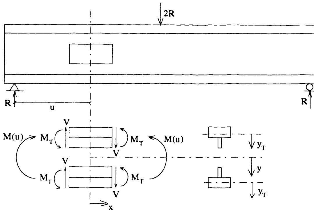
Figure 2.1, Vierendeel analysis
