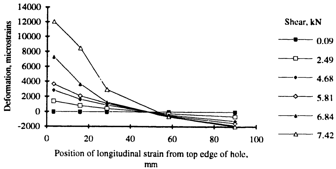
9.5dT6, Longitudinal demec readings at top right of hole
