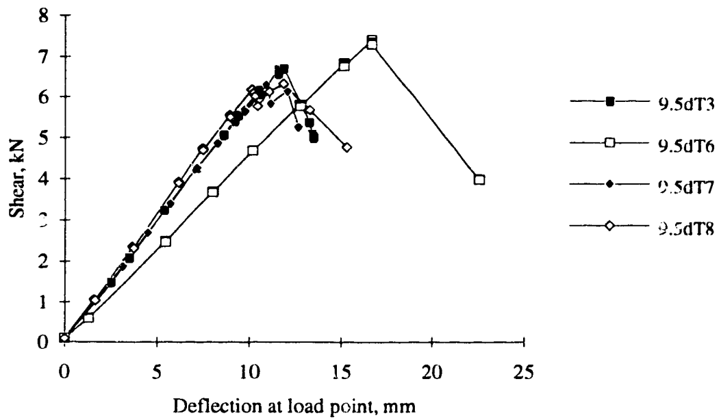
Figure 5.4. Shear vs. deflection of beam during test, specimens 9.5dT3, 6, 7 and 8
