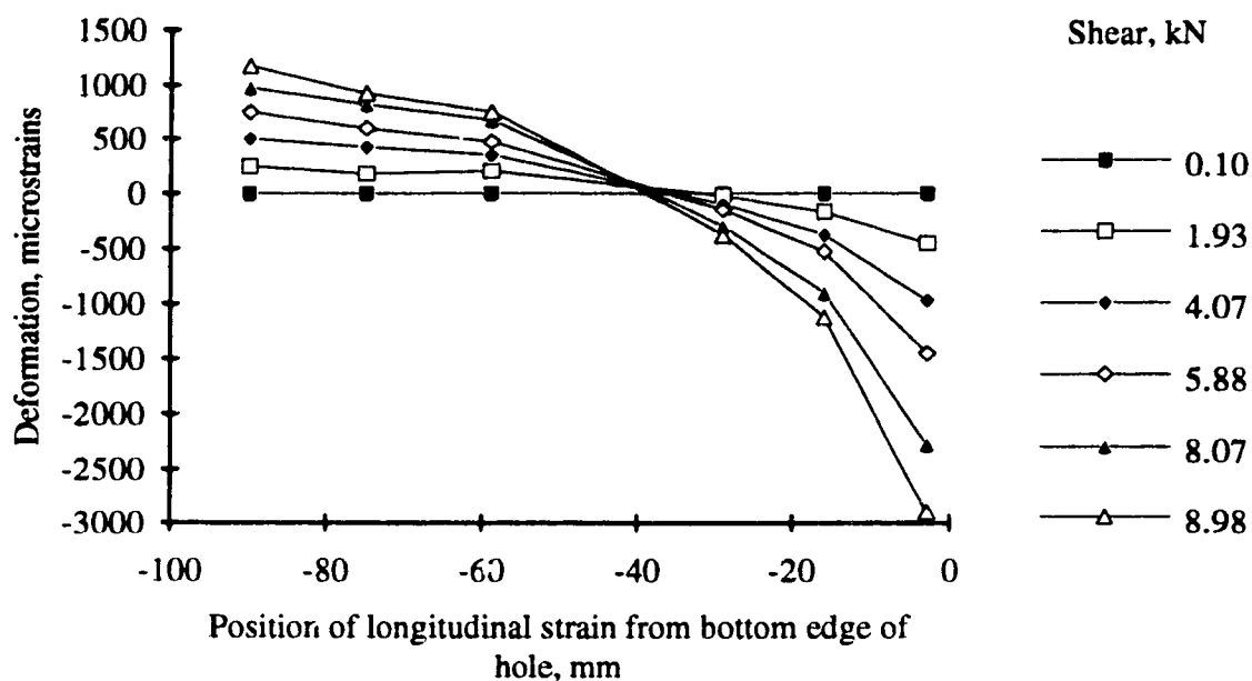
Figure 5.10. Longitudinal strain at the right section of the hole in specimen 9.5dT1
