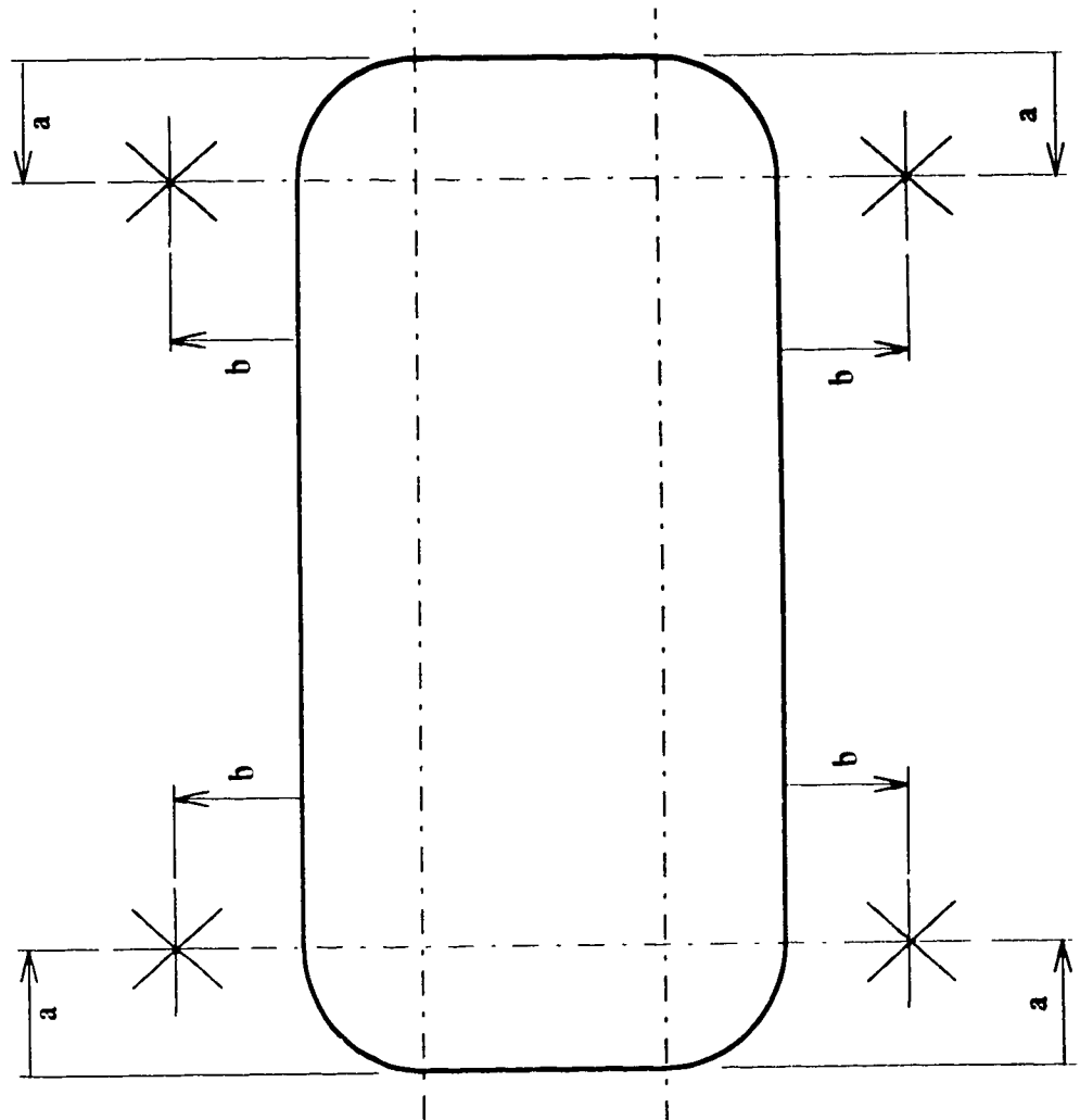
Position of corner rosettes with respect to the hole for specimens 24dT1, 3, and 5
