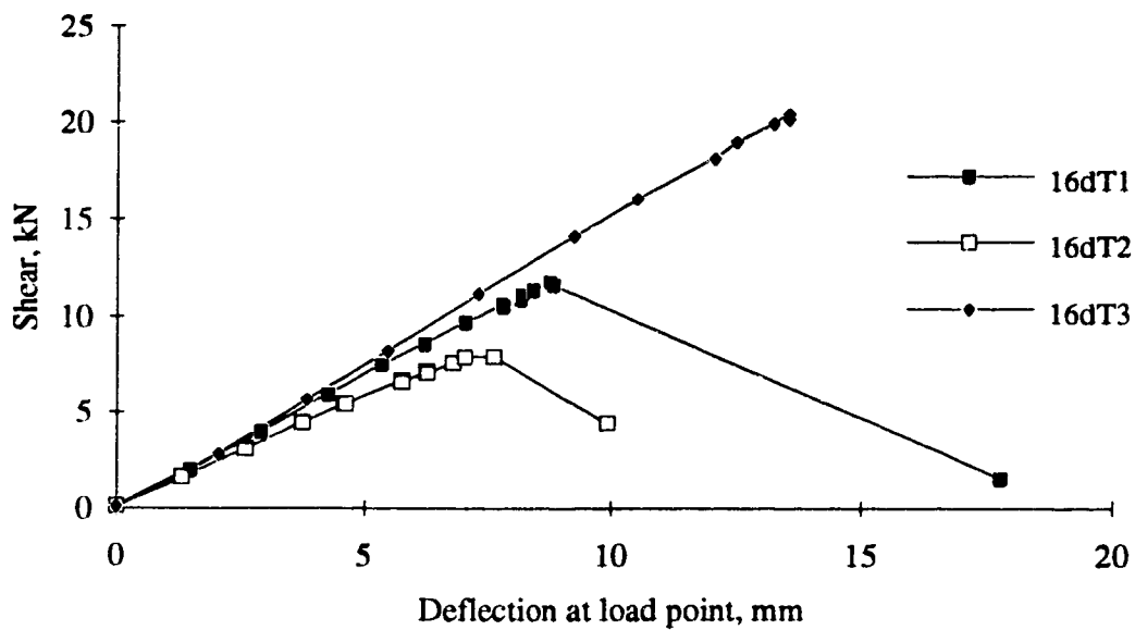
Figure 5.2. Shear vs. deflection of beam during test, 406 mm specimens
