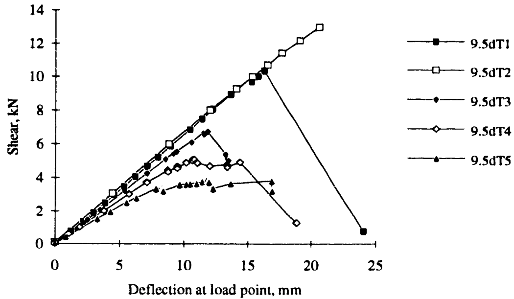
Figure 5.3. Shear vs. deflection of beam during test, specimens 9.5dT1 to 9.5dT5
