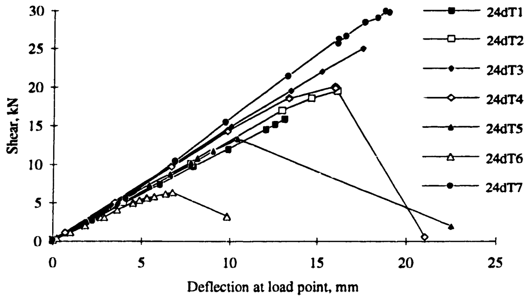
Figure 5.1. Shear vs deflection of beam during test, 610 mm specimens
