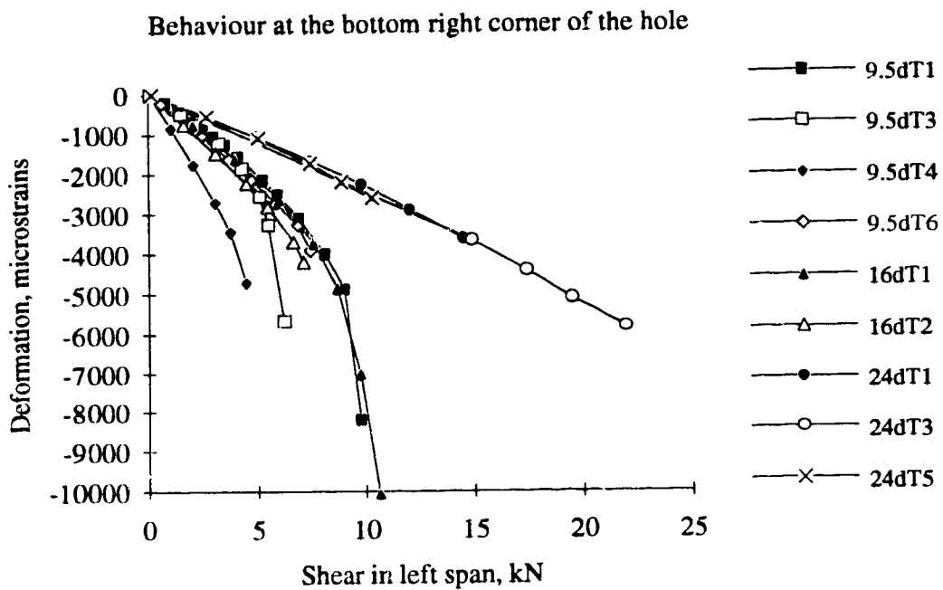
Figure 5.33. 45 degree demec readings at the right corners of the hole
