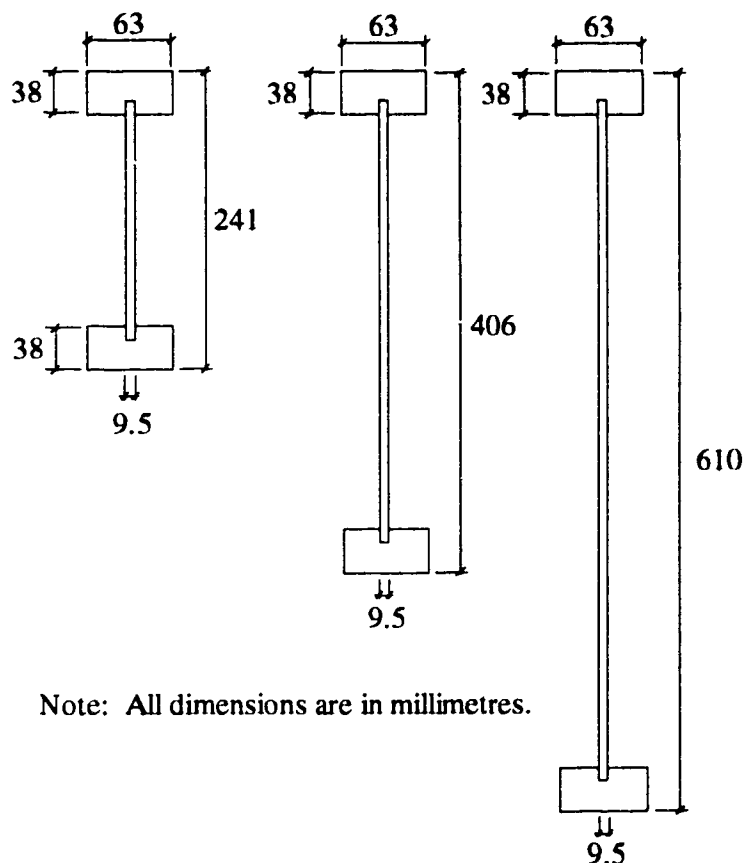
Figure 3.1, Nominal dimensions of OSB I-beam specimens
