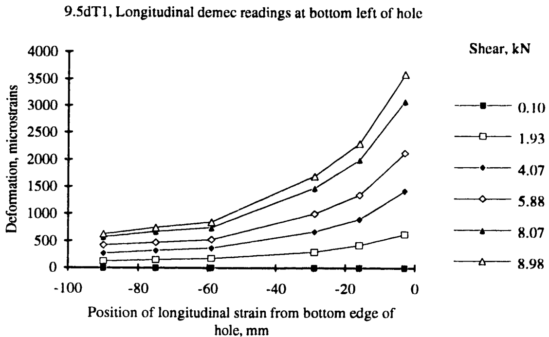
Figure 5.9. Longitudinal strain at the left section of the hole in specimen 9.5dT1
