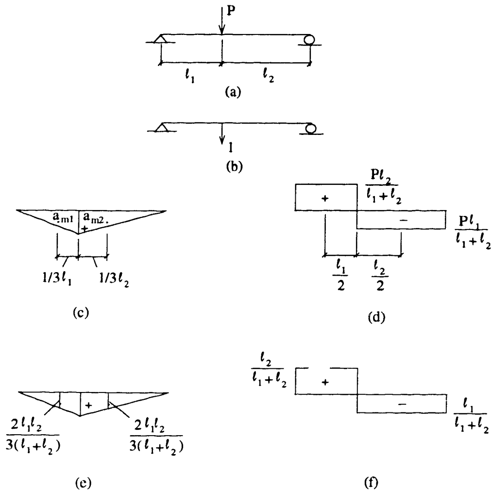
Figure 6.1 Loading on reference beam, (a) Beam (b) Coordinate system
