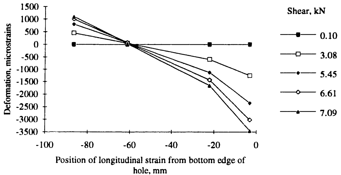
Figure 5.26. Longitudinal strain at the right section of the hole in specimen 16dT2
