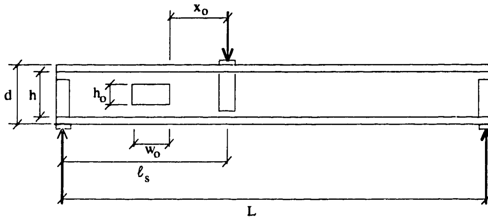
Figure 3.2. Schematic test set-up
