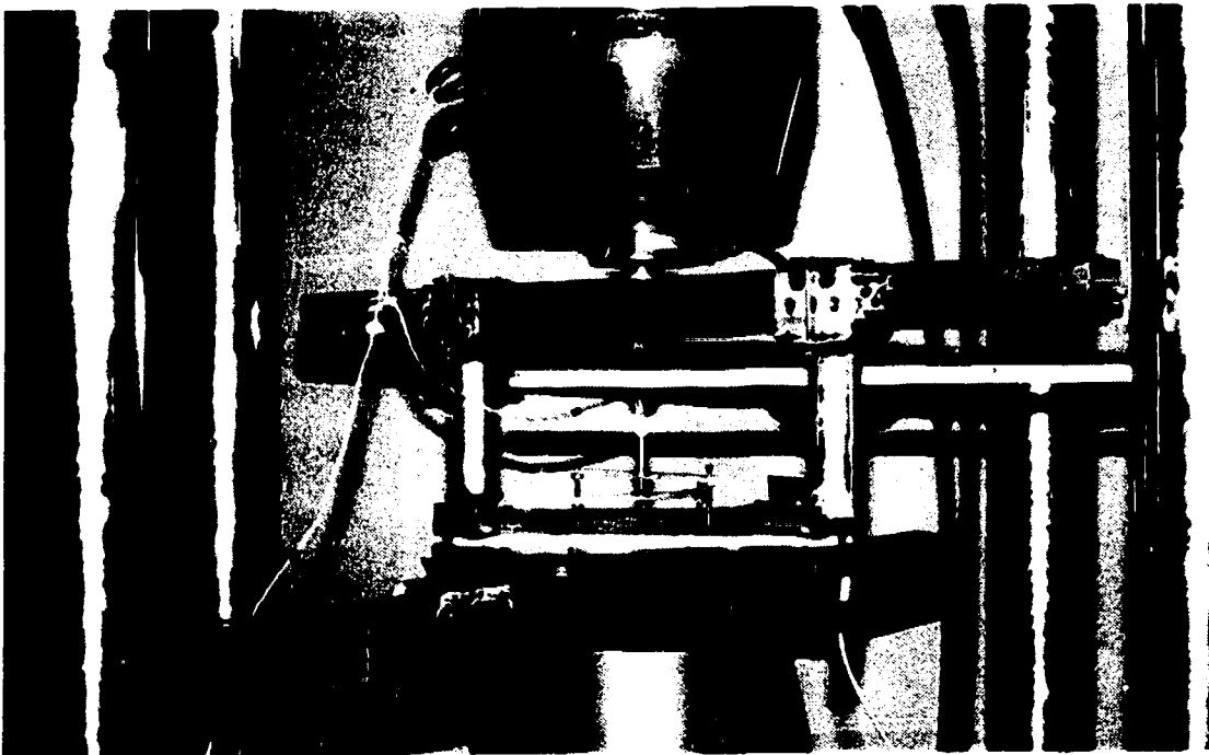
Figure 4.3. Plate shear modulus tests for OSB
