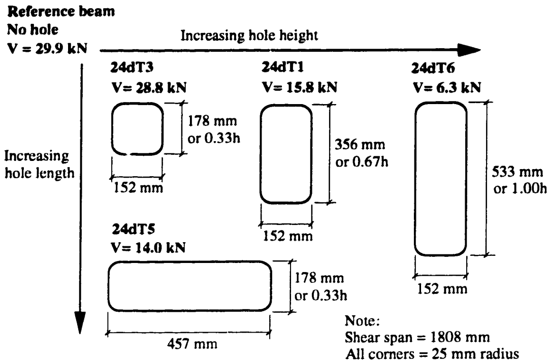
Figure 5.5. Effect of hole size in 610 mm beams
