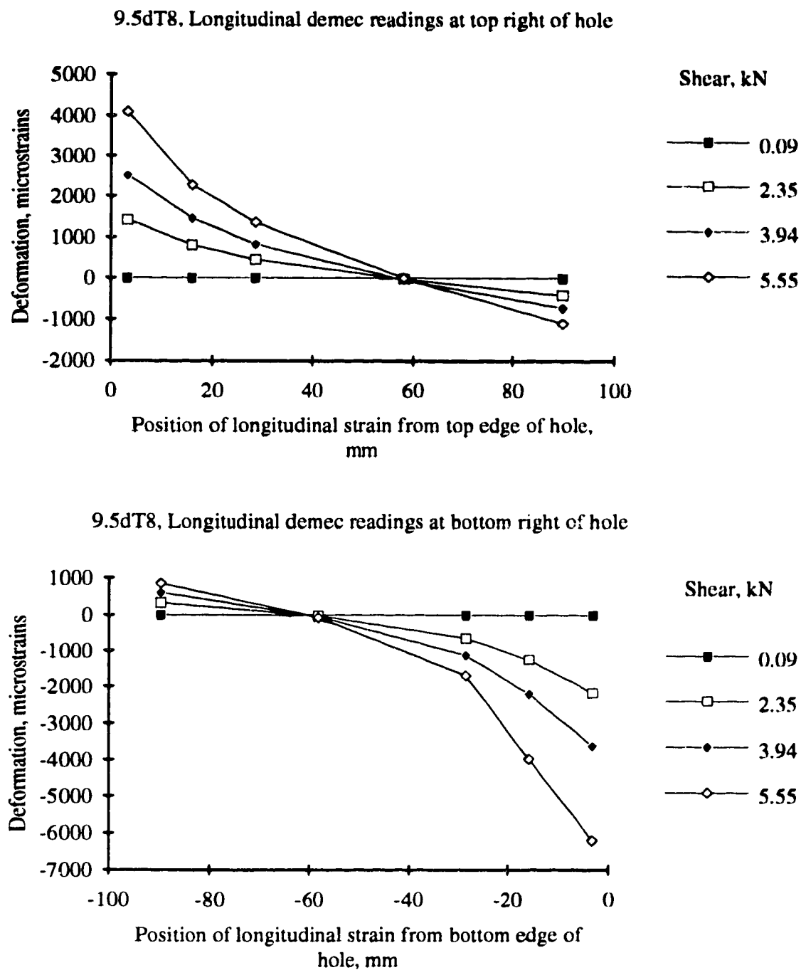
Figure 5.21. Longitudinal strain at the right section of the hole in specimen 9.5dT8
