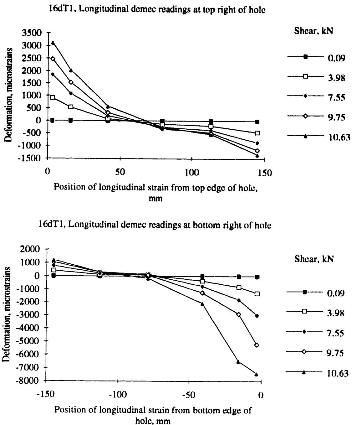
Figure 5.23. Longitudinal strain at the right section of the hole in specimen 16dT1
