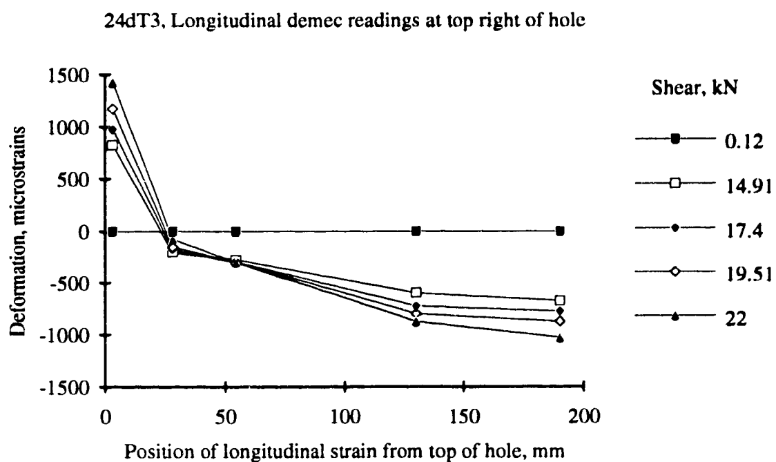
Figure 5.29. Longitudinal strains at the top right and bottom left corners of 24dT3
