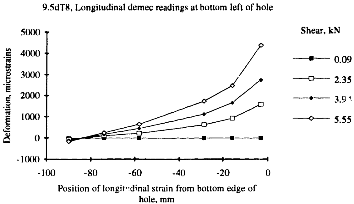
Figure 5.20. Longitudinal strain at the left section of the hole in specimen 9.5dT8
