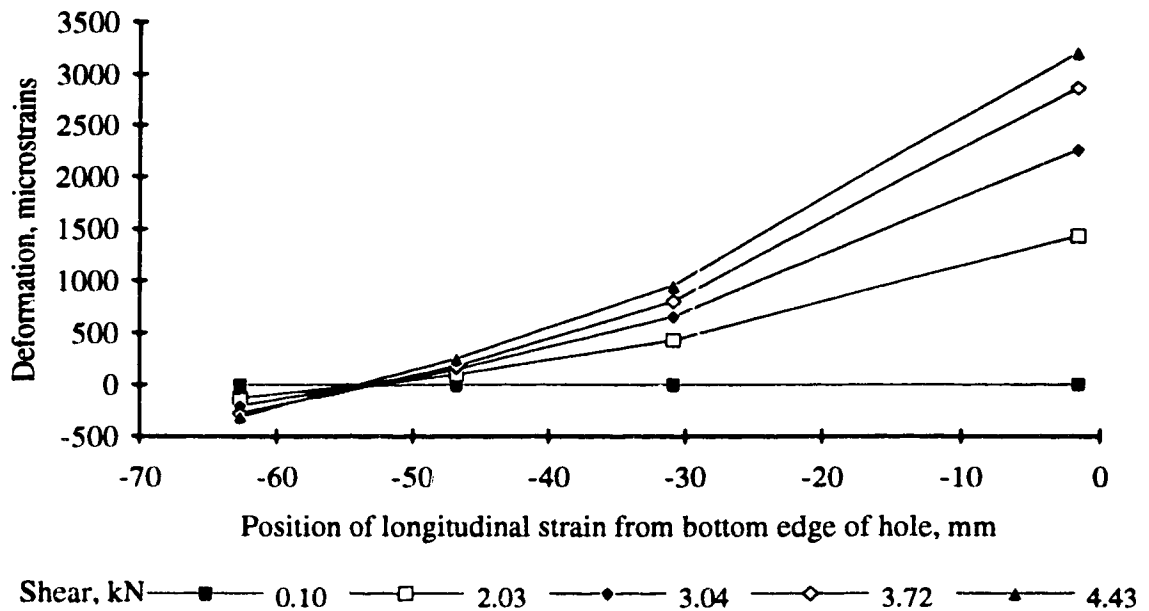
Figure 5.14. Longitudinal strain at the left section of the hole in specimen 9.5dT4
