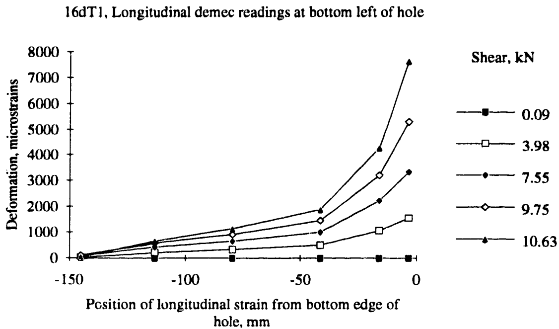
Figure 5.22. Longitudinal strain at the left section of the hole in specimen 16dT1
