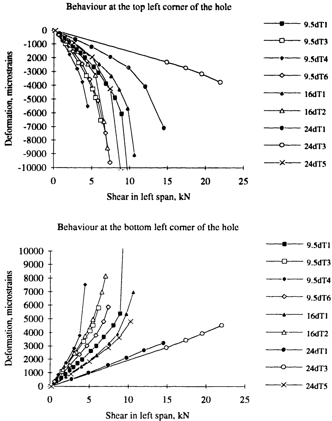
Figure 5.32. 45 degree demec readings at the left corners of the hole
