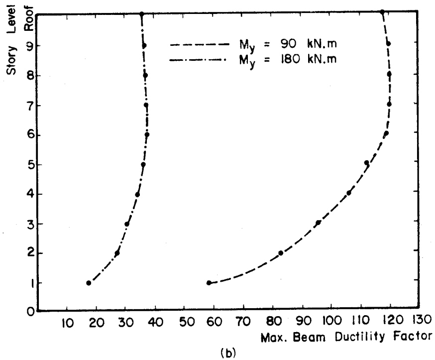
Figure 6-3 Maximum Beam Moments and Maximum Beam Ductility Factor Showing the Effect of Beam Strength (Slender Beams, R.C.)
