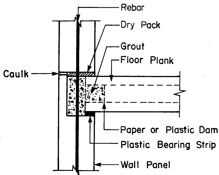
(b) Platform Connection (Reinforcing)
