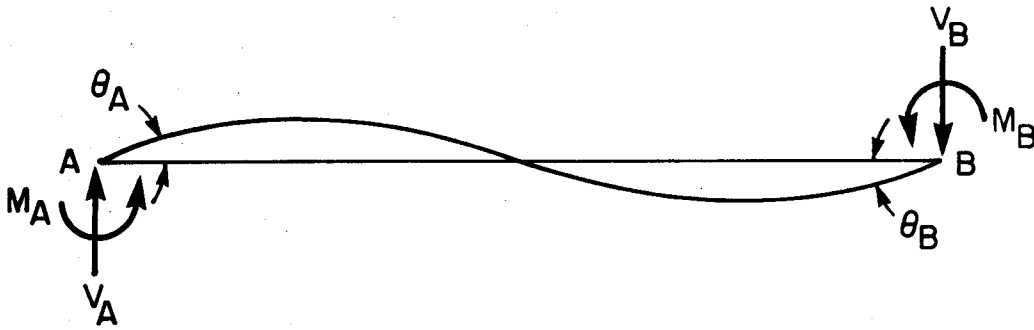
(a) Displaced Configuration of Coupling Beams
