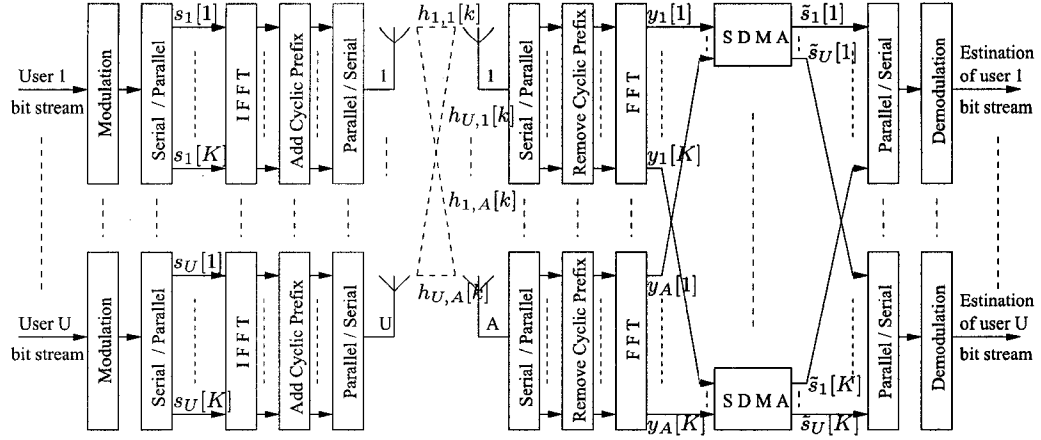
Fig. 2.1. System model.
