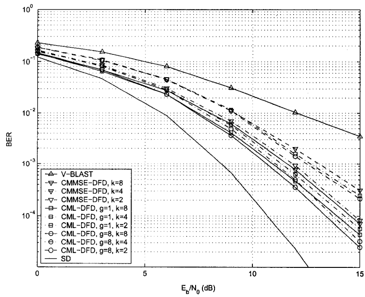
Fig. 3.5. Performance comparison of combined constrained and decision feedback detectors in an 8 \times 8 BPSK MIMO system.
