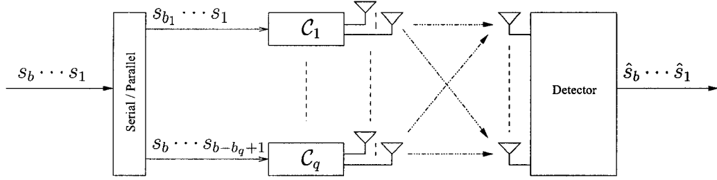
Fig. 2.6. System model.
