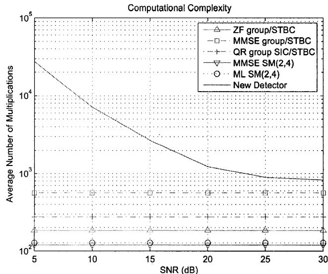
Fig. 2.10. Computational complexity of a (4,4) STBC/SM system (4QAM).
