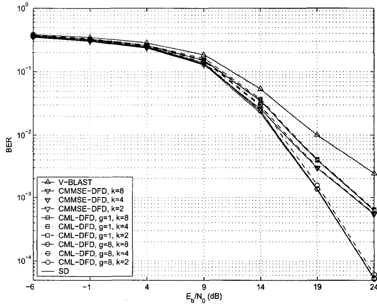
Fig. 3.9. Performance comparison of combined constrained and decision feedback detectors in an 8 \times 8 16QAM MIMO system.
