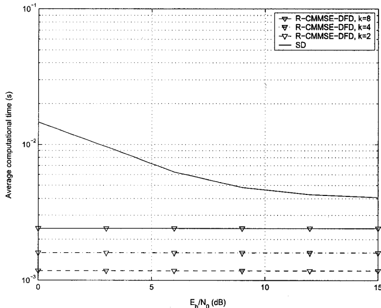
Fig. 3.8. Average computational time of combined constrained and decision feedback detectors in an 8 \times 8 BPSK MIMO system using real constraints.
