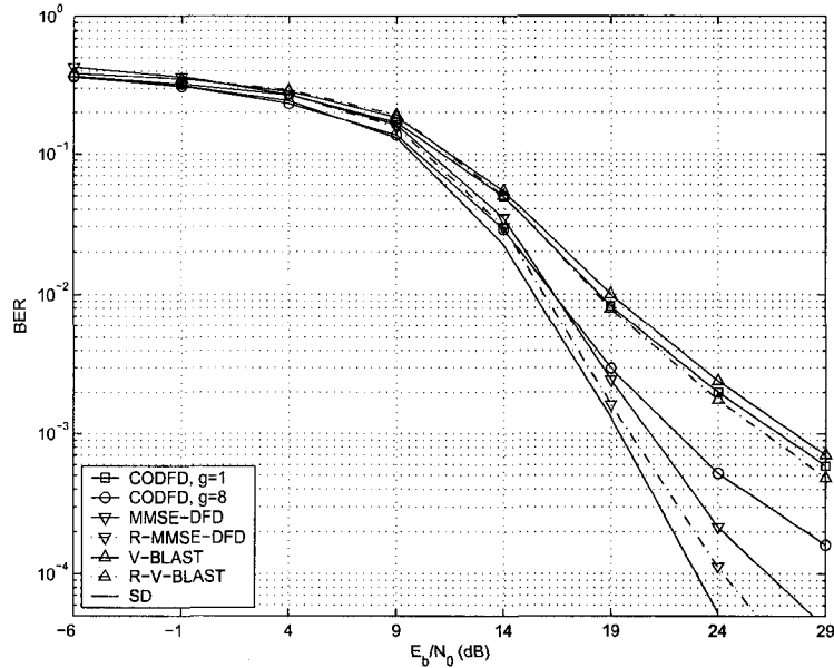
Fig. 3.4. Performance comparison of constrained ordering decision feedback detectors in an 8 \times 8 MIMO system with 16QAM.
