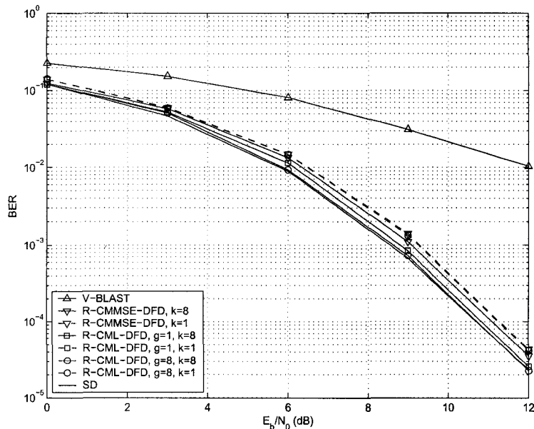
Fig. 3.7. Performance comparison of combined constrained and decision feedback detectors in an 8 \times 8 BPSK MIMO system using real constraints.
