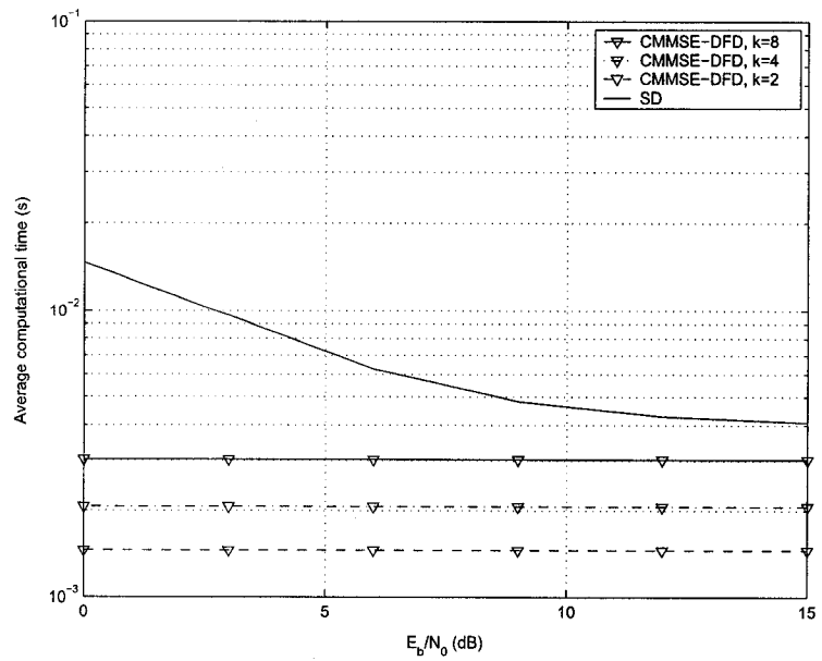
Fig. 3.6. Average computational time of combined constrained and decision feedback detectors in an 8 \times 8 BPSK MIMO system.
