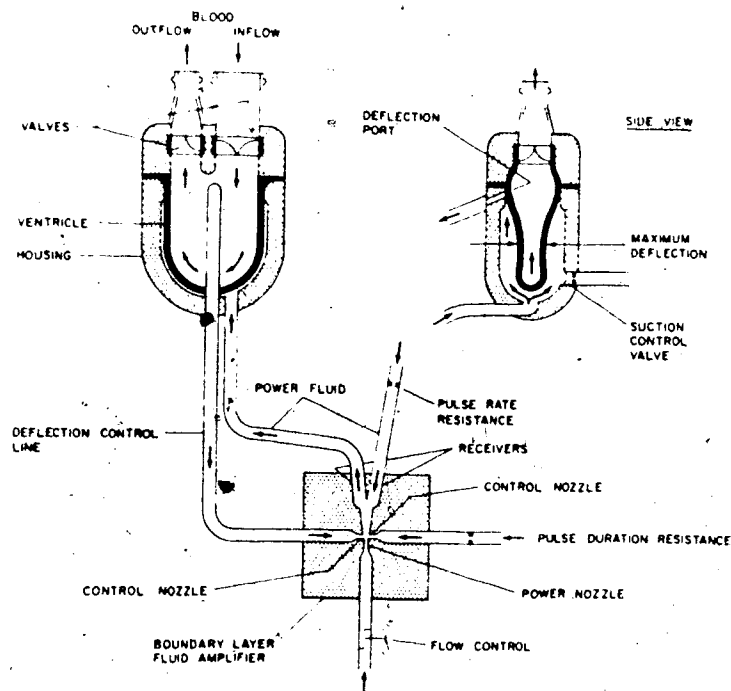
Fig. 1.9 One sac-type heart used a fluid amplifier control mechanism.
