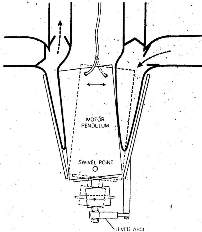
Fig. 1.2 Pendulum artificial heart. Swinging pendulum collapses left and right ventricle sacs.
