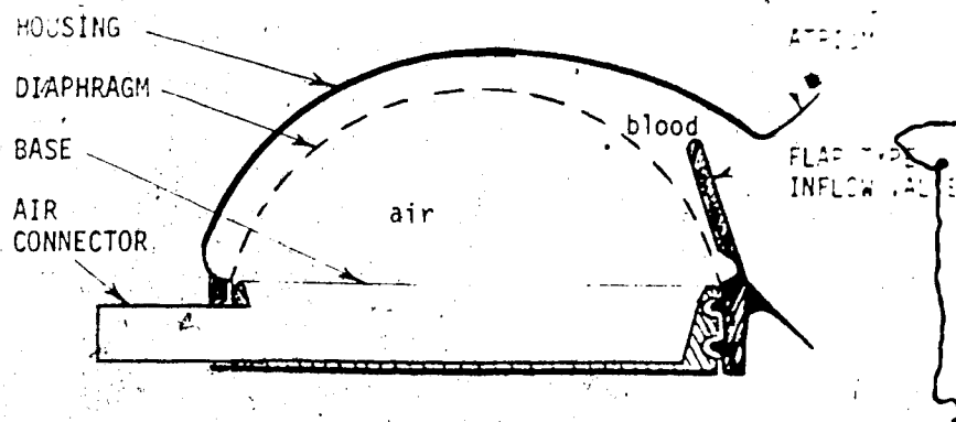
Fig. 1.16 World record survivals of up to 264 hours in calves have been reported with this air-powered silicone rubber artificial heart with hemispherical ventricles.
