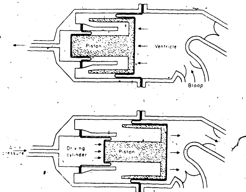
Fig. 1.8 Rolling diaphragm artificial heart is powered by compressed air and the ventricles fill by venous pressure.
