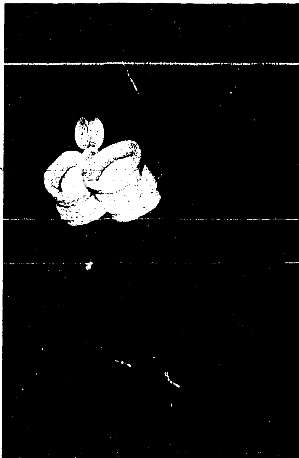
Fig. 3.20 Mk VII design was fabricated entirely from natural rubber but could not generate sufficient left ventricular pressure.
