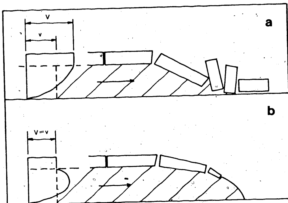
Figure 6.6 Laminar flow of slurry and solid flakes. (a) Self-damming Poiseuille flow, (b) Flakes slowed down by side friction — sustained flow.
