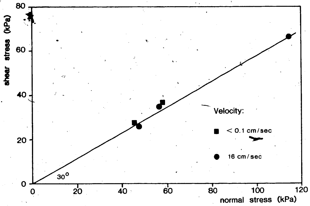
Figure 12.7 Strength envelopes of the dry 8—10 sand (coarse).
