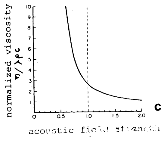
Fig. 10.14 Acoustic fluidization: a) strength reduction b) vibro-viscosity vs. acceleration ratio (Barkan, 1962); c) vibro-viscosity vs. stress amplitude (theoretical, Melosh, 1979)
