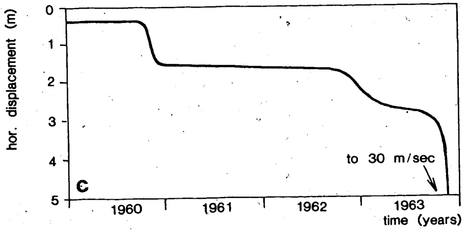
Figure 1.1 Time history of landslides. (a) Concept by Terzaghi (1950) (b) soft clay excavation (da Silva, 1979) (c) Vajont rock slide (Mueller, 1964).
