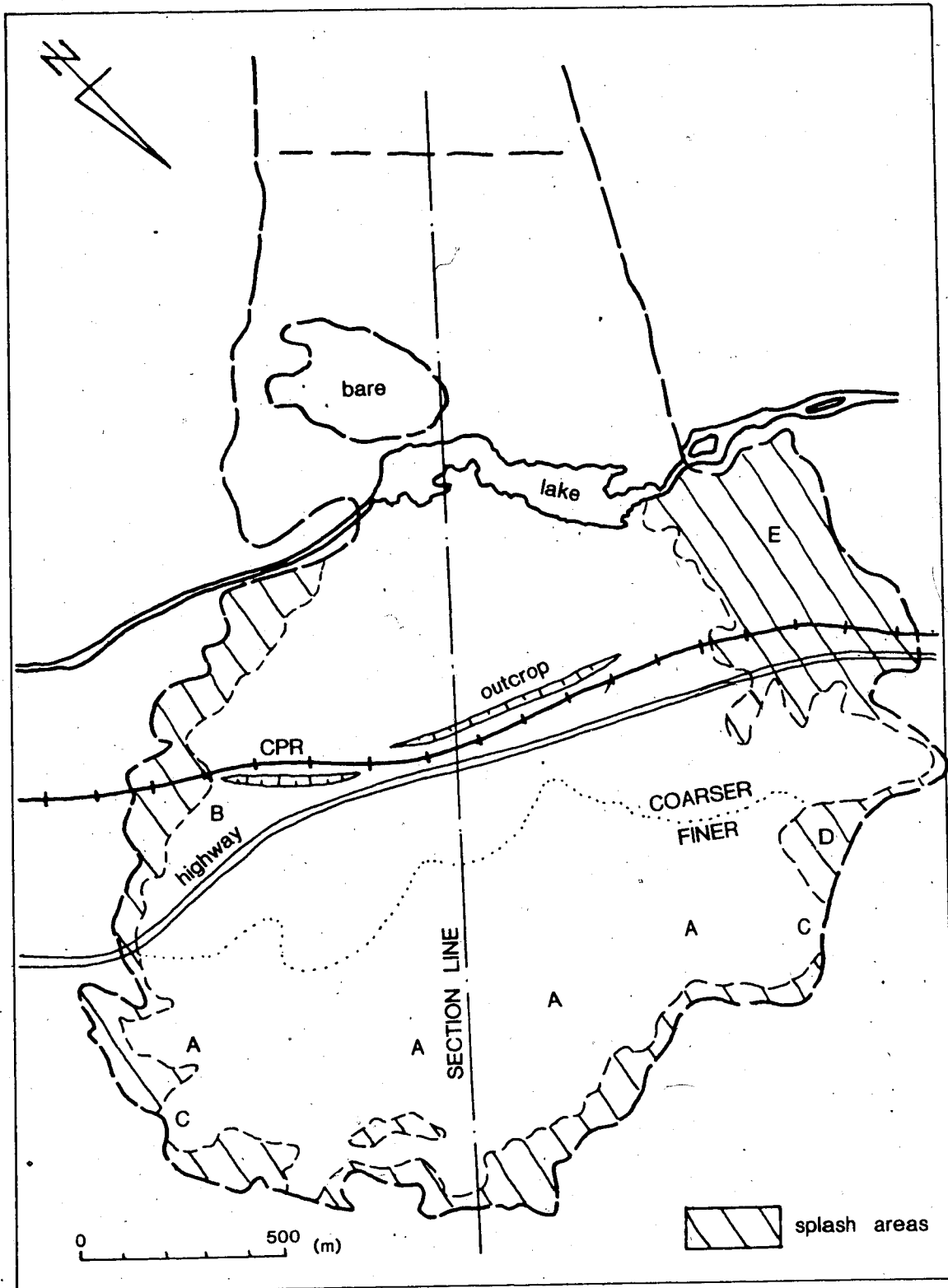
Figure 10.5a Plan of the Frank Slide deposit. Overlay for Fig. 10.5.
