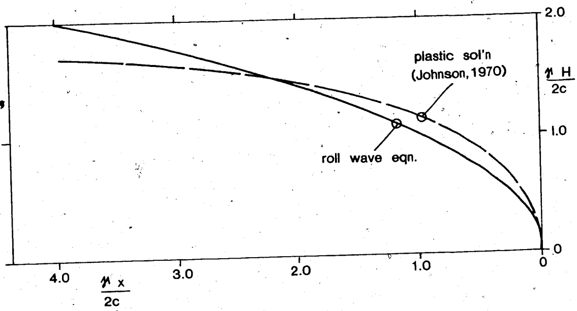
Figure 5.3 Flow front profile for a purely cohesive material.
