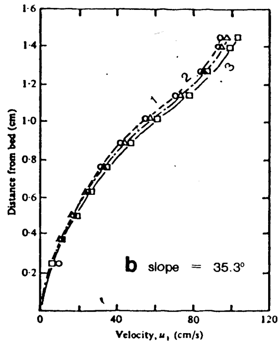
Figure 7.1. Grain flow profiles recorded by Savage (1979) (using polystyrene beads) 1, 2 and 3 refer to stations 33, 64 and 94 cm from flume entry.
