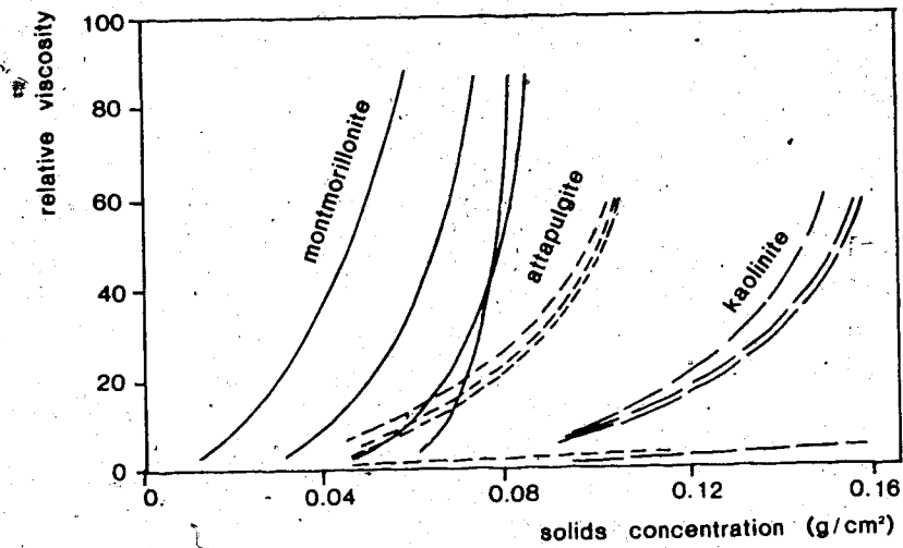
Figure 6.2 Viscosity — concentration relationship for three clays with various pore water chemistry (Searle and Grimshaw, 1959).
