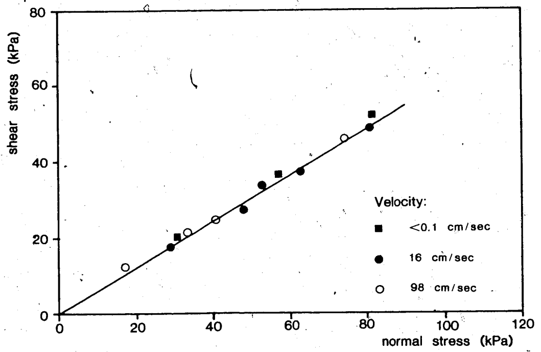
Figure 12.10 Strength envelopes of the 4:2 sand and rock flour mixture.
