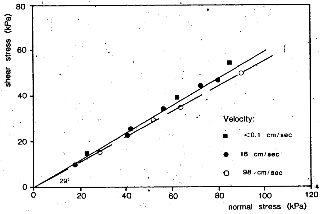
Figure 12.9 Strength envelopes of the 4:1 sand and rock flour mixture.
