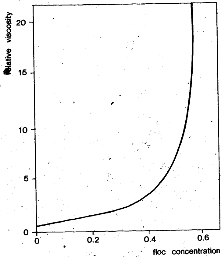
Figure 6.1 Viscosity vs. floc concentration for flocculated kaolin. (Michaels and Bolger, 1962).
