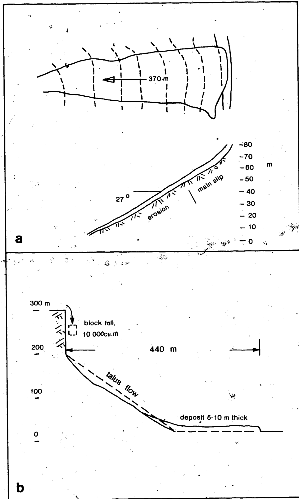
Figure 9.2 Debris avalanches. (a) Hong Kong flow of fill (Lumb, 1975) (b) Modalen flow slide (Bjerrum and Jorstad, 1968).
