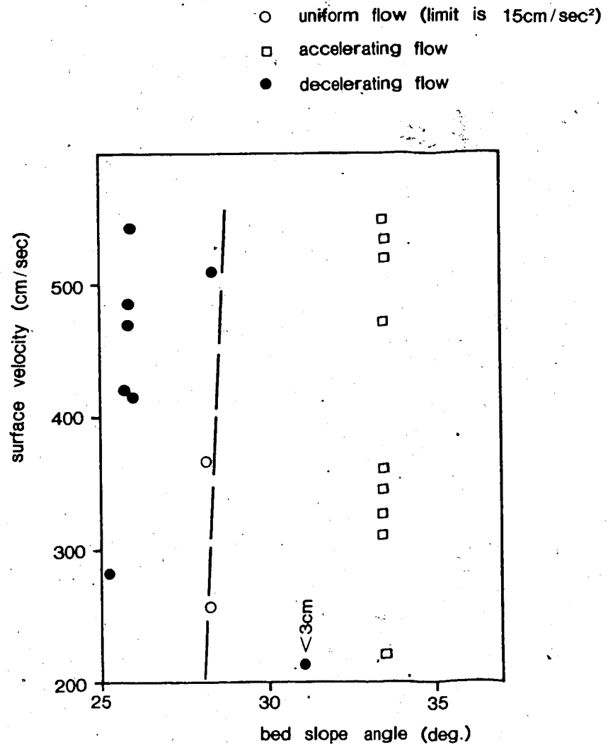
Figure 11.12 Flow classification versus bed slope angle and surface (maximum) velocity.
