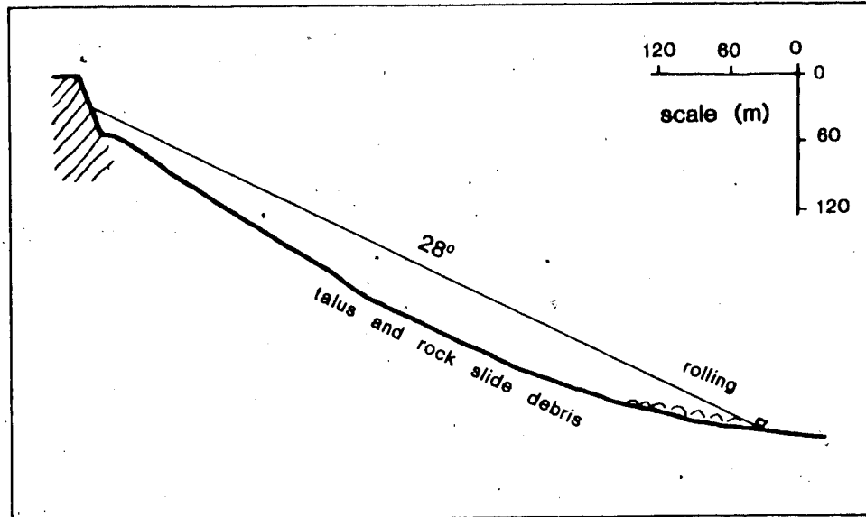
Figure 2.1 Path of a 60 cu.m boulder (Govi, 1977).
