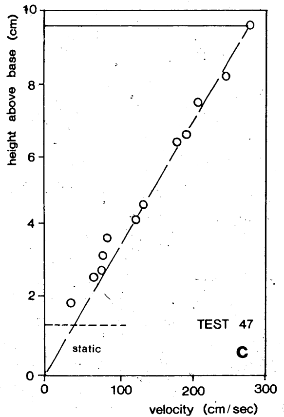
Figure 11.22 Velocity profiles measured through the side of the flume.
