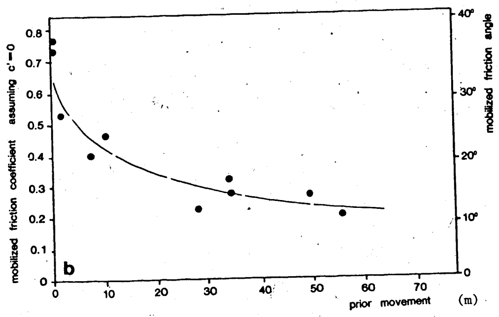
Figure 3.10 Back calculated variation of the mobilized effective friction angle. (a) Vs. strain rate in shear zone, (b) vs. displacement. Data from Gould (1960).
