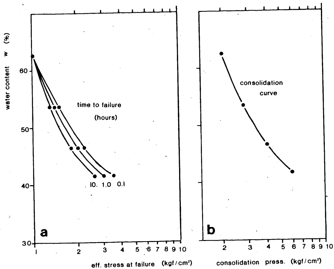
Figure 3.9 Effective stress at peak strength in undrained triaxial tests on sensitive clay as a function of w and of rate of testing (data from Crawford, 1969).
