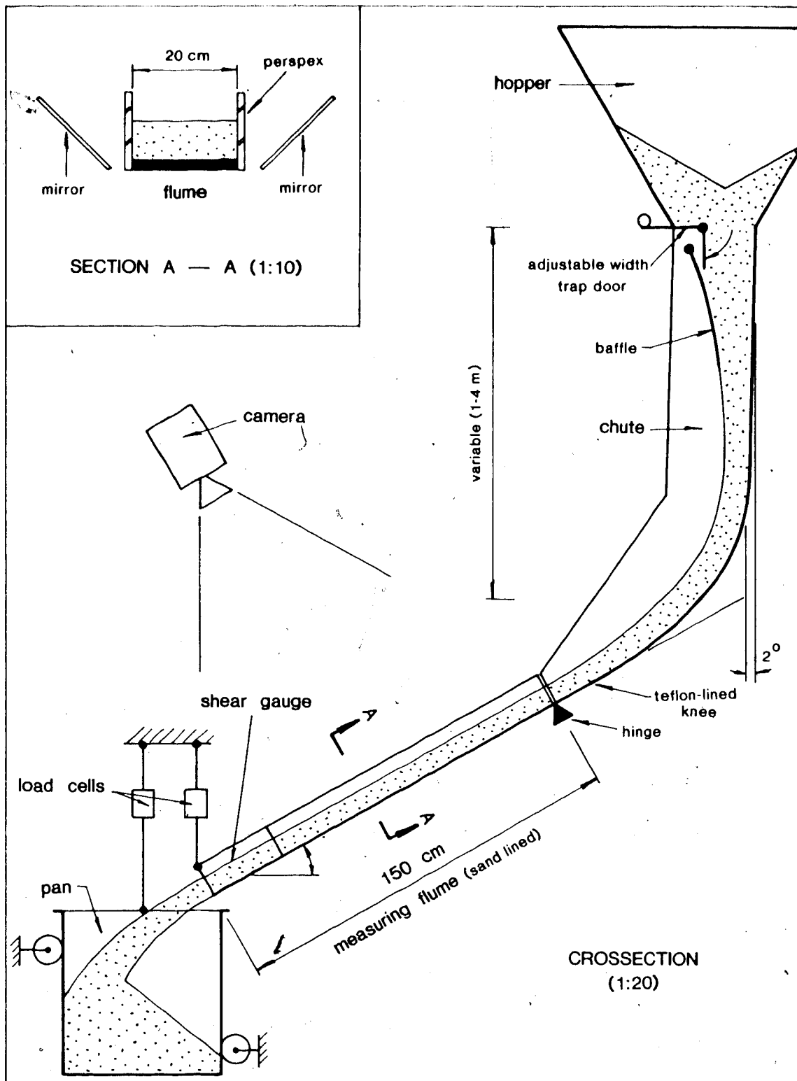
Figure 11.1 Schematic diagram of the test flume.
