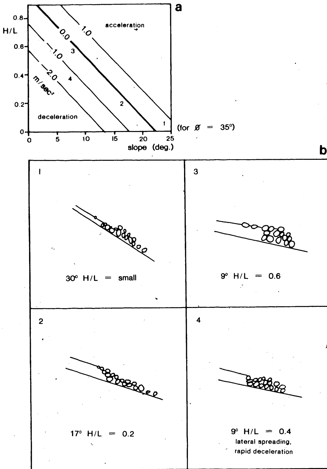
Figure 9.6 Dynamic equilibrium of a frontal boulder accumulation.
