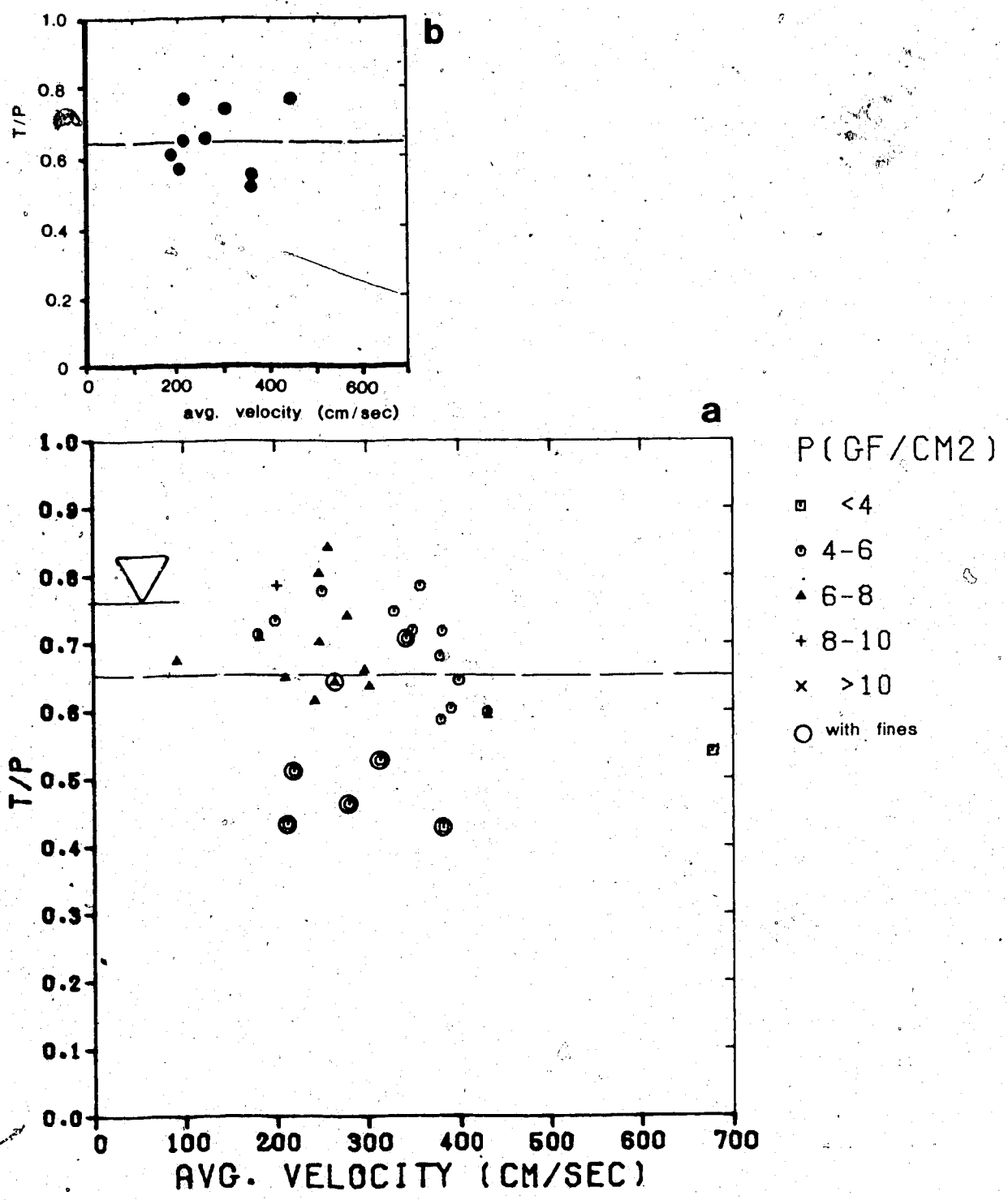
Figure 11.11 Bed friction coefficient, angular sand: (a) From direct measurement, (b) from accelerations.
