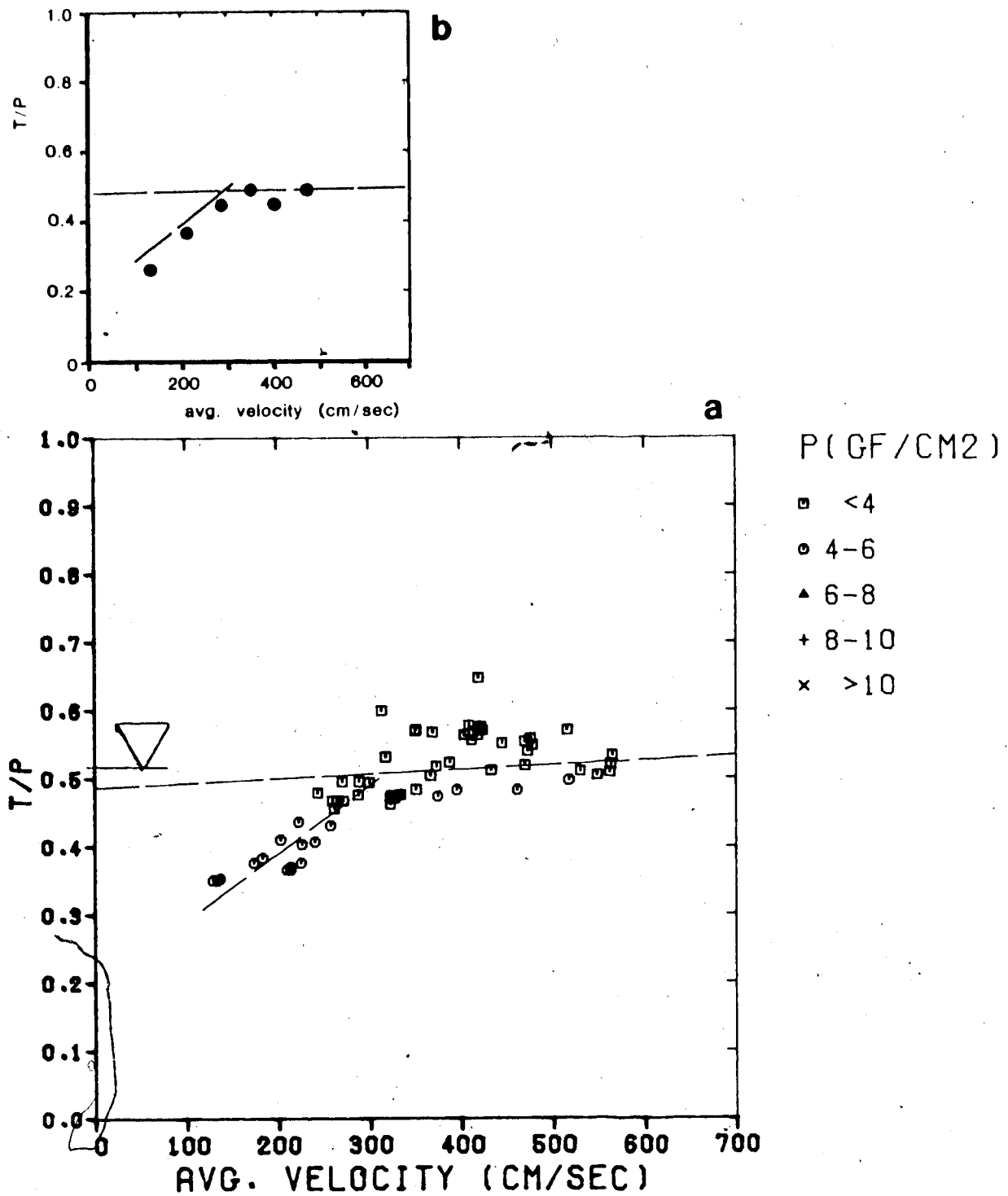
Figure 11.10 Bed friction coefficient, Polystyrene beads. (a) From direct measurement, (b) from accelerations.
