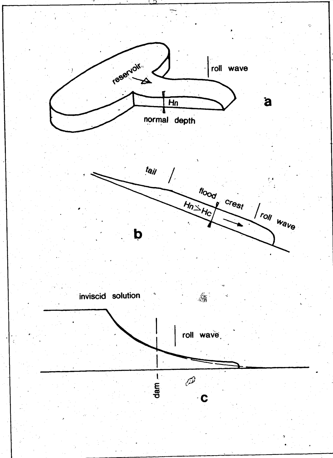
Figure 5.1 Roll wave: (a) during steady discharge from a reservoir, (b) at the front of a shallow flood, (c) at the front of the dam break wave (variable velocity).
