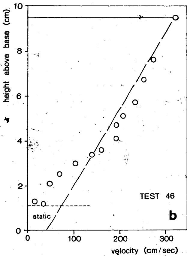
Figure 11.22 Velocity profiles measured through the side of the flume.
