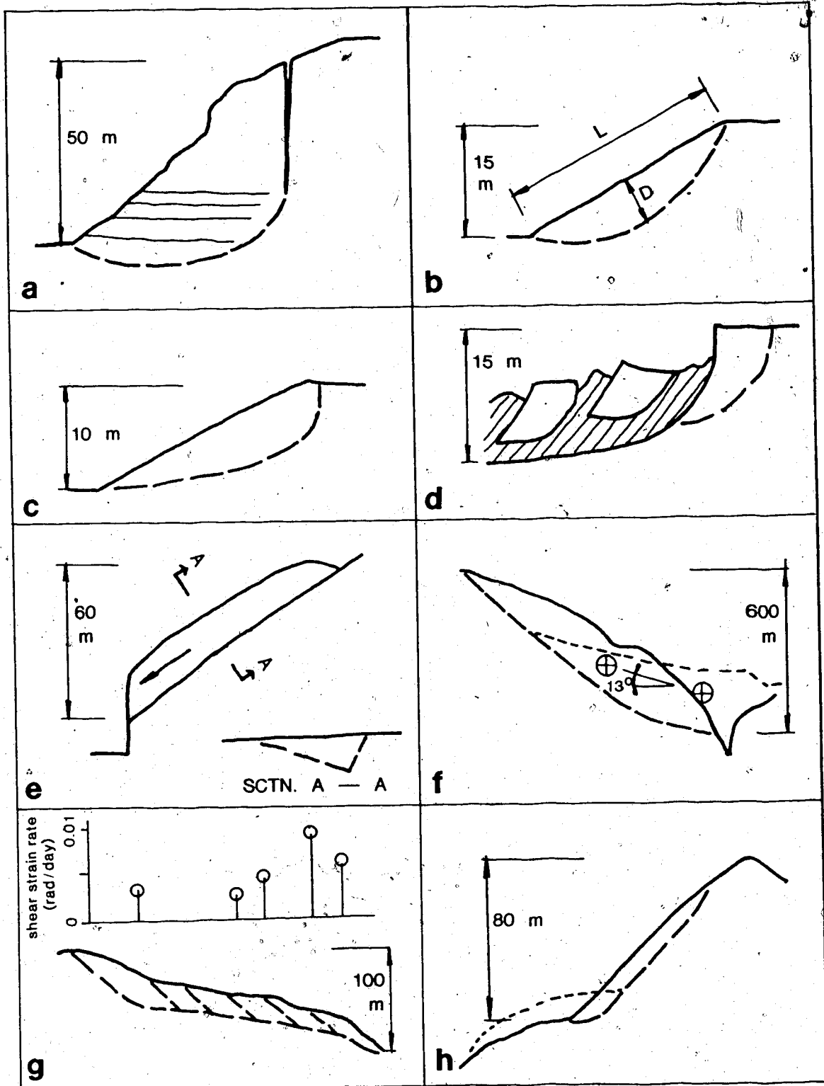
Figure 3.1 Crosssections of typical slides and slumps.
