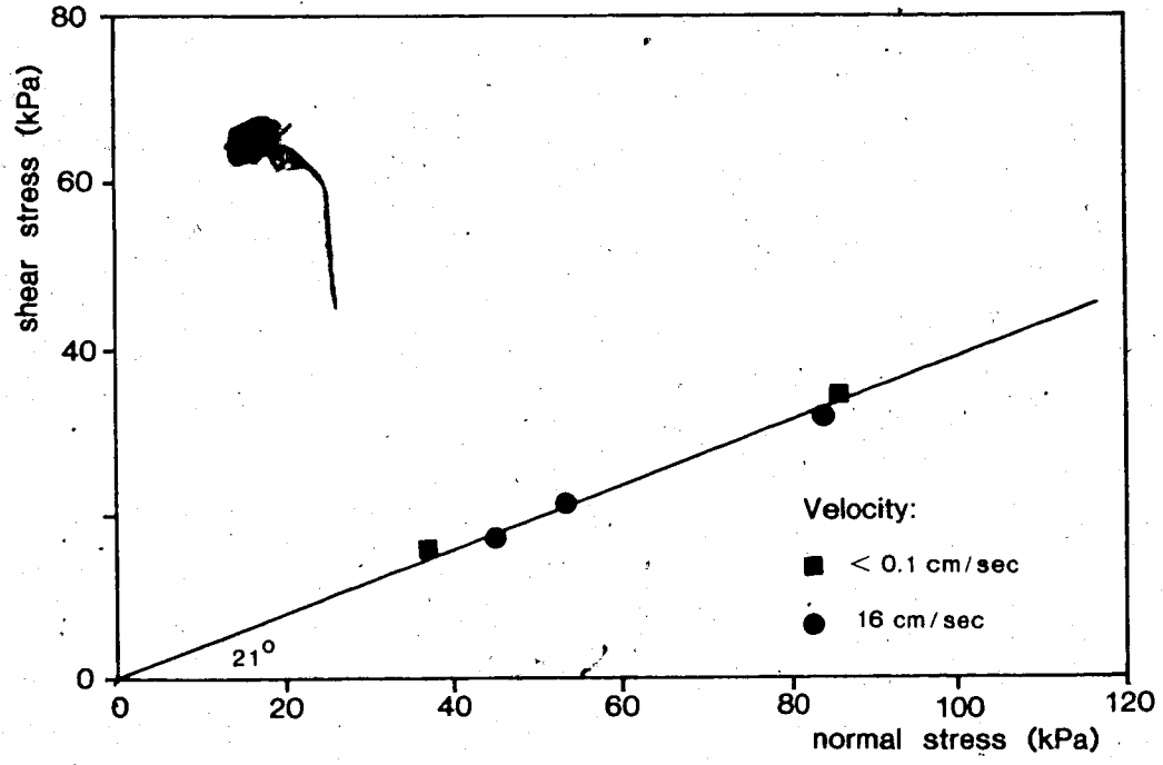
Figure 12.8 Strength envelopes of the polystyrene beads.
