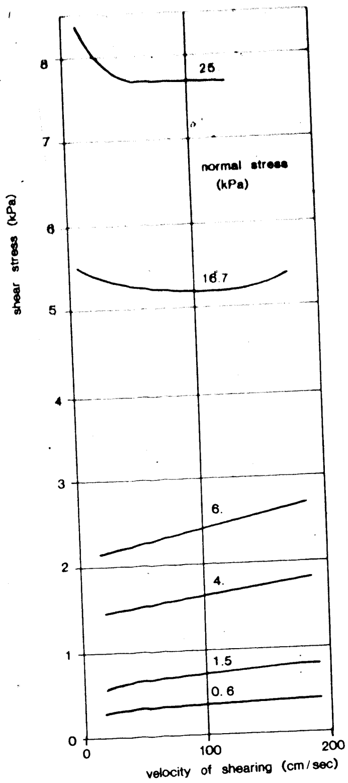
Figure 3.5 Critical state friction in glass beads as a function of velocity of shearing and normal stress (Bridgwater, 1972).
