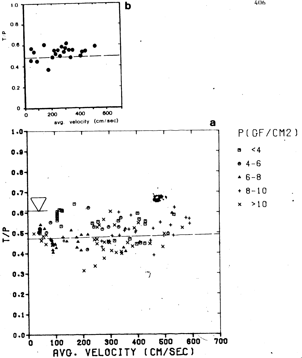
Figure 11.9 Bed friction coefficient, Ottawa sand. (a) From direct measurement, (b) from accelerations.
