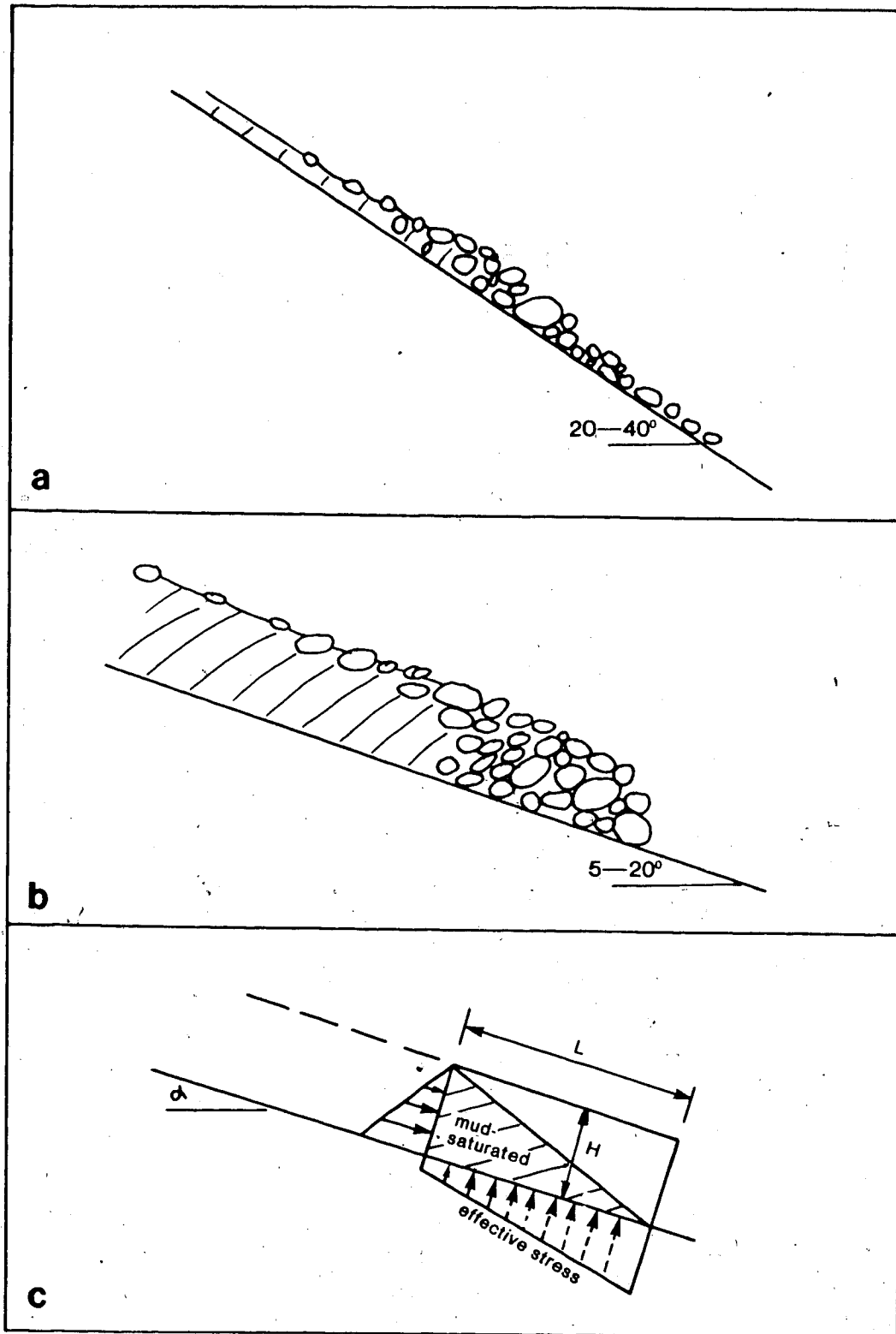
Figure 9.5 Frontal boulder accumulation in debris flow. (a) Steep slope, (b) flat slope, (c) schematic representation.
