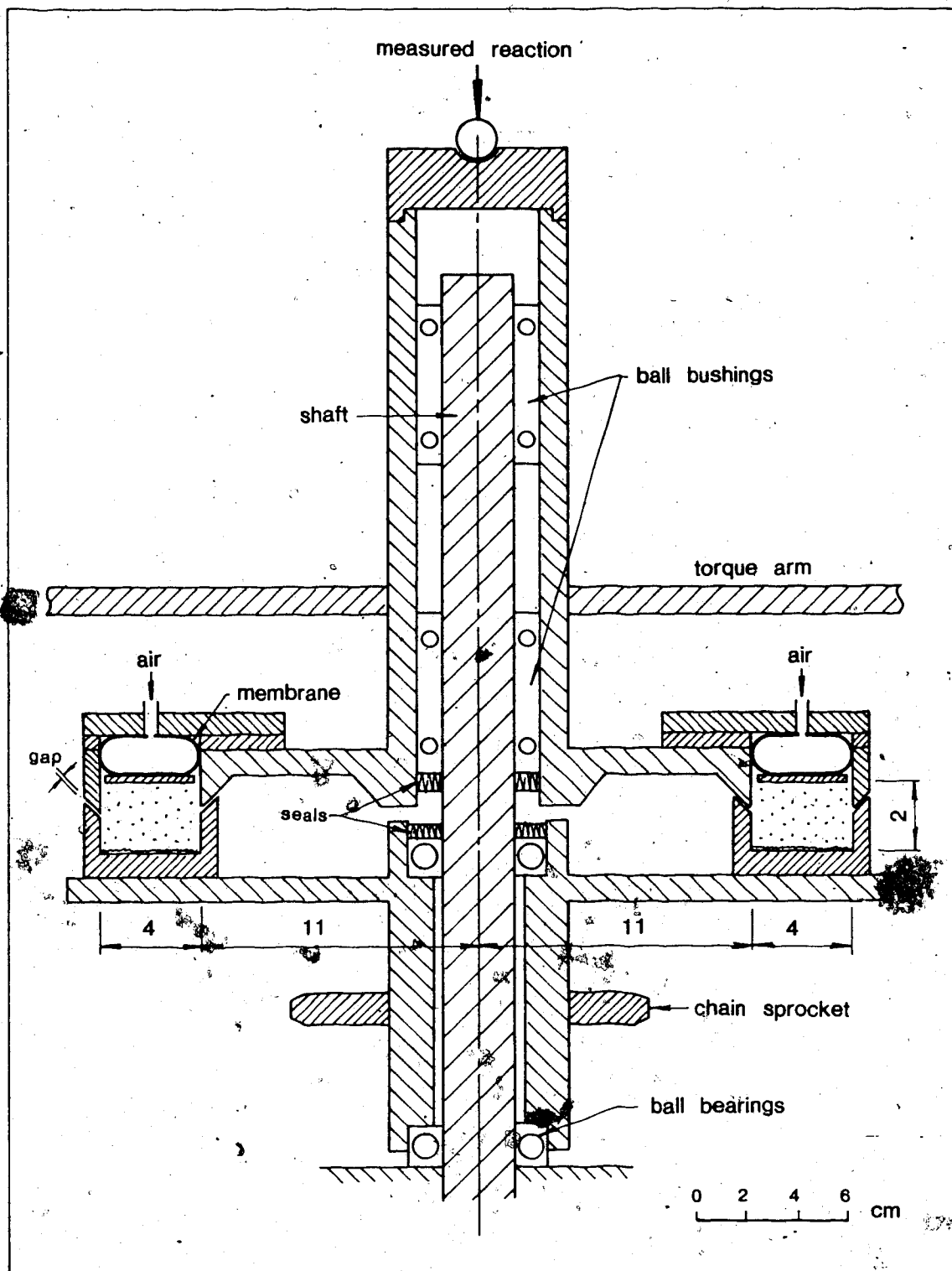
Figure 12.2 Vertical section of the ring shear boxes. Dimensions in cm. Lower box rotating, upper fixed.
