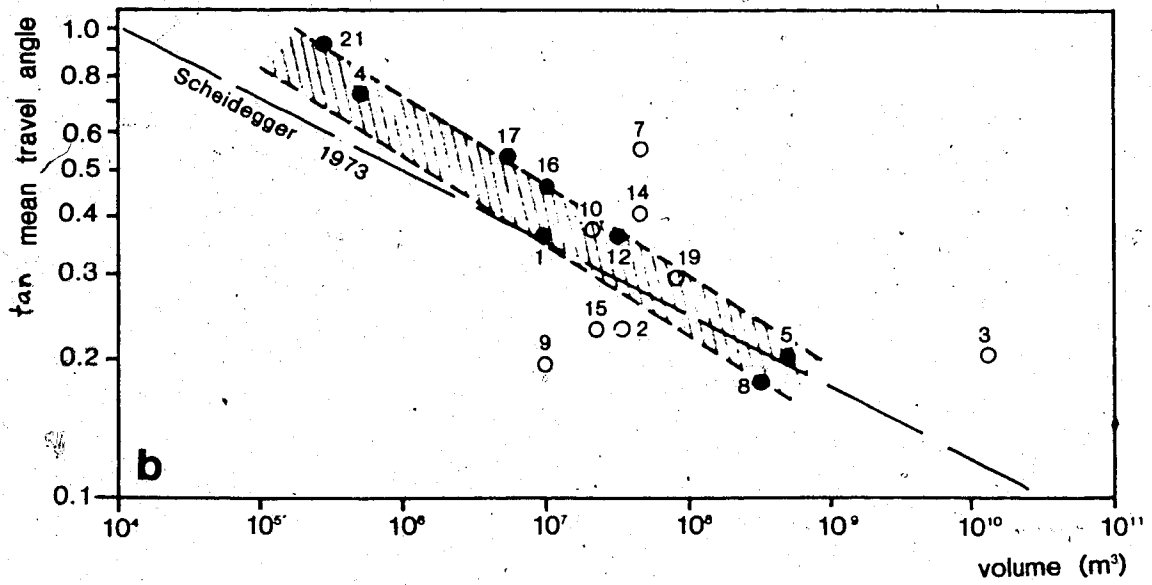
Figure 10.3 Correlations of (a) fahrboeschung (Scheidegger, 1973), and (b) mean travel angle with avalanche volume.
