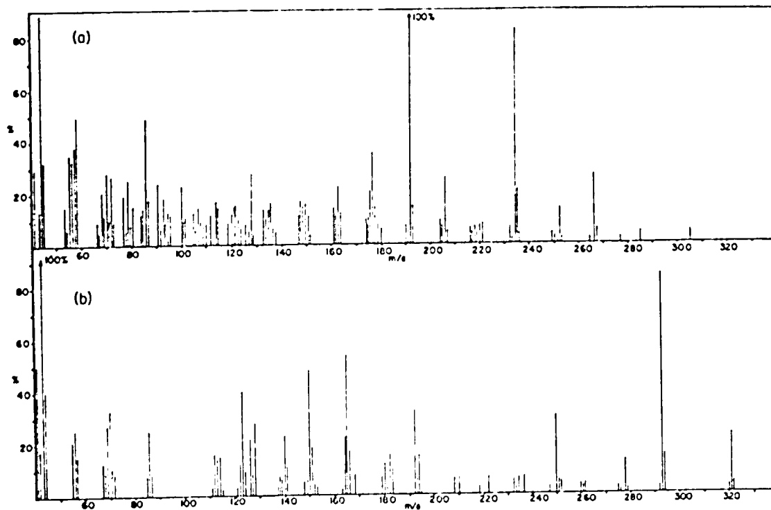
Figure 8 Mass spectrum of (a) N-acetylfawcettimine (b) N-acetylalopecuridine
