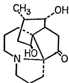
Serratinine 7
