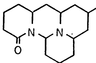
Cernuine 9
