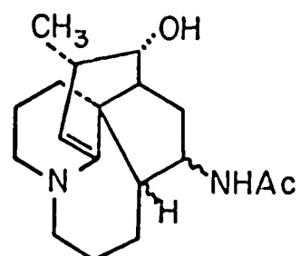
Serratinidine 8
