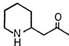
Pelletierine
