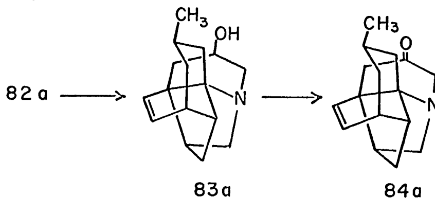
Hydrolysis of dehydroalopecurine (81a) with aqueous
