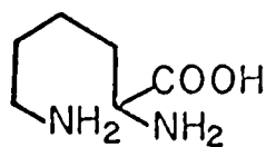
Lysine
