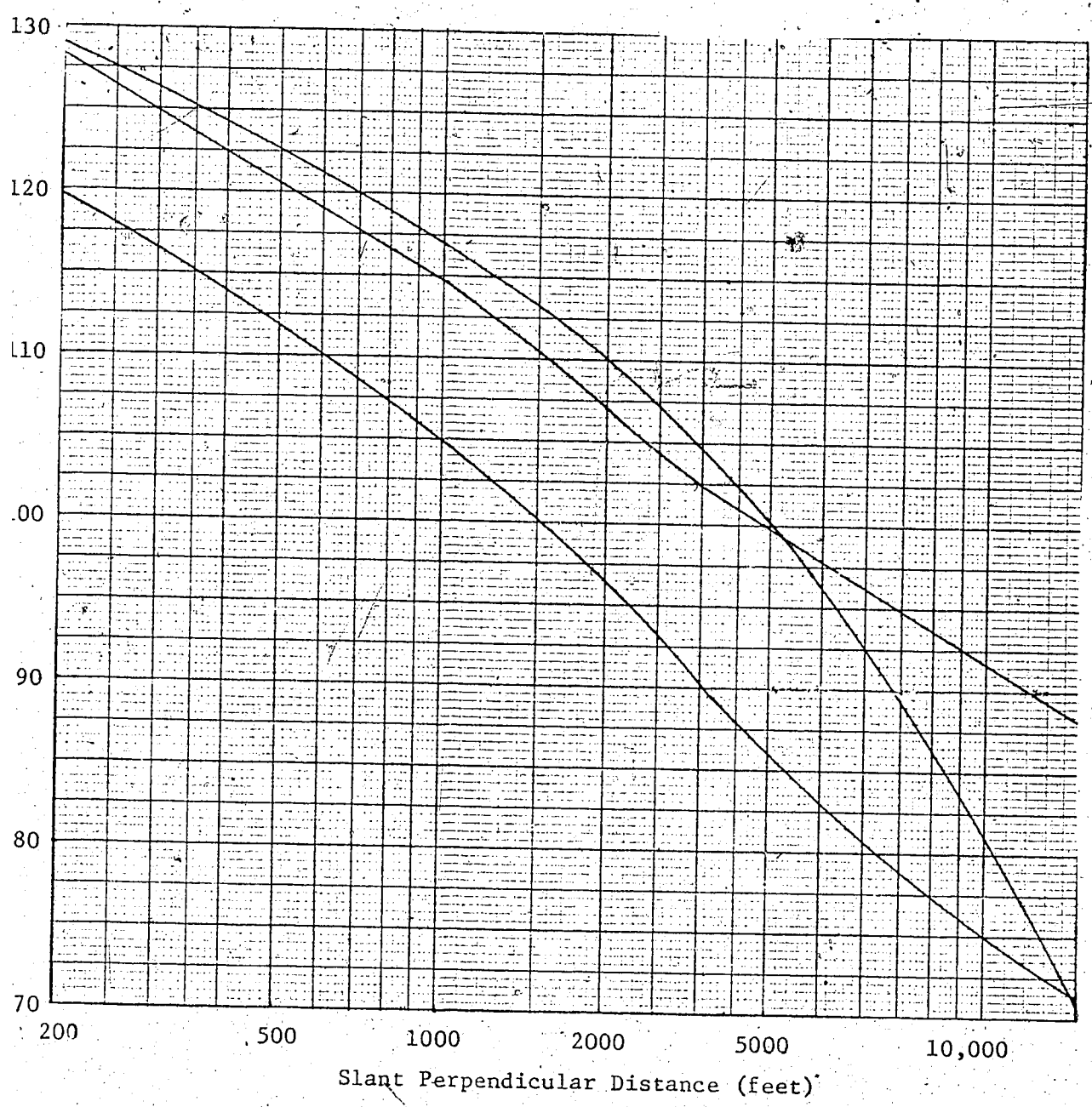
EPNdB VS. SLANT PERPENDICULAR DISTANCE (FOUR-ENGINE TURBOJET) (Source: CATA, CNR and NEF, p.22)
