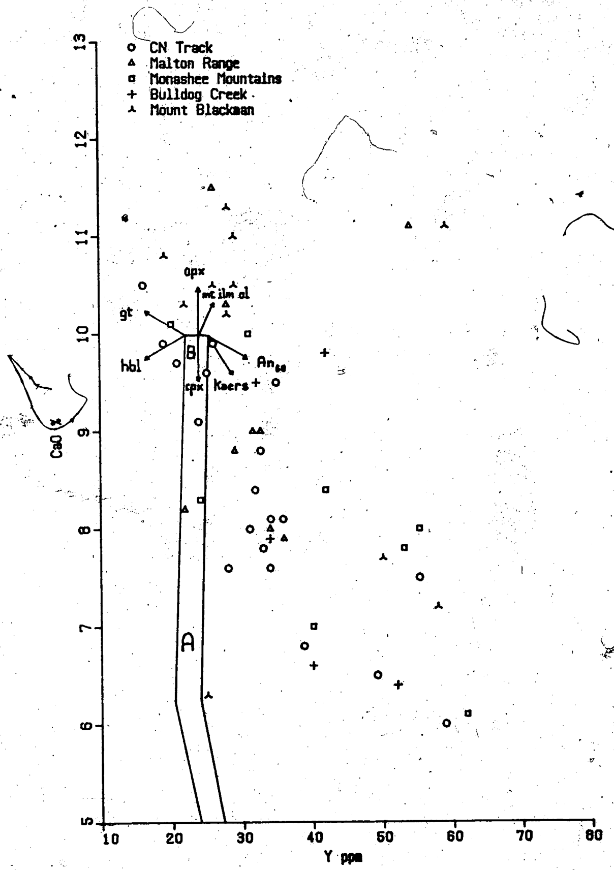
Figure 3.7 CaO v Y plot for the mafic gneisses of the Malton Gneiss Complex. BA shows Lambert and Holland's (1974) standard calc-alkaline trend. Arrows show the direction of liquid movement resulting from the crystallization of the minerals indicated.
