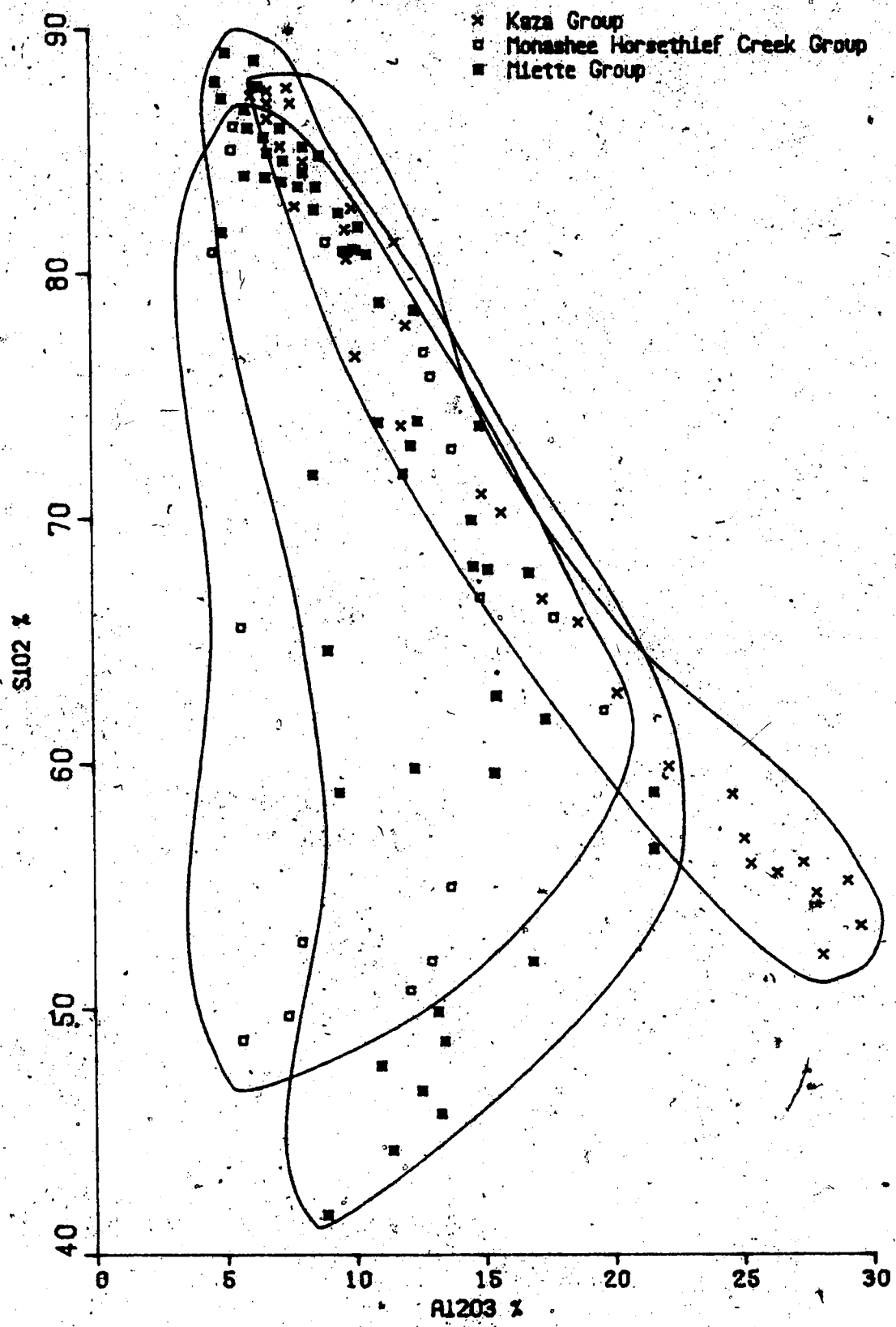
Figure 4.8 S102 v Al2O3 plot for metasediments from the Kaza, Mlette and Monashee Horseshief Creek Groups in the Valemount area
