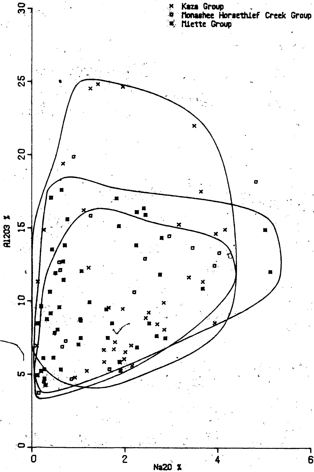
Figure 4.10 Al 2 O 3 v Na 2 O plot for metasediments from the Kaza, Mlette and Monashee Horseshief Creek Groups in the Valeport area
