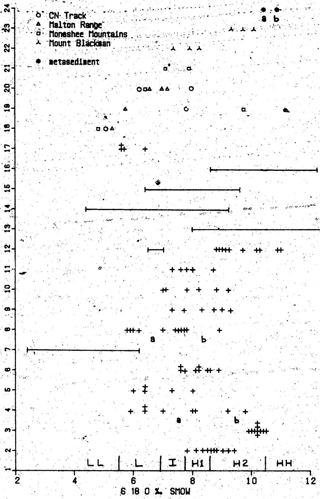
Figure 6.1 Oxygen isotopic compositions of whole rocks from the Malton Gneiss Complex compared with those from other Archean complexes and with those from the Berridale Batholith
