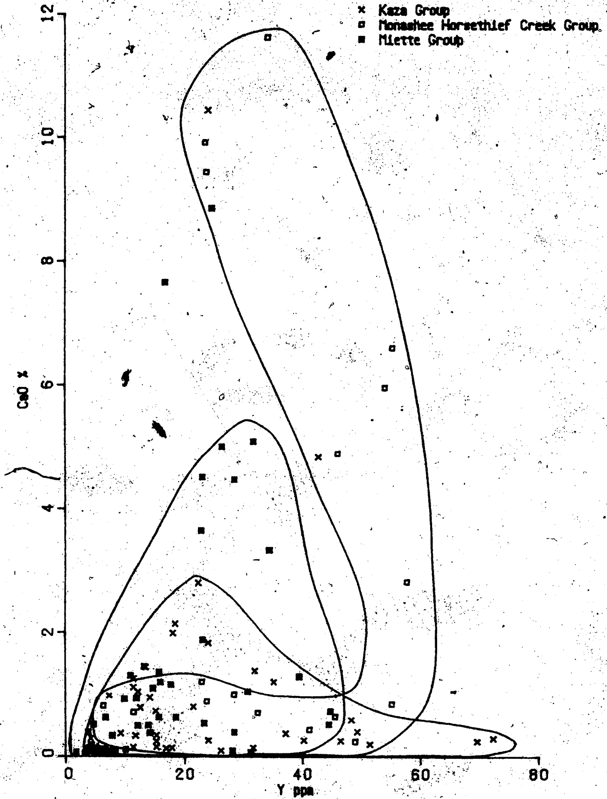
Figure 4.5 CaO v Y plot for metasediments from the Kaza, Milette and Monashee Horseshief Creek Groups in the Valenmount area
