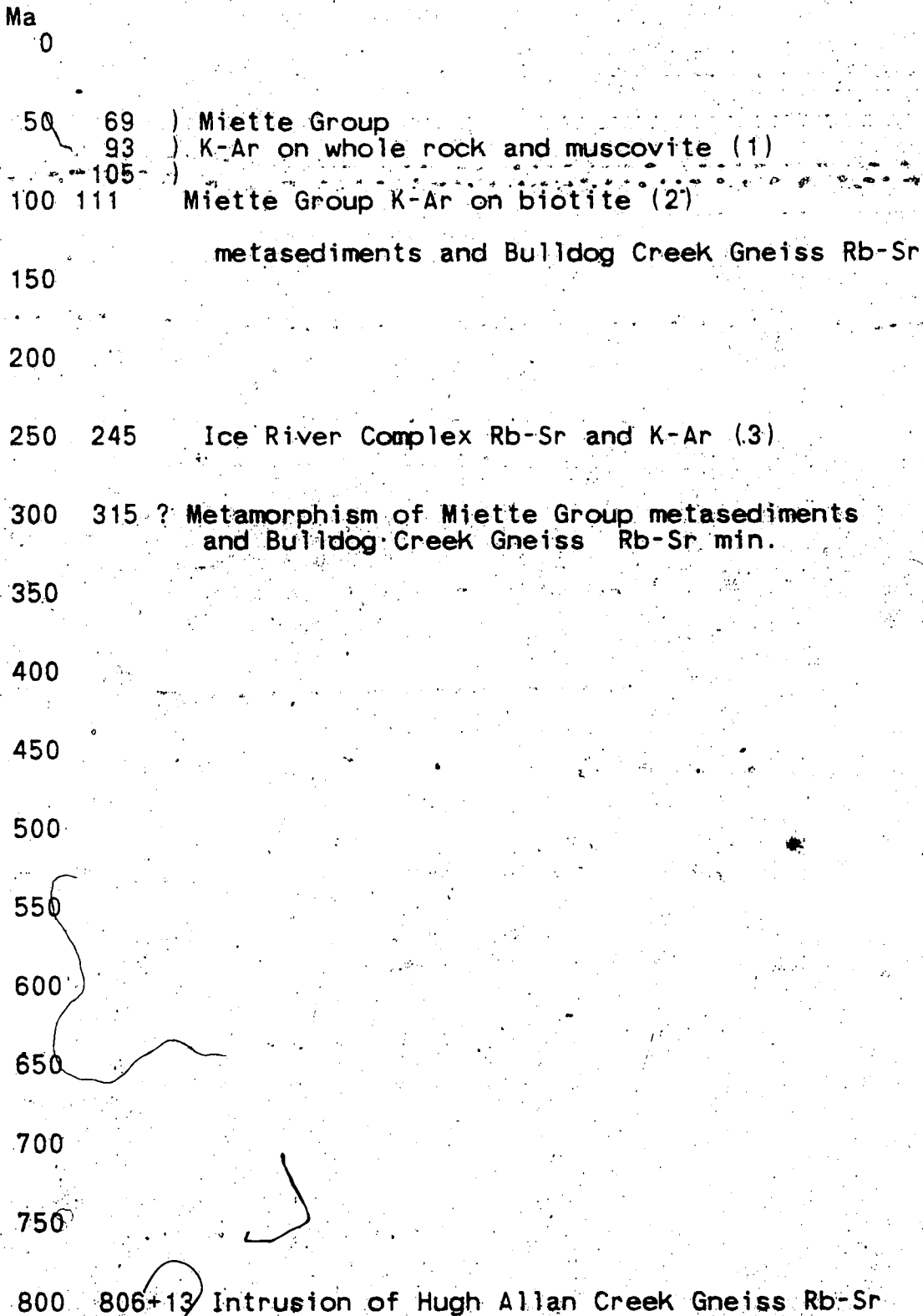
Figure 5.15 Age determinations east of The Rocky Mountain Trench
