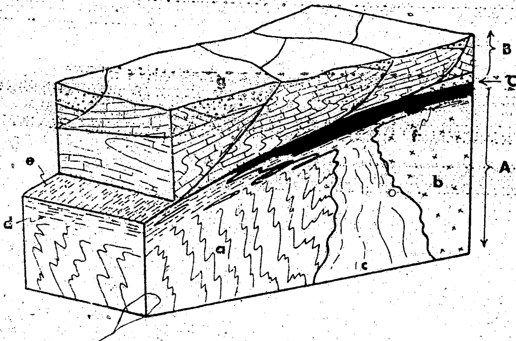
Figure 2. Schematic structural block diagram of typical domains of Cordilleran metamorphic core complexes; A, basement terrane; B, cover terrane; C, decollement zone; a, older metasedimentary rocks; b, older pluton; c, younger pluton (early to middle Tertiary); d, mylonitic foliation; e, mylonitic lineation; f, marble tectonite (black); g, lower to middle Tertiary sedimentary and volcanic rocks.
