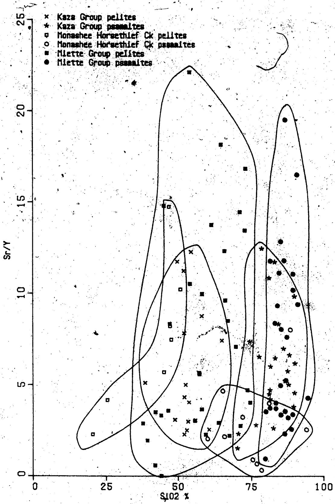
Figure 4.6 Sr/Y v SiO2 plot for pelites and psammites from the Kaza, Miette and Monashee Horsethief Creek Groups in the Valenmount area
