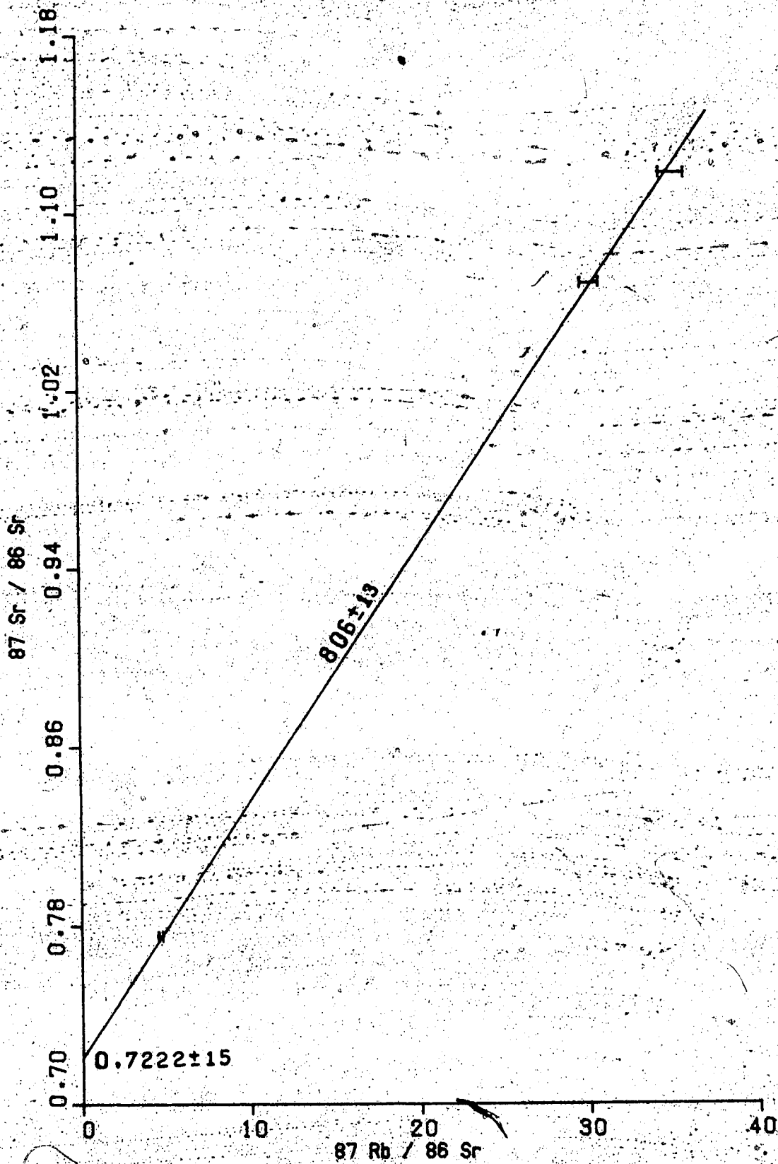
Figure 5.9 Rb-Sr isochron diagram for the High Allan Creek Gneiss of the Malton Gneiss Complex
