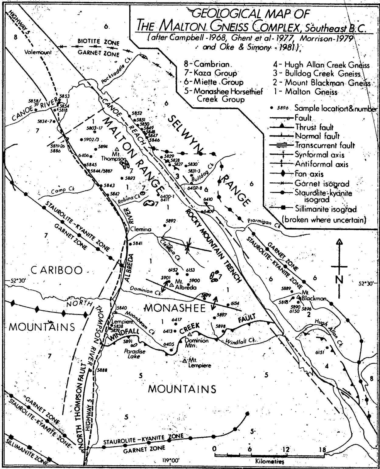
Figure 1.2 The Malton Gneiss Complex, after Campbell (1968), Ghent et al. (1977), Morrison (1979) and Oke and Simony (1981)
