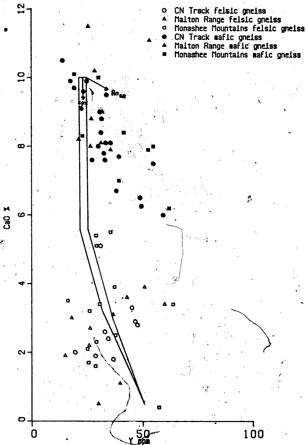
Figure 3.10 CaO v Y plot for the Grey Gneiss and the mafic gneisses of the Malton Block, showing Lambert and Holland's (1974) standard calc-alkaline trend.
