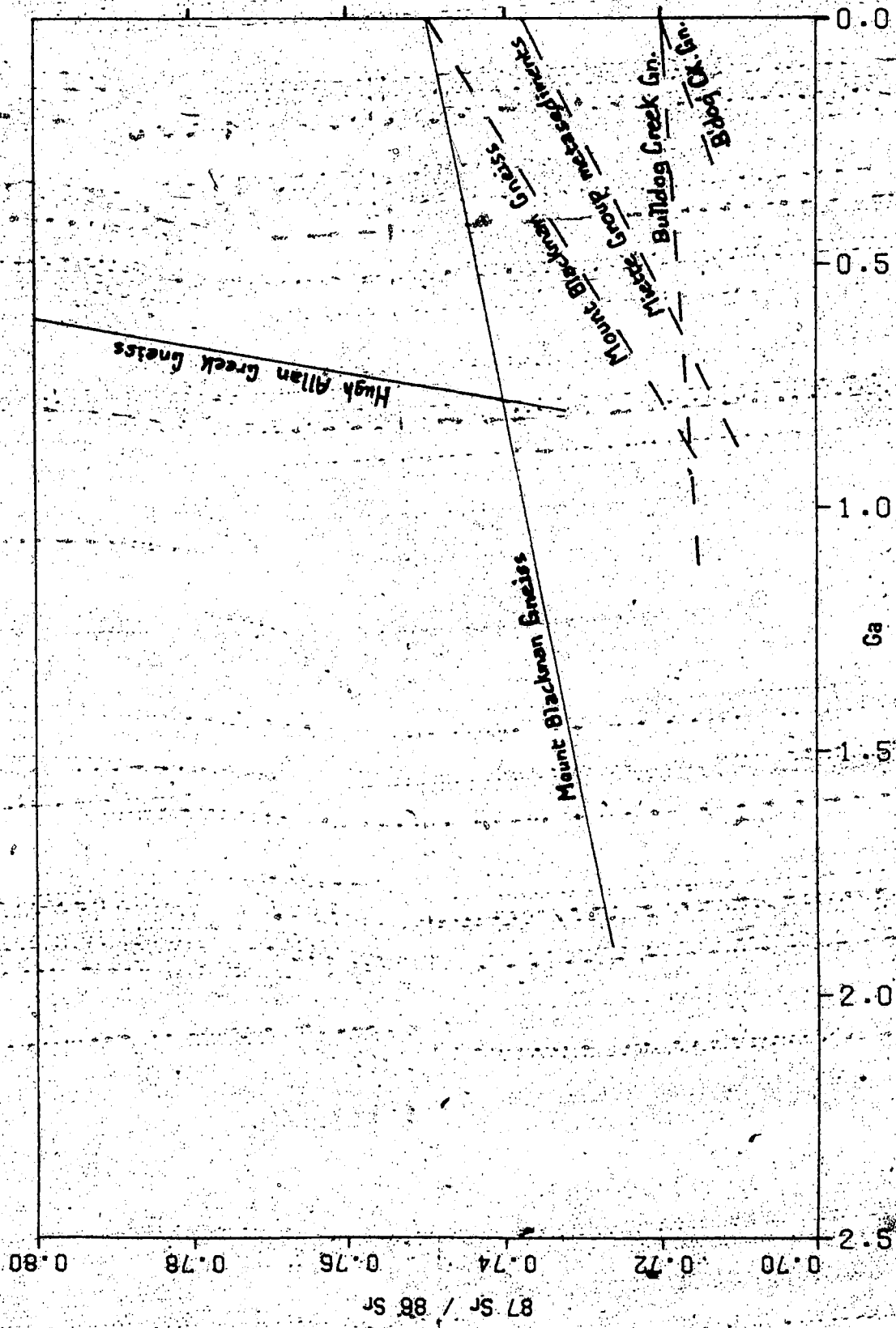
Figure 5.10 Strontium evolution diagram for rocks east of the Rocky Mountain Trench in the Valenmont area
