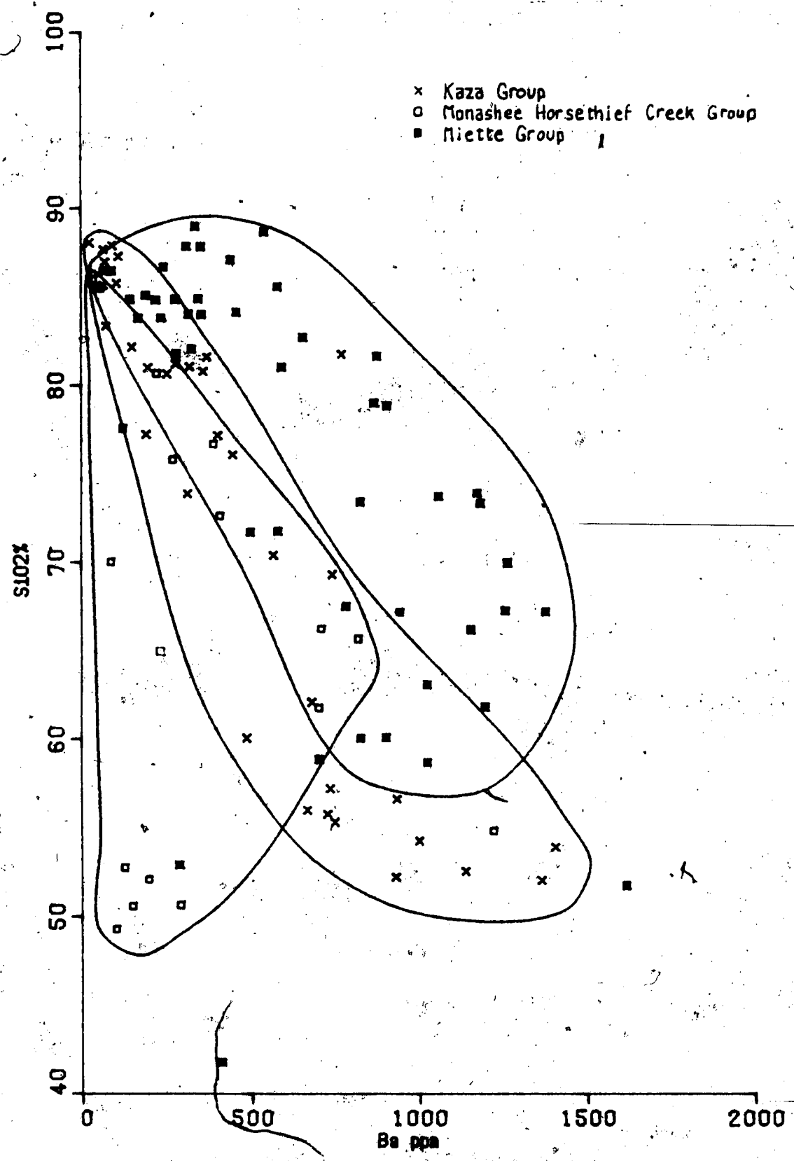
Figure 4.11 SiO 2 v Ba plot for metasediments from the Kaza, Miette and Monashee Horseshief Creek Groups in the Valemount area
