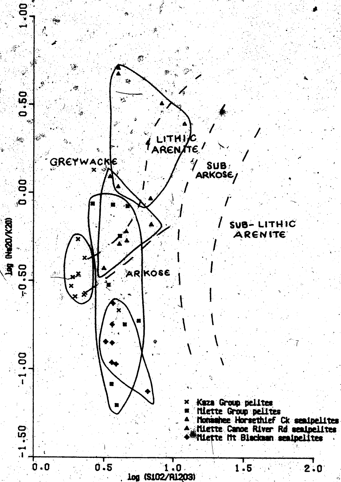
Figure 4.2. Classification (after Pettijohn et al., 1973) of the pelitic rocks from the Kaza, Mlette and Monashee Horsethief Creek Groups in the Valenmont area.
