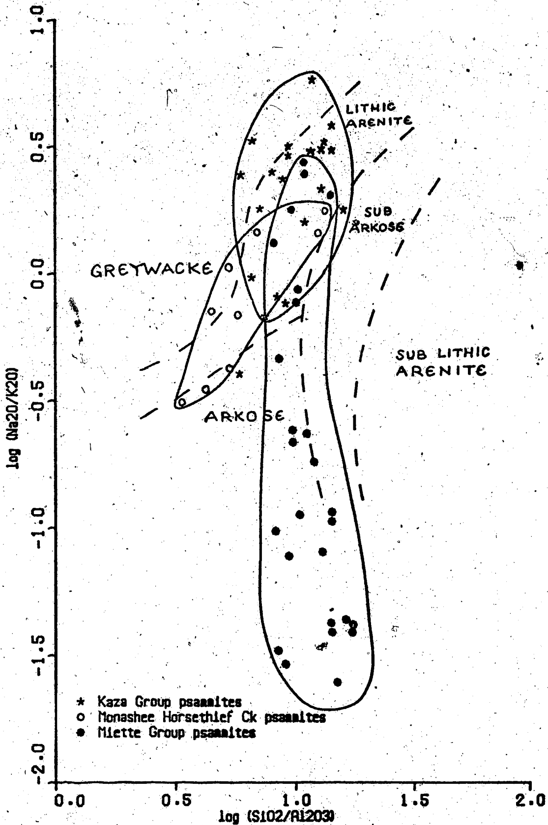
Figure 4.3 Classification (after Pettijohn et al., 1973) of the psammite rocks from the Kaza, Miette and Monashee Horsethief Creek Groups in the Valenmount area.
