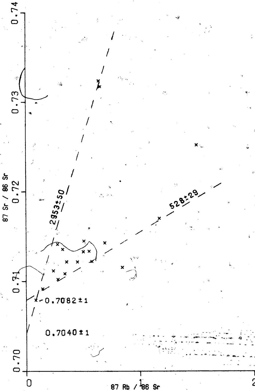
Figure 5.4 Rb-Sr isochron diagram for the mafic gneisses west of the Rocky Mountain Trench in the Malton Gneiss Complex. The diagram shows possible maximum and minimum ages for the mafic gneisses.
