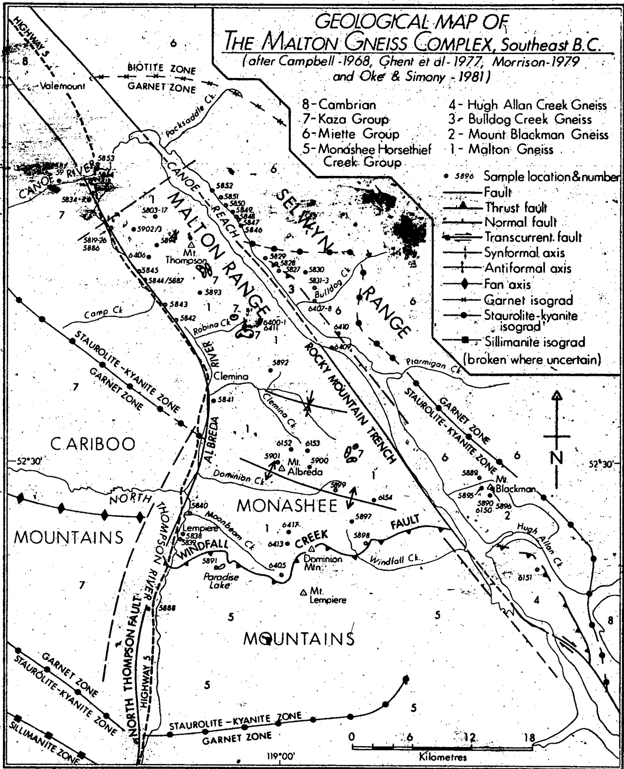
Figure 3.1 The Malton Gneiss Complex, after Campbell (1968), Ghent et al. (1977), Morrison (1979) and Oke and Simany (1981)
