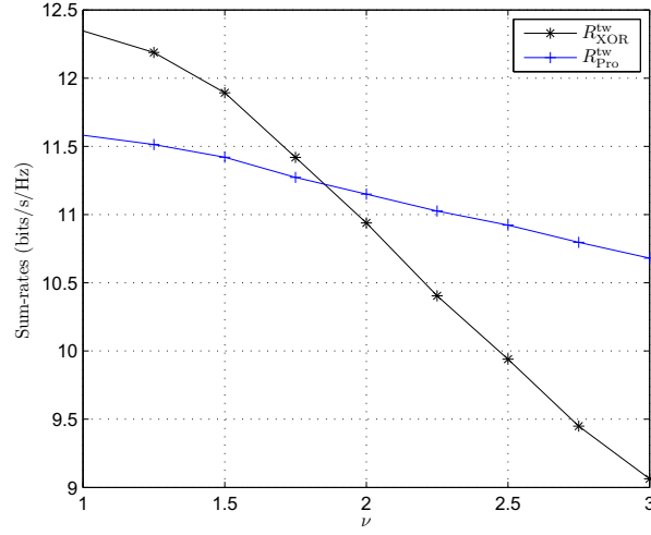
(a) Sum-rates vs. \nu , comparison of the XOR-based scheme of [83] (without considering power consumption minimization) and the proposed scheme averaged over 5000 channel realizations ( P_r^{\text{max}} = 3 ).
