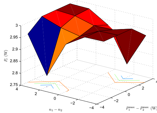
(b) Relay power consumption at optimality.
