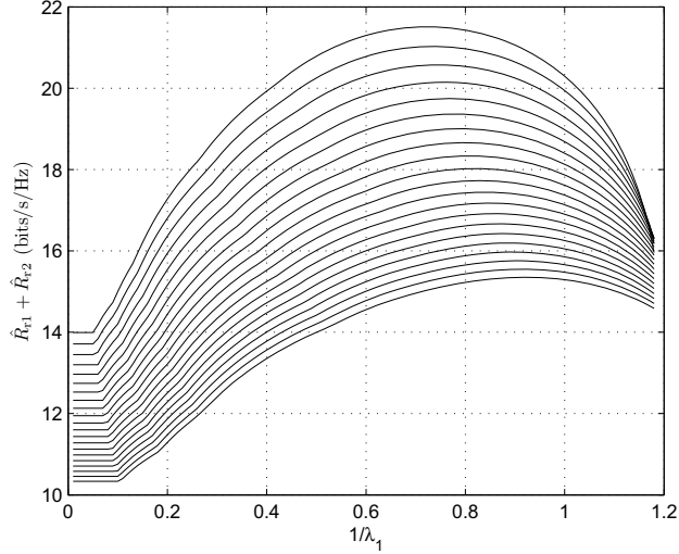
Figure 3.2: \hat{R}_{r1} + \hat{R}_{r2} versus 1/\lambda_1 under different P_r^{\max}/\sigma^2 .
