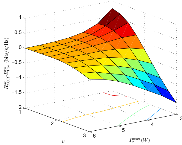
(b) Difference of sum-rates vs. P_r^{\text{max}} and \nu , comparison of the XOR-based scheme of [83] (without considering power consumption minimization) and the proposed scheme averaged over 5000 channel realizations.
