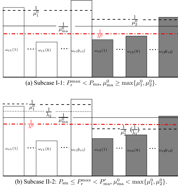
Figure 3.1: Illustration of \mu_1^0 , \mu_2^0 , \mu_{\text{ma}}^0 , and \lambda^0 for the scenario of relay optimization.
