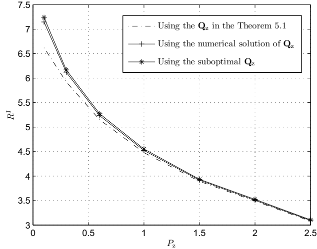
Figure 5.1: Comparison of R^J versus P_z with \mathbf{Q}'_z given by (5.15), the algorithm in Table 5.2, and (5.23), respectively.
