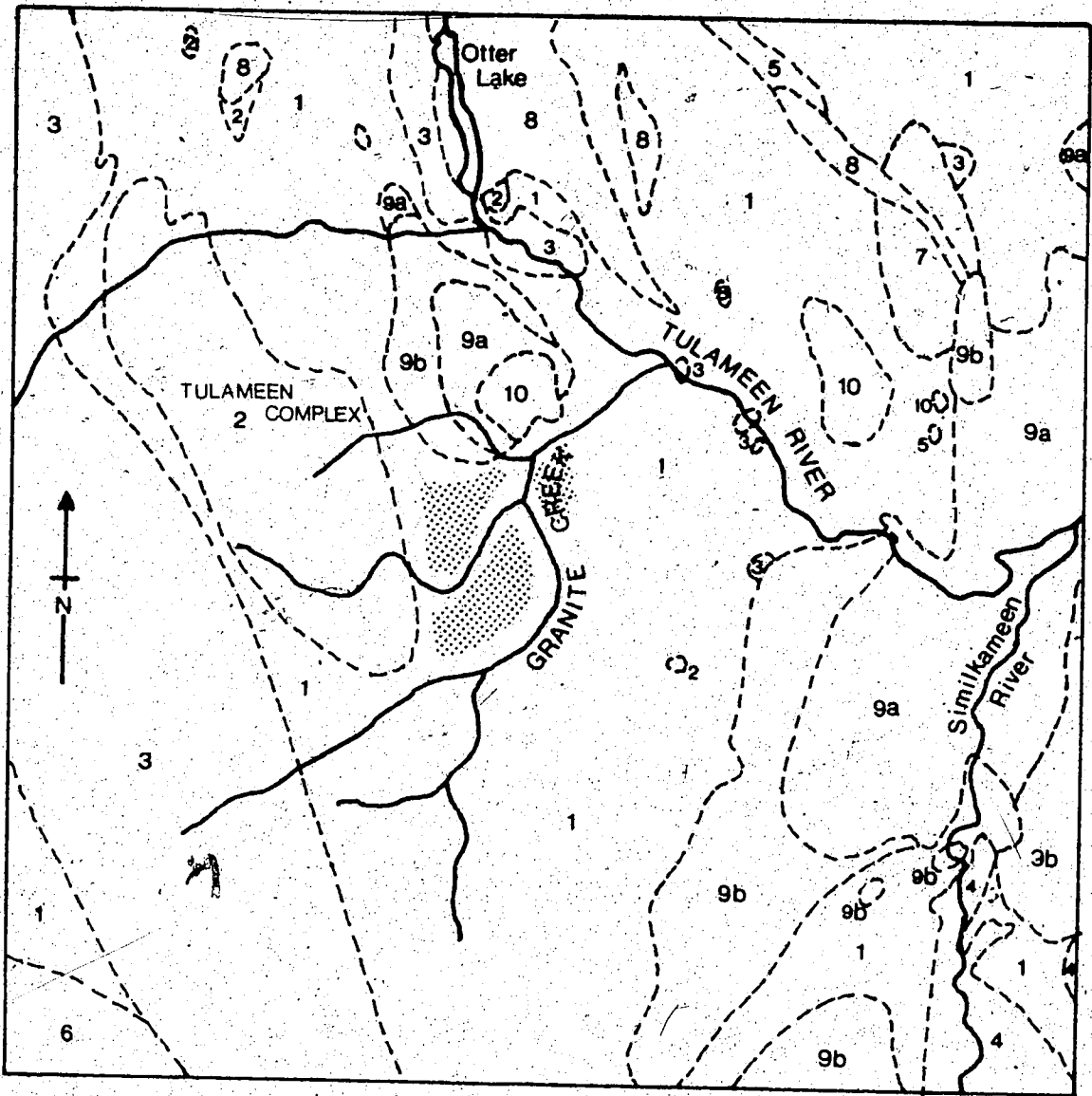
GEOLOGY OF THE GRANITE CREEK AREA (Adapted from Rice, 1947)
