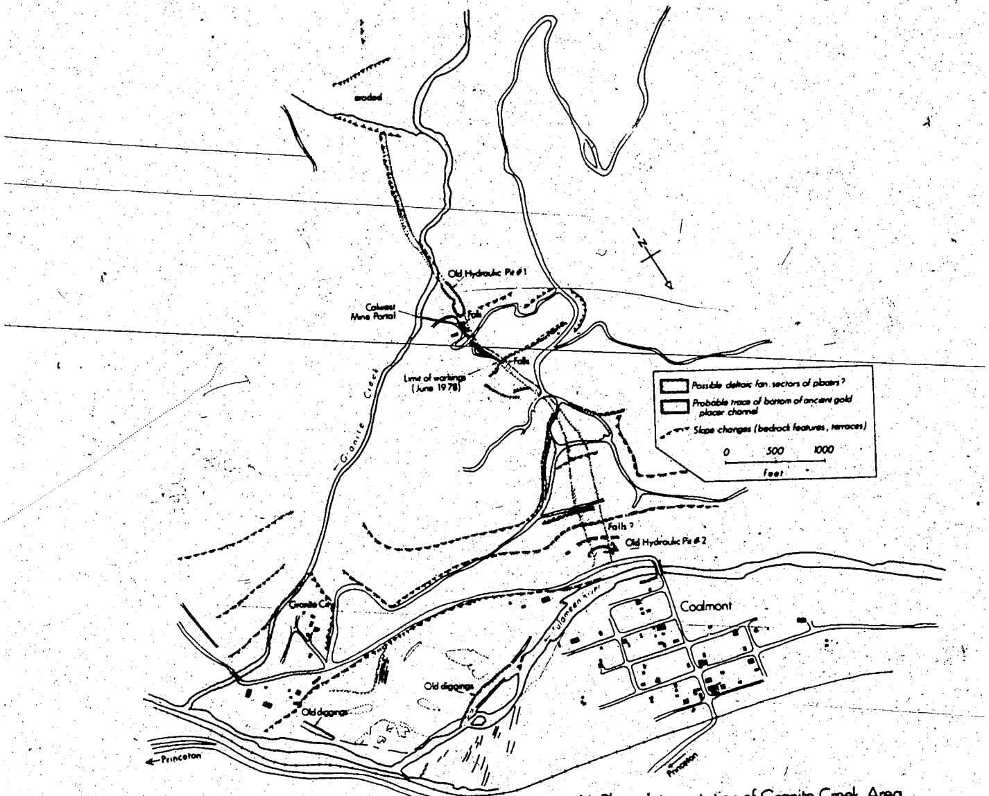
Air Photo Interpretation of Granite Creek Area showing location of buried placer channel
