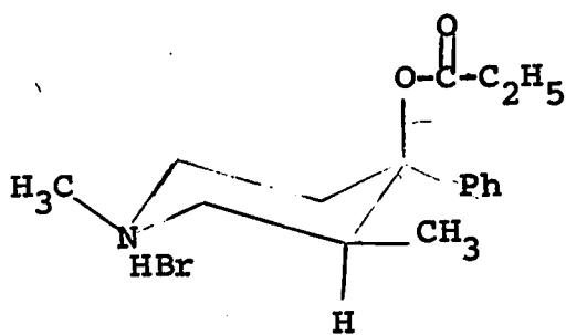
dl - \alpha - Prodine HBr
