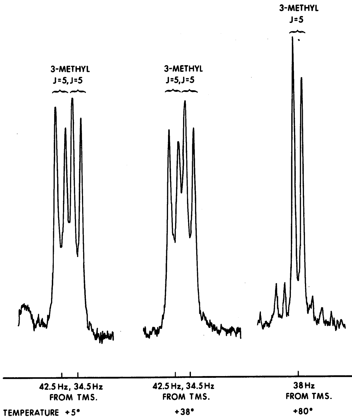
Fig. 3. Part of the PMR spectra of \alpha -( trans 3-Me/4-OH) 1, 3-dimethyl-4-hydroxyl-4-piperidinodiphenyl carbinol. Recorded on a Varian A-60 instrument in \text{CDCl}_3 at various temperatures.
