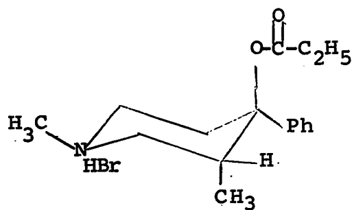
dl - \beta - Prodine HBr
