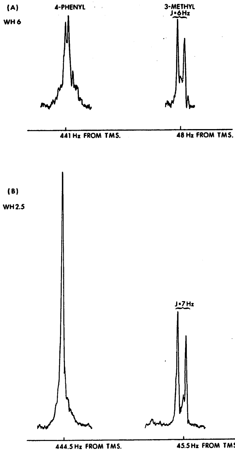
Fig. 1. Part of the PMR spectra of \alpha -1,3-dimethyl-4-phenyl-4-piperidinonitrile (A) and of the corresponding \beta -nitrile (B). Recorded on a Varian A-60 instrument in \text{CDCl}_3 .
