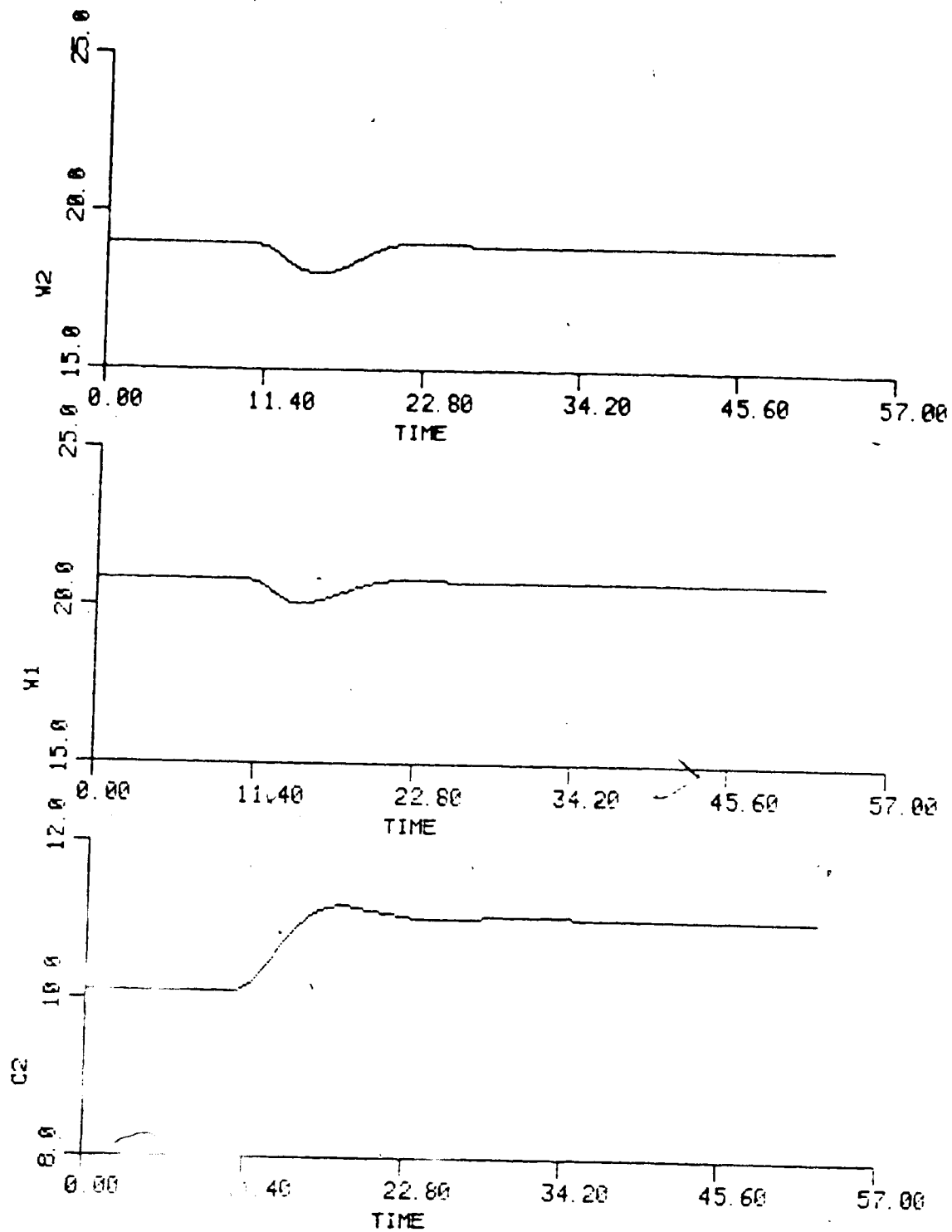
Figure 5.12 Simulated response of evaporator to a +10% change in product concentration. The fifth order discrete state space model and the compensator/controller of 5.3 were used.
