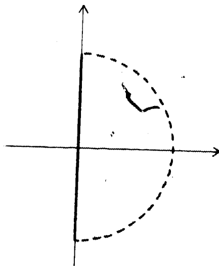
Figure 9.2 Nyquist D -contour in the s -plane
