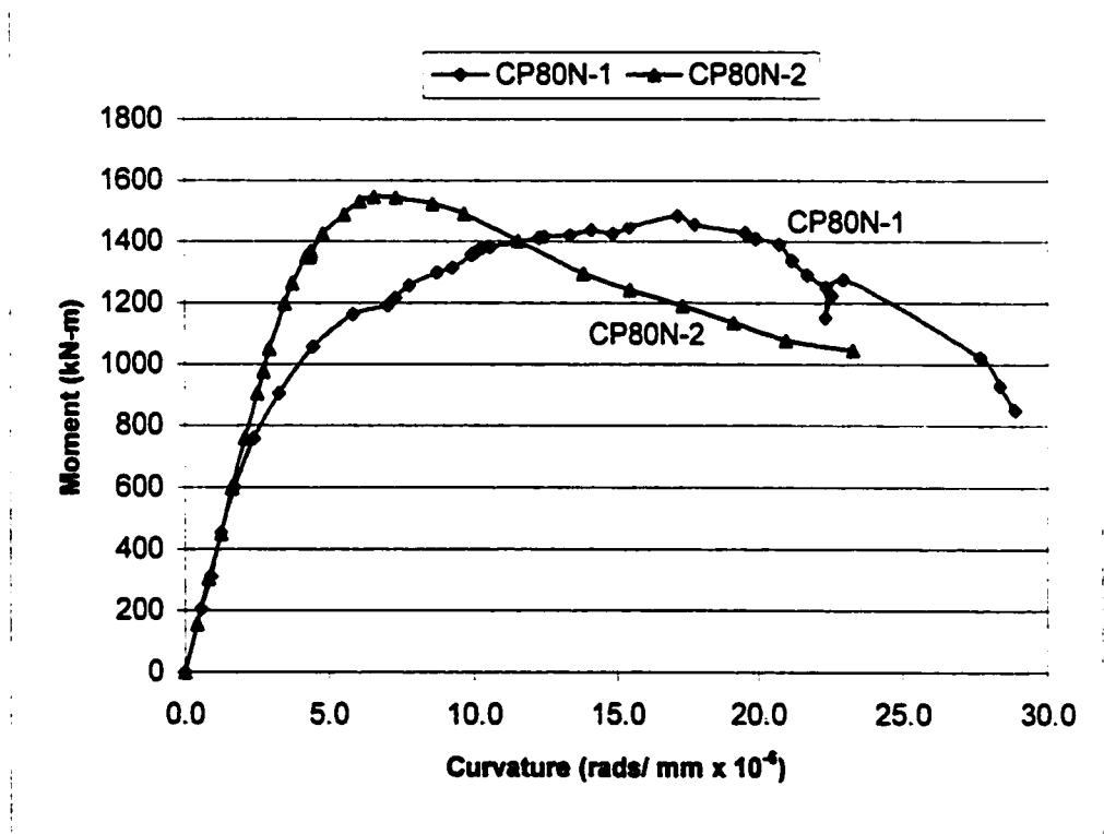
Figure 5.16 - Moment versus Curvature Plot for Tests by Dorey et al. (1999)
