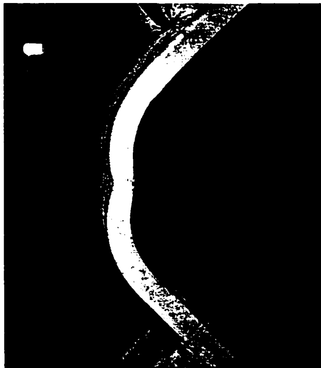
Figure 4.50 - Crest of Test Strip After Cyclic Loading
