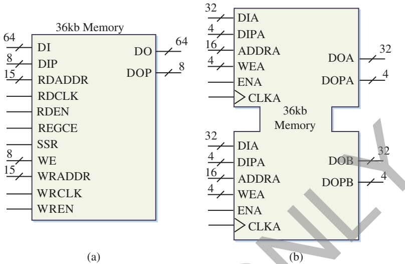
Figure 1.3 Virtex®-7 series FPGA block memory: (a) simple dual-port RAM and (b) true dual-port RAM.
