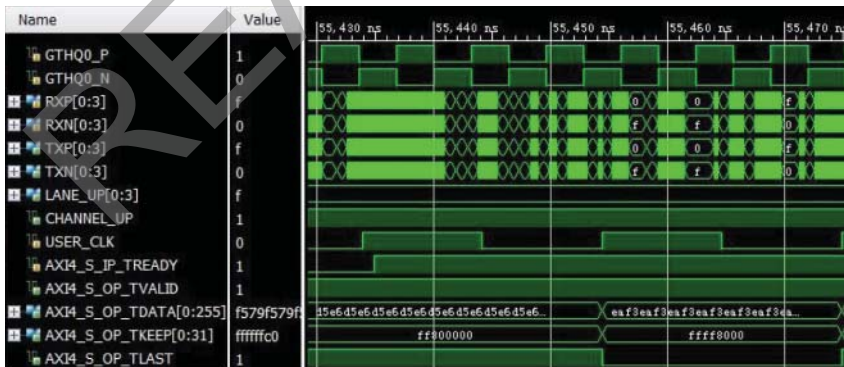
Figure 1.6 Communication process: (a) block diagram and (b) digital signal waveforms. Source: Xilinx, Inc.
