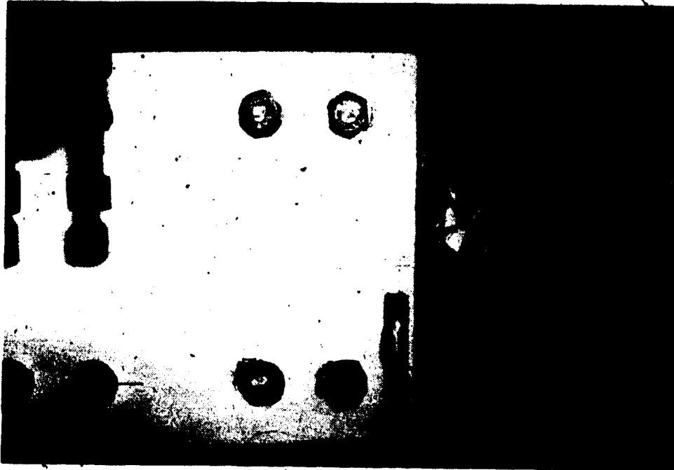
Figure 5.8 Local Splice Plate Yielding
