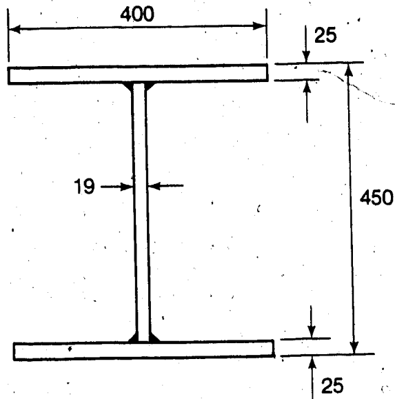
Figure 4.3 Large Scale Test Beam Cross-Section
