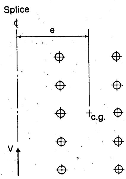
Figure 3.2 Eccentrically Loaded Web Splice Bolt Group
