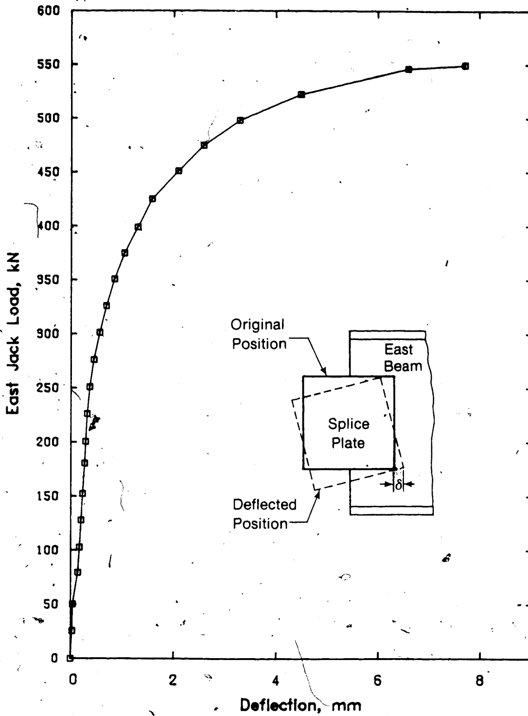
Figure 5.9 Typical Load Versus Splice Plate Deflection Response
