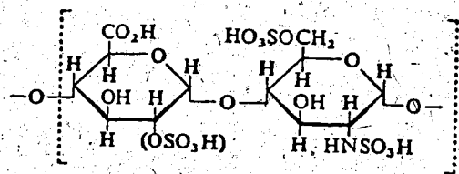
Fig. 2 The Repeating Disaccharide Structure of the Glycosaminoglycans
