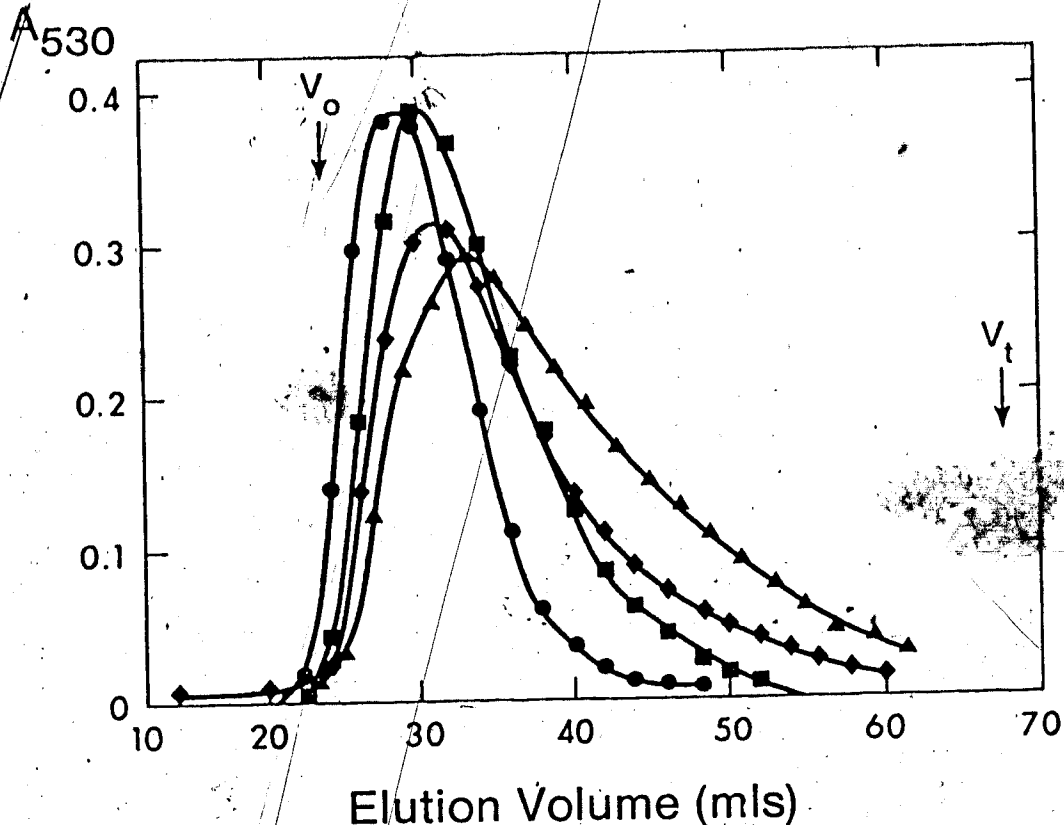
Fig. 13 Effect of pH on the Periodate Oxidation and Alkaline Elimination of Chondroitin Sulphate
