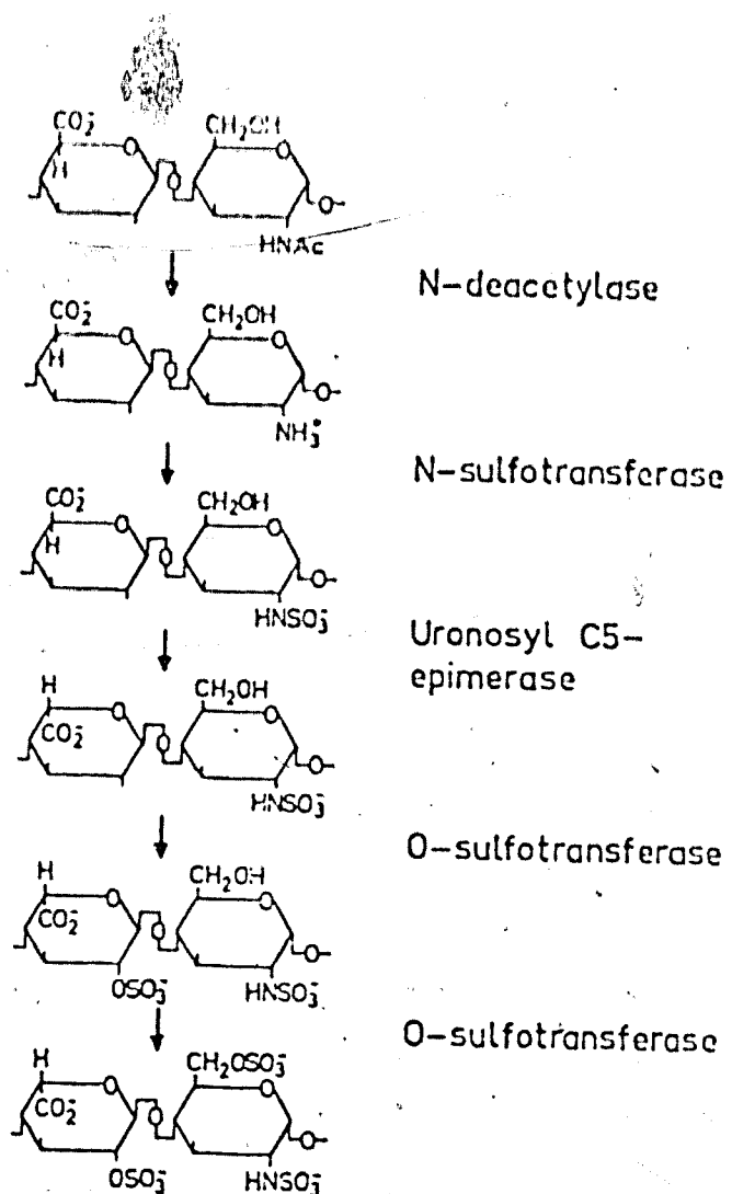
Fig. 3 The Sequence of Polymer Modification Reactions Leading to Formation of the Predominant Disaccharide Unit in Heparin.
