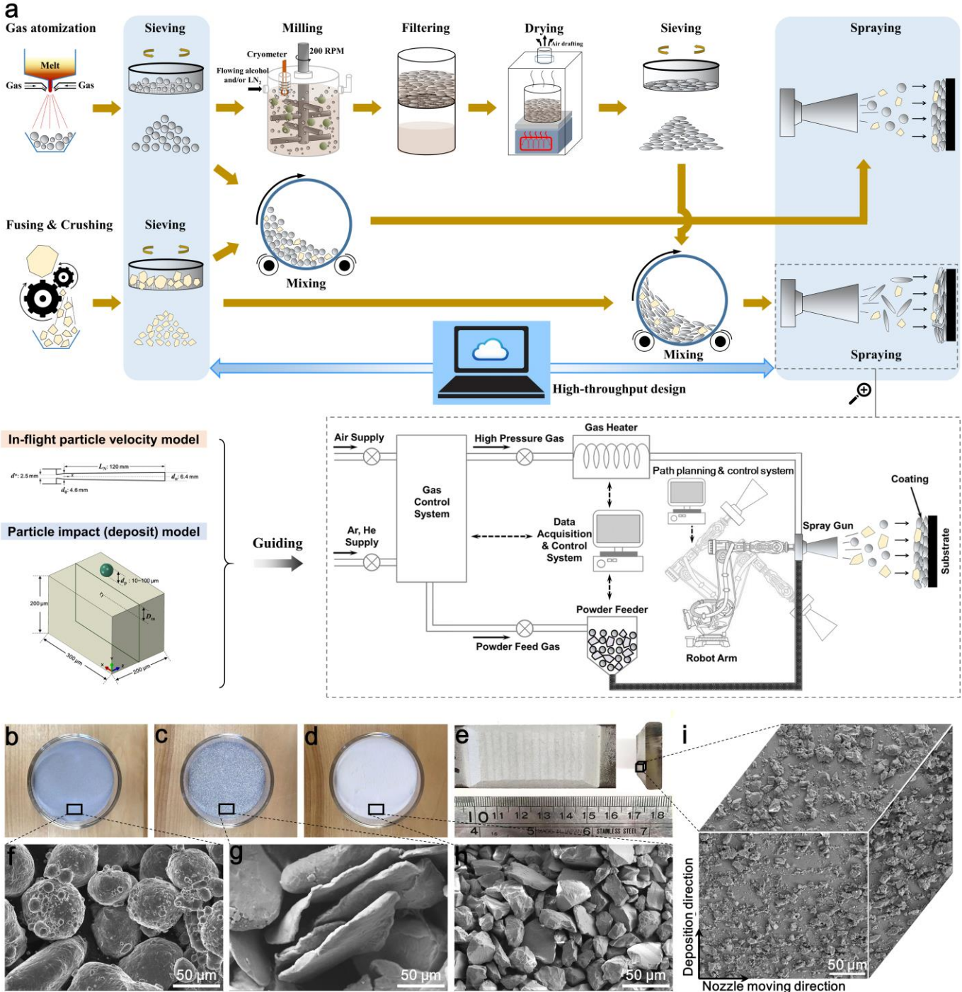
Fig. 2. Material and preparation. (a) Schematic illustration of the fabrication process for nanocrystalline Al-Al 2 O 3 composites pursued in this study. (b-i) Macroscopic and microscopic observations of powders used in cold spray composite deposition. (b,f) Spherical Al powder before milling; (c,g) Al powder after milling in the liquid nitrogen environment; (d,h) irregularly shaped Al 2 O 3 powder; (e,i) a typical Al-Al 2 O 3 composite
