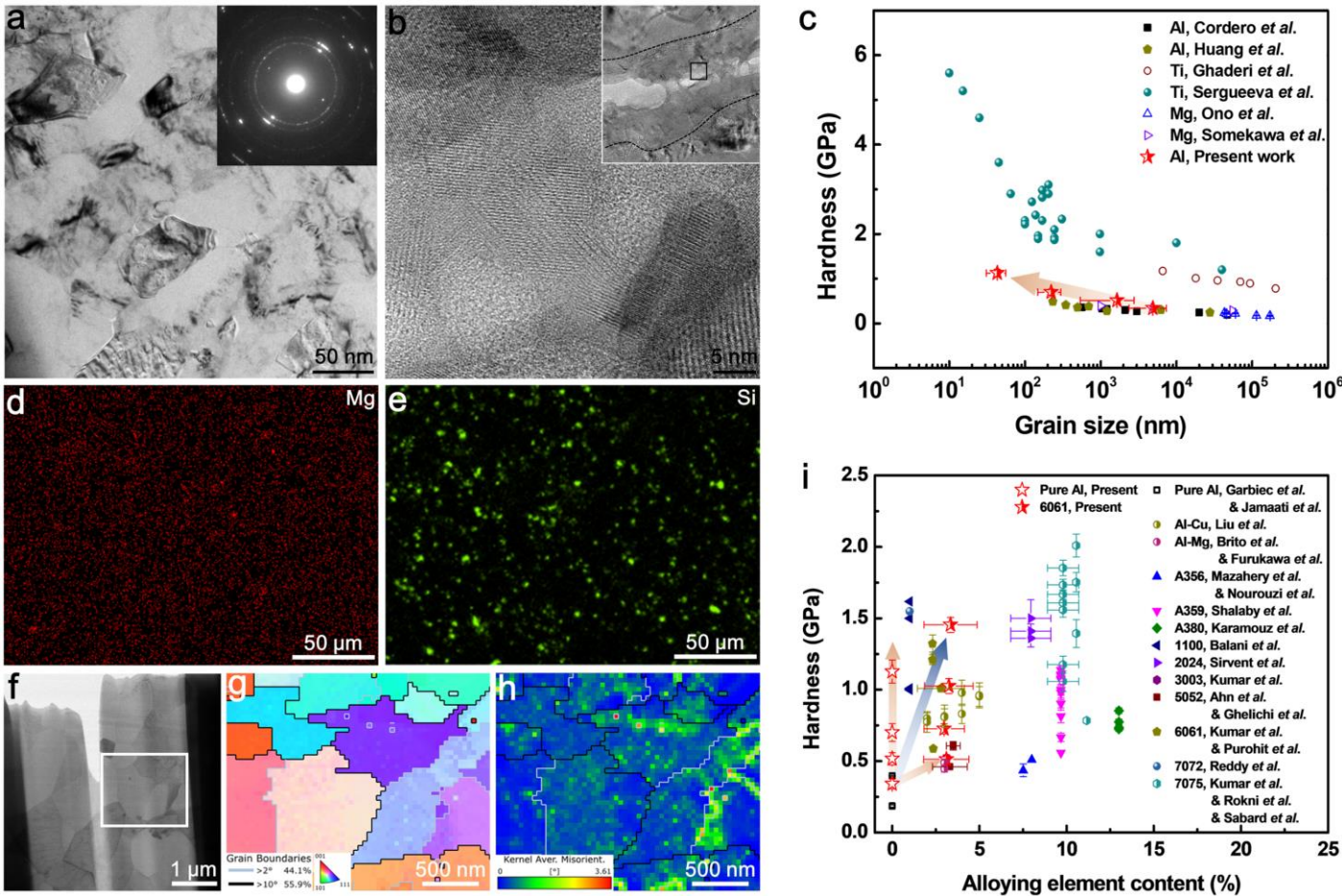
Fig. 3. (a-c) Grain refinement (to nanoscale) via low-temperature milling and cold spraying processes. (a) Typical TEM image showing nanosized grains in a deposited Al. Inset shows a corresponding selected area electron diffraction (SAED) pattern. (b) High-resolution TEM image of the nanostructure at powder/powder boundary of the as-prepared Al. Inset is the corresponding lower magnification image with the boundary zone outlined by black dashed lines and the magnified area marked by a black box. (c) Correlation of grain size and hardness for the present cold sprayed Al deposits and other light metals from the literature. The closed points indicate hardness measured by hardness tests while the open points indicate yield strengths that were multiplied by a Tabor factor of 3 by compression or tension tests. (d-i) Solid solution atom and precipitate coupling with grain size. (d,e) Elemental mappings of Mg and Si, (f) TEM image showing the microstructure of the alloy matrix, (g,h) corresponding inverse pole figures (IPF) and Kernel Average Misorientation (KAM) mappings characterizing the crystalline orientation in the white box of ‘c’, showing microstructure in cold sprayed Al 6061 using the powders milled at room temperature. (i) Correlation of alloying element content and hardness for the present cold sprayed Al and Al 6061, as well as other Al
