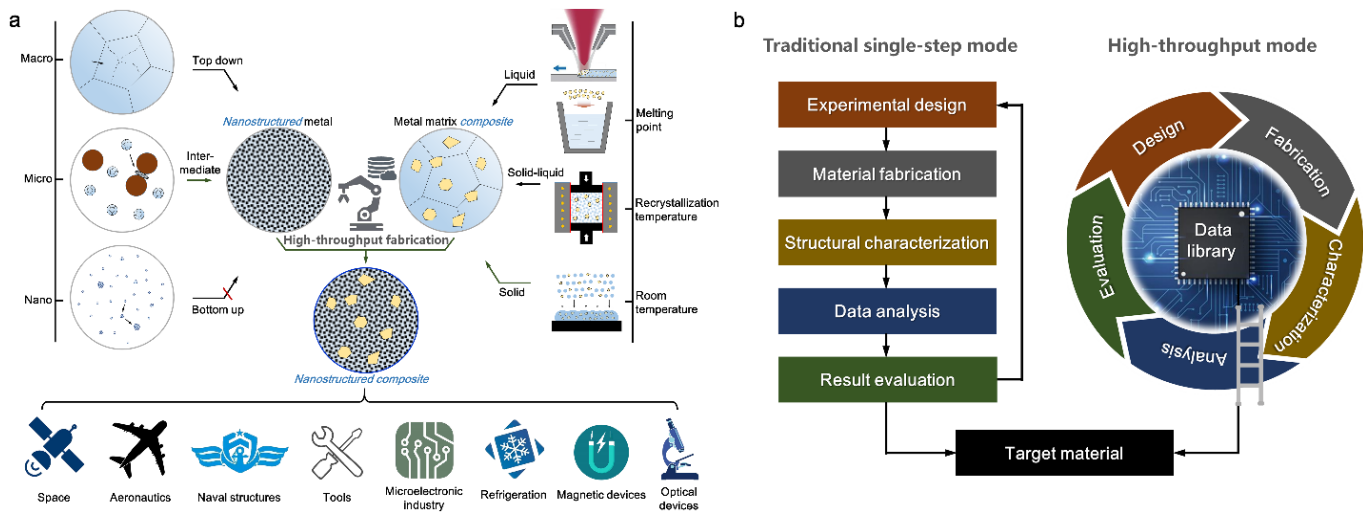
Fig. 1. Overview of synthetic approaches and applications of nanostructured metal matrix composites emphasized on the high-throughput design. (a) Base metal nanocrystallization includes top-down breaking the grains down in bulk material, bottom-up building the solid up from atomic scale units or nanoclusters, and reducing the structures in micron-scale (intermediate) particles before building them up. Metal matrix composites prepared by three (liquid, solid-liquid, and solid) approaches based on the state of matrix metal during forming process, including laser cladding/additive manufacturing, casting/impregnating, powder metallurgy, and depositing. Nanostructured composites show potentially structural and functional applications. (b) Comparison of two routes of new material development.
