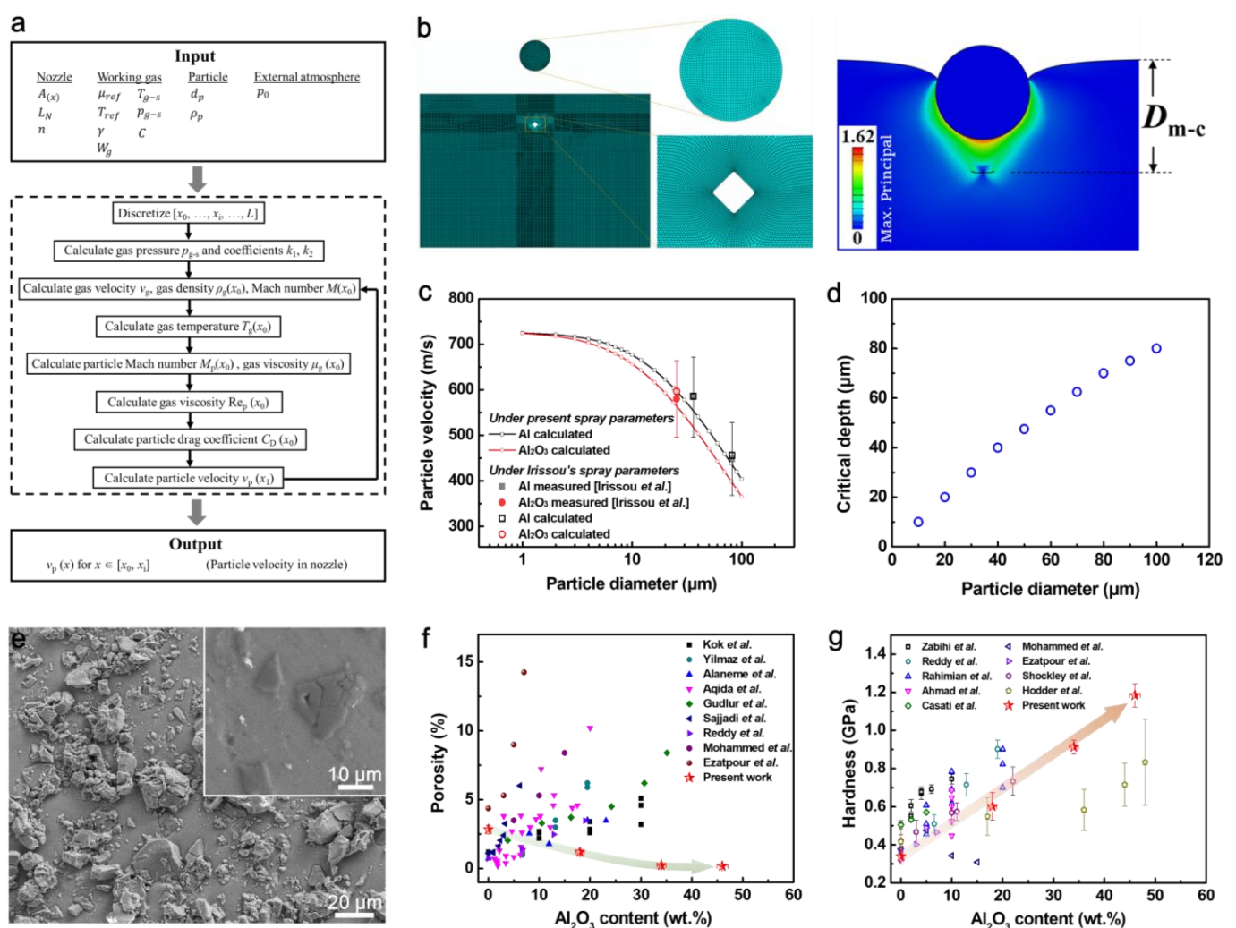
Fig. 4. Porefree high-strength AMCs fabrication guided by numerical simulations. (a-d) Numerical approach for selecting optimized powder sizes for cold spray: (a) Model flowchart for in-flight particle velocity evolution during cold spraying, (b) finite element methods (FEM) simulation on spraying with impact of Al 2 O 3 particle onto the Al matrix, (c) relationship between in-flight powder velocity and size after acceleration in the spray nozzle, (d) relationship between critical depth of embedded pore and Al 2 O 3 particle size in the impact process. (e) Typical morphology of present Al-46% Al 2 O 3 composite, showing minimal porosity
