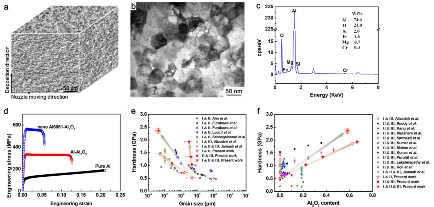
Fig. 5. Multi-level strengthening in present nanocrystalline Al 6061-Al 2 O 3 composite. (a-c) Microstructural information of the present composite designed by the synergistic strengthening strategy: (a) Three-dimensional microstructure under SEM; (b) TEM image showing nanograin matrix; (c) the characteristic elemental x-ray energy peaks detected in the area containing Al matrix and Al 2 O 3 particles. (d) Compression of stress-strain curves (in Y direction) of Al, Al-Al 2 O 3 , and nano Al 6061-Al 2 O 3 under compression. (e) Hardness of the present composites compared with other Al(-Al 2 O 3 ) materials from the literature designed by two or three strengthening strategies: Hardness versus grain size in matrix, (f) hardness versus Al 2 O 3 particle content relationship for different strengthening strategies compared with those from the literature. (Please trace the hardness data through Data Source Section of Supplementary Information)
