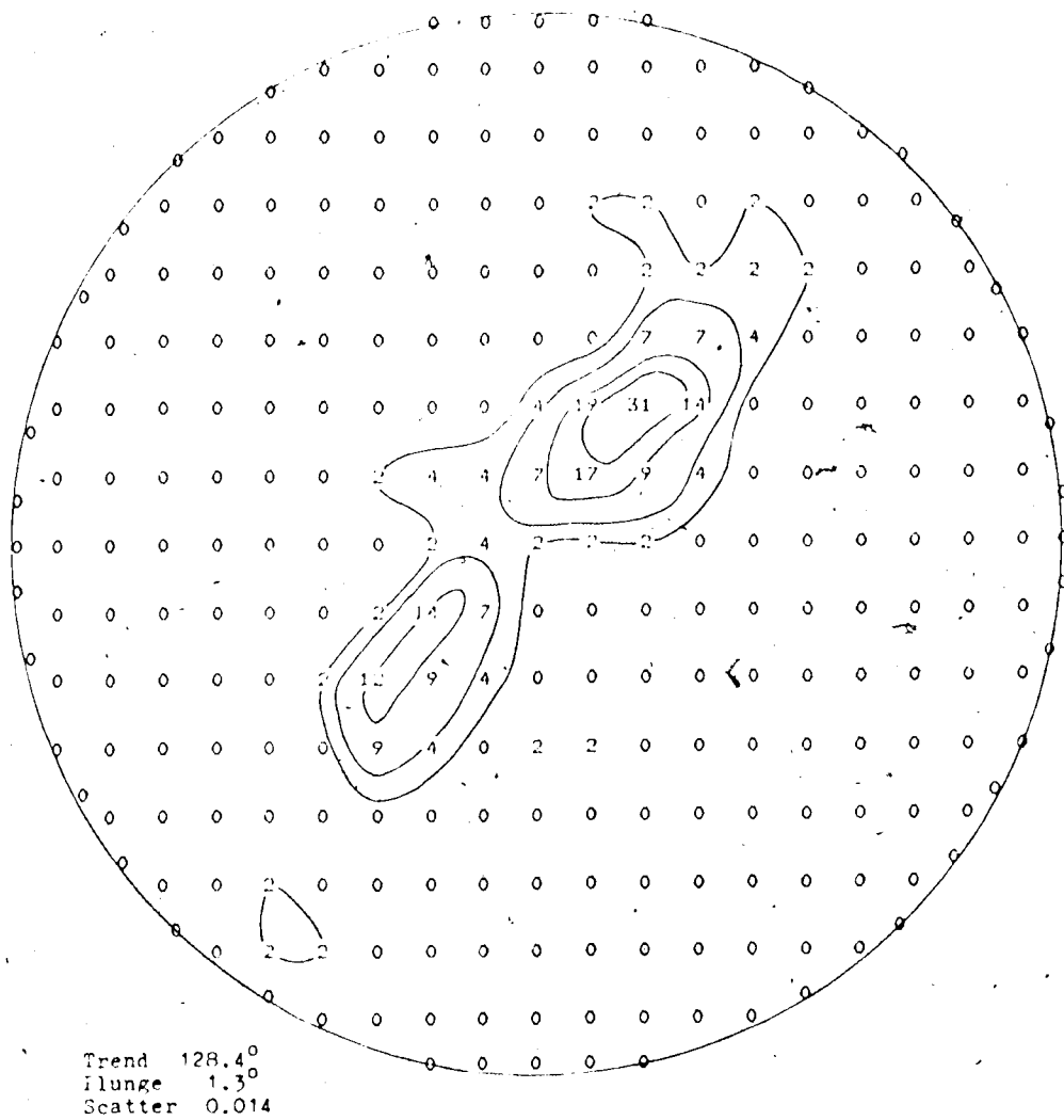
Figure Computer generated pi-diagram of outcrop bedding orientations northwest of line 60+00.
