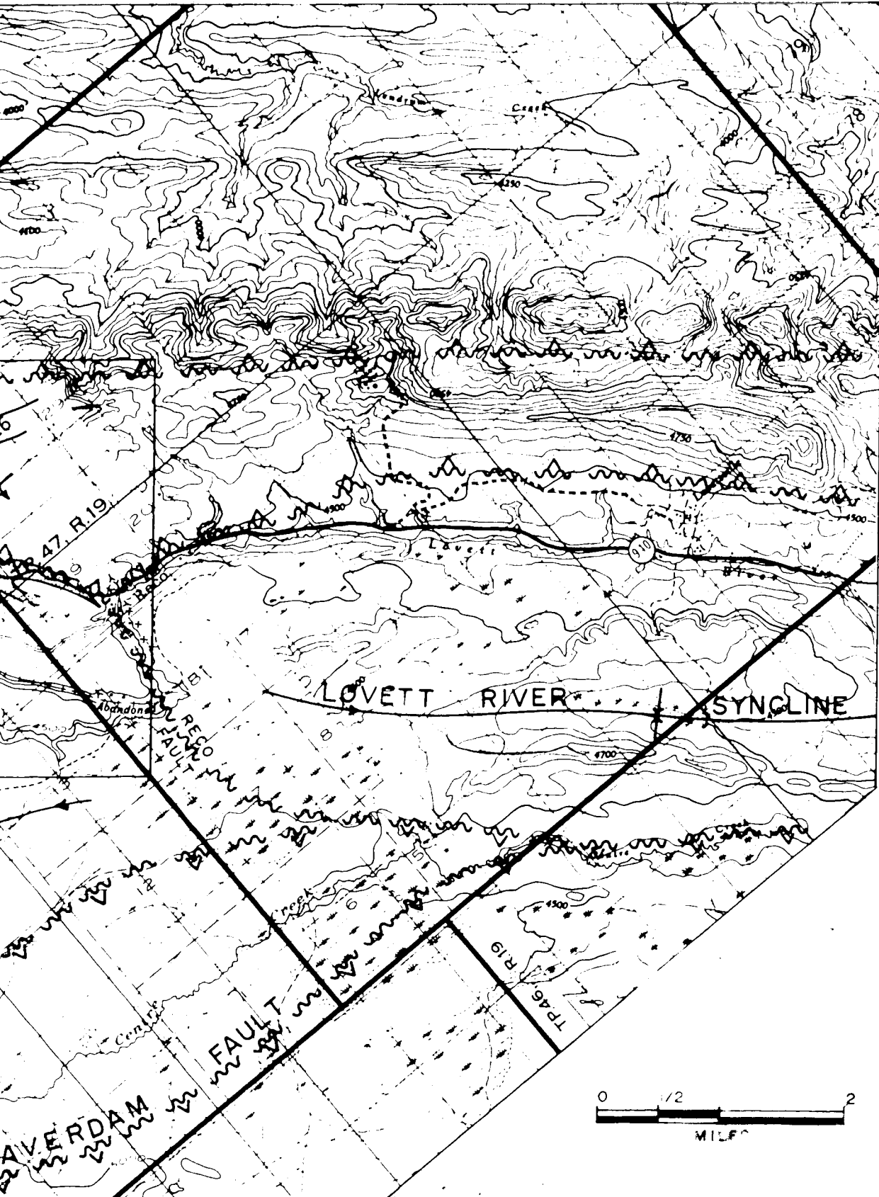
FIGURE 2: REGIONAL GEOLOGY of the STUDY AREA
