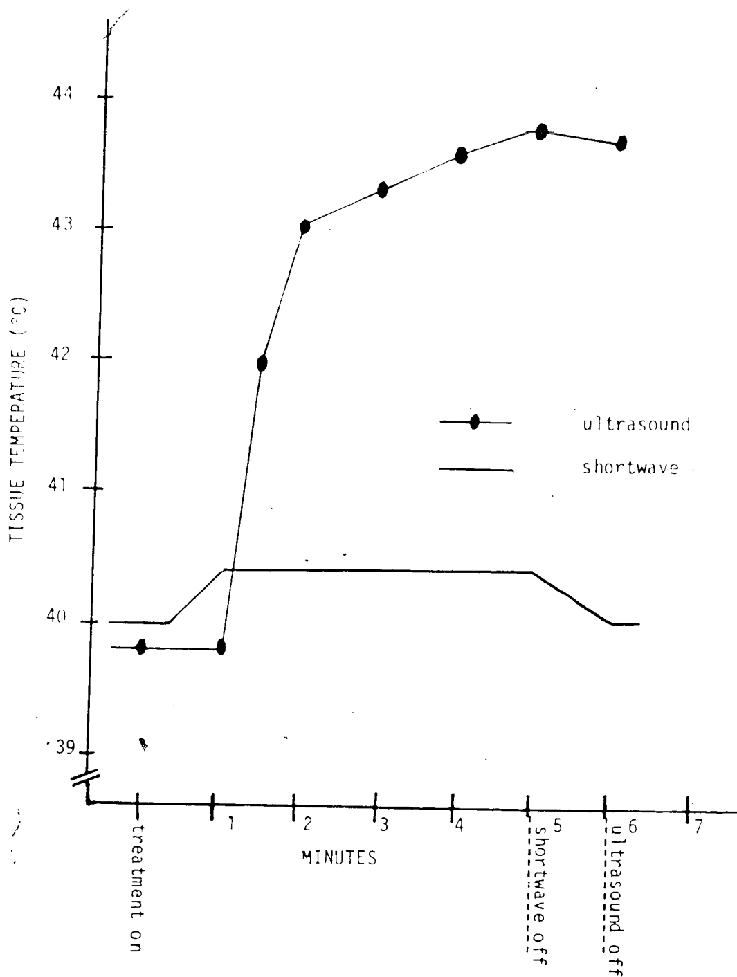
FIGURE 1: CHANGE IN TEMPERATURE INSIDE THE HIP JOINT FOLLOWING THE APPLICATION OF SHORTWAVE DIATHERMY AND ULTRASOUND
