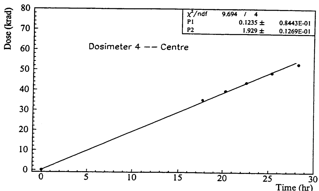
Figure 4.25: Combined TLD and Fricke test: Dose versus time measured in the central dosimeter.
