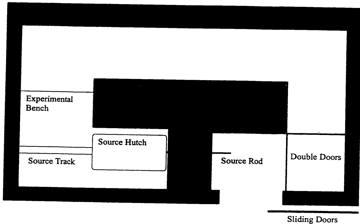
Figure 2.2: Cave-type cobalt-60 source at the University of Alberta, not to scale.
