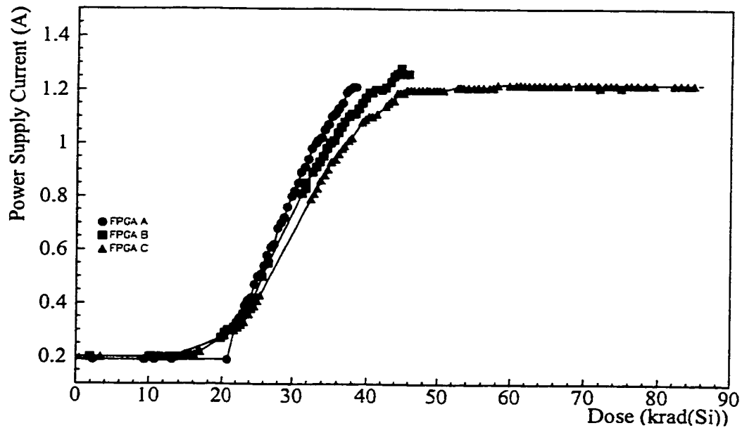
Figure 5.7: Current versus dose for XLA FPGAs, first irradiation period.
