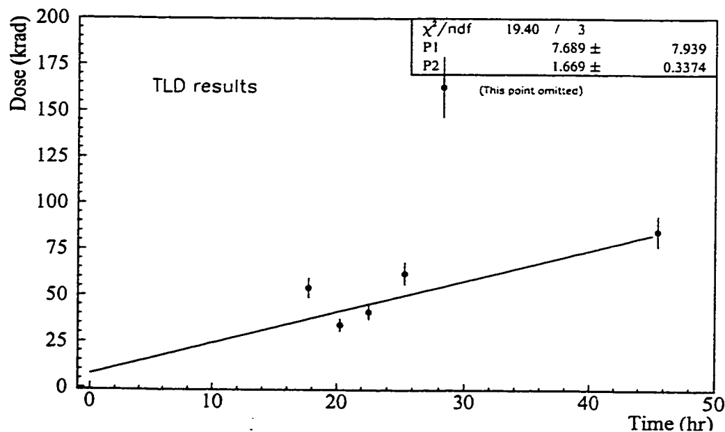
Figure 4.29: Combined TLD and Fricke test: Comparison of TLD results to time spent under irradiation.
