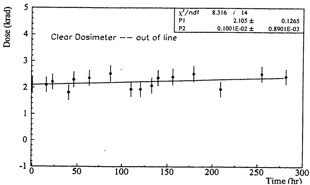
Figure 4.12: Lead wall test: Dose versus time measured in the background dosimeter out of the line of radiation.
