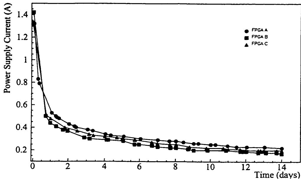
Figure 5.9: Current versus time for XLA FPGAs during annealing.
