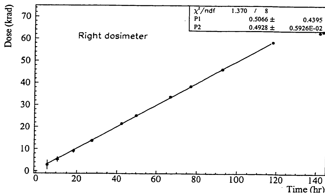
Figure 4.4: First Fricke dosimetry test: Dose versus time measured in the right dosimeter.
