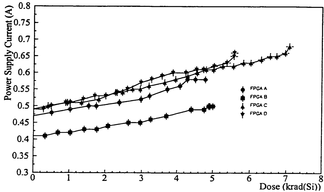
Figure 5.4: Current versus dose for XL FPGAs, second irradiation period.
