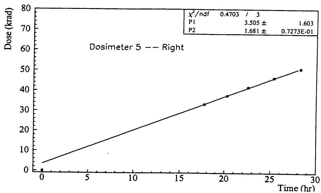
Figure 4.26: Combined TLD and Fricke test: Dose versus time measured in the near right dosimeter.
