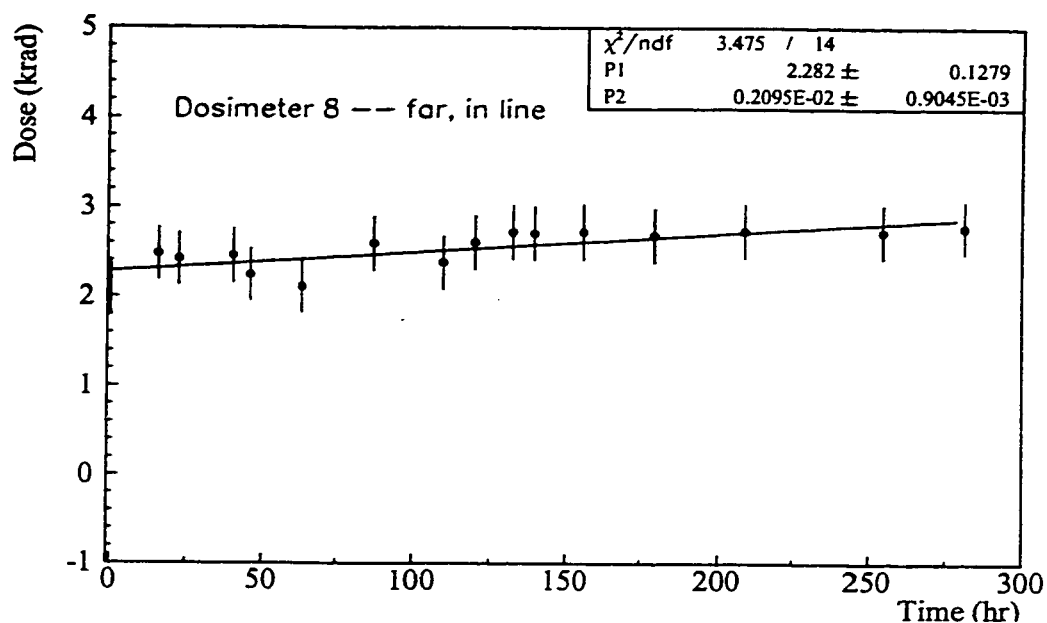
Figure 4.11: Lead wall test: Dose versus time measured in the background dosimeter in the line of radiation.
