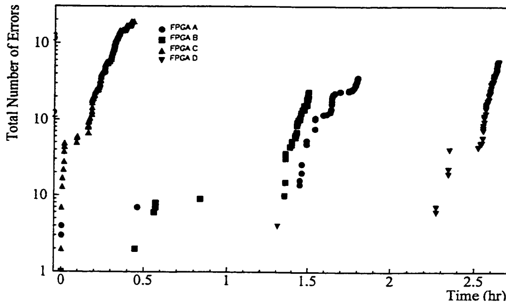
Figure 5.2: Errors versus time since first error for XL FPGAs, first irradiation period.
