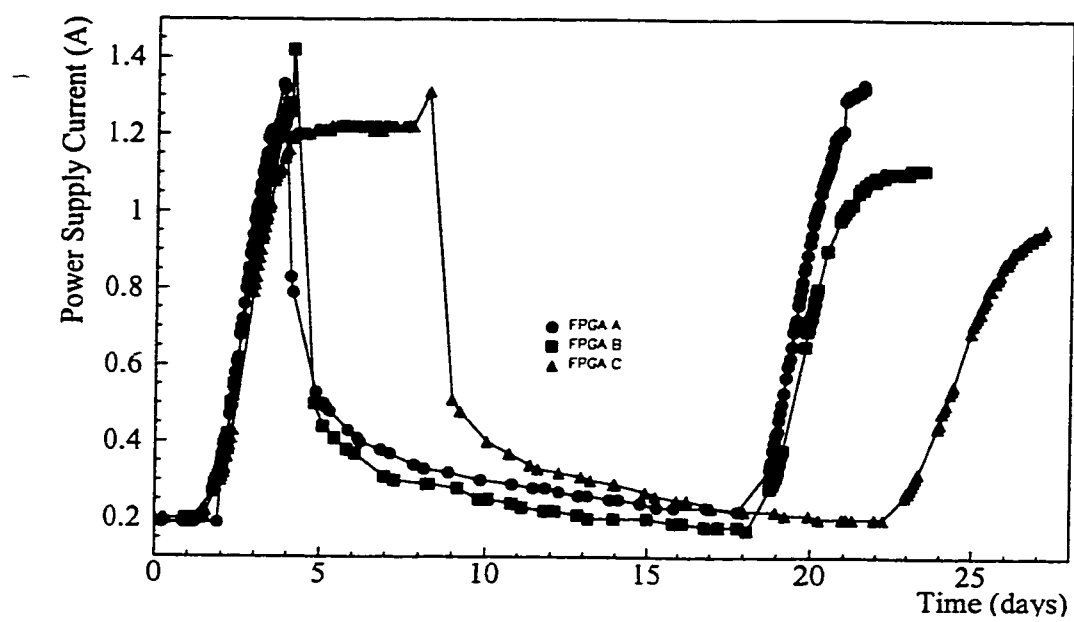
Figure 5.12: Current versus time for XLA FPGAs, entire test.
