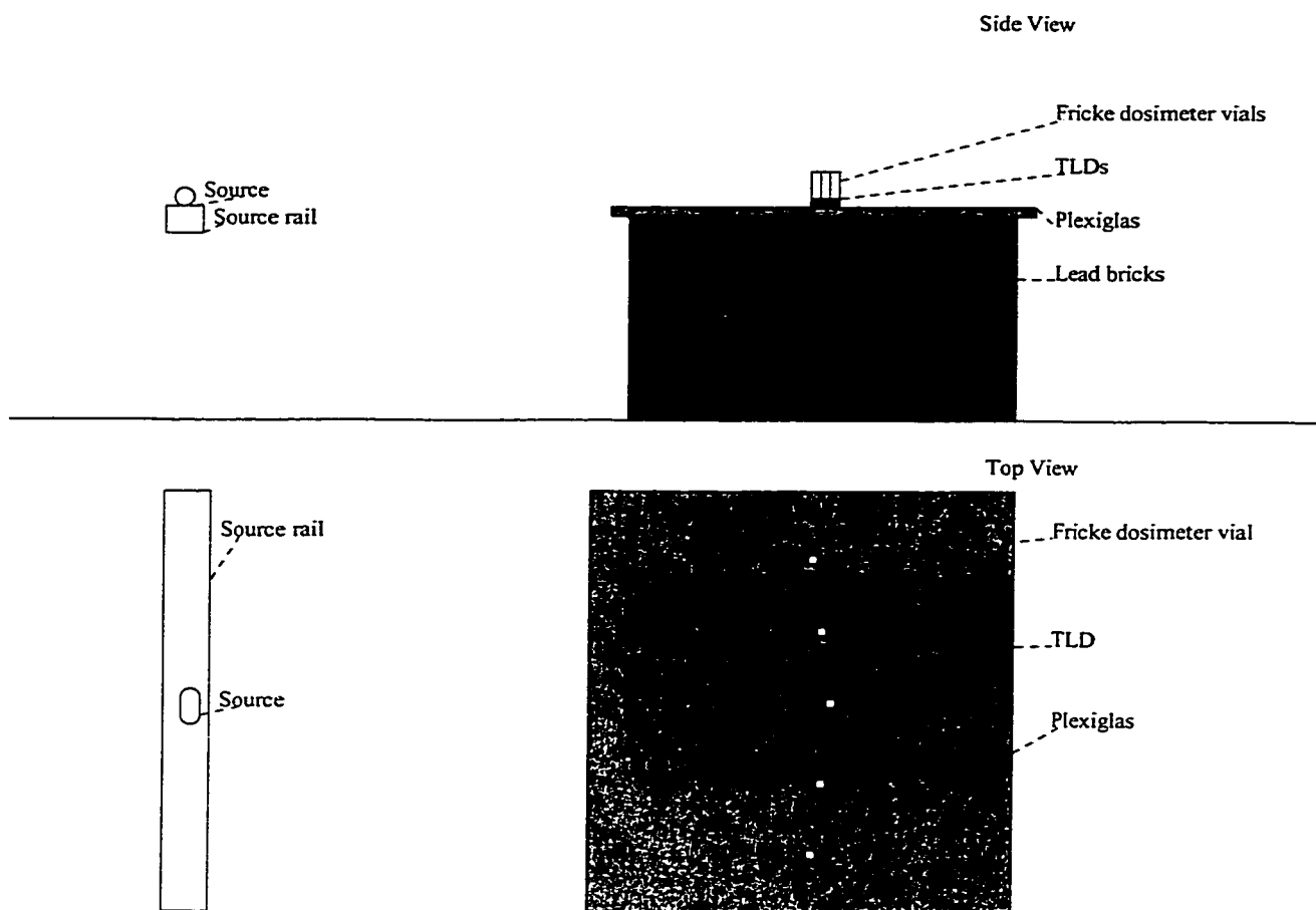
Figure 4.22: Setup for combined TLD and Fricke dosimetry test, not to scale.
