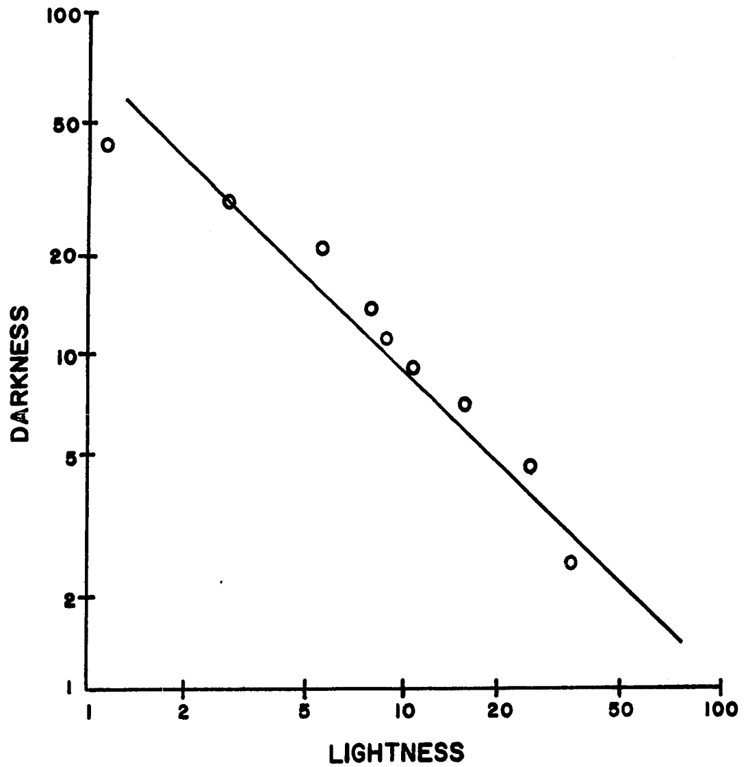
Figure 5. Magnitude estimations of darkness as a function of magnitude estimates of lightness in log-log coordinates. The straight line was fitted by eye.
