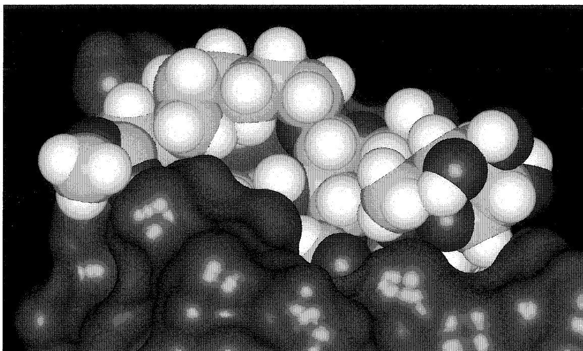
Figure 3.2. Model based on the X-ray structure of the binding site of chimeric BR96 complexed with 8-methoxycarbonyloctyl Le y derivative 22. 33 The Connolly surface of the antibody is displayed in blue; the CPK model of the Le y antigen is displayed in green (carbon), red (oxygen), and white (hydrogen). The aglycon of Le y derivative 22 contributes favourably to the interaction with BR96.
