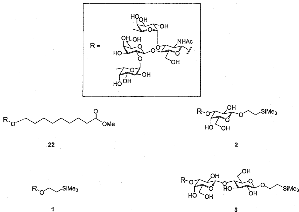
Figure 3.1. Analogues of the Le y determinant (R) for which B3 binding affinities were estimated by FAC/MS
