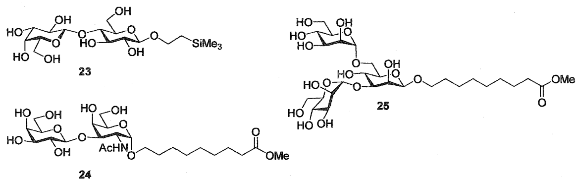
Figure 3.7. Void markers for the B3 affinity column. These compounds were used to ascertain the elution volume in the absence of specific binding.
