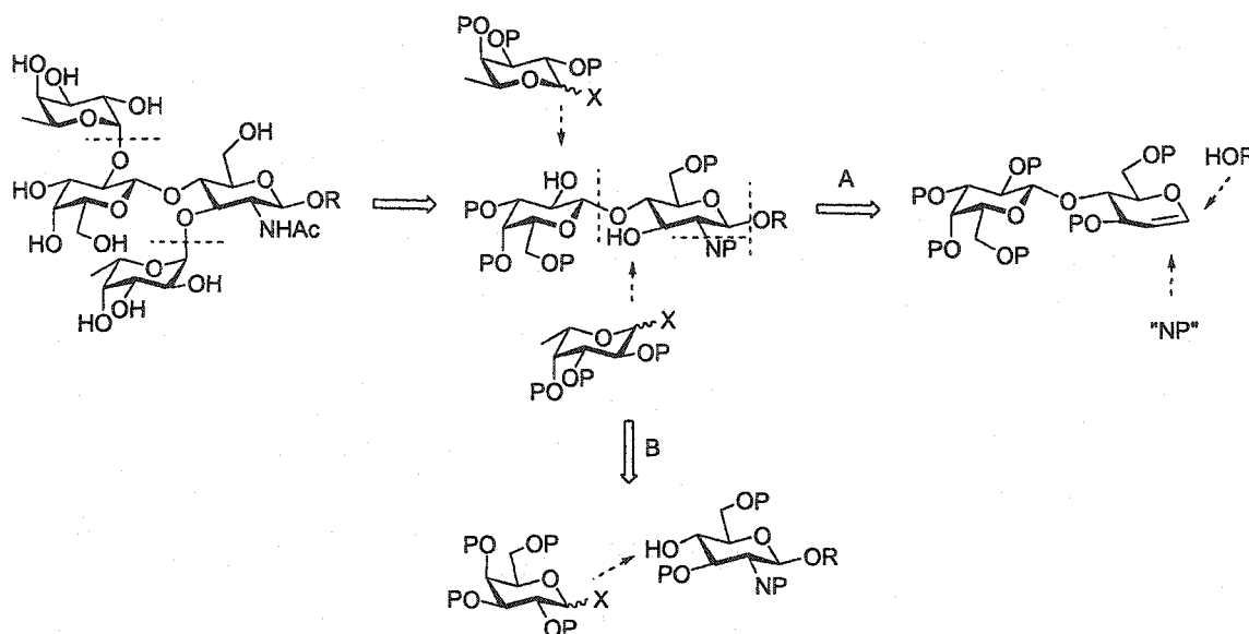
Figure 2.7. Le' retrosynthetic strategies in which two disconnections are made simultaneously to give a fucose donor and lactosamine acceptor. P = protective group; X = anomeric leaving group. Route A: lactosamine is derived from lactal (see Table 2.1, entries 1, 2, 4 and 6). Route B: lactosamine is constructed from galactose and glucosamine, either enzymatically (see Table 2.1, entry 5) or chemically (see Table 2.2, entries 1-4, 6-8).
