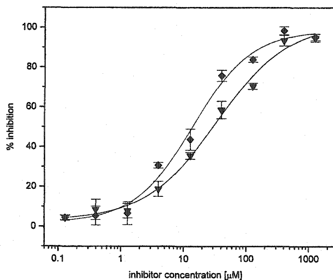
Figure 3.13. Inhibition of B3 binding to synthetic Le y -BSA glycoconjugate with 2 synthetic Le y derivatives. Shown overlaid are the data obtained from inhibition ELISAs using tetrasaccharide 1 (▼) and hexasaccharide 3 (◆).
