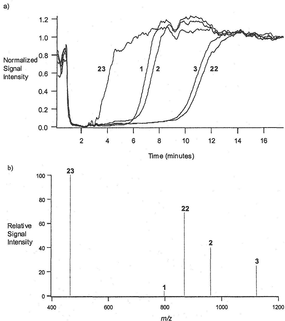
Figure 3.11. FAC/MS screening of B3 affinity for Le^y derivatives 1, 2, 3, and 22. A mixture of the three Le^y derivatives and void volume marker 23 ( 2 \mu\text{M} each) in buffer ( 10 \text{ mM NH}_4\text{OAc} , 1 \text{ mM NaCl} , \text{pH } 7.4 ) was infused ( 8 \mu\text{L}/\text{min} ) through a B3 affinity column and the effluent was monitored by electrospray MS in SIM and positive ion mode. (a) The overlaid, extracted ion chromatograms for the compounds, drawn using the IGOR program. (b) Mass spectrum of the effluent from the B3 affinity column after compounds 1, 2, 3, 22 and 23 have broken through at their infusion concentration. The compounds were monitored at m/z values corresponding to their sodium adducts, i.e., (M + \text{Na})^+ .
