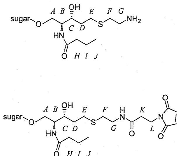
Figure 6.1. Labelling of aglycon protons used in NMR signal assignments
