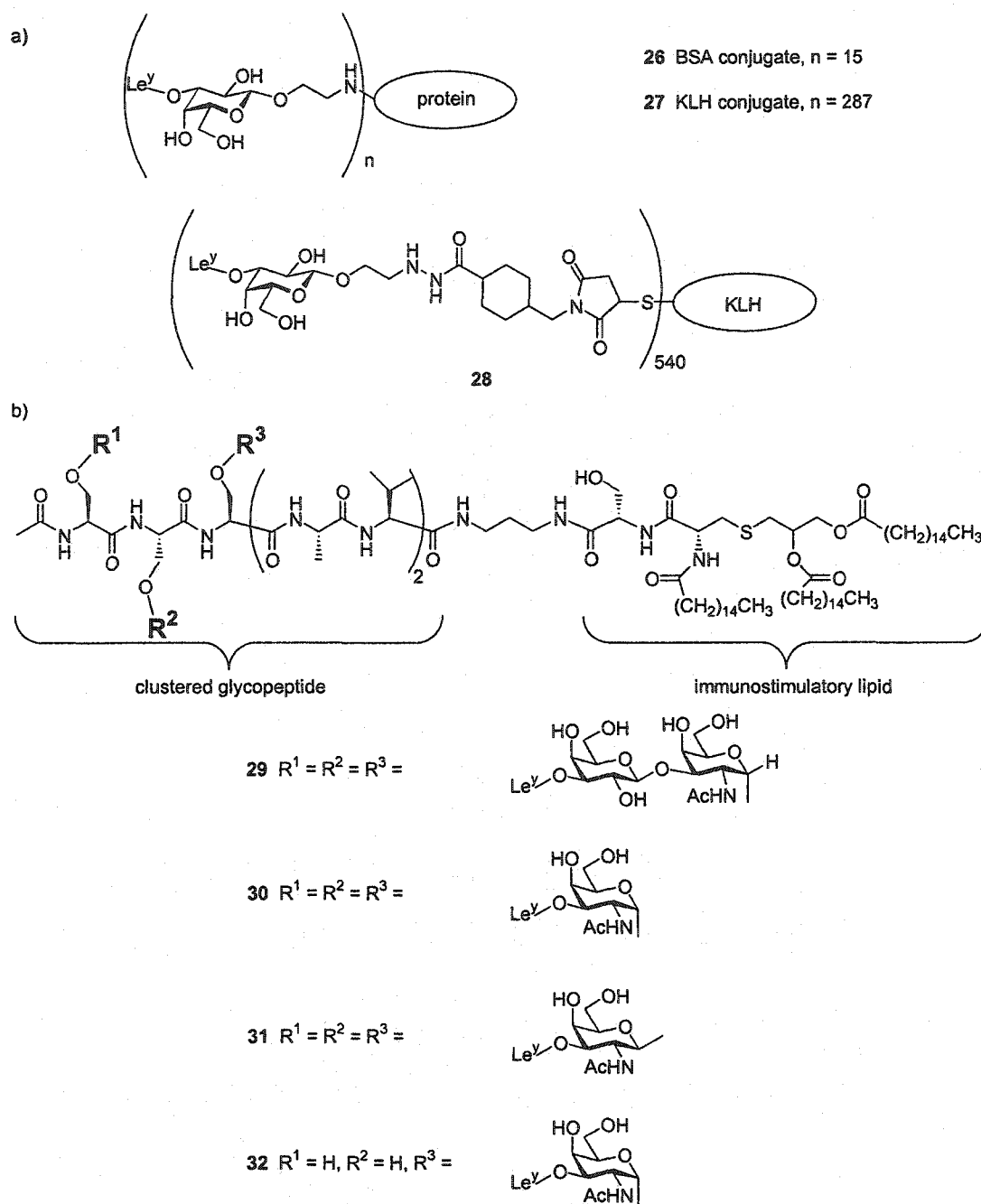
Figure 4.1. Mono-antigenic, Le^y -based anticancer vaccines synthesized by Danishefsky et al. a) Monovalent conjugate vaccines (b) Clustered conjugate vaccines. Glycolipopeptides 29-32 were designed to mimic the clustered domains of O-linked mucin glycoproteins.
