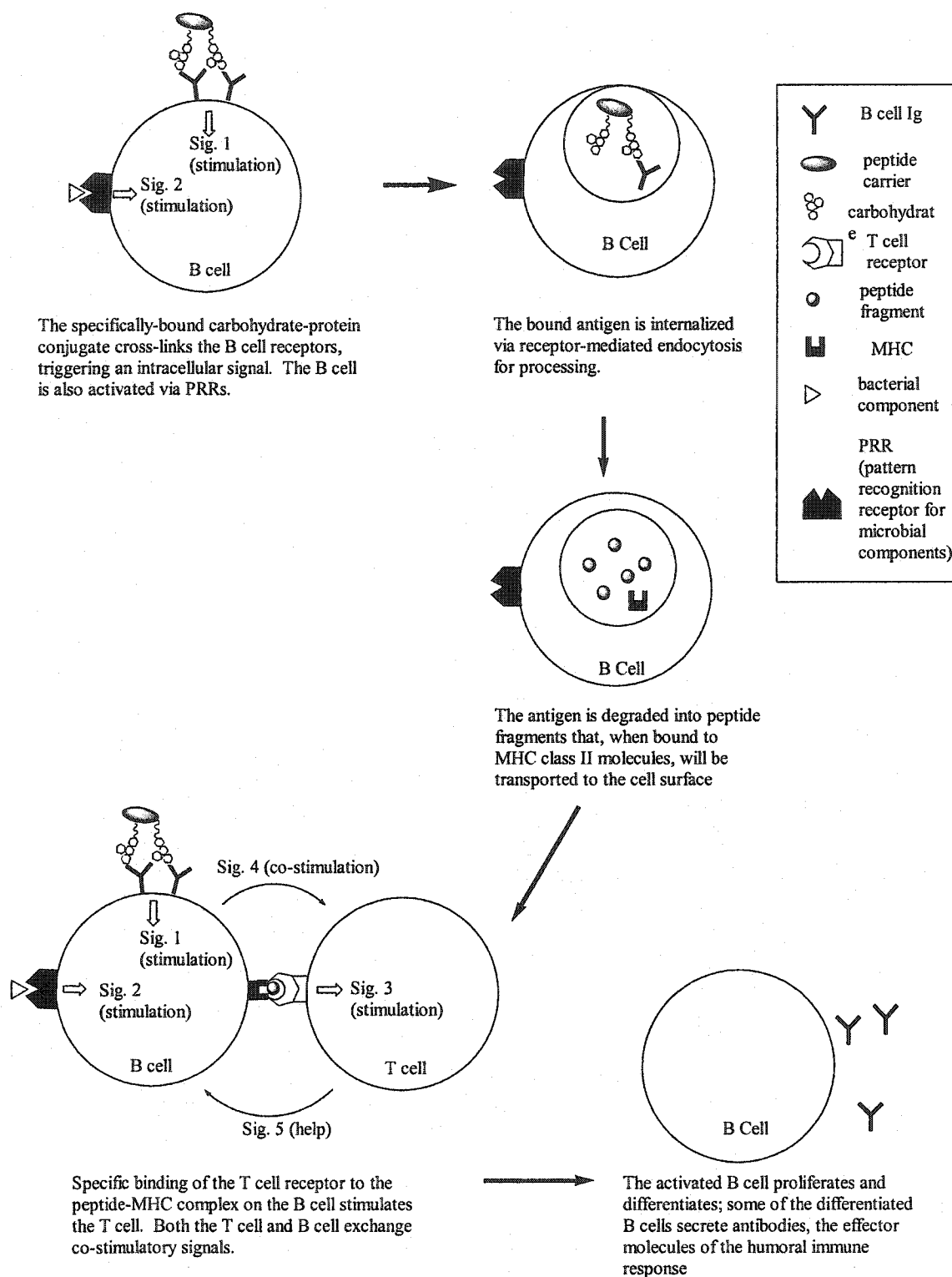
Figure 1.3. Protein antigens conjugated to carbohydrate antigens allow T cells to help activate carbohydrate-specific B cells
