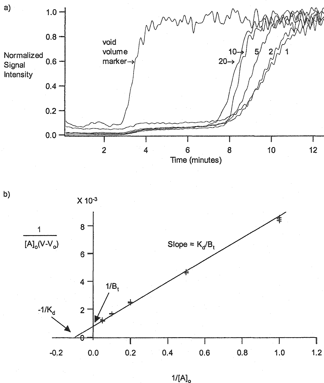
Figure 3.6. a) Overlay of frontal profiles obtained following the infusion of 5 different concentrations of ligand A ( [A]_0 = 1, 2, 5, 10, \text{ or } 20 \mu\text{M} ) through an affinity column. Measurement of the retention volume ( V-V_0 ) for each concentration of the analyte [A]_0 allows the determination of K_d and B_t as shown in (b). b) Plot illustrating the linear relationship between the reciprocal of adsorbed A and the reciprocal of [A]_0 as described by Equation 2. K_d is obtained from the slope and B_t is obtained from the y-intercept of the line.
