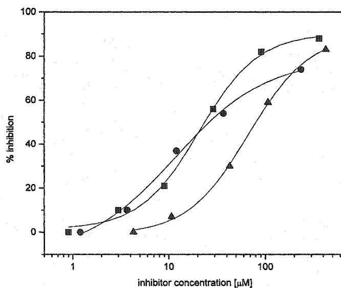
Figure 3.12. Inhibition of B3 binding to synthetic Le y -BSA glycoconjugate with 3 synthetic Le y derivatives. Shown overlaid are the data obtained from inhibition ELISAs using pentasaccharide 2 (▲), hexasaccharide 3 (■), and tetrasaccharide 22 (●).
