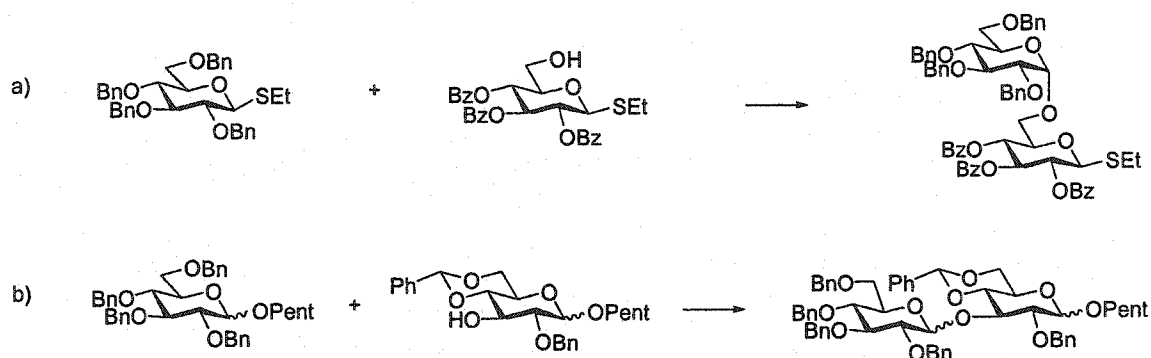
Figure 2.2. Examples of chemoselective glycosylations controlled by protective groups. 46 Self-condensation does not occur. (a) Acyl substituents reduce the reactivity of a donor compared to alkyl groups. (b) The fused ring of a cyclic acetal reduces the reactivity of a donor by inflicting torsional strain upon the developing oxo-carbenium ion intermediate. In both A and B, the product itself is also a potential donor.
