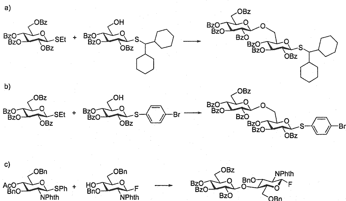
Figure 2.3. Examples of chemoselective glycosylations controlled by modifying the anomeric leaving group. 46, 47 Self-condensation does not occur. (a) Bulky thiol aglycons reduce the reactivity of a donor. (b) Decreased electron-donating properties of thiol aglycons reduce the reactivity of a donor. (c) "Orthogonal glycosylation" results from selective activation of different anomeric leaving groups. In A, B, and C, the product itself is also a potential donor.
