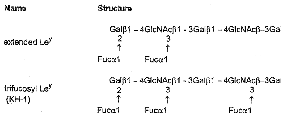
Figure 3.3. Antigenic determinants incorporating the Le y motif. Trifucosyl Le y , though sharing structural similarities with Le y , falls into a different class of antigens. Unlike the Le y antigen that is detected in a number of normal tissues but is very highly expressed in some tumor cells, trifucosyl Le y is highly expressed in tumor cells but absent in progenitor cells. 4
