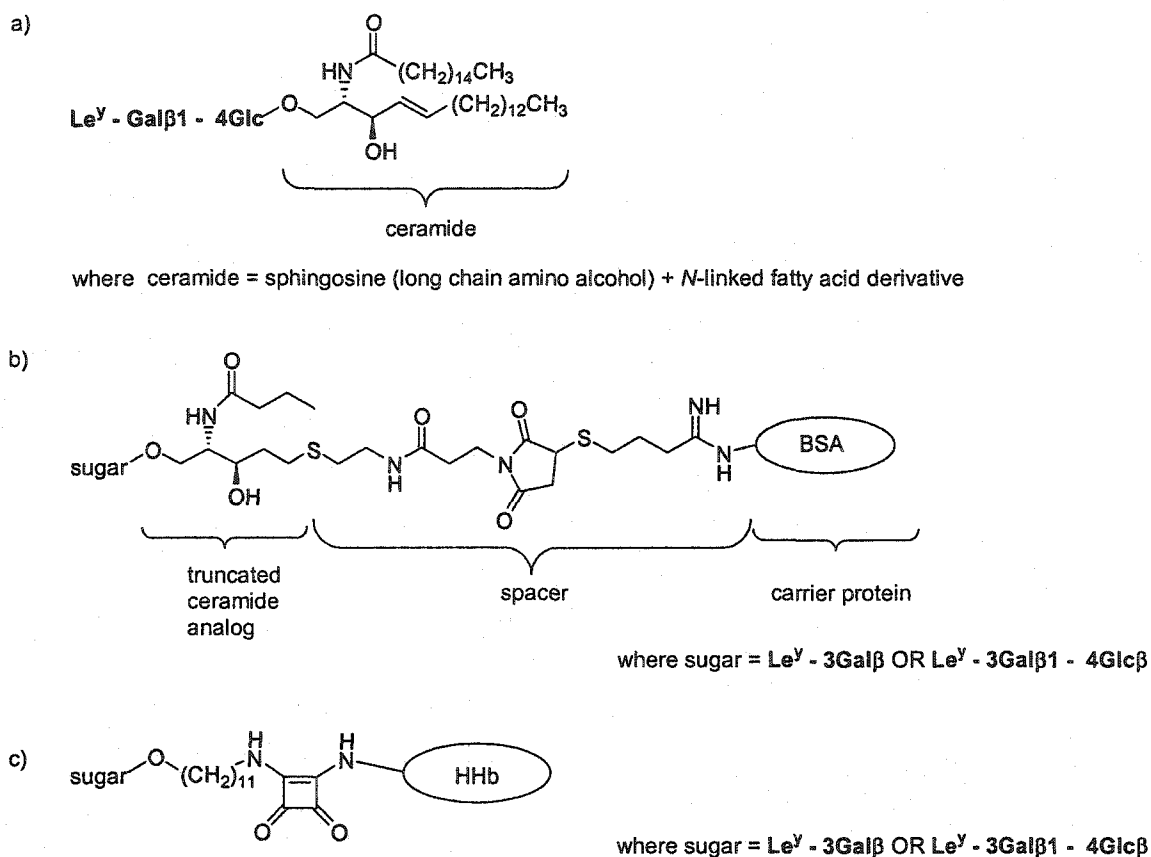
Figure 4.3. Design of synthetic glycoconjugate targets. (a) Generalized structure of naturally occurring \text{Le}^y glycosphingolipid (b) \text{Le}^y -BSA conjugate vaccine that mimics the presentation of \text{Le}^y in the context of a glycolipid (c) \text{Le}^y -HHb conjugate for ELISA screening of carbohydrate-specific antibodies.
