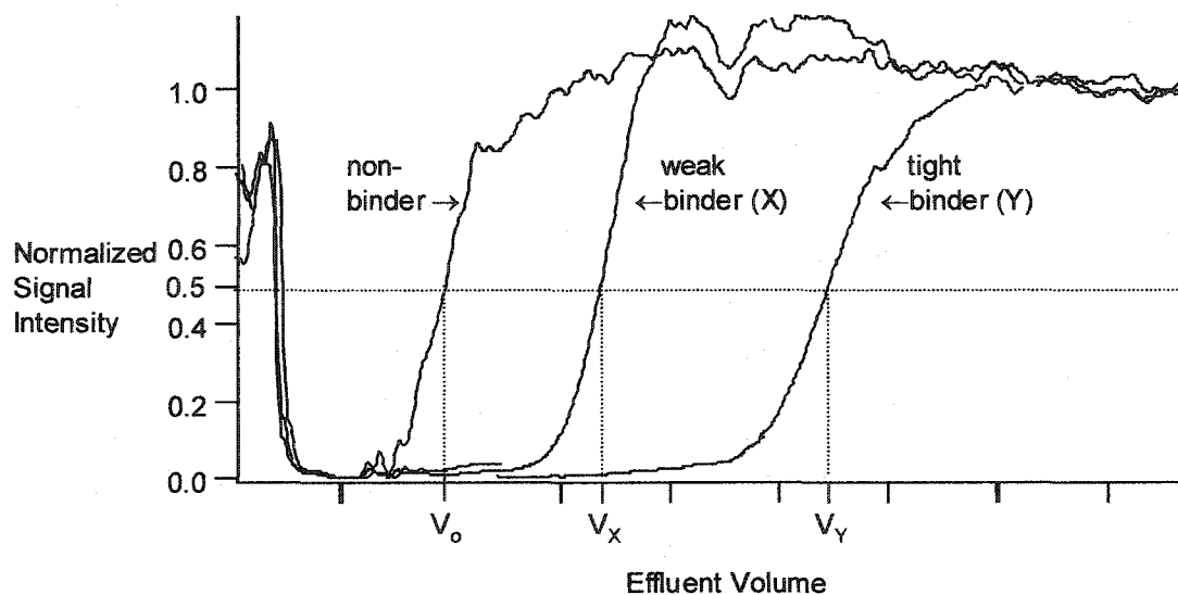
Figure 3.5. Example of a FAC/MS chromatogram obtained from the continuous infusion of a mixture of 3 ligands of various activities through an affinity column. More active ligands are retarded on the column to a greater extent and consequently break-through later. One non-binding compound should be included in every analyte mixture to serve as a marker of the break-through volume in the absence of specific interaction ( V_0 ) for the accurate measurement of retention volumes of active ligands ( V-V_0 ). Selected ion monitoring of the effluent from the column by electrospray MS allows the extraction of frontal chromatograms for each m/z of interest, shown here overlaid and normalized.
