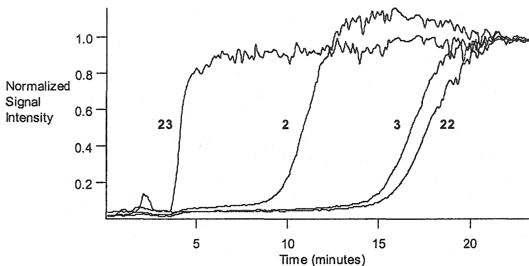
Figure 3.10. FAC/MS screening of the activity of Le^y derivatives 2, 3, and 22 as ligands for antibody B3. The data shown here was drawn using the IGOR program. A mixture of the three Le^y derivatives and void volume marker 23 ( 2 \mu\text{M} each) in buffer (10 mM ammonium acetate, 1 mM sodium chloride, pH 7.4) was infused ( 8 \mu\text{L}/\text{min} ) through a B3 affinity column and the effluent was monitored by electrospray MS in SIM and positive ion mode. The overlaid, extracted ion chromatograms for the compounds are shown here.
