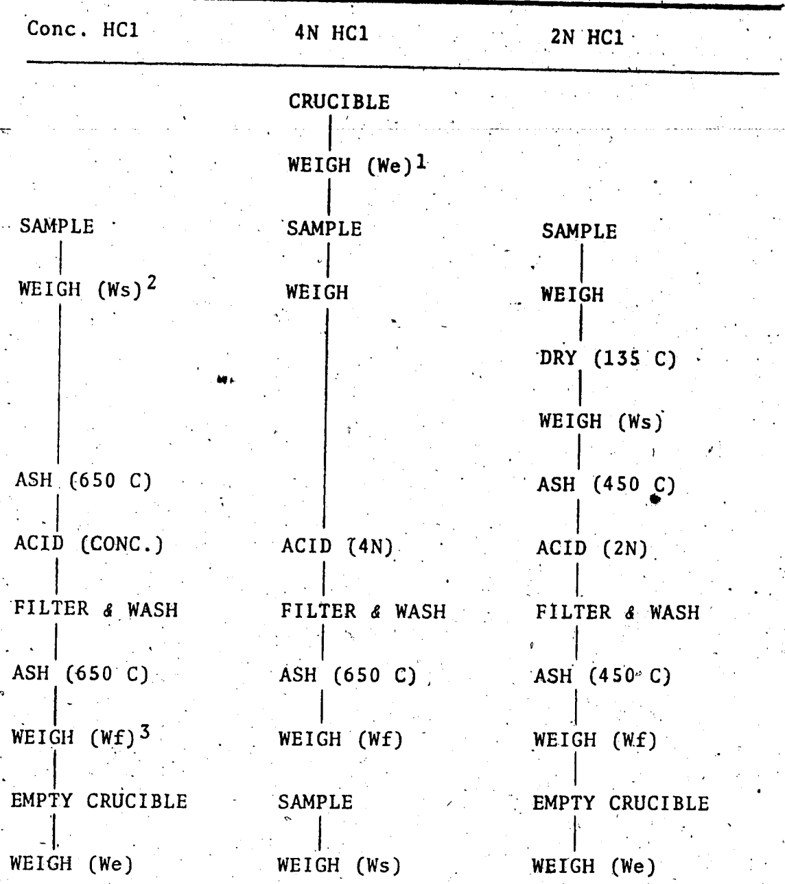
Figure 1. Acid-insoluble ash analytical procedures. Details of each are given in Appendices 1, 2 and 3.
