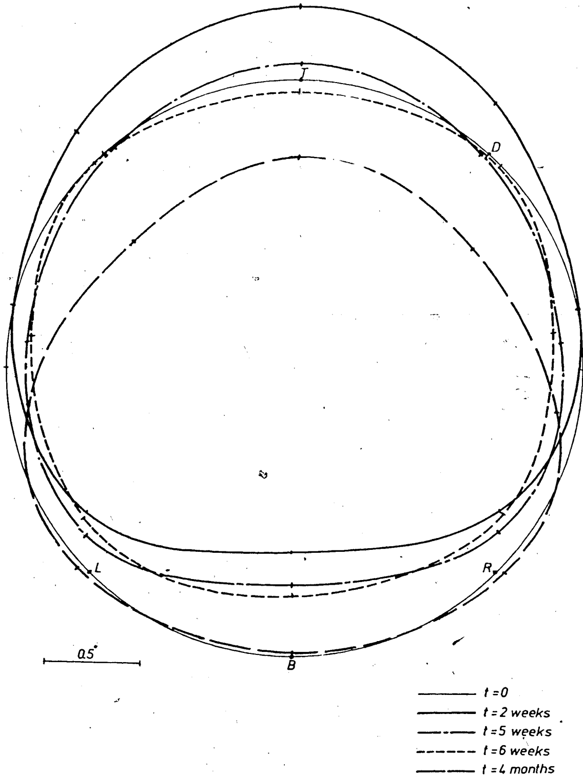
Figure 4.2 Deformed Shapes of the Ribs.
