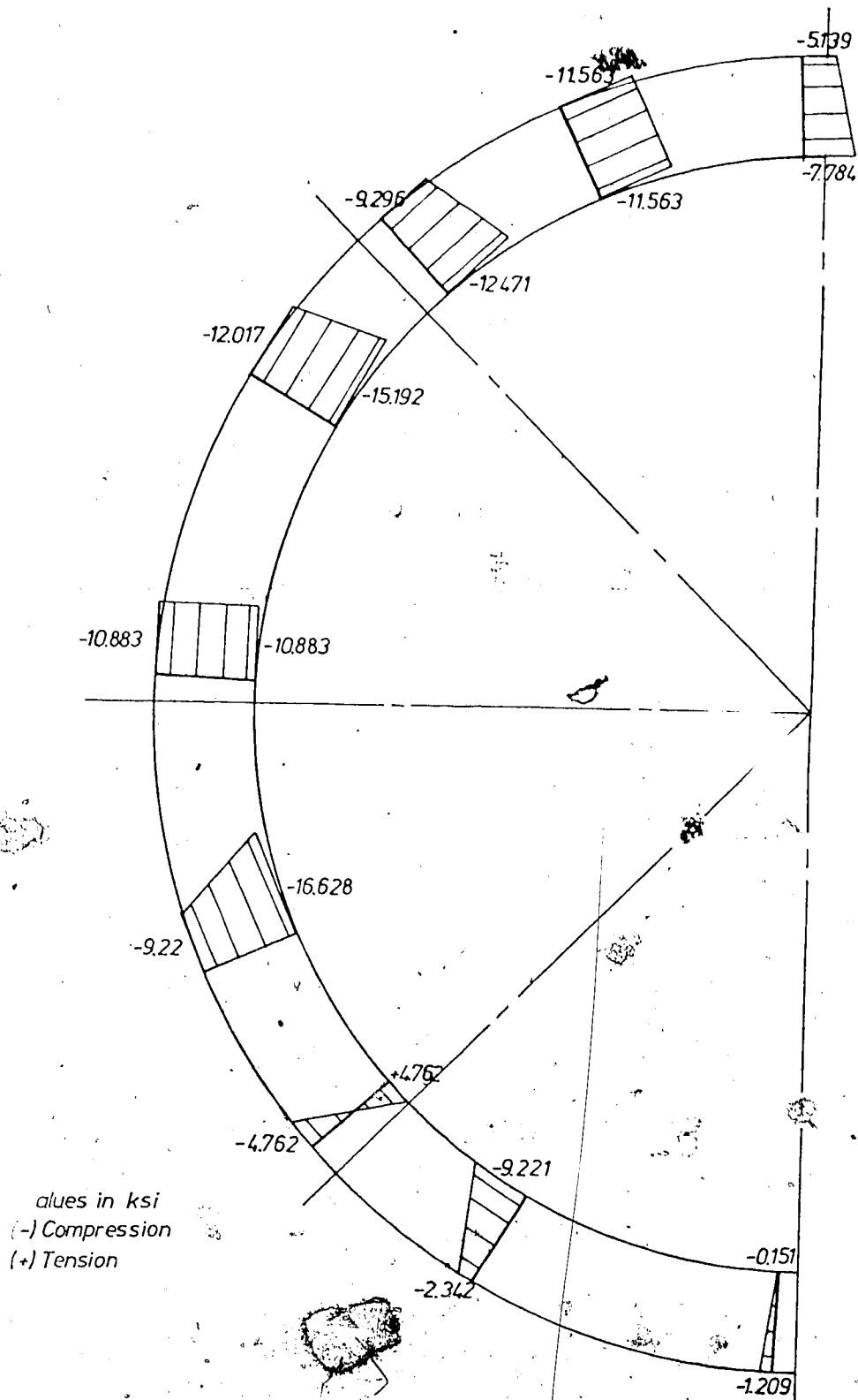
Figure 4.8 Calculated Stresses in the Ribs Using the Finite Element Method (June 1st, 1977)
