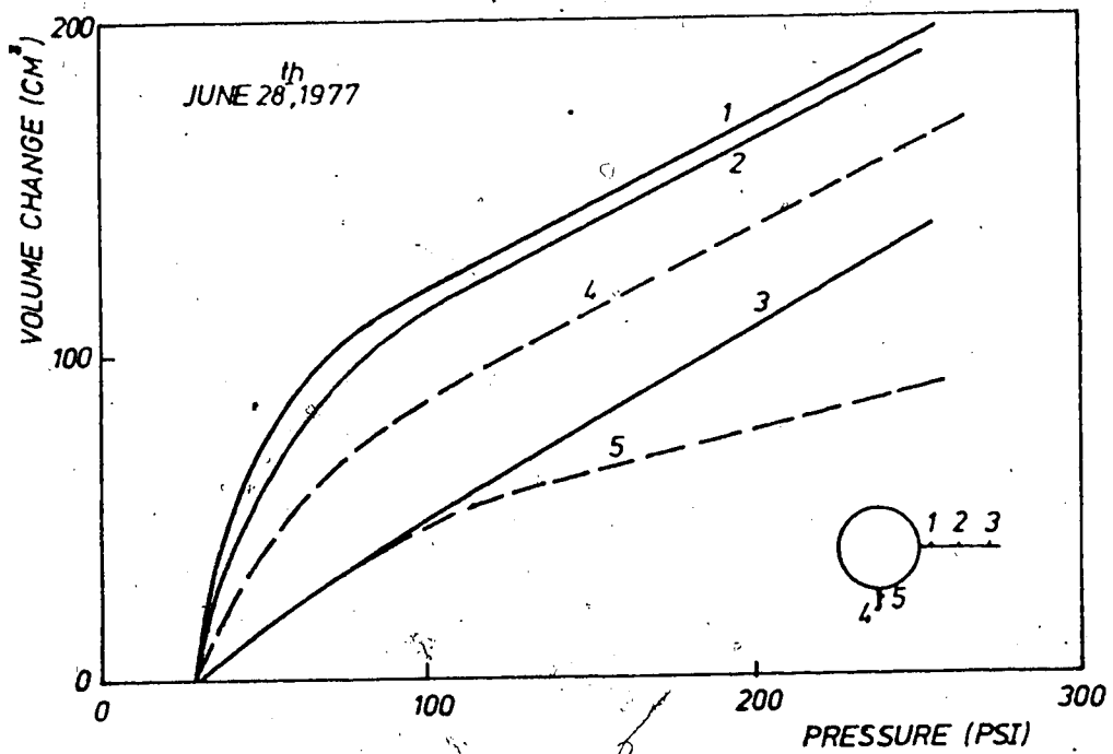
Figure 3.10 Results of In-situ Pressuremeter Tests.
