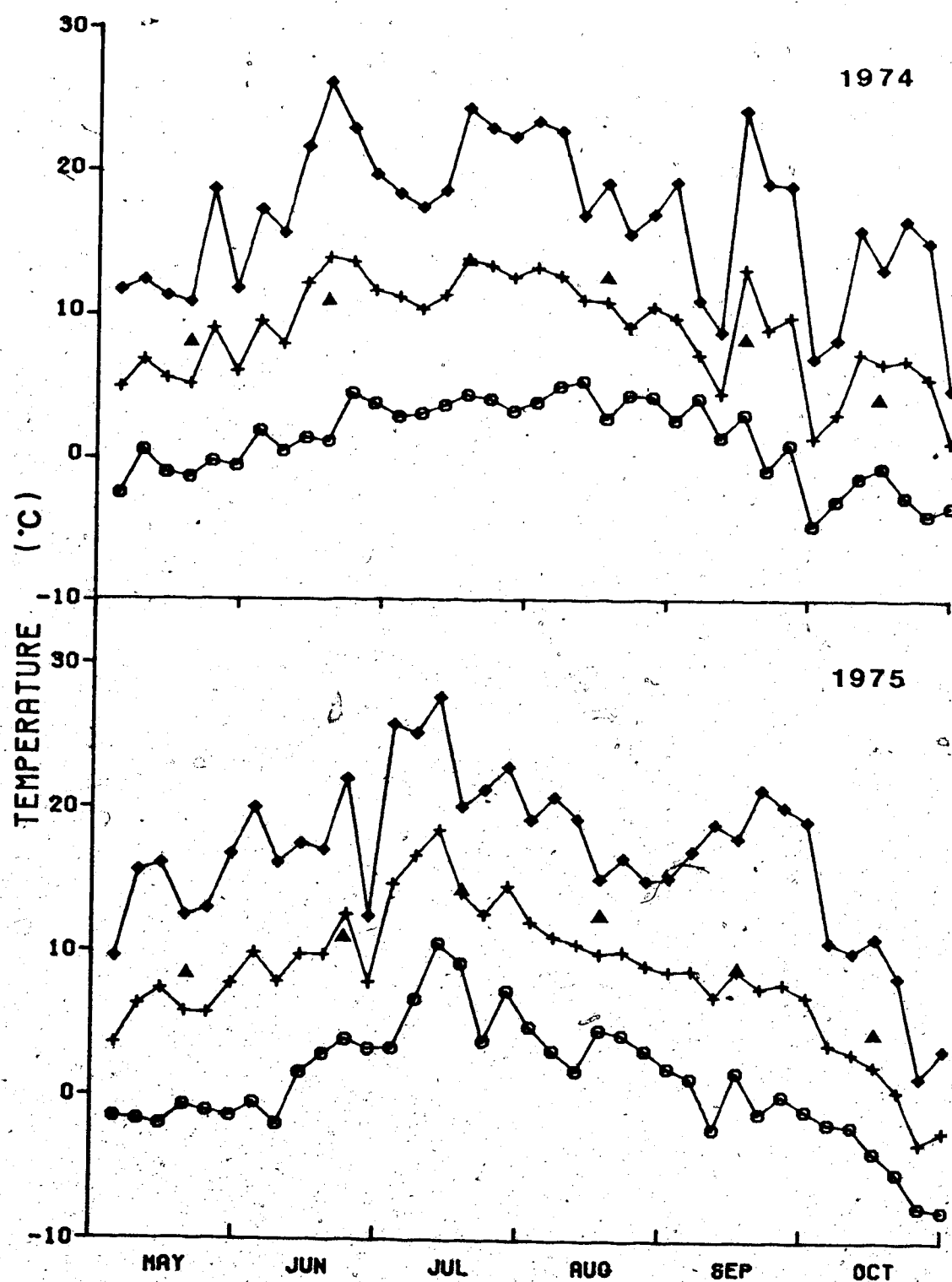
Figure 6. Five-day mean air temperatures at Tomenthypnum site: \blacklozenge = maximum; + = mean; \circ = minimum; \blacktriangle = 30-year means.
