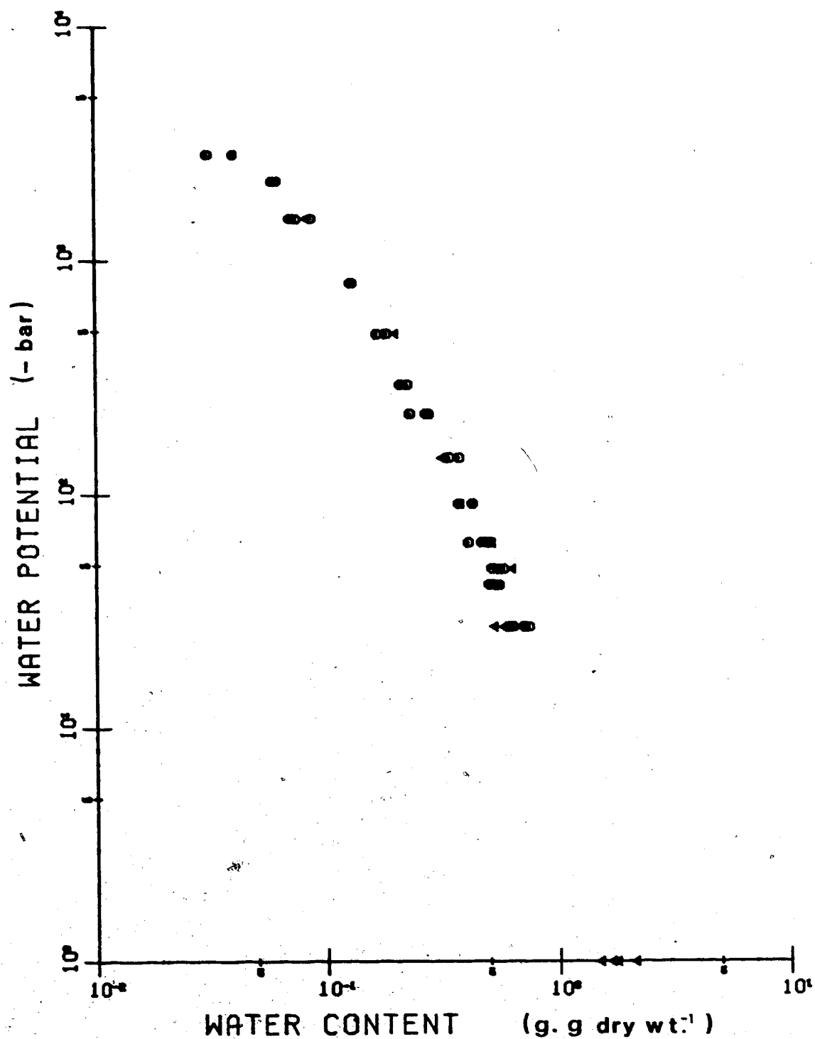
Figure 27. Ptilium crista-castrensis : water potential vs. water content. O = drying curve; ◄ = wetting curve.
