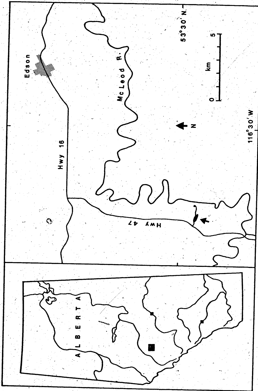
Figure 1. Location of study site 15 km s.w. of Edson, in west-central Alberta, Canada.
