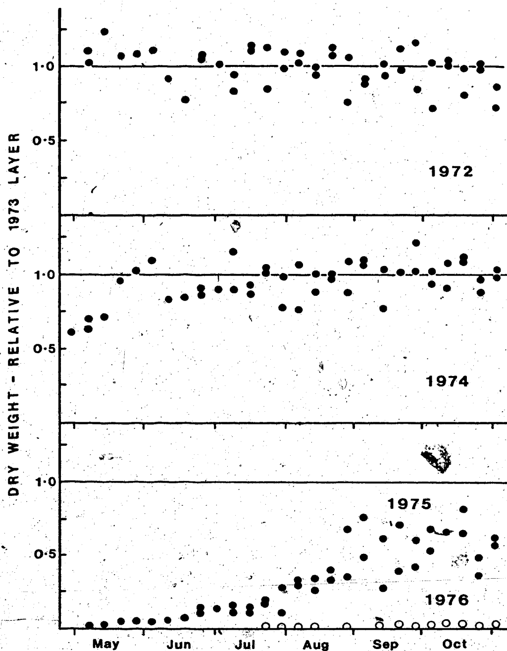
Figure 17. Growth of Hylocomium splendens in 1975. Changes in dry weight of the 1972, 1974, 1975 and 1976 layers expressed as ratios of the 1973 layer.
