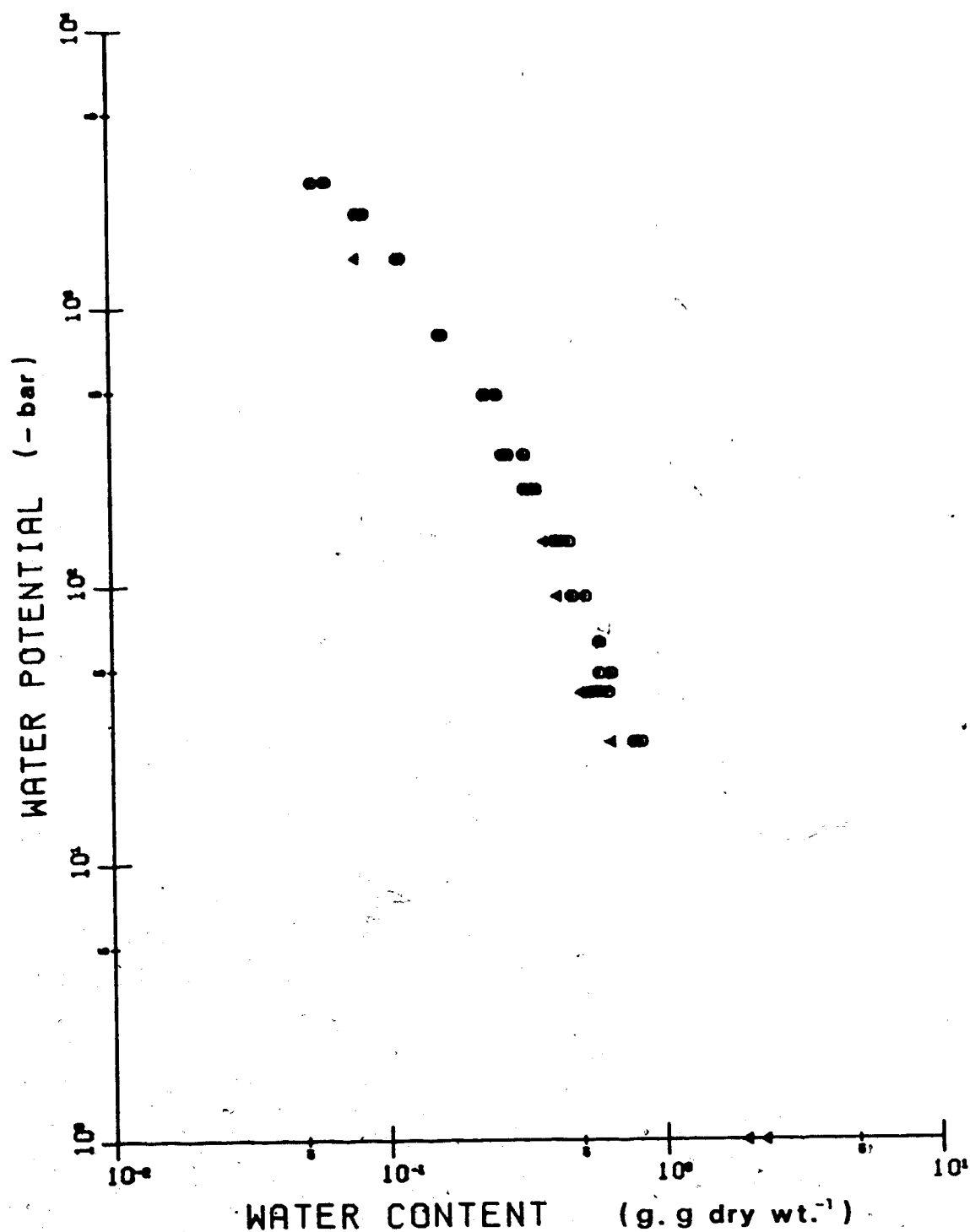
Figure 28. Tomenthypnum nitens : water potential vs. water content. O = drying curve; ◄ = wetting curve.
