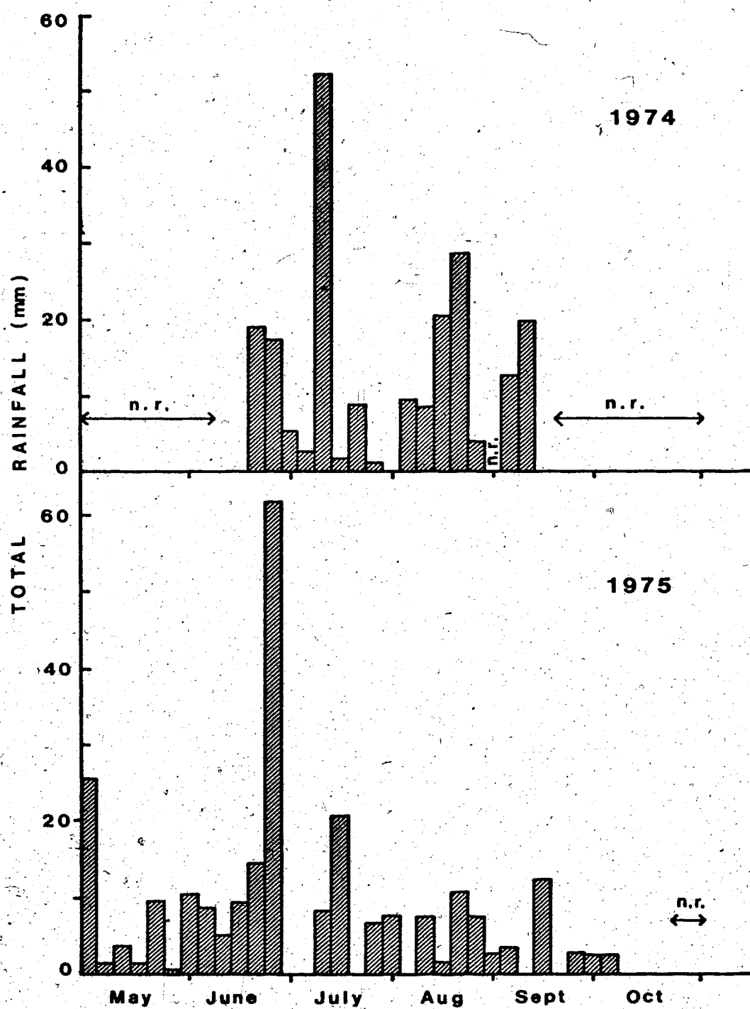
Figure 15: Five-day rainfall totals at Tomenthypnum site; n.r. = not recorded.
