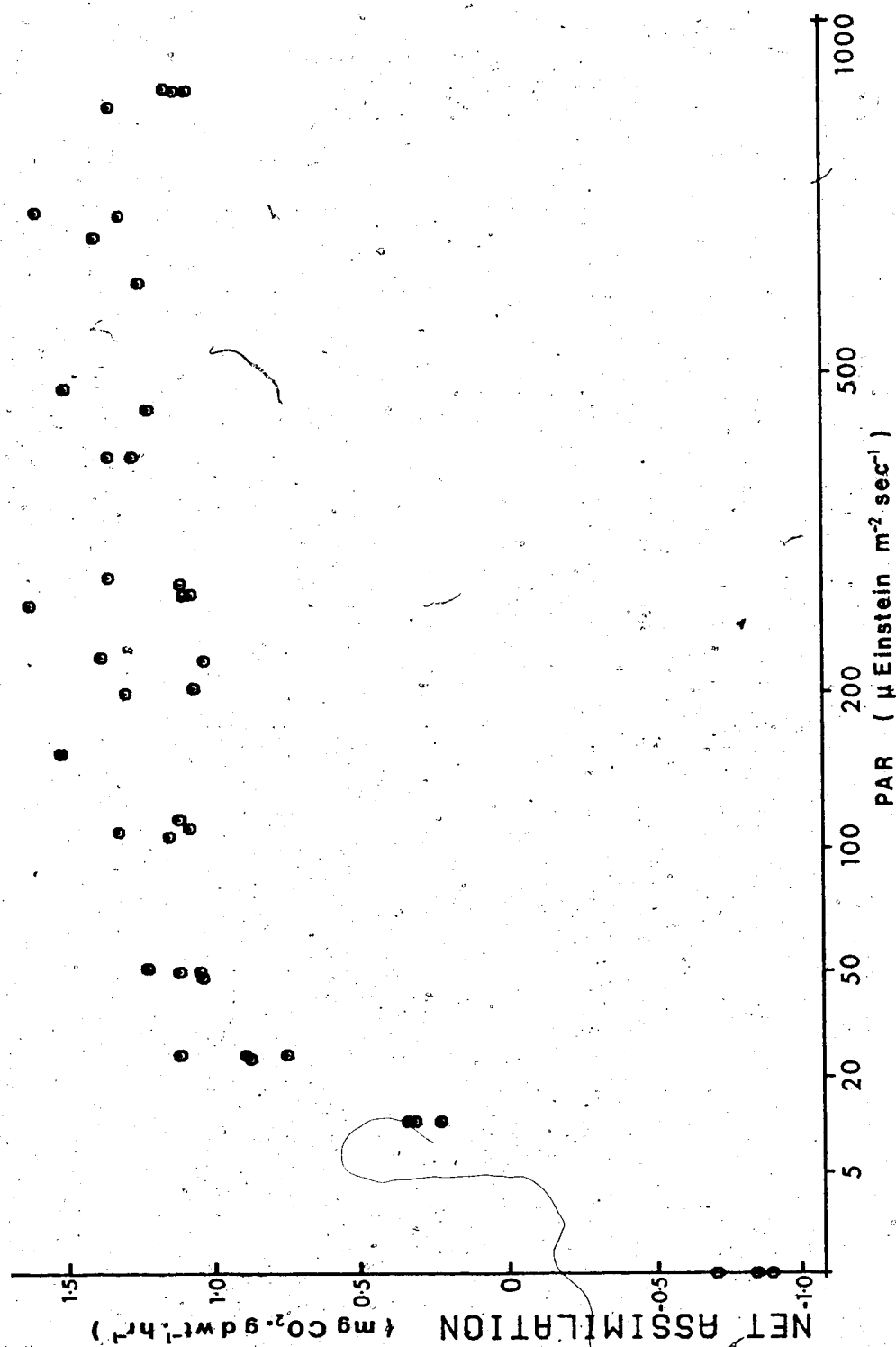
Figure 20. Light response curve of Tomenthypnum nitens at 15°C. PAR = Photosynthetically Active Radiation (400 - 700 nm).
