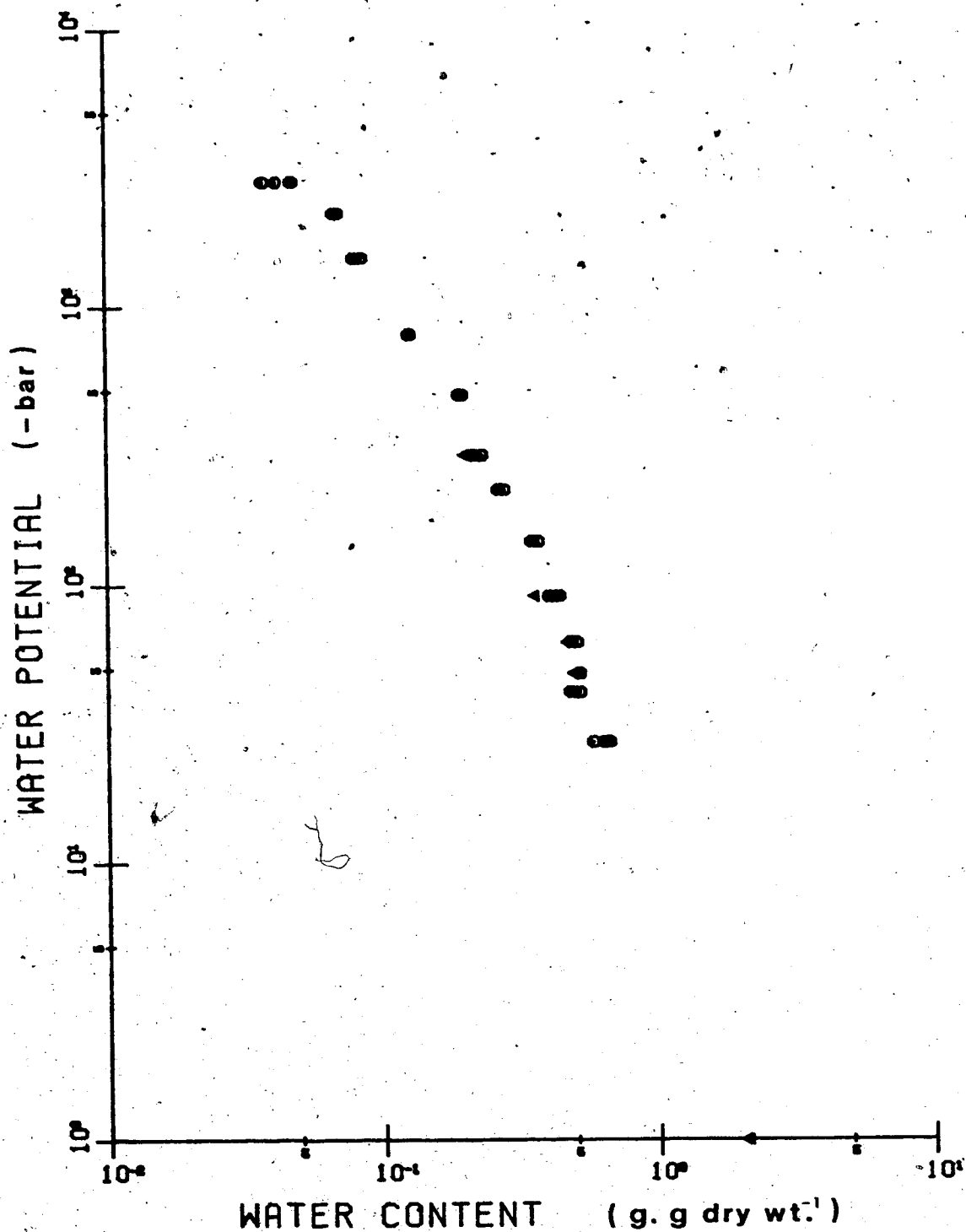
Figure 26. Pleurozium schreberi : water potential vs. water content. O = drying curve; ◄ = wetting curve.
