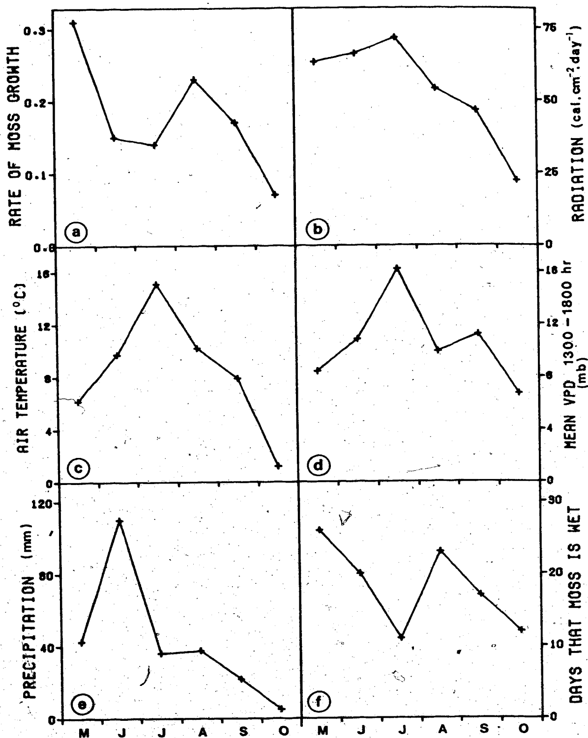
Figure 29. Growth of Hylocomium splendens (relative to 1973 layer) compared with selected environmental factors.
