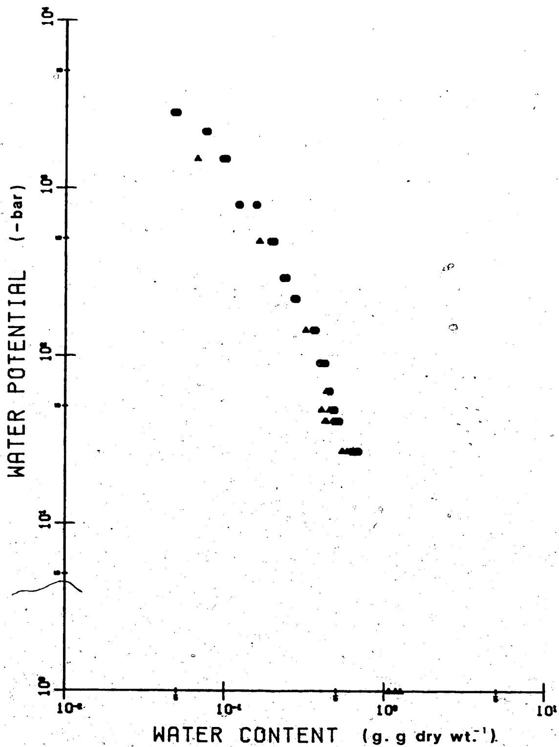
Figure 25. Hylocomium splendens : water potential vs. water content. O = drying curve; \Delta = wetting curve.
