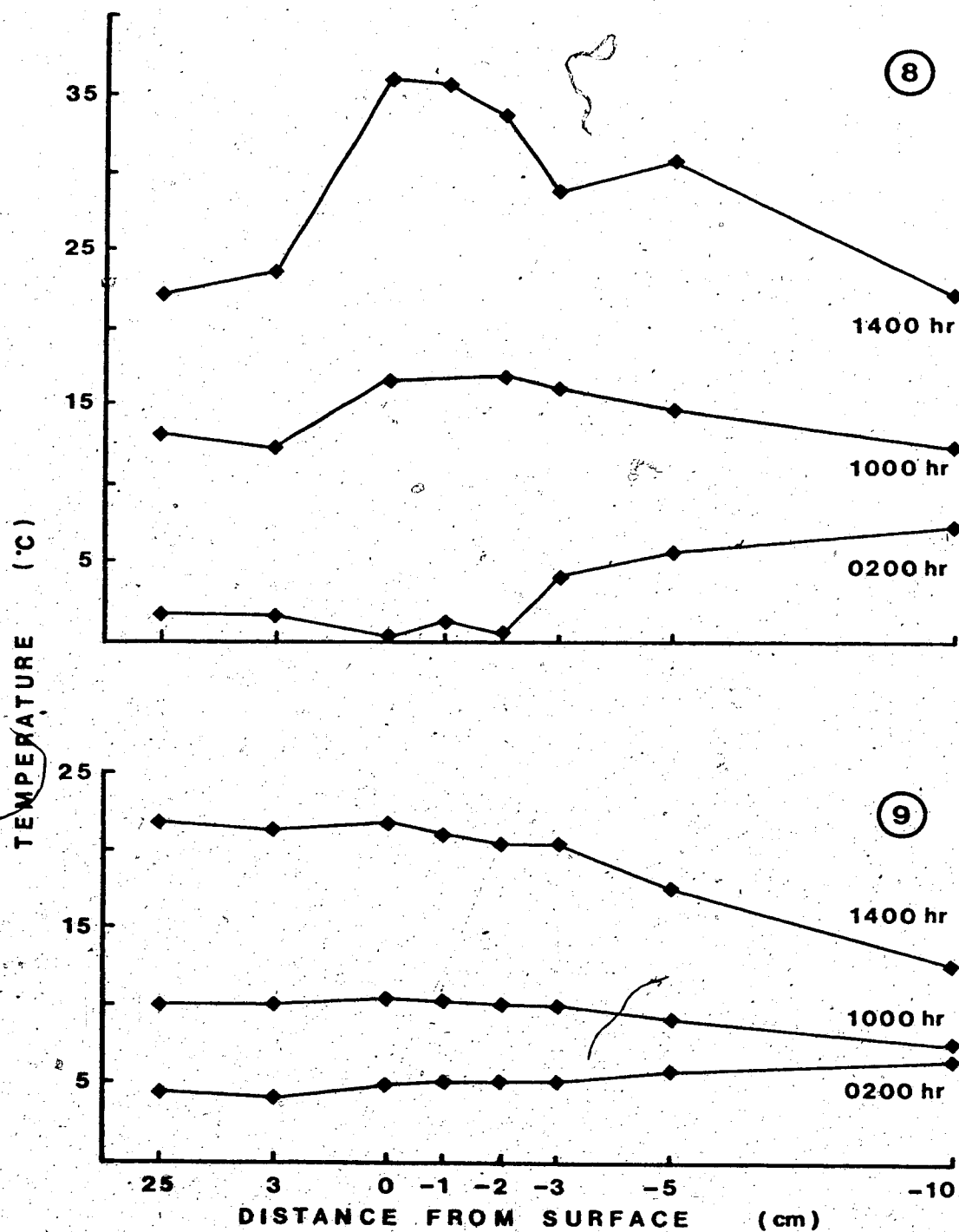
Figure 8. Selected air and moss temperature profiles at Tomenthypnum site, 31 July 1974.
