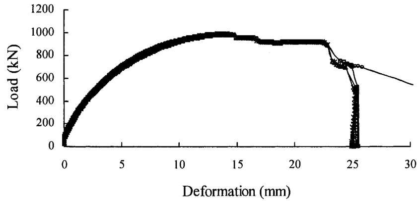
Figure C-18: Load vs. Deformation Curves for C18E1b
