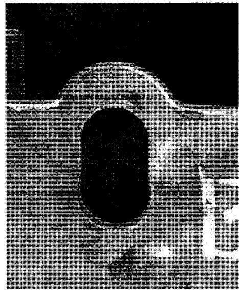
Figure 4-24: Ductility at a Hole (Specimen B5, unloaded at the peak)
