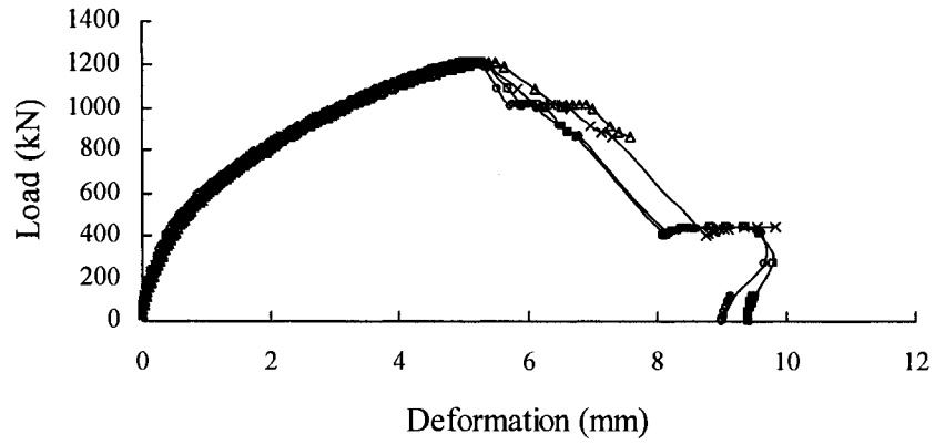
Figure C-10: Load vs. Deformation Curves for C10E4a
