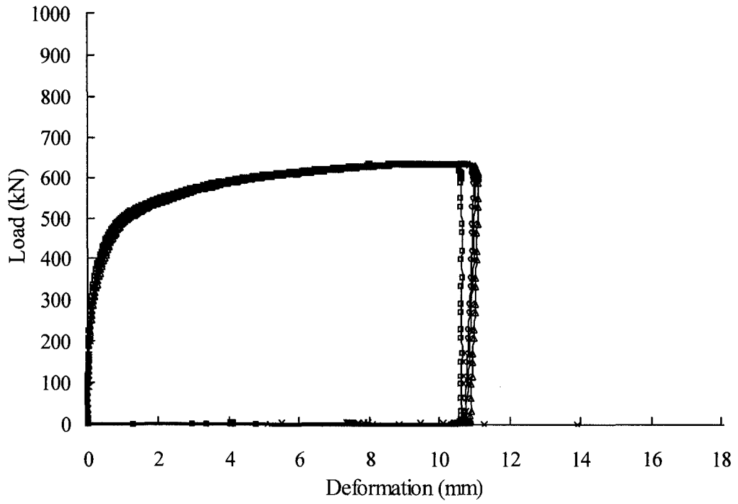
Figure 4-5: Load vs. Deformation Curve for A3R1
