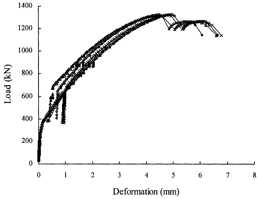
Figure C-16: Load vs. Deformation Curves for C16E6
