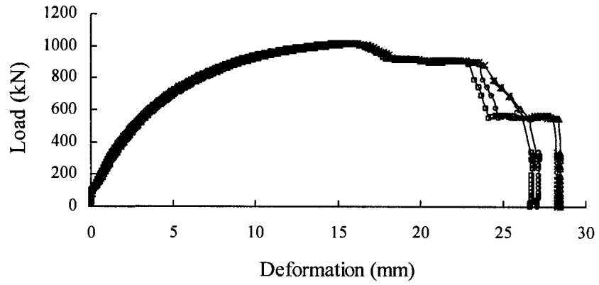
Figure C-20: Load vs. Deformation Curves for C20E2a
