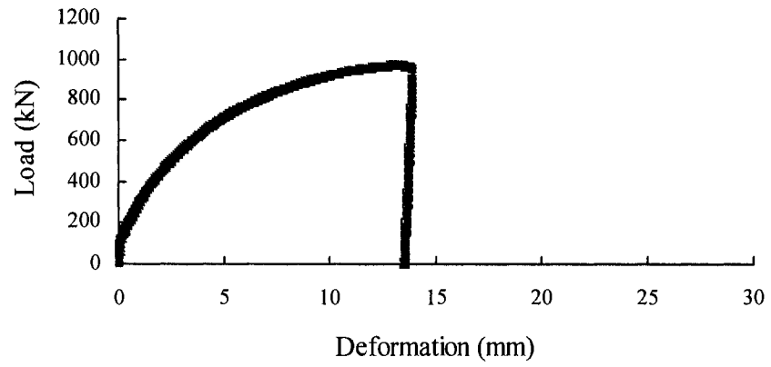
Figure C-17: Load vs. Deformation Curves for C17E1a
