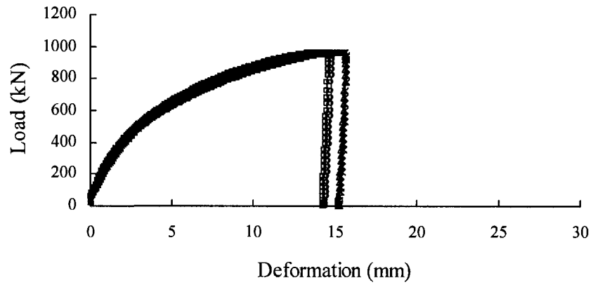
Figure C-21: Load vs. Deformation Curves for C21E2b
