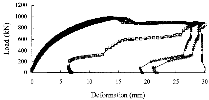
Figure C-22: Load vs. Deformation Curves for C22E2c
