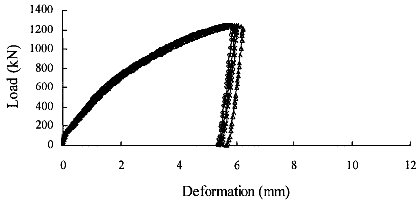
Figure C-11: Load vs. Deformation Curves for C11E4b
