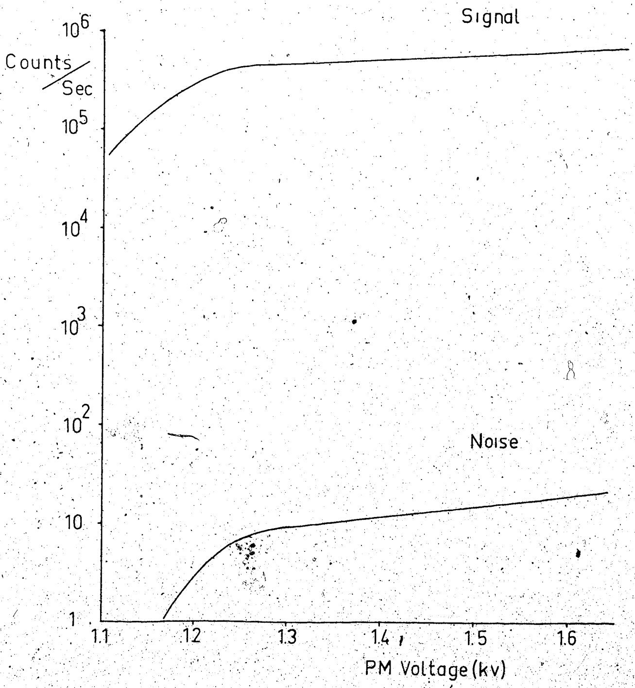
Fig 5-1 Output of EMI 9502S Photomultiplier
