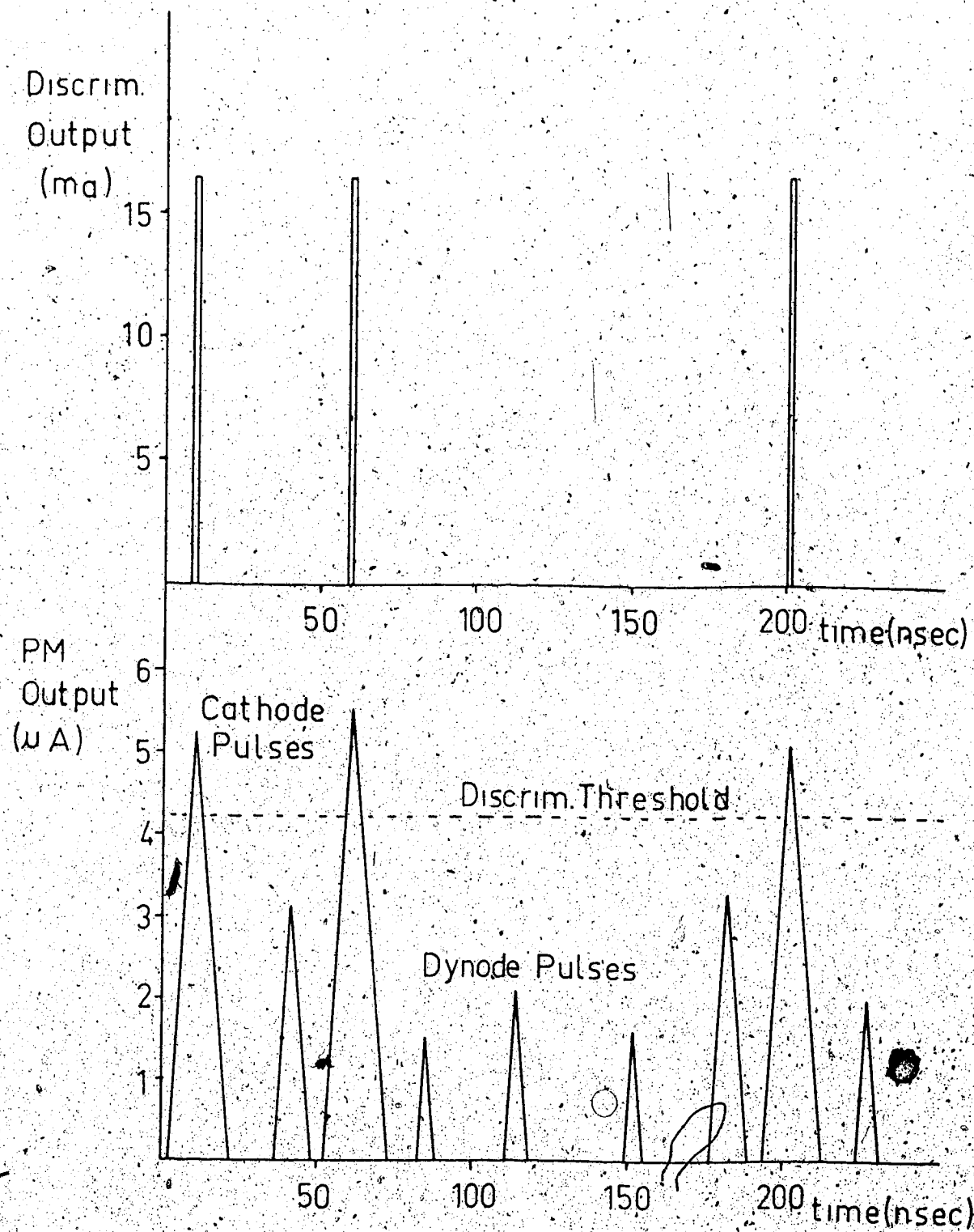
Fig 5-2 The Pulse Discrimination Process
