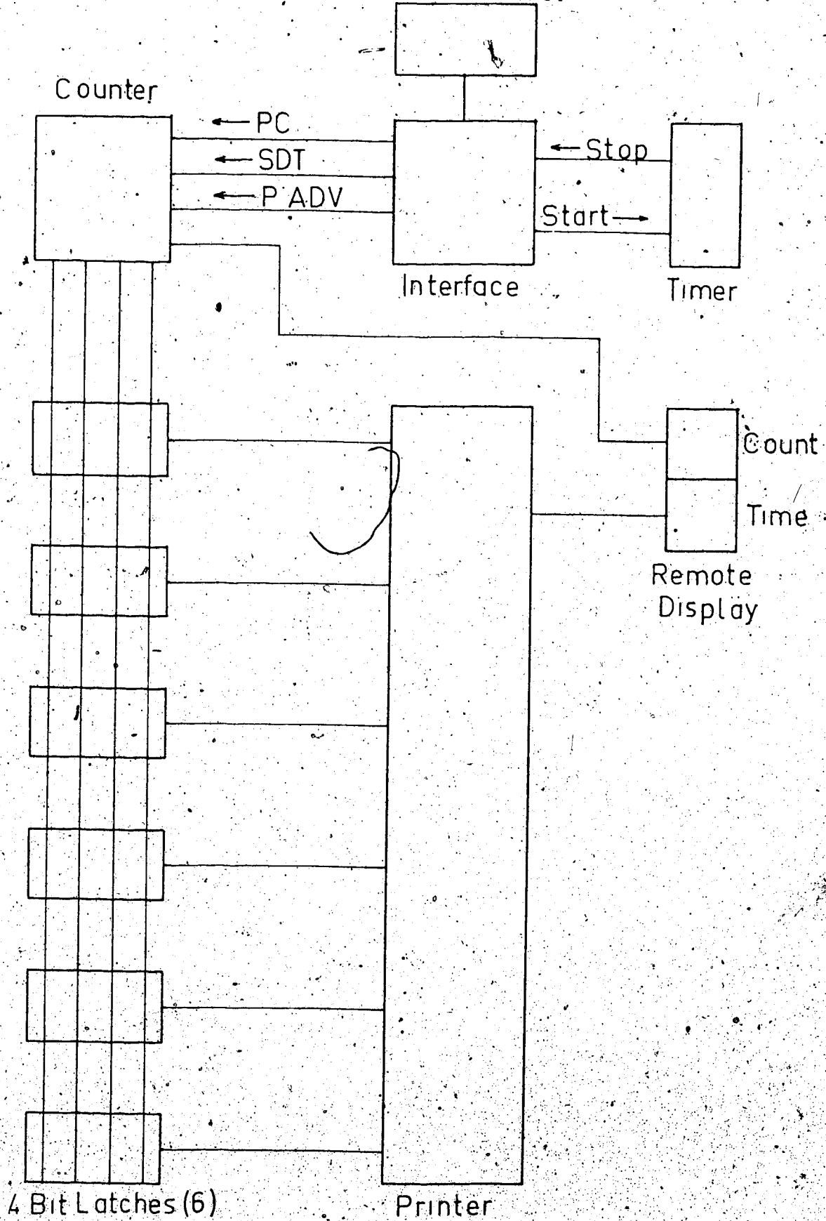
Fig 3-3 Electronic Block Diagram
