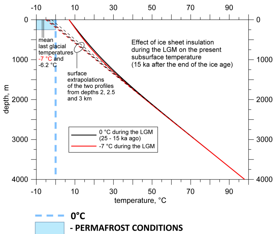
Fig. 2. Paleo-permafrost vs. synthetic T-z profiles (modified from Majorowicz and Safanda 2008) based on the ground surface temperature history shown for a homogeneous model with conductivity of 2\text{ W/(m K)} , diffusivity of 0.9\text{E}-6\text{ m}^2\text{s}^{-1} , typical tectonically stabilized continental heat flow of 50\text{ mWm}^{-2} . They correspond to the time 15 ka after the end of the last ice age and differ due to different surface temperatures, -7^{\circ}\text{C} or 0^{\circ}\text{C} , during the LGM 25–15 ka ago. Also shown are upward steady-state extrapolations of the two profiles from depths of 2, 2.5 and 3 km, respectively. These all point to sub-zero temperature conditions and some 150 m-thick permafrost for the model assumed
