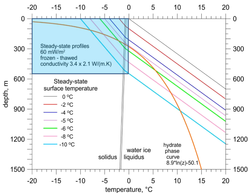
Fig. 3. Maximum thickness of paleo-permafrost for temperature-depth profiles constrained by 0- (-10) °C surface conditions. Theoretical steady-state profiles for the geothermal model in which heat flow is assumed 60mWm -2 (typical for thermal results in the Polish deep sedimentary basin in places like the Toruń-1 well location (Majorowicz and Safanda 2009; discussed further). Conductivity of the frozen and thawed rock is assumed to be 3.4 and 2.1Wm -1 K -1 respectively, modified from Majorowicz et al. (2012). The depth of permafrost for the -10°C sub-glacial ice surface will reach a thickness of 550 m (box area). The stability of hydrate (CH 4 ) is also shown to illustrate that warming and pressure after glacial retreat can result in destabilizing greenhouse gas CH 4 from gas hydrate within permafrost and/or below (more likely to occur) in sedimentary rocks under paleo-glacial
