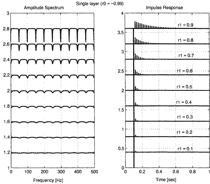
Figure 3.5: Amplitude spectrum for the impulse response of a single layer system as the one presented in figure 3.4. Case 1 : reflection coefficients at the interfaces have opposite signs.
