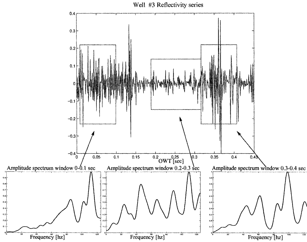
Figure 2.6: Reflectivity series and windowed amplitude spectrum corresponding to cyclic and transitional impedance layering for Well 3 from the WCB.
