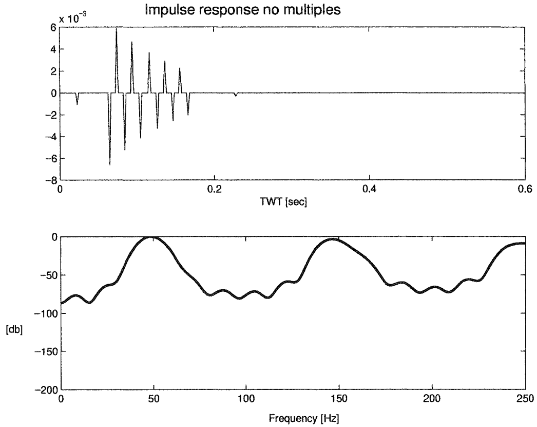
Figure 3.9: Top: impulse response with transmission loss but no multiples. Bottom: corresponding amplitude spectrum.
