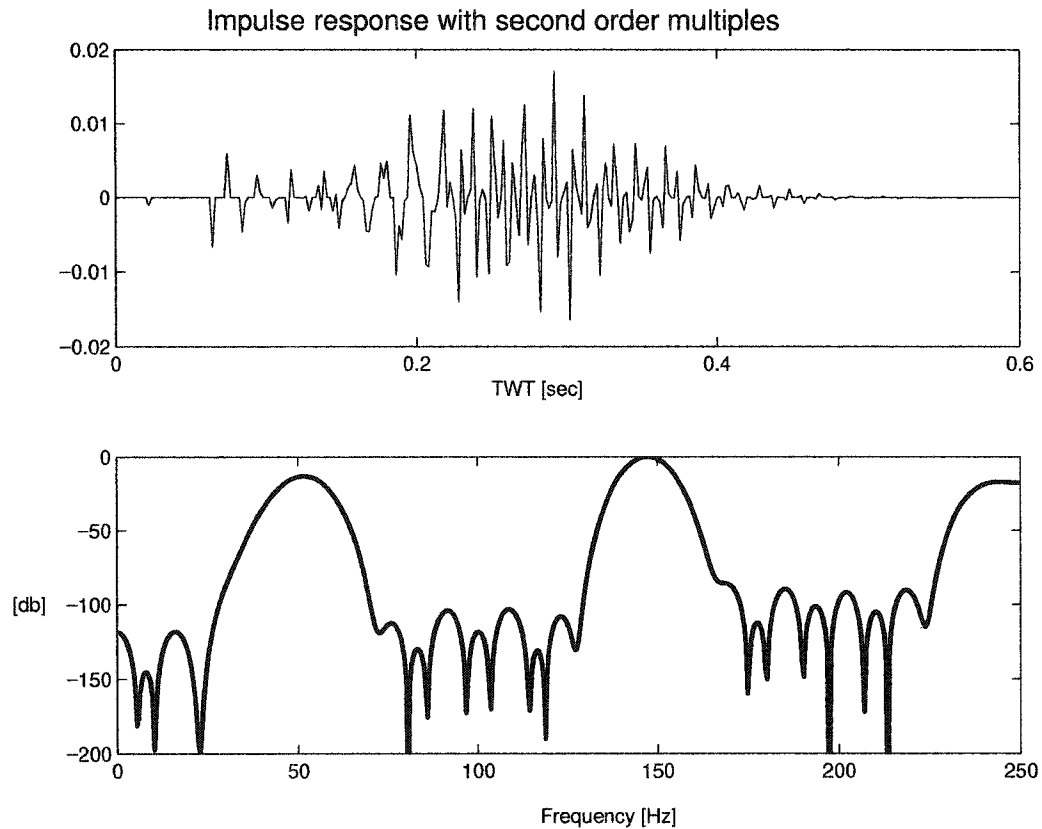
Figure 3.11: Top: impulse response with transmission loss and with 2nd order multiples. Bottom: corresponding amplitude spectra.
