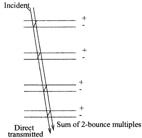
Figure 3.3: The cumulative effect of the multiple reflections for a sequence of thin layers.
