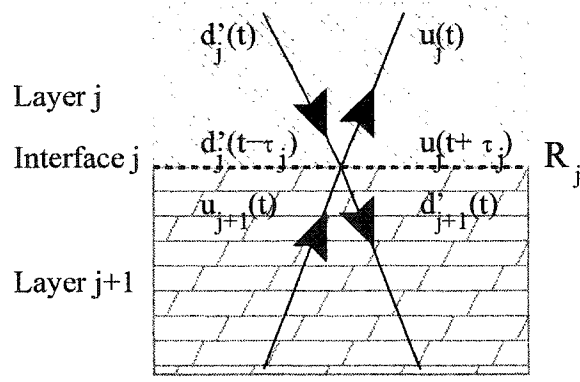
Figure 5.4: Reflected and transmitted waves at interface j .
