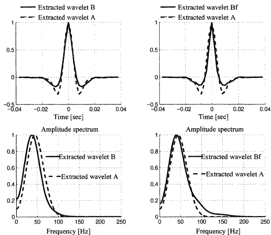
Figure 4.12: Top left: extrated wavelet B from data below the transmission filter. Bottom left: amplitude spectrum of the extracted wavelet B overlying amplitude spectrum from extracted wavelet A (Above transmission filter). Top right:extrated wavelet Bf from data below the transmission filter, after compensatory filter. Bottom right: amplitude spectrum of the extracted wavelet Bf, overlying amplitude spectrum from extracted wavelet A.
