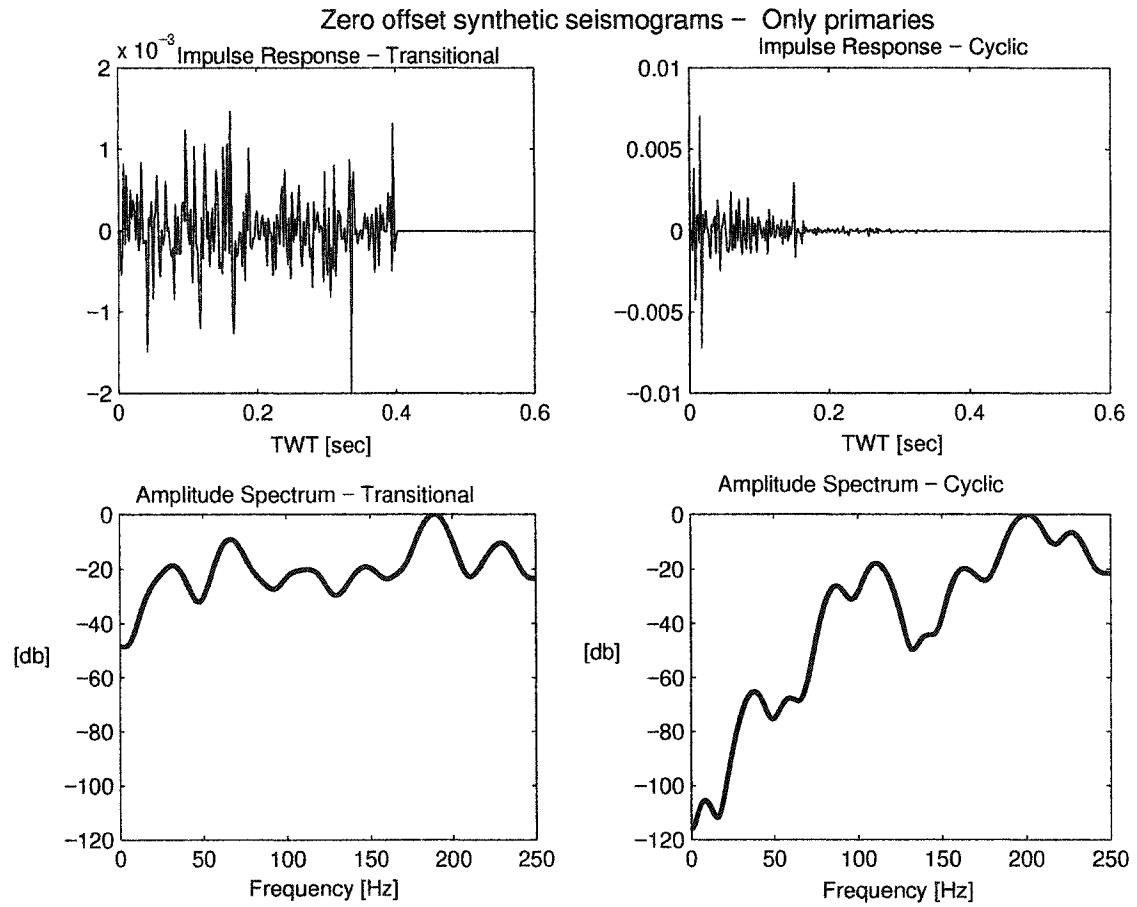
Figure 3.13: Top: impulse response with transmission loss and no multiples for a transitional and cyclic reflectivity sequences. Bottom: corresponding amplitude spectra.
