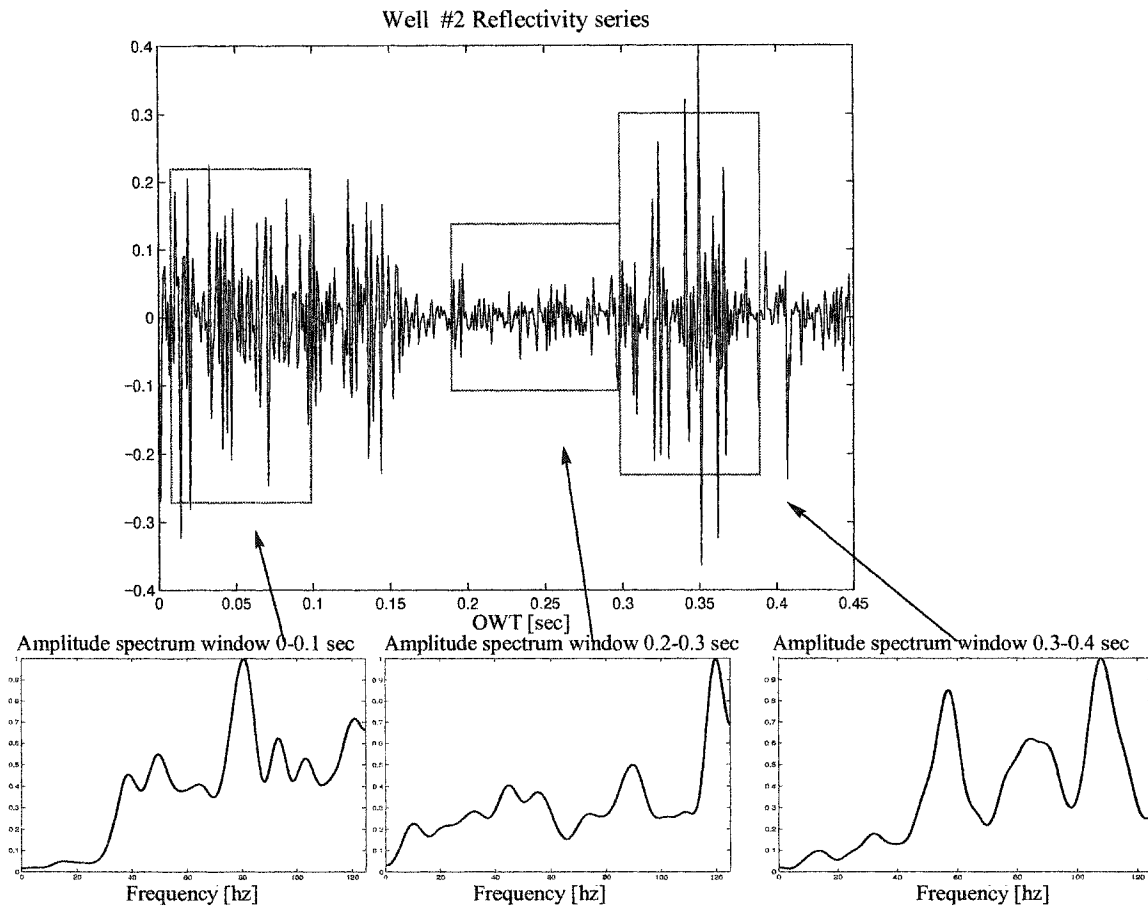
Figure 2.5: Reflectivity series and windowed amplitude spectrum corresponding to cyclic and transitional impedance layering for Well 2 from the WCB.
