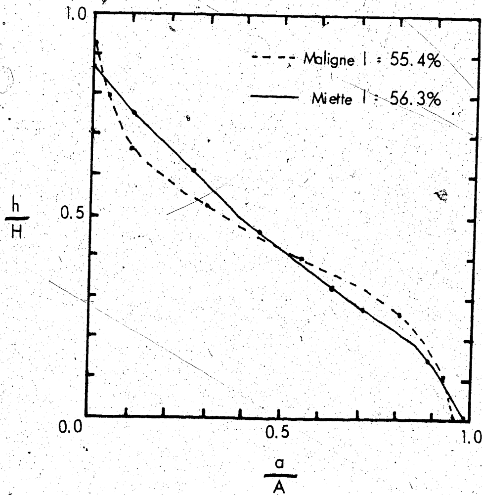
Figure 26 Hypsometric Curves of the Maligne and Miette Basins
