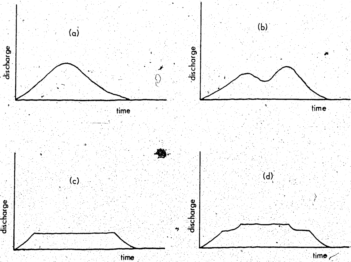
Figure 24 Model Hydrographs for Subsurface Flow in Limestone Terrain
