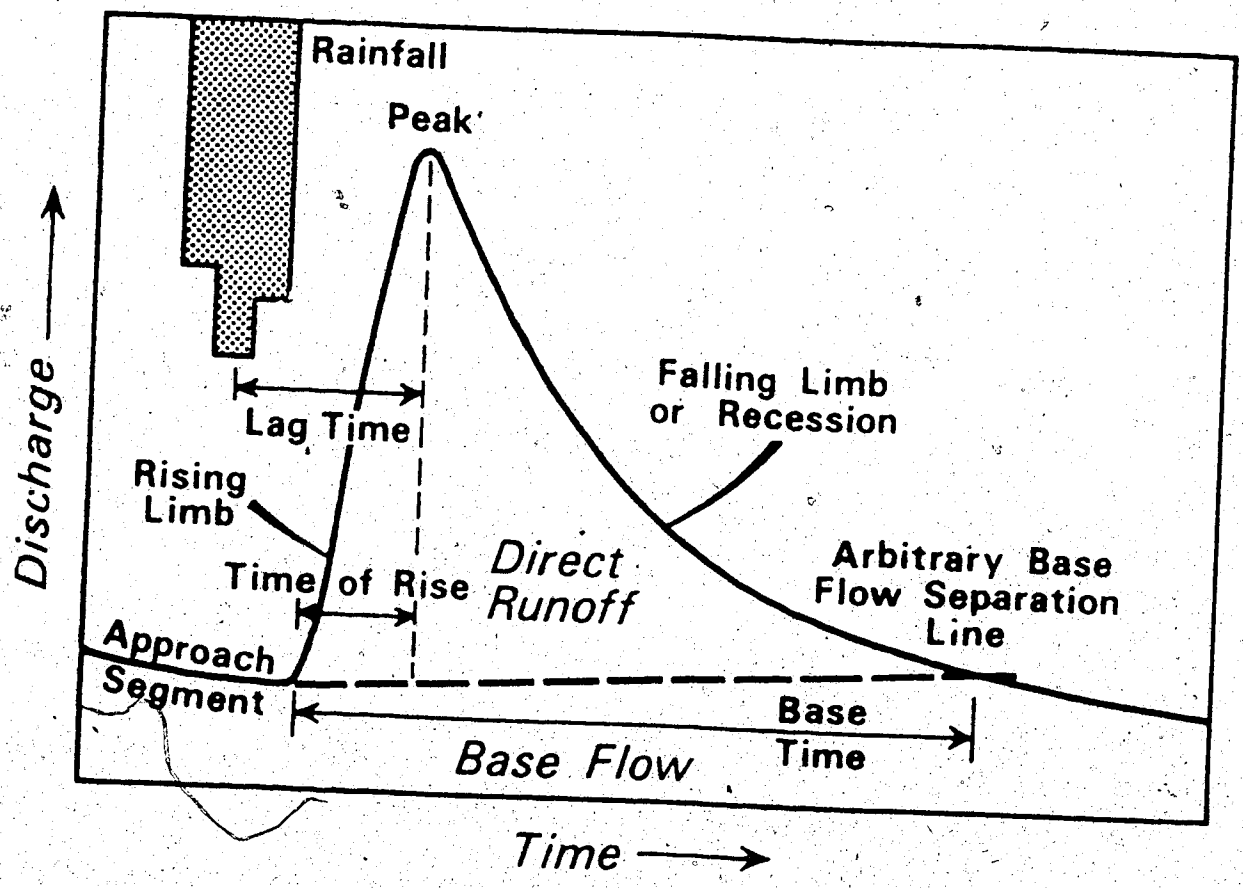
Figure 18 Characteristics of a Storm Hydrograph Source: Gregory and Walling, 1973
