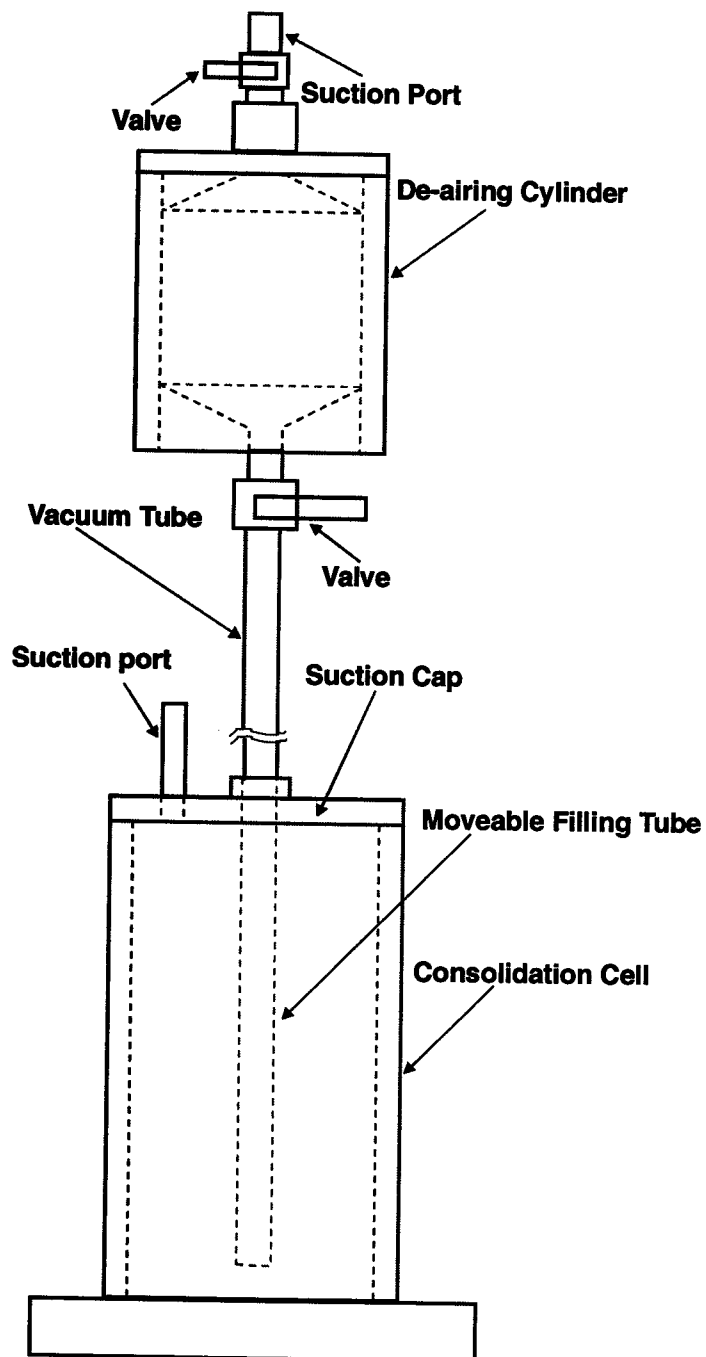
Figure 3.4 Tailings placement technique
