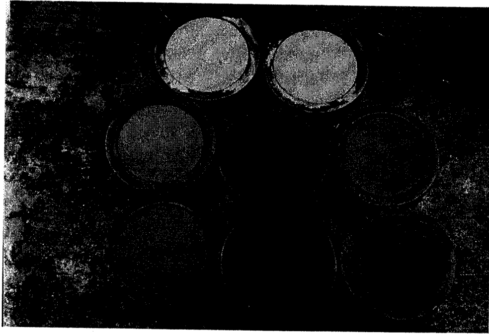
Figure 3.15 Shrinkage test specimens and dishes
