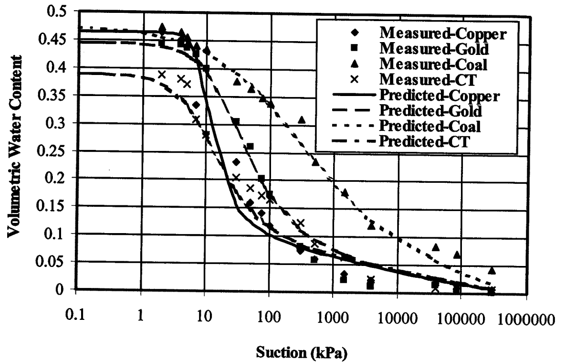
Figure 5.6 A comparison between the measured soil-water retention curves and those predicted by Fredlund's model
