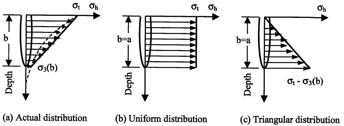
Figure 6.7 Assumptions of the tensile stress distributions
