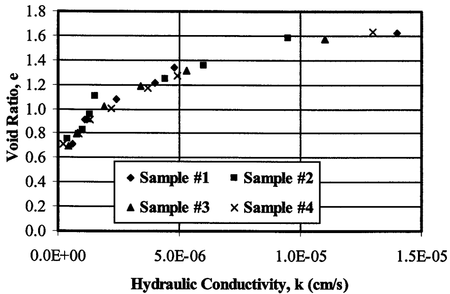
Figure B. 6 Void ratio versus hydraulic conductivity curve for coal tailings
