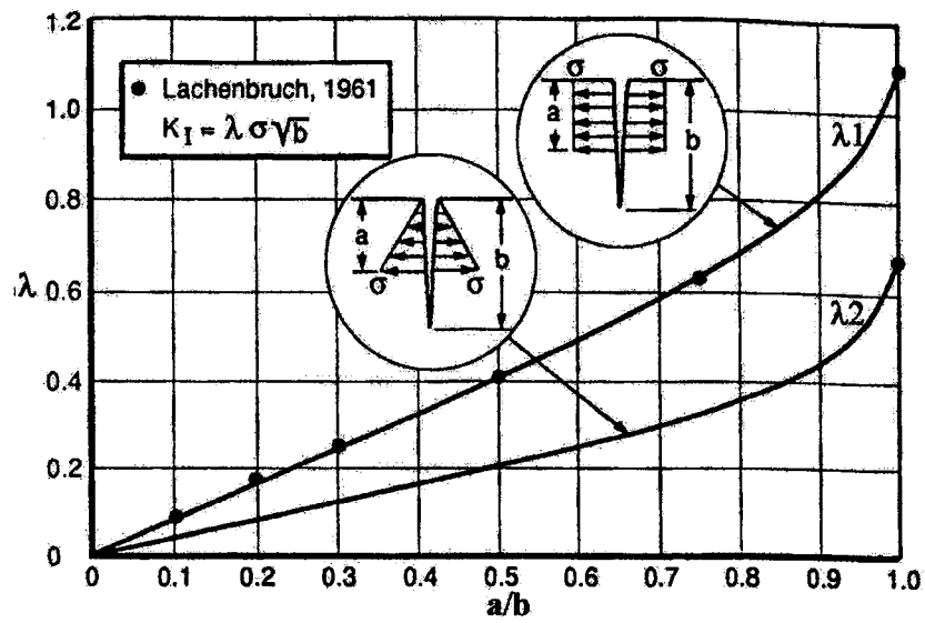
Figure 2.10 Stress intensity functions for uniform and linear stress distribution (modified from Konrad et al. 1997)
