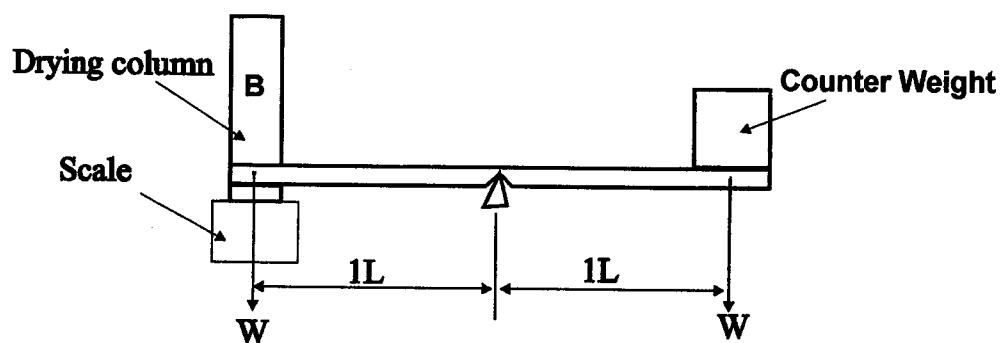
Figure 3.9 Beam system used to accurately weigh 20 kg sample
