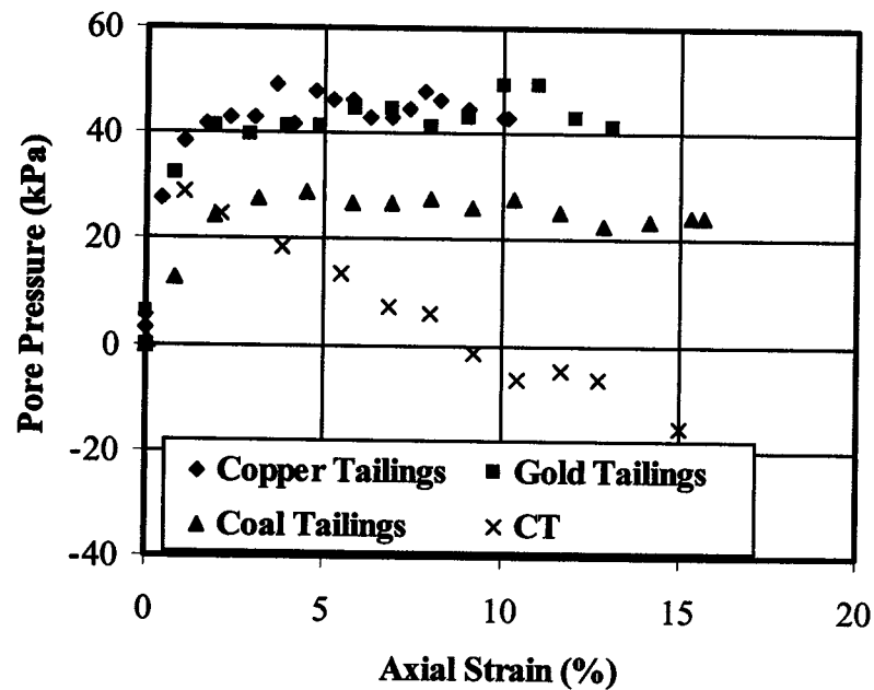
Figure 4.17 Pore pressure change versus strain plot after 50 kPa consolidation
