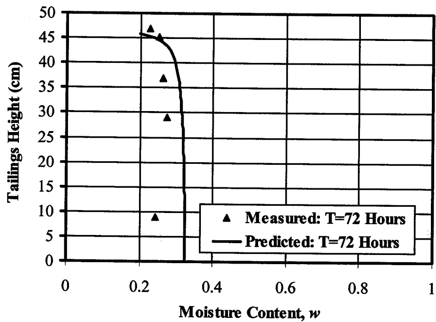
Figure 7.6 Measured and predicted moisture content profile of gold tailings in drying test
