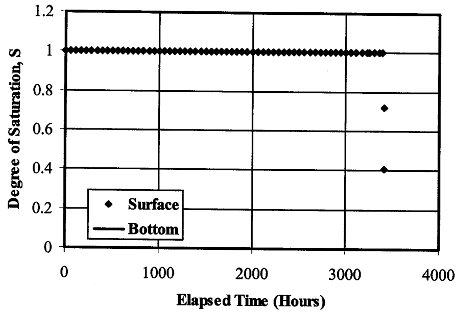
Figure 7.19 Degree of saturation change in CT
