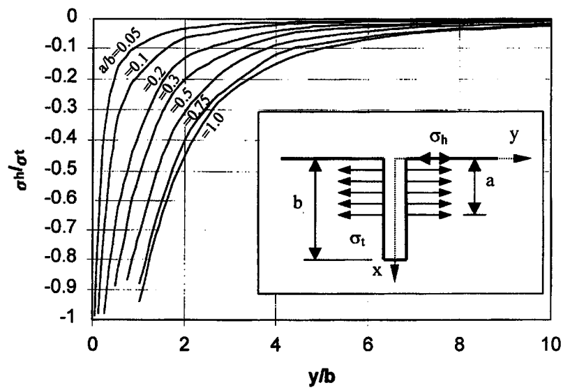
Figure 2.8 Theoretical values of elastic stress relief due to a vertical crack (modified from Lachenbruch 1962)
