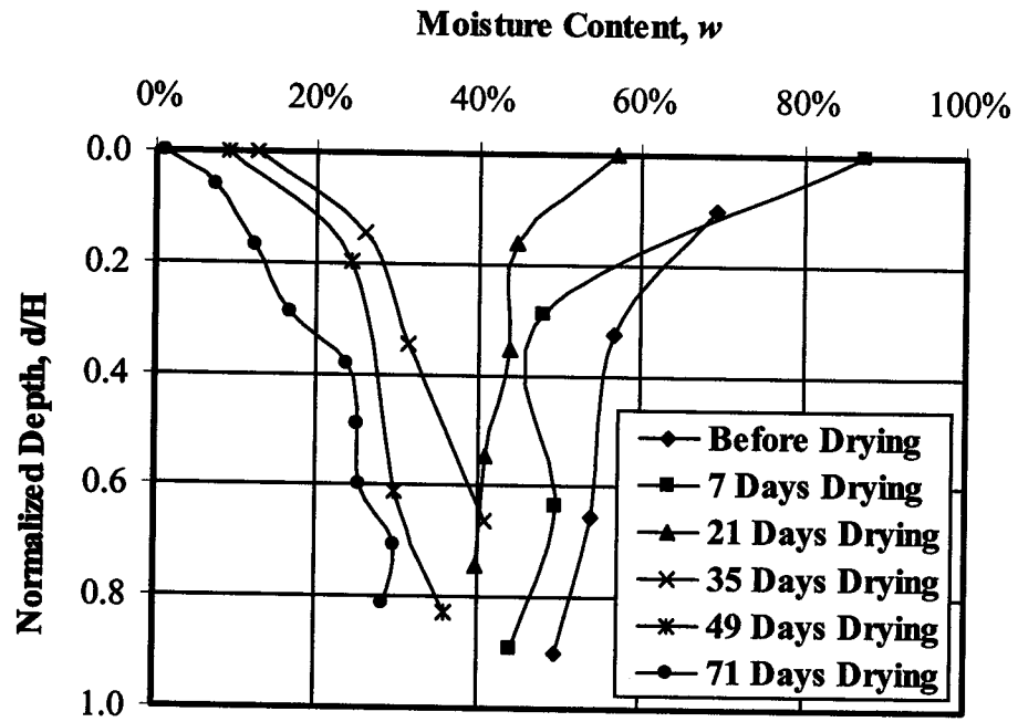
Figure 4.14 Moisture profile changes of CT
