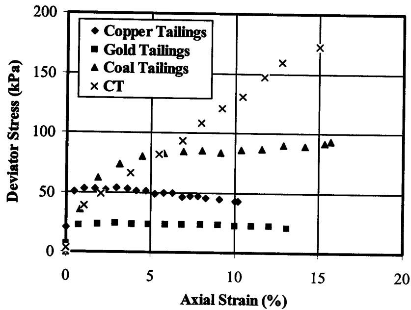
Figure 4.16 Deviator stress versus strain plot after 50 kPa consolidation
