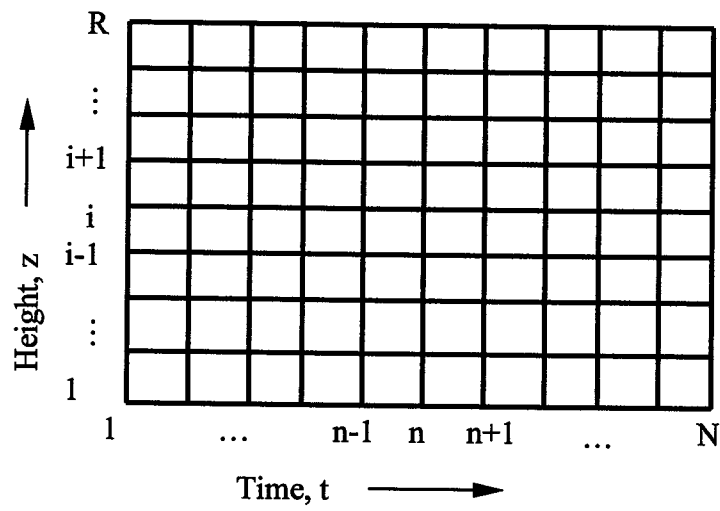
Figure 5.9 Finite difference mesh
