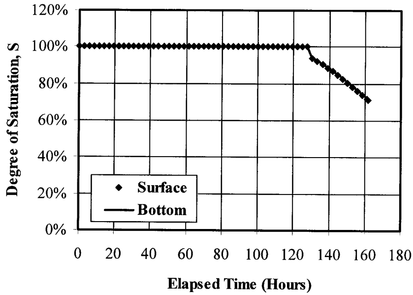
Figure 7.30 Degree of saturation in one-day operation for case history #1
