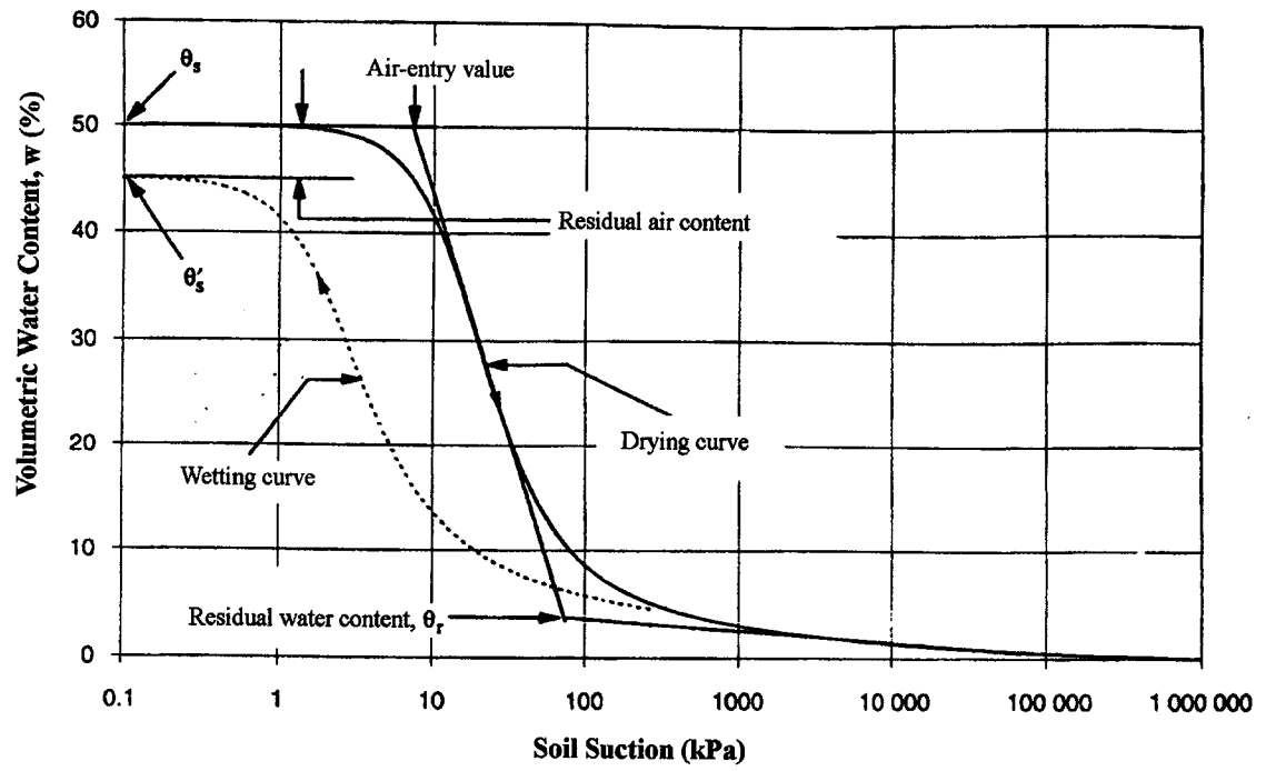
Figure 2.5 Typical water-soil characteristic curves (modified from Fredlund et al. 1994)
