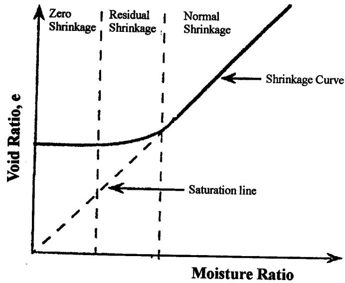
Figure 2.6 Typical shrinkage curve of soils
