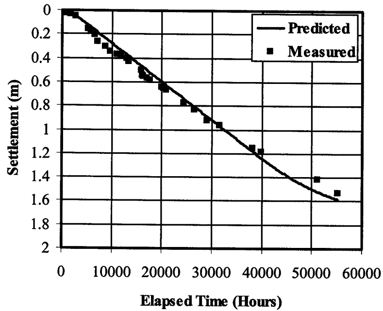
Figure 7.1 Measured and predicted settlement in a Ten Meter Standpipe
