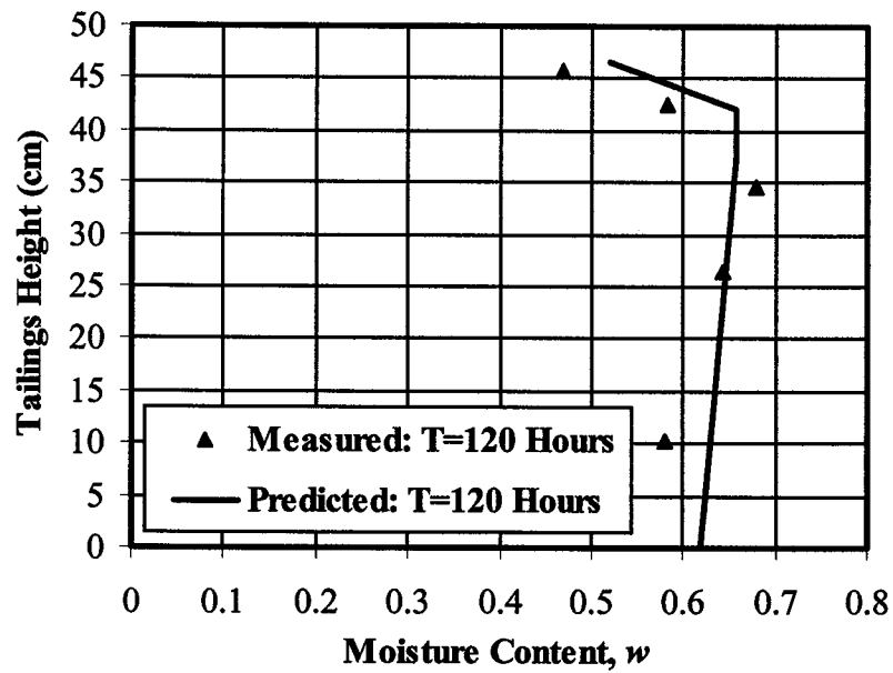
Figure 7.8 Measured and predicted moisture content profile of coal tailings in drying test
