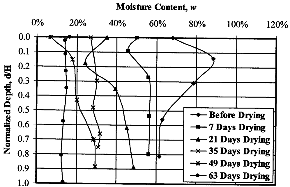
Figure 4.13 Moisture profile changes of coal tailings
