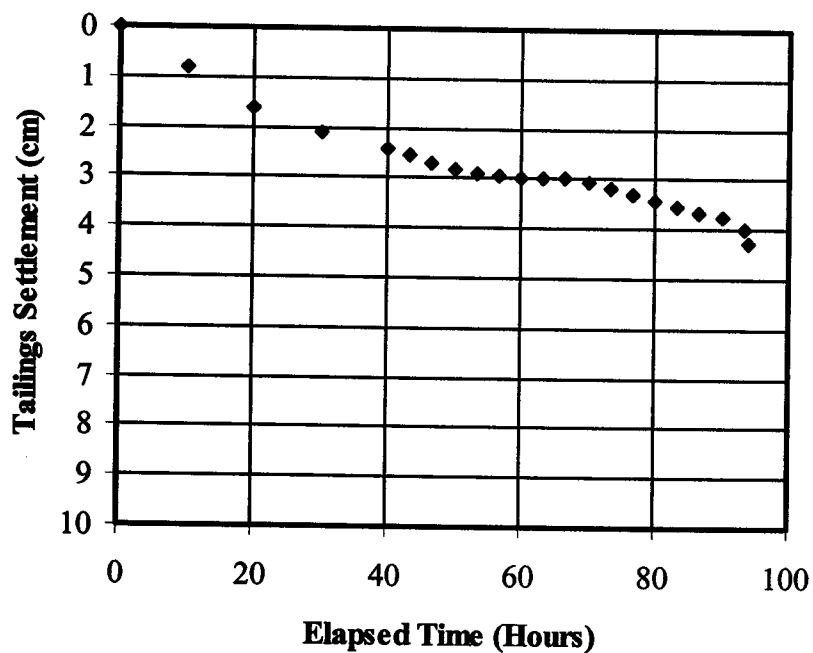
Figure 7.14 Predicted single layer settlement of the coal tailings at cracking
