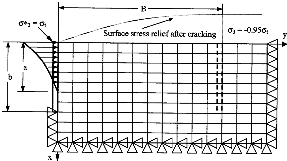
Figure 6.8 Use fictitious stress principle to determine tensile stress reduction (modified from Konrad and Ayad 1997)
