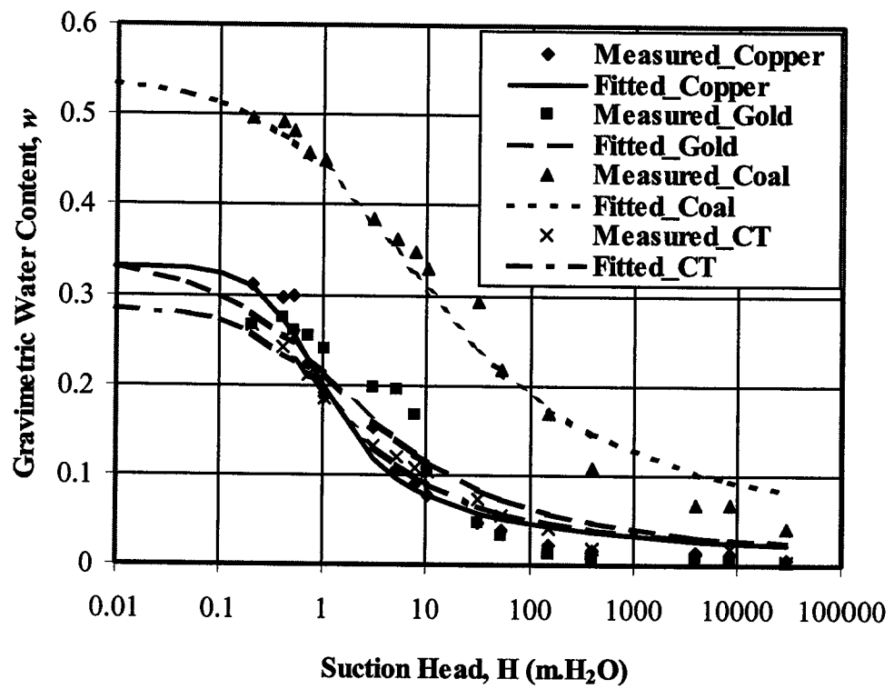
Figure 4.6 Measured and fitted water retention curves for tailings
