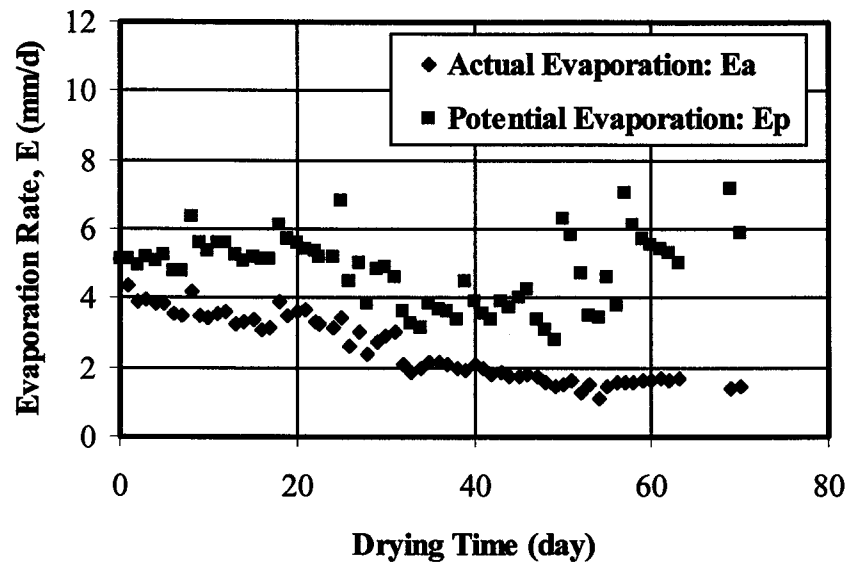
Figure B. 16 Evaporation changes in column drying tests for CT
