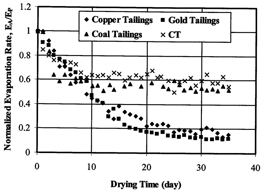
Figure 4.8 Normalized evaporation rate of mine tailings
