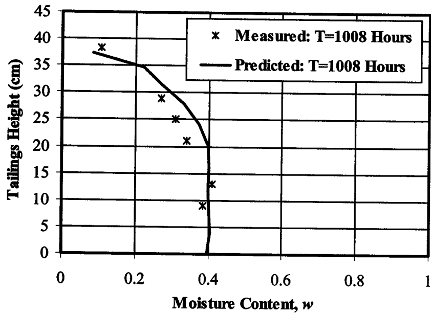
Figure 7.10 Measured and predicted moisture content profile of CT in drying test
