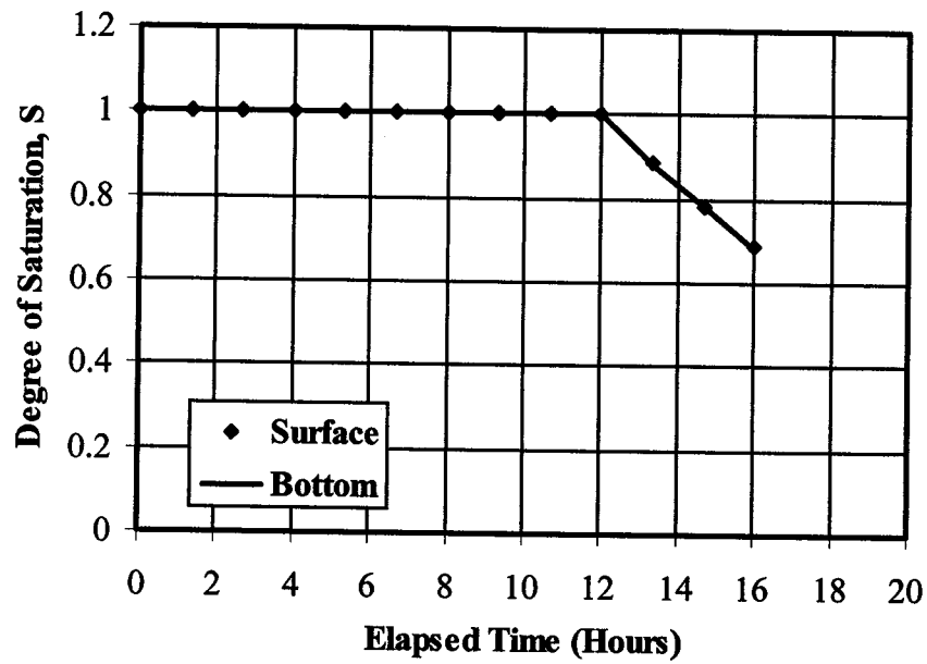
Figure 7.17 Degree of saturation change in gold tailings
