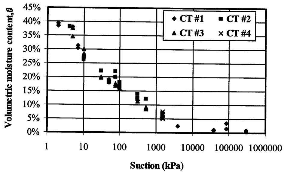
Figure B. 20 Soil-water retention curve test results for CT
