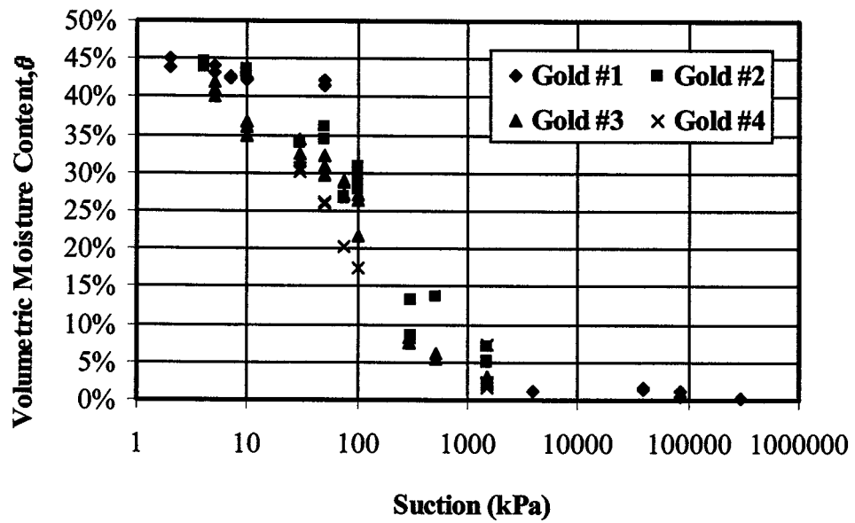
Figure B. 18 Soil-water retention curve test results for gold tailings
