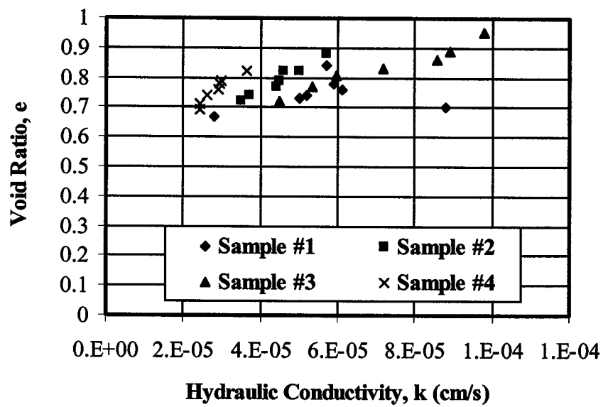
Figure B. 2 Void ratio versus hydraulic conductivity curve for copper tailings
