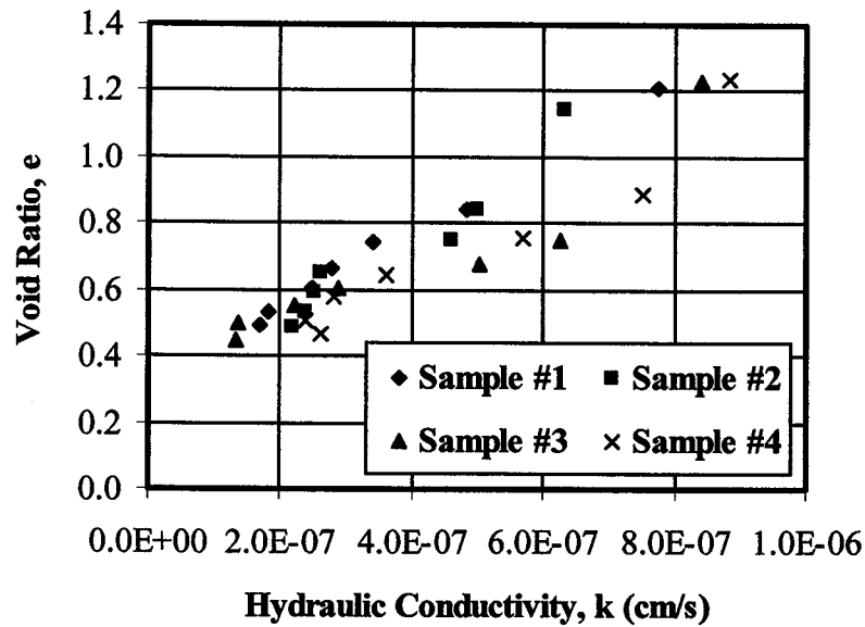
Figure B. 8 Void ratio versus hydraulic conductivity curve for oil sand CT
