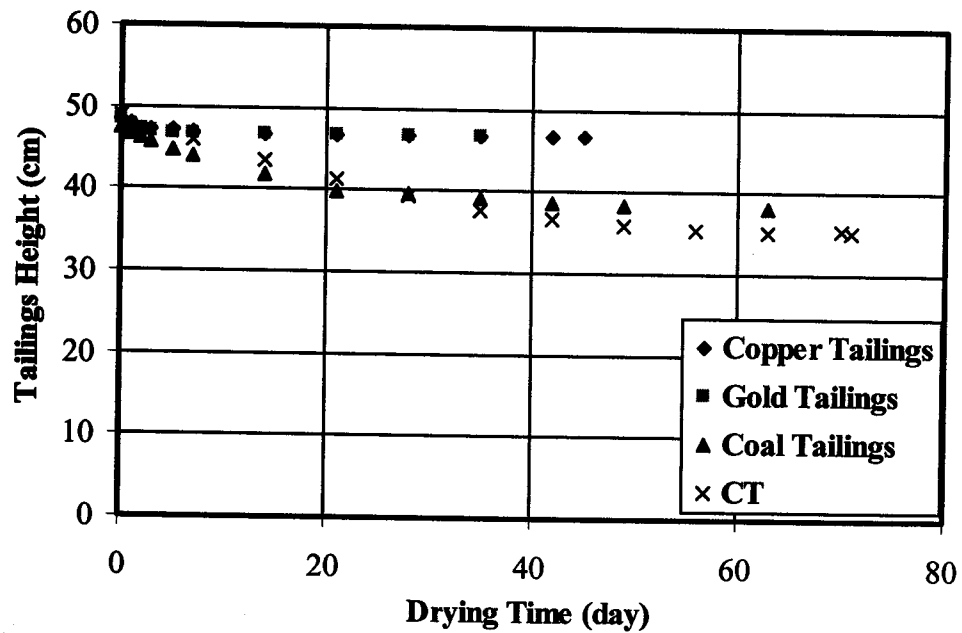
Figure 4.15 Specimen height changes of different tailings
