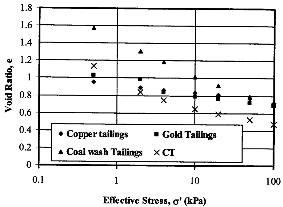
Figure 4.2 Compressibility of tailings
