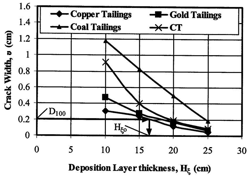
Figure 7.11 Relationship between crack width and layer thickness
