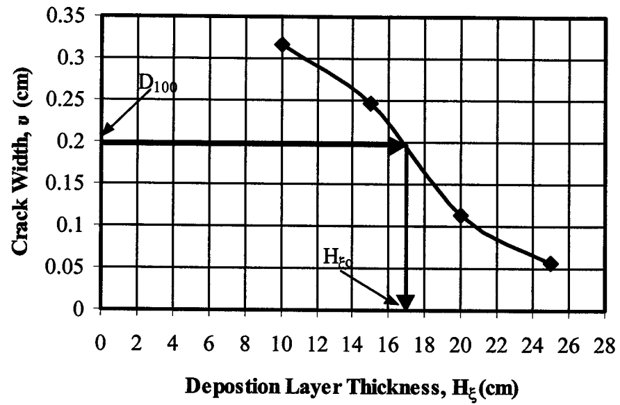
Figure 7.28 Optimum design curve for case history #3
