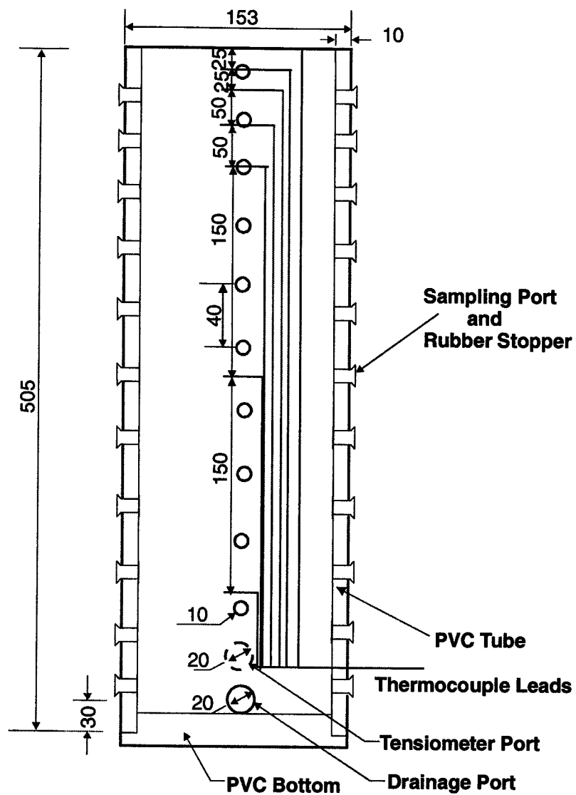
Figure 3.7 Drying column (modified from Wilson 1990)
