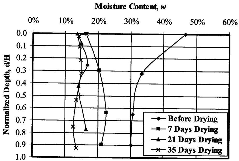
Figure 4.12 Moisture profile changes of gold tailings
