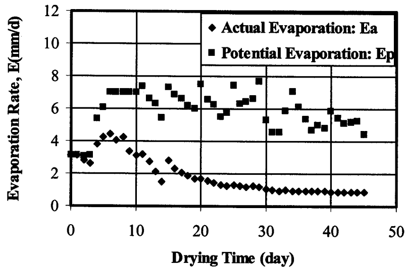
Figure B. 10 Evaporation changes in column drying tests for copper tailings
