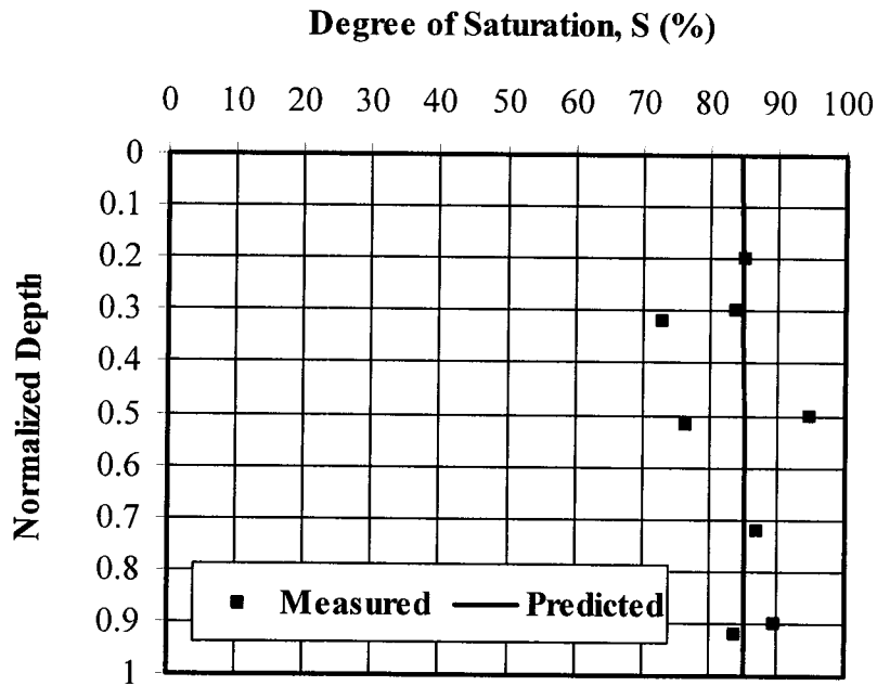
Figure 7.31 Measured and predicted degree of saturation in case history #1
