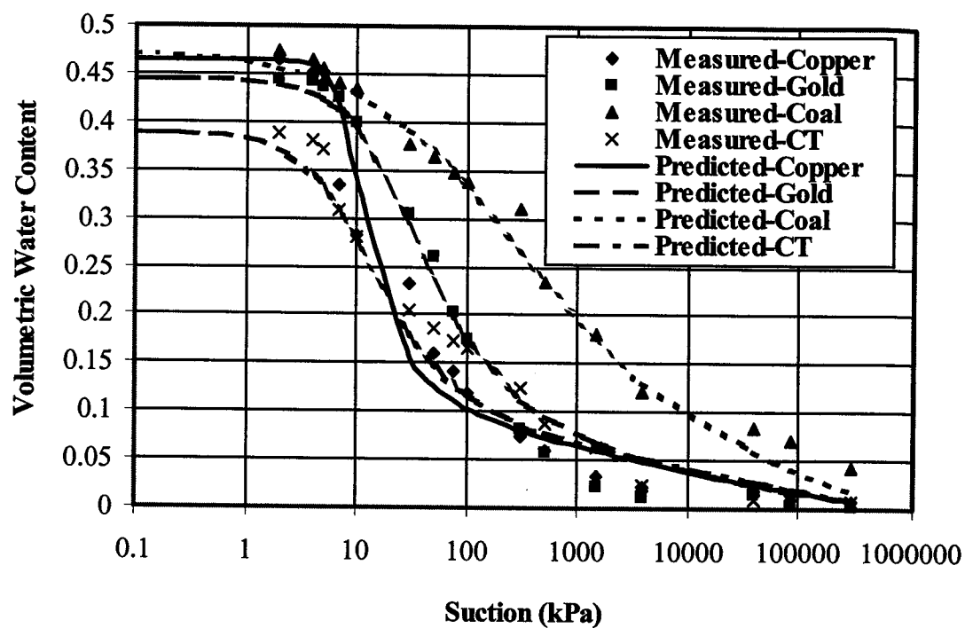
Figure 4.5 Measured and predicted soil-water retention curves of tailings
