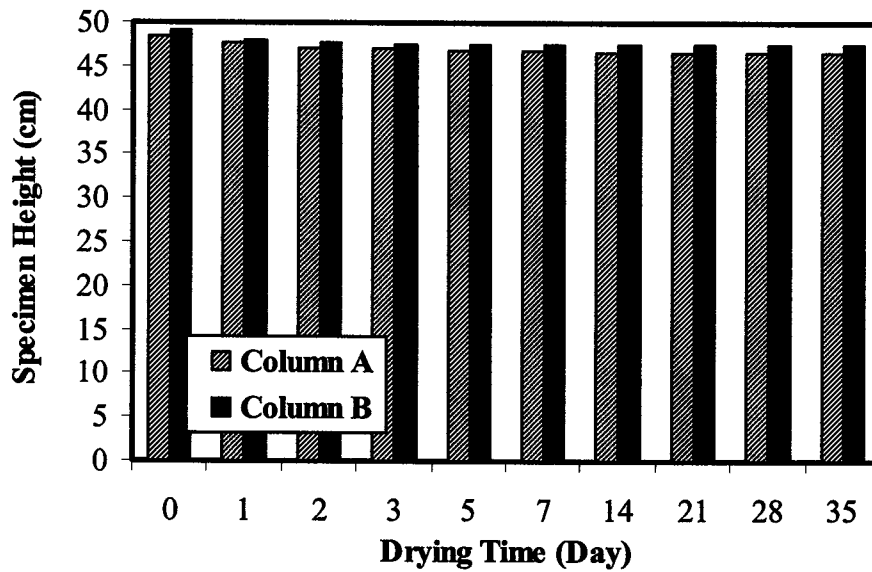
Figure B. 11 Specimen height changes in column drying tests for gold tailings
