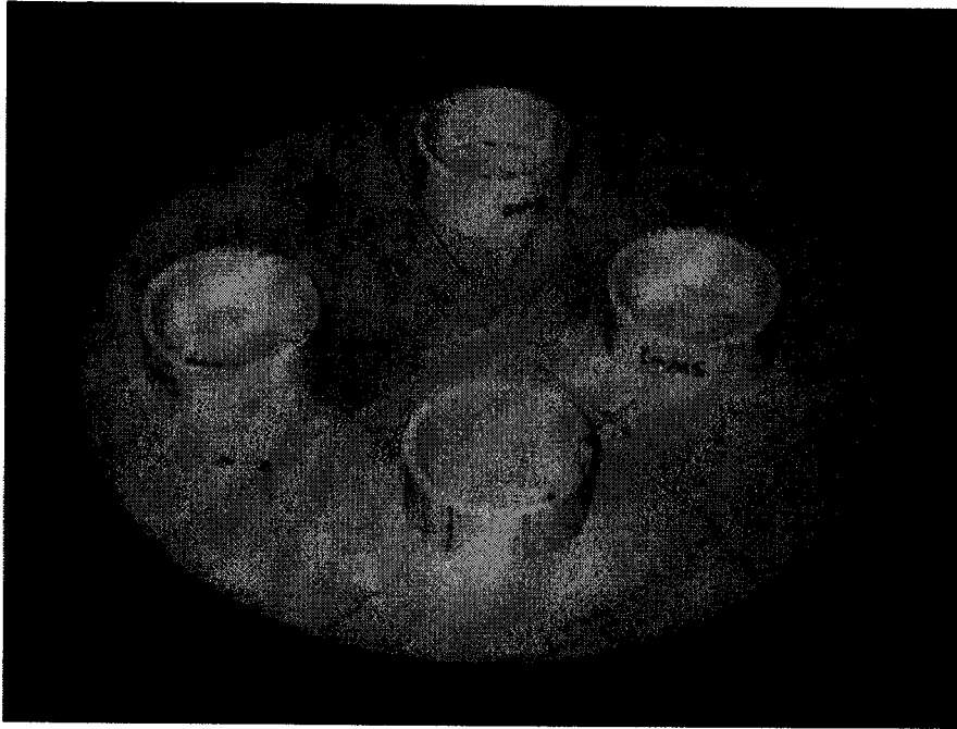
Figure 3.11 Sample retainer ring and porous ceramic plate
