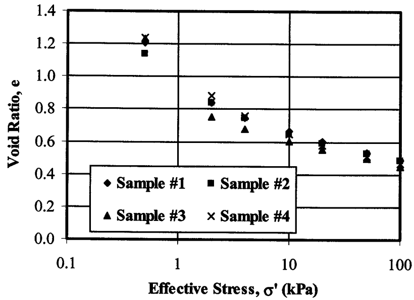
Figure B. 7 Compressibility of CT
