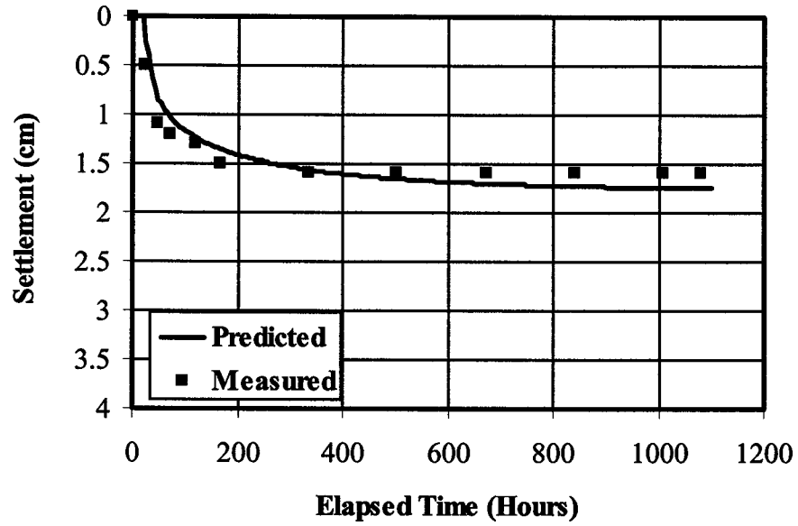
Figure 7.3 Measured and predicted settlement of copper tailings in drying test
