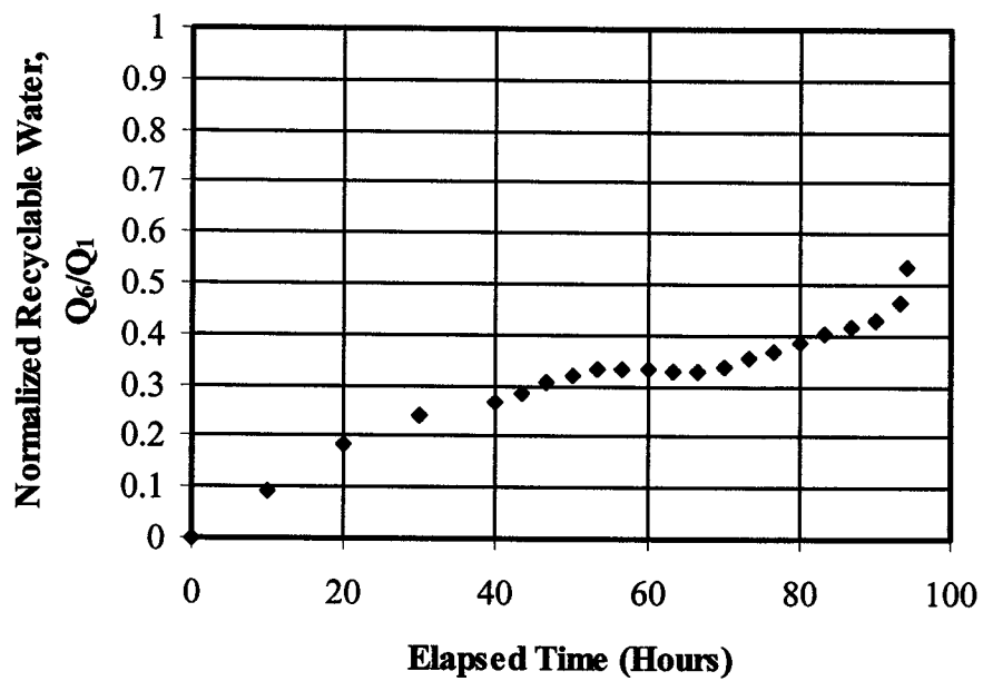
Figure 7.22 Normalized recyclable water in coal tailings
