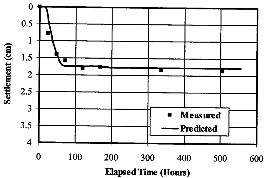
Figure 7.5 Measured and predicted settlement of gold tailings in drying test
