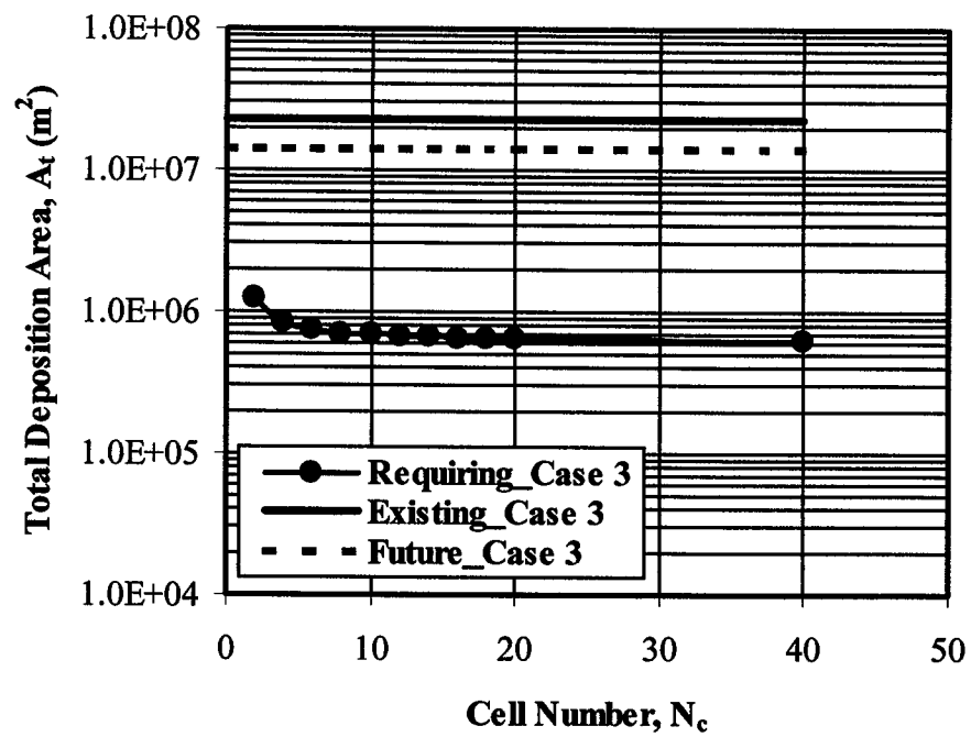
Figure 7.29 Deposition area versus cell number plot for case history #3
