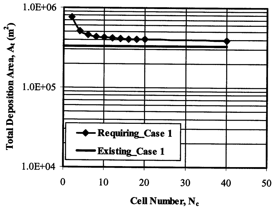
Figure 7.25 Deposition area versus cell number plot for case history #1
