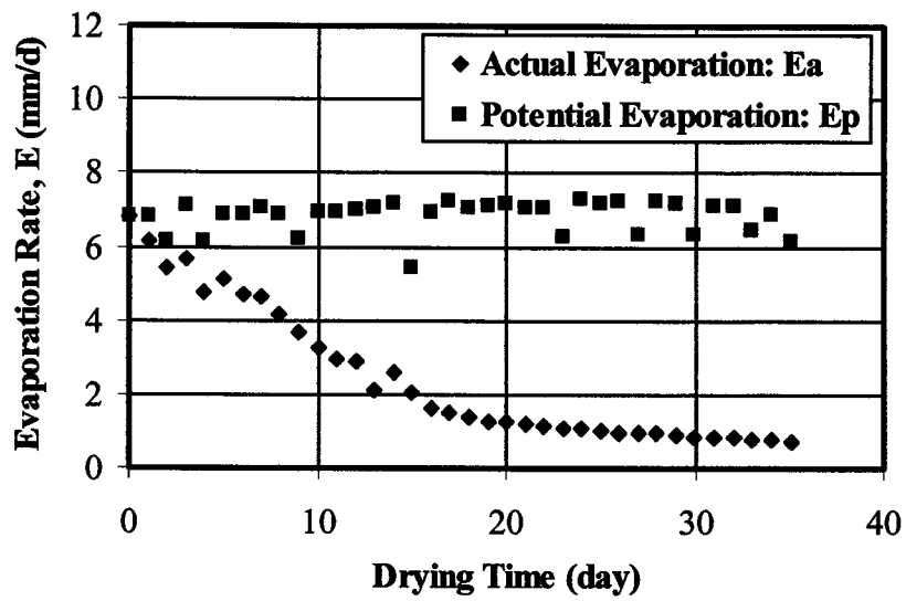
Figure B. 12 Evaporation changes in column drying tests for gold tailings
