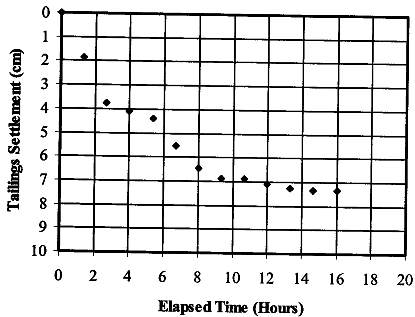
Figure 7.13 Predicted single layer settlement of the gold tailings at cracking
