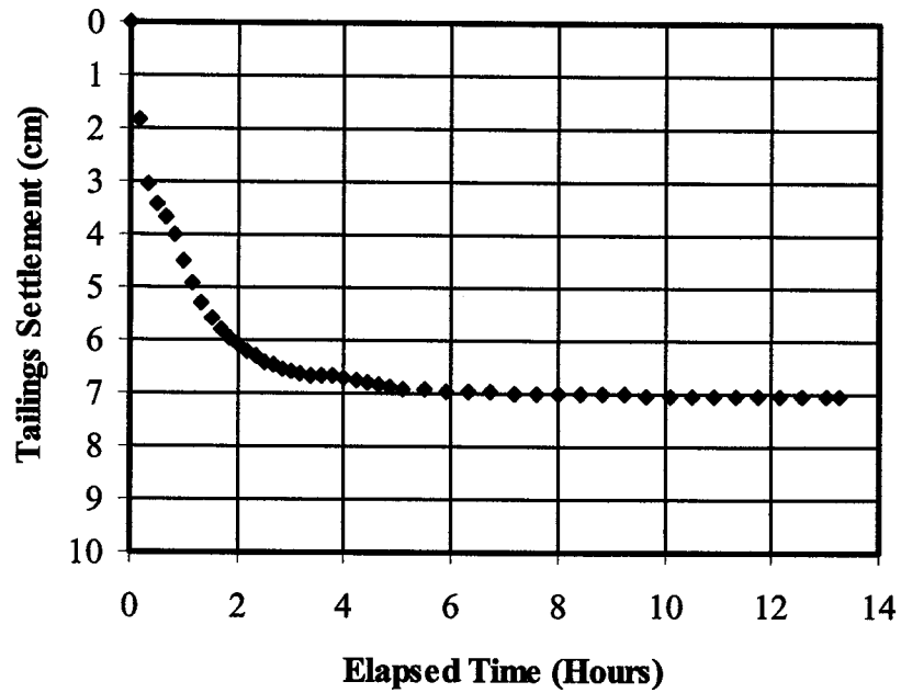
Figure 7.12 Predicted single layer settlement of the copper tailings at cracking
