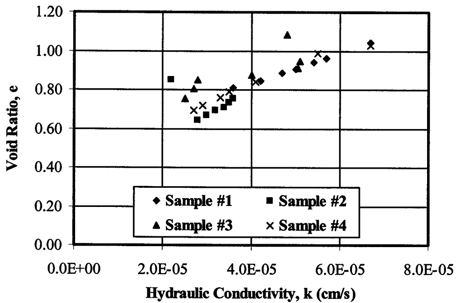
Figure B. 4 Void ratio versus hydraulic conductivity curve for gold tailings
