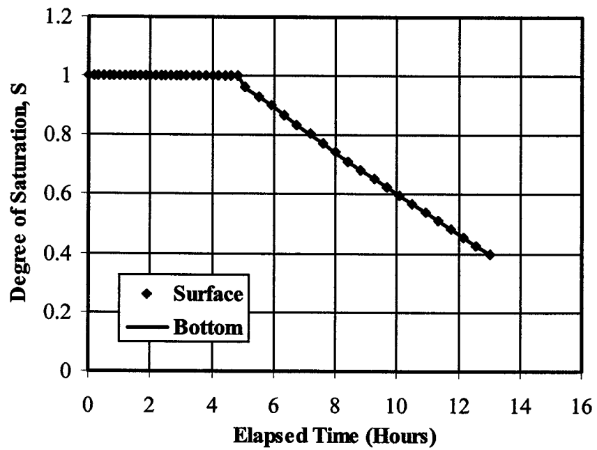
Figure 7.16 Degree of saturation change in copper tailings
