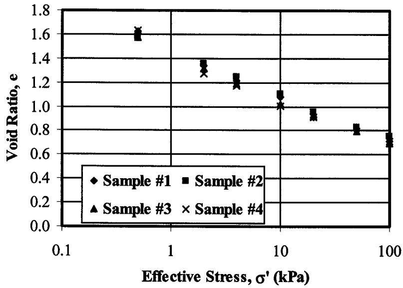
Figure B. 5 Compressibility of coal tailings
