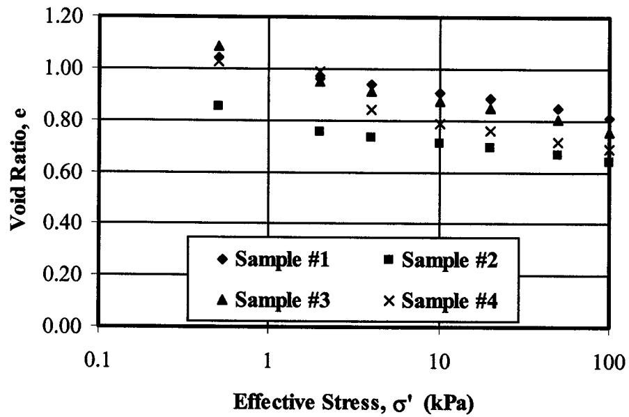
Figure B. 3 Compressibility of gold tailings
