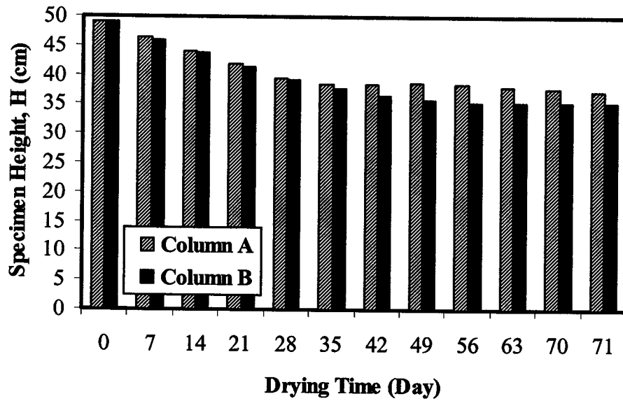
Figure B. 15 Specimen height changes in column drying tests for CT
