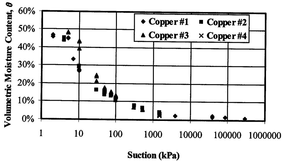
Figure B. 17 Soil-water retention curve test results for copper tailings
