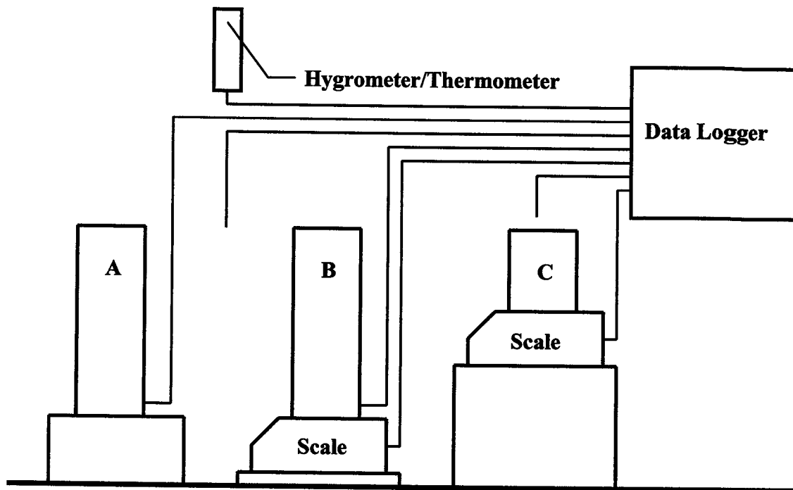
Figure 3.8 Layout of the drying test apparatus
