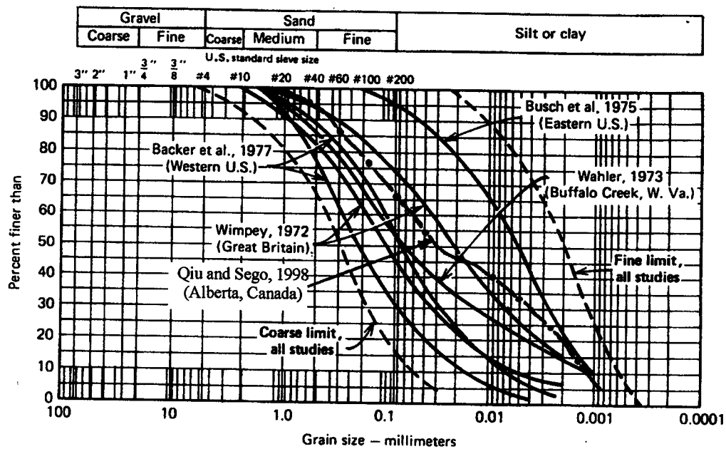
Figure A. 3 Grain size distribution of fine coal refuse (modified from Vick 1983)
