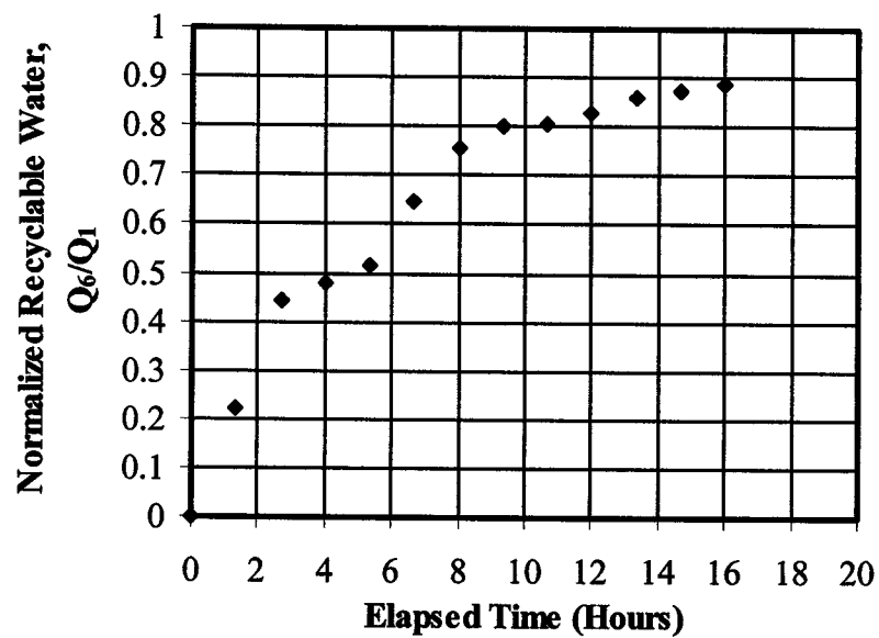
Figure 7.21 Normalized recyclable water in gold tailings
