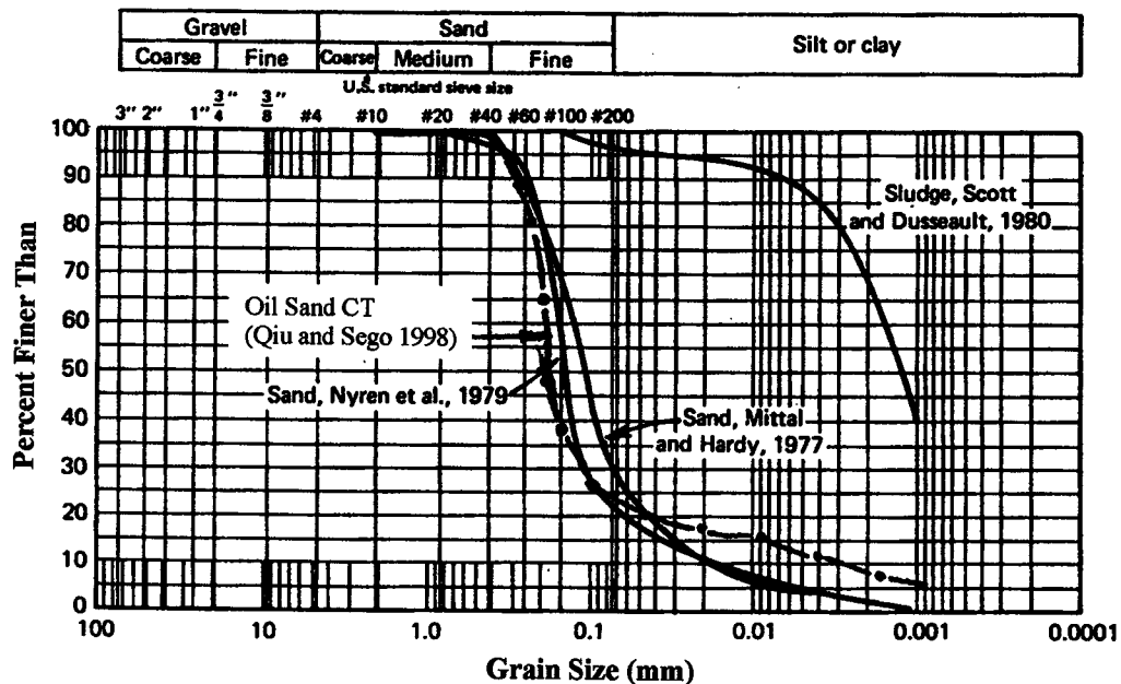
Figure A. 4 Grain size distribution of oil sand tailings (modified from Vick 1983)
