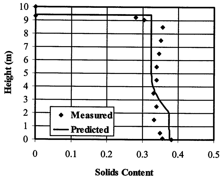
Figure 7.2 Measured and predicted solids content profile in a Ten Meter Standpipe after 20400 hours
