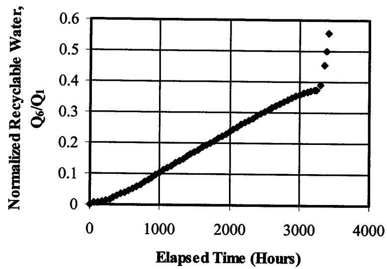
Figure 7.23 Normalized recyclable water in CT
