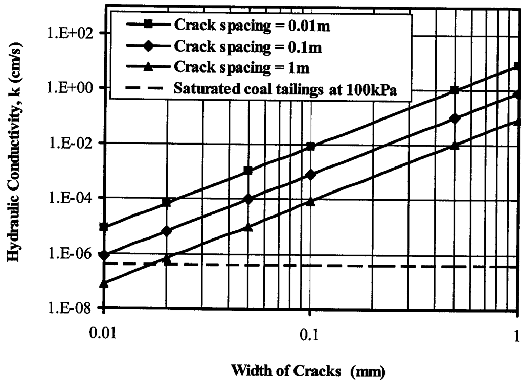
Figure 2.9 Comparison between the cracked and intact saturated hydraulic conductivity
