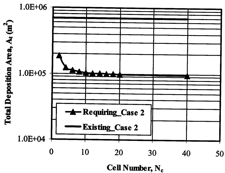
Figure 7.27 Deposition area versus cell number plot for case history #2
