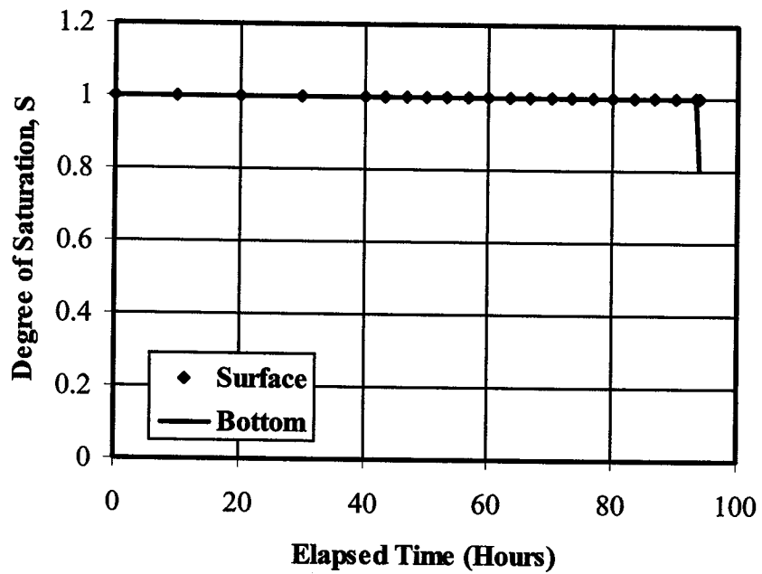
Figure 7.18 Degree of saturation change in coal tailings
