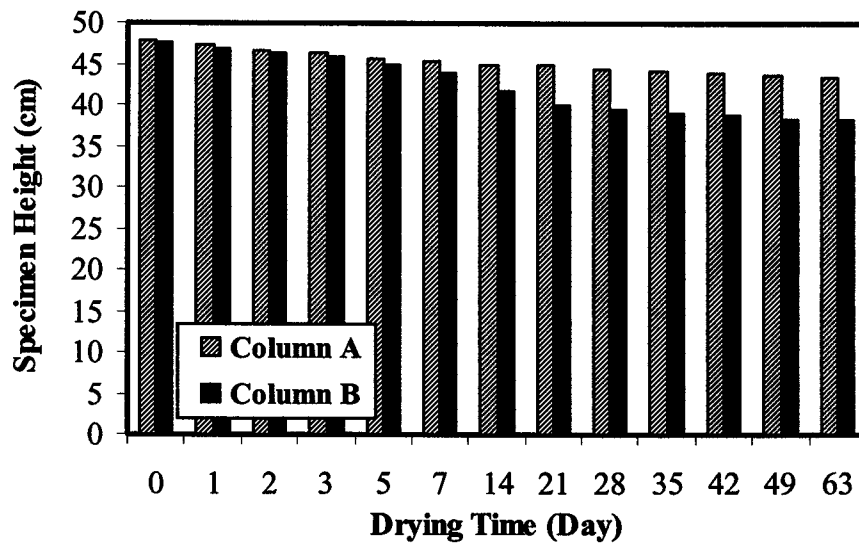
Figure B. 13 Specimen height changes in column drying tests for coal tailings
