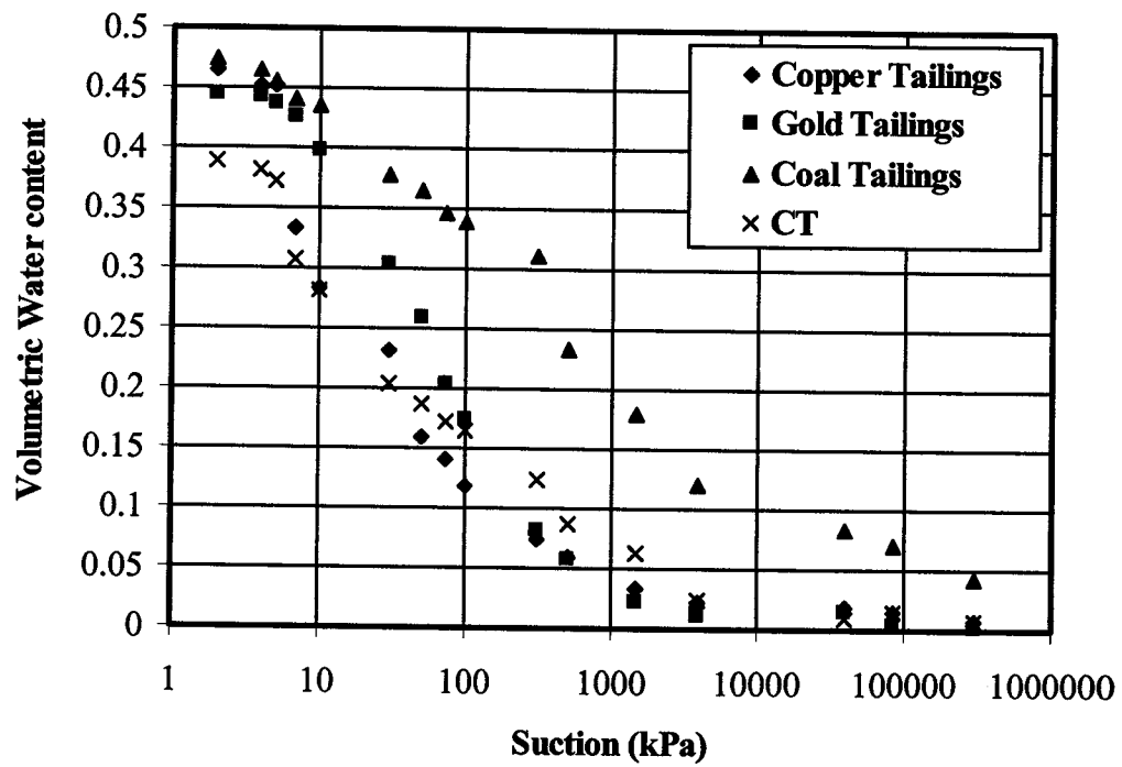
Figure 4.4 Soil-water retention curves of tailings
