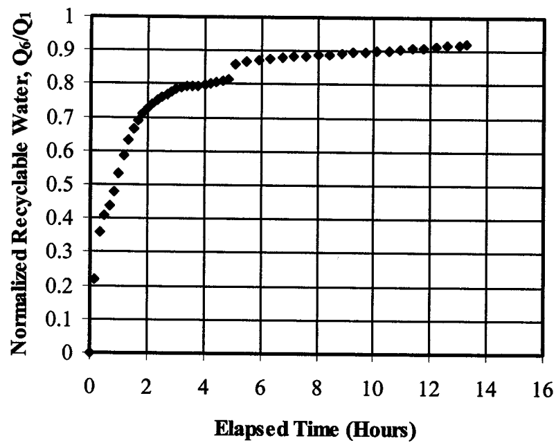
Figure 7.20 Normalized recyclable water in copper tailings
