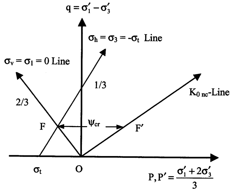
Figure 6.5 Stress path and critical suction for desiccating tailings (modified from Konrad and Ayad 1997)
