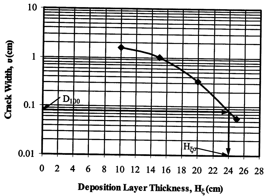
Figure 7.26 Optimum design curve for case history #2
