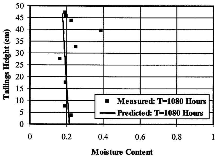
Figure 7.4 Measured and predicted moisture content profile of copper tailings in drying test
