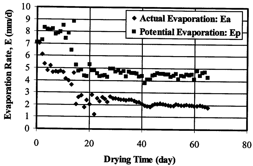
Figure B. 14 Evaporation changes in column drying tests for coal tailings
