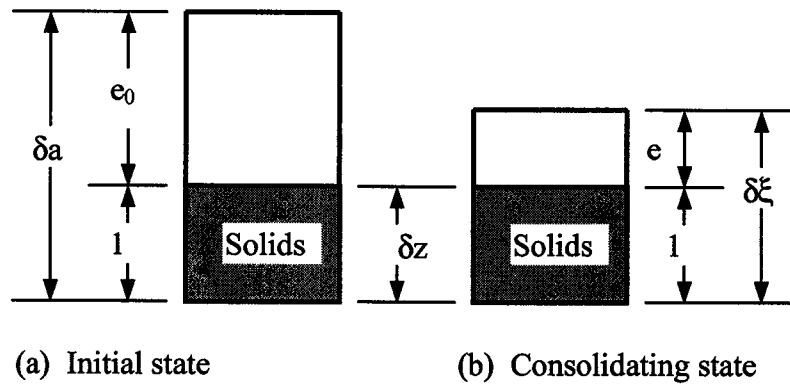
Figure 2.4 Solids coordinate z and relations with Eulerian and Lagrangian coordinates (modified from Gibson et al. 1981; Schiffman et al. 1988)
