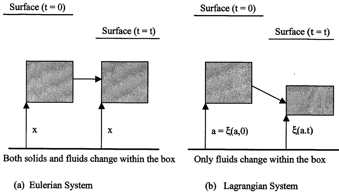
Figure 2.3 The Eulerian and Lagrangian coordinate systems (modified from Swarbrick 1992)
