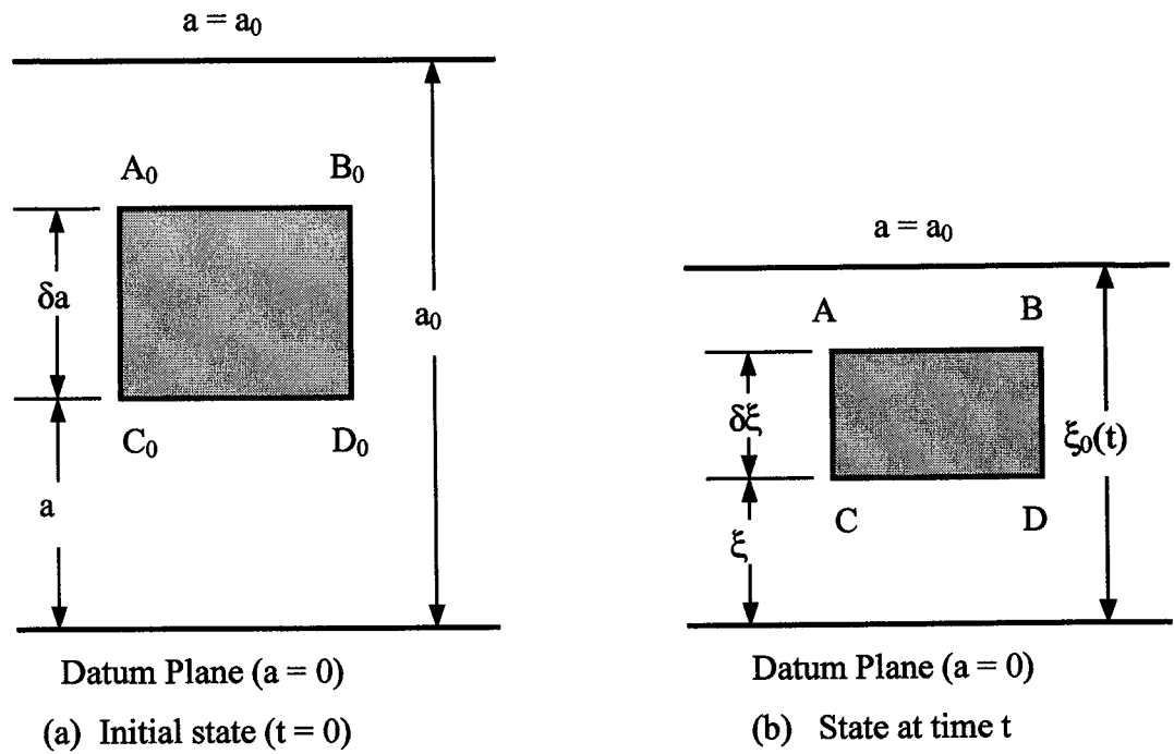
Figure 5.2 Lagrangian and convective coordinates (modified from Gibson et al. 1967, 1981)
