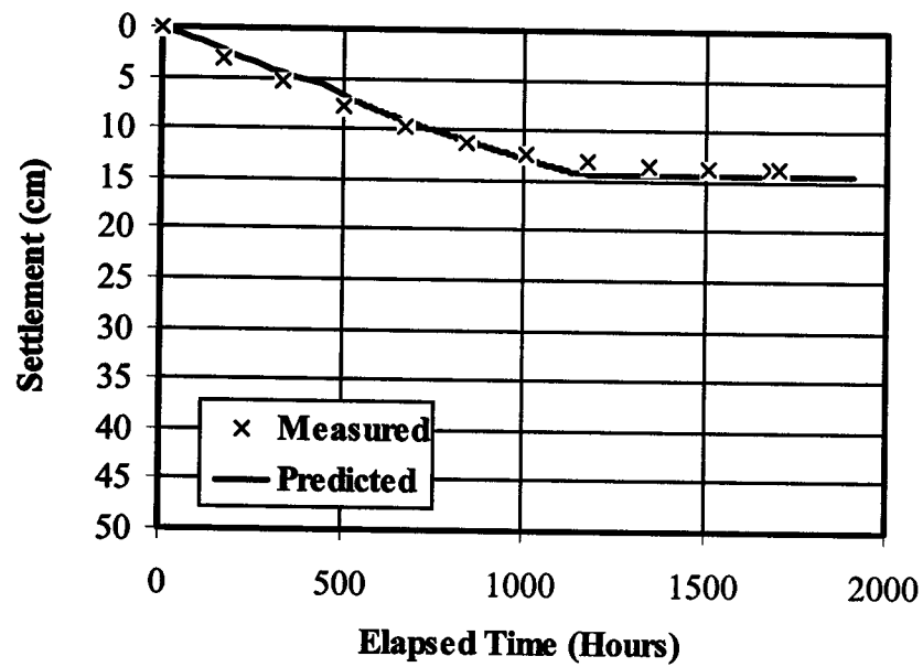
Figure 7.9 Measured and predicted settlement of CT in drying test
