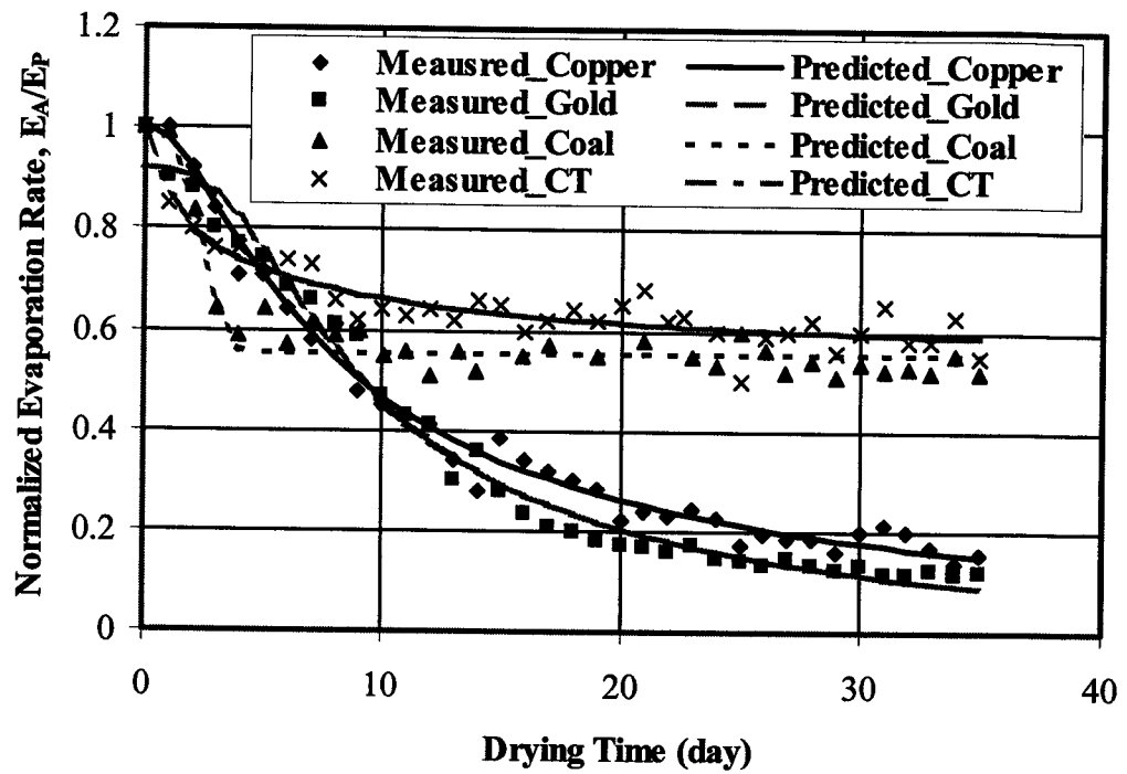
Figure 4.9 Comparison of measured and predicted evaporation of tailings
