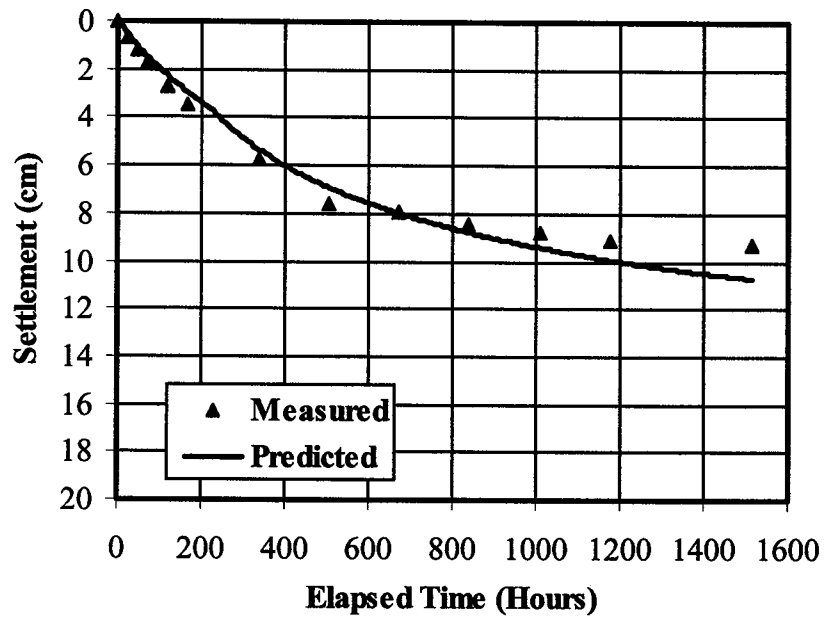
Figure 7.7 Measured and predicted settlement of coal tailings in drying test
