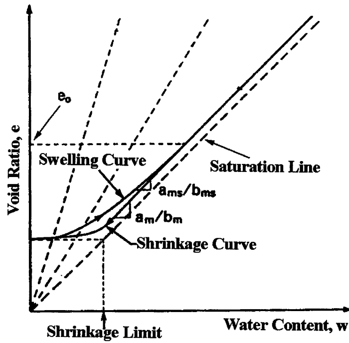
Figure 5.8 Typical shrinking and swelling curves for a soil (modified from Fredlund and Rahardjo 1993)
