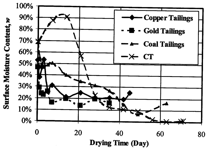
Figure 4.10 Moisture changes on the surface of the tailings
