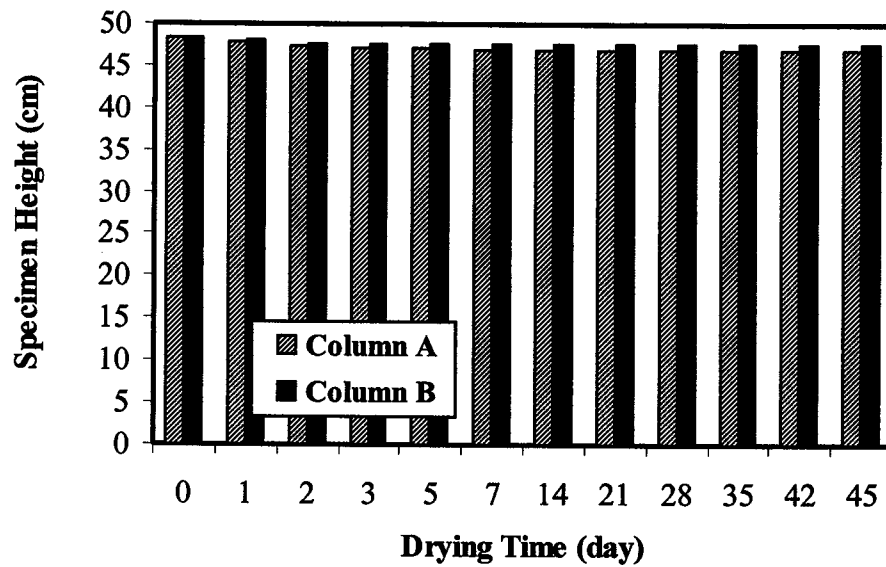
Figure B. 9 Specimen height changes in column drying test for copper tailings
