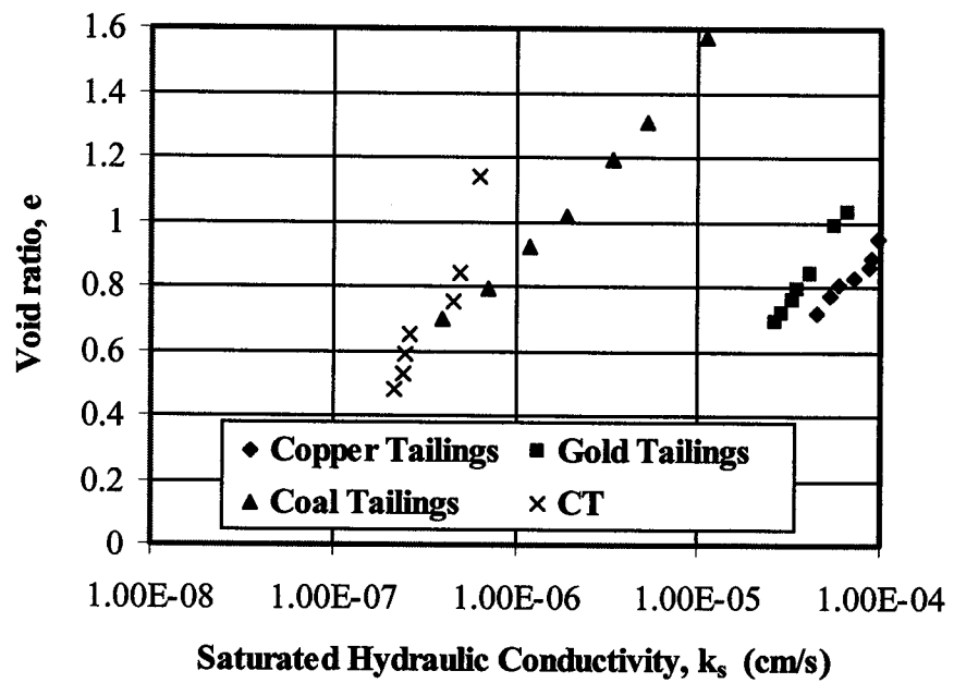
Figure 4.3 Void ratio versus hydraulic conductivity plots of tailings
