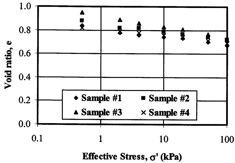
Figure B. 1 Compressibility of copper tailings
