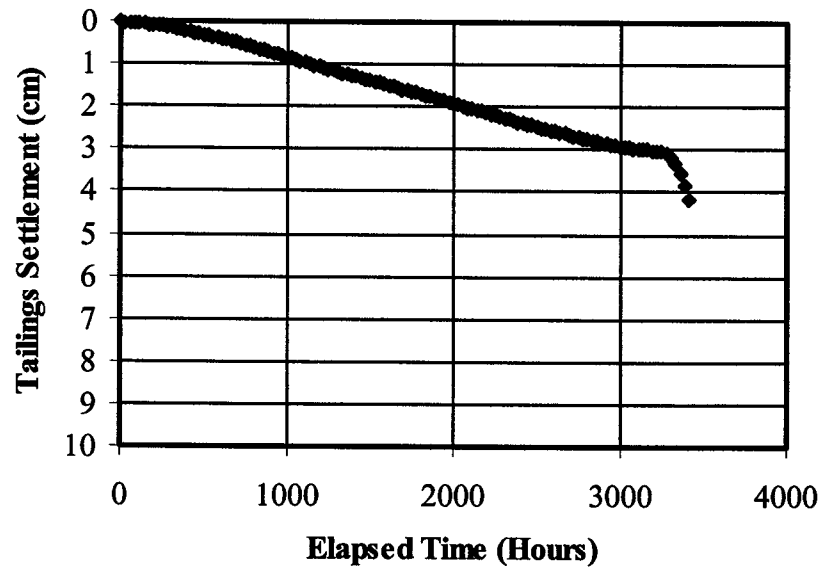
Figure 7.15 Predicted single layer settlement of CT at cracking
