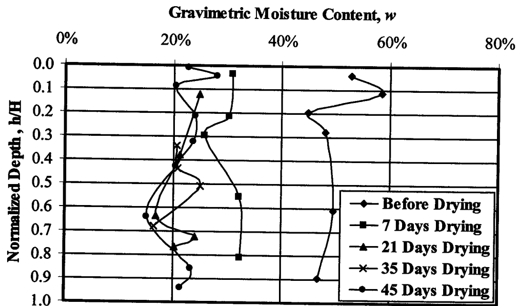
Figure 4.11 Moisture profile changes of copper tailings
