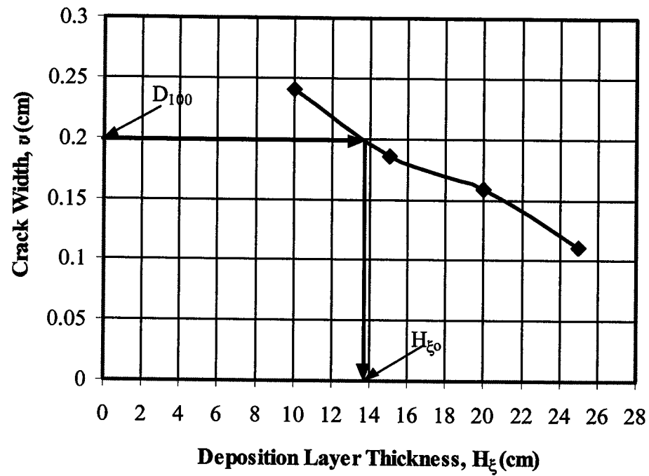
Figure 7.24 Optimum design curve for case history #1
