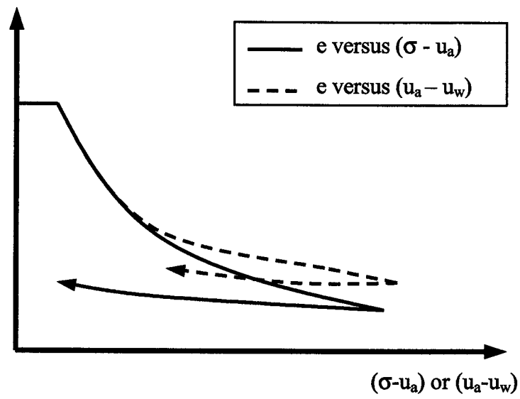
Figure 6.10 Constitutive relationship for soils (modified from Fredlund and Rahardjo 1993)
