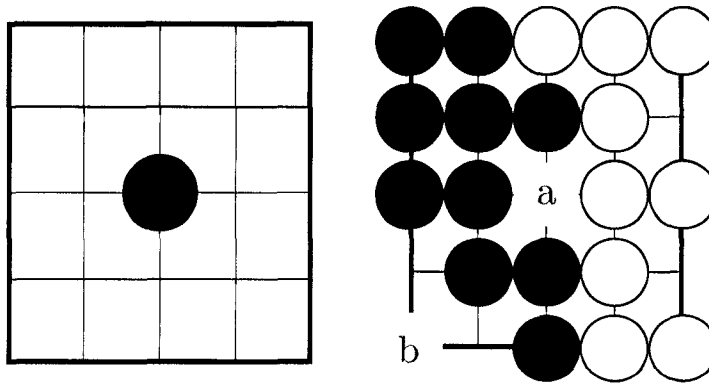
Figure 3.5: (Left) A 1 \times 1 , location-dependent feature with a central black stone. (Right) With Black to play, move b is the winning move. Playing at b creates two eyes in the black block, making that block alive (impossible for White to capture). If Black plays at a , then White can play at b , and the black block is dead (impossible for Black to save). Using 1 \times 1 features, the converging agent plays centrally at a , having learned a high weight for the feature that has a black stone there. However, the tracking agent learns that Black must play at b in this particular game, even though in general a corner move is not best.
