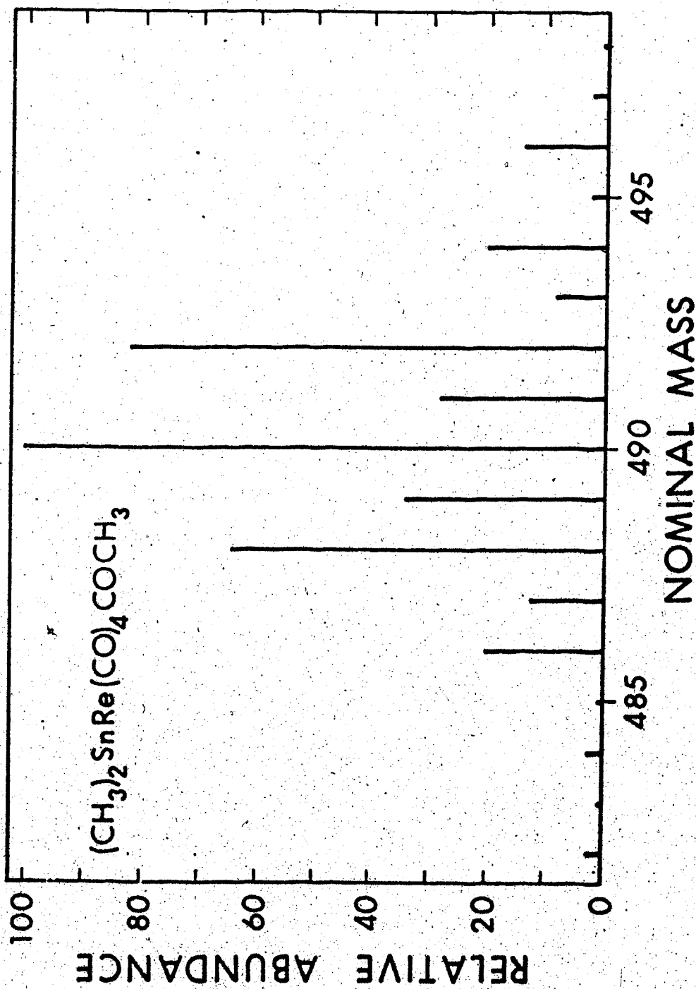
Figure 6. Calculated mass spectral isotope combination pattern for the parent ion of \text{Me}_2\text{SnRe}(\text{CO})_4\text{COCH}_3 .
