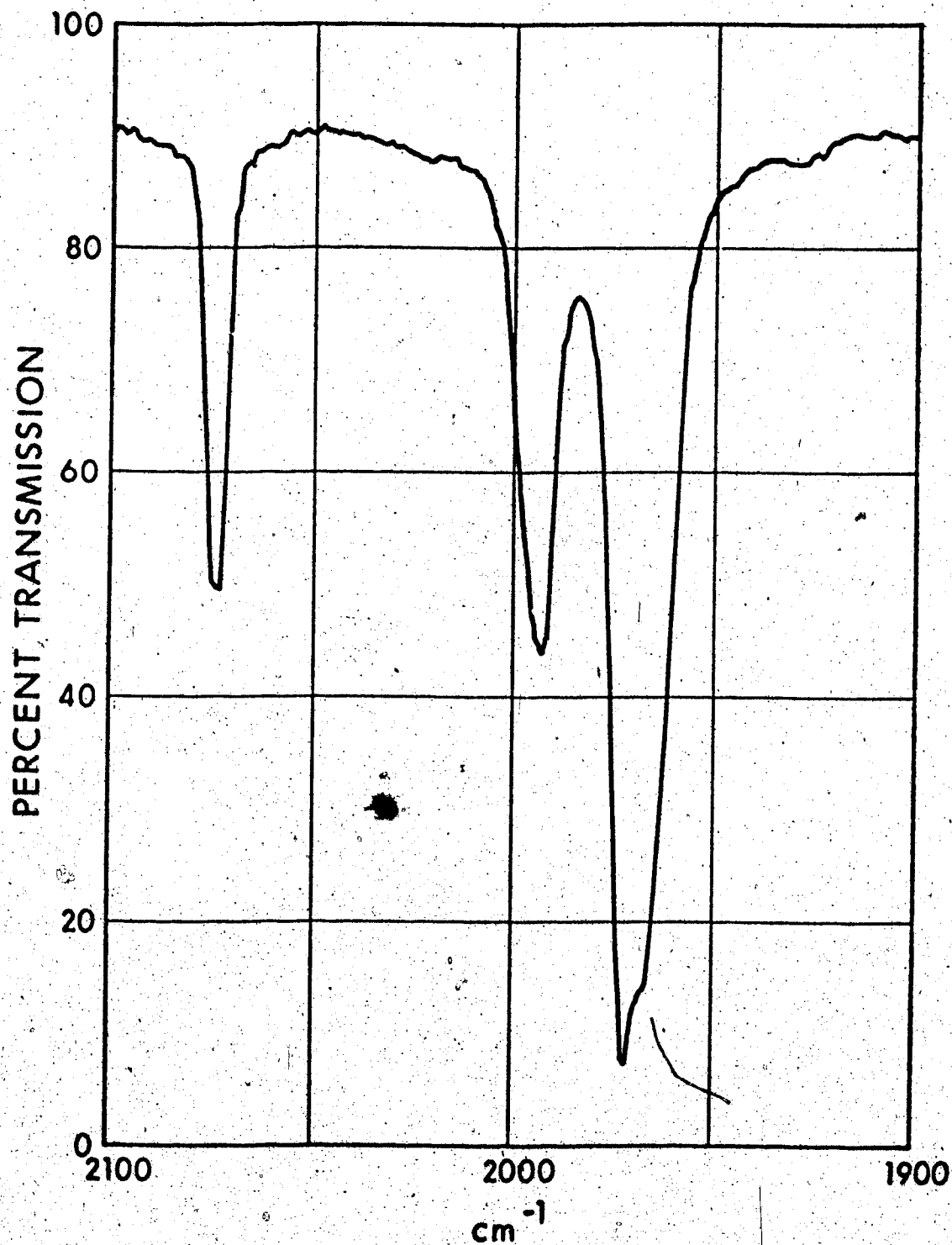
Figure 12. Infrared spectrum [ \nu(\text{CO}) region] of cis - \text{Ph}_2\text{MeGeRe}(\text{CO})_4\text{C}(\text{OEt})\text{Me} in cyclohexane.
