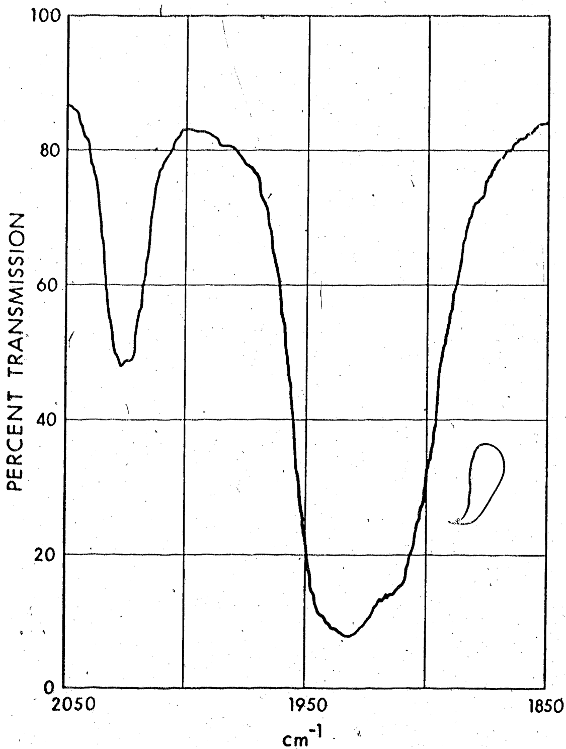
Figure 15. Infrared spectrum [ \nu(\text{CO}) region] of [\text{cis-Ph}_2(\text{HO})\text{GeMn}(\text{CO})_4\text{C}(\text{O})\text{Me}][\text{Et}_4\text{N}] in \text{CH}_2\text{Cl}_2 .
