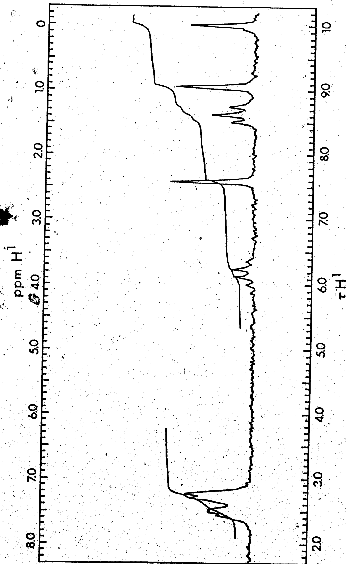
Figure 14. ^1\text{H} NMR spectrum of cis - \text{Ph}_2\text{MeGeMn}(\text{CO})_4\text{C}(\text{OEt})\text{Me} in \text{CDCl}_3 .
