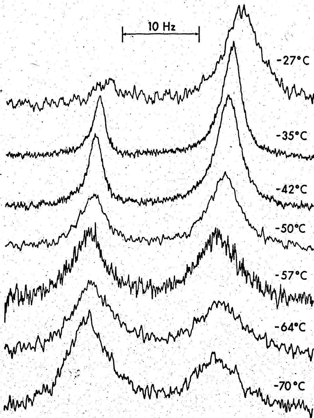
Figure 11. Variable temperature ^1\text{H} NMR study of \text{Me}_2\text{GeMn}(\text{CO})_4\text{COMe} in \text{CD}_2\text{Cl}_2 , showing an expansion of the \text{C-CH}_3 region only.
