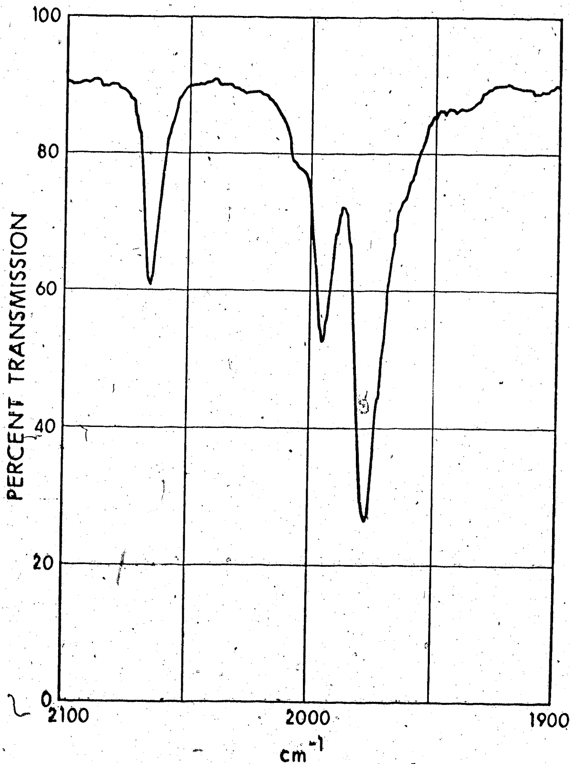
Figure 18. Infrared spectrum [ \nu(\text{CO}) region] of cis - \text{Ph}_2\text{FGeMn}(\text{CO})_4\text{C}(\text{OEt})\text{Me} in cyclohexane . (The peak at 2007\text{ cm}^{-1} is assigned to an impurity).
