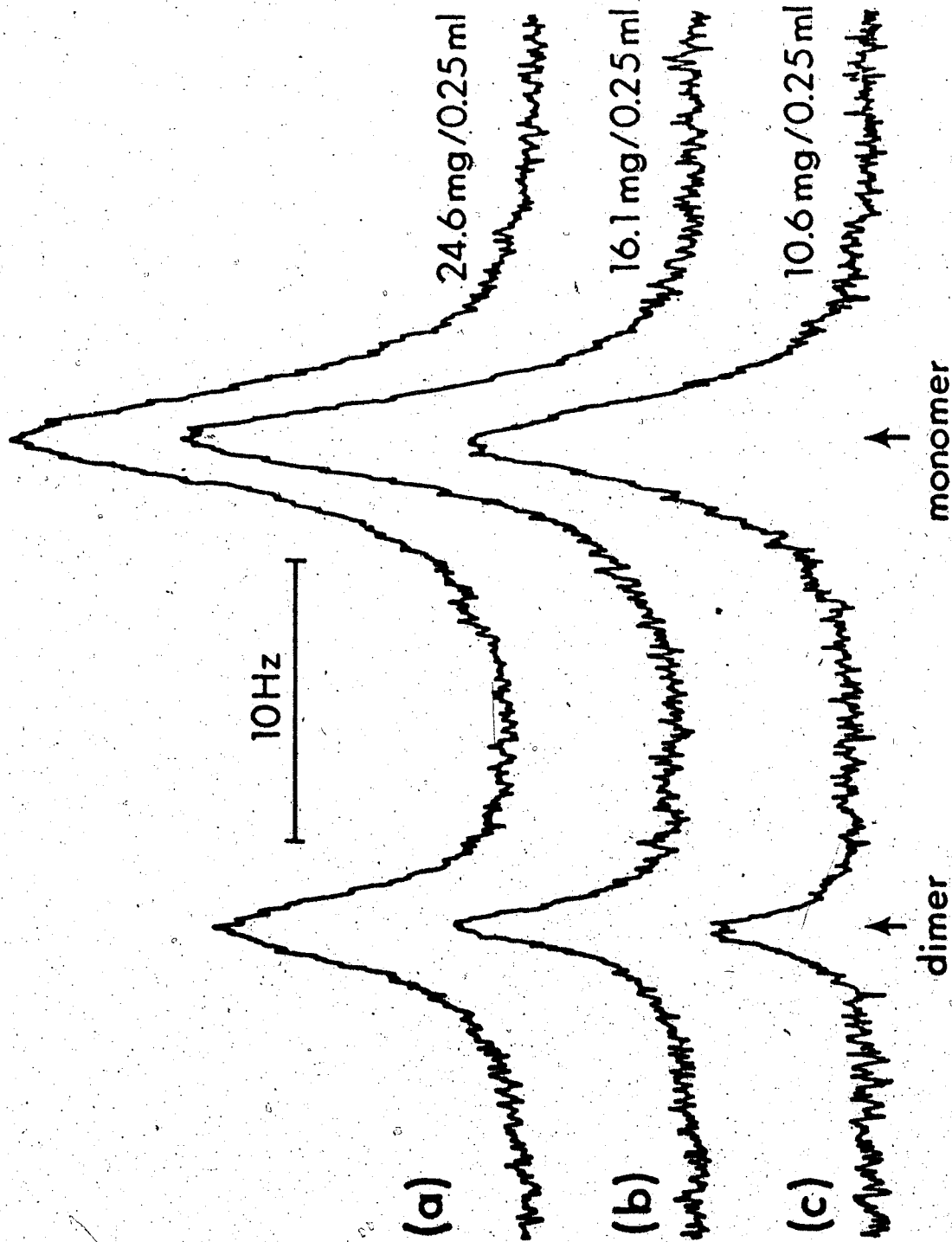
Figure 10. Variable concentration ^1\text{H} NMR study of \text{Me}_2\text{Gemn}(\text{CO})_4\text{COME} in \text{CD}_2\text{Cl}_2 at
