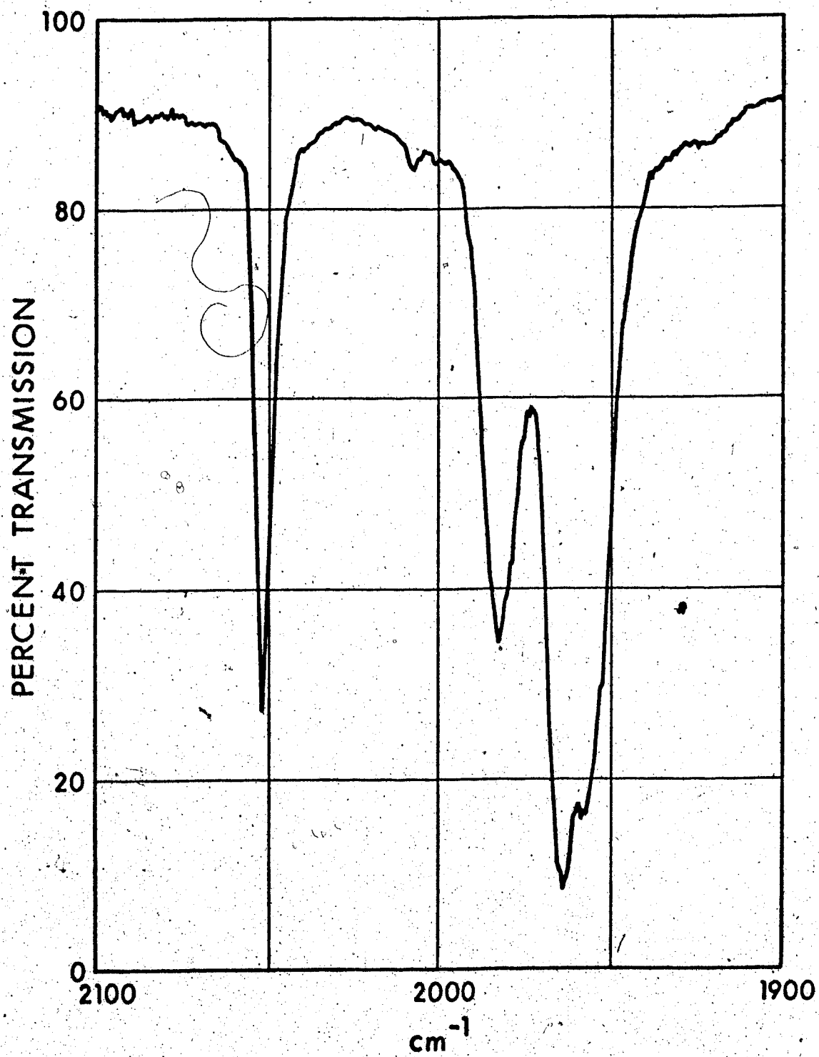
Figure 13. Infrared spectrum [ \nu(\text{CO}) region] of cis - \text{Ph}_2\text{MeGeMn}(\text{CO})_4\text{C}(\text{OEt})\text{Me} in cyclohexane.
