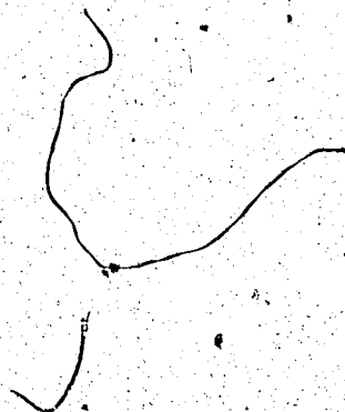
FIGURE 24. Reconstitution of electron transport in pentane extracted mitochondria by duroquinone.
