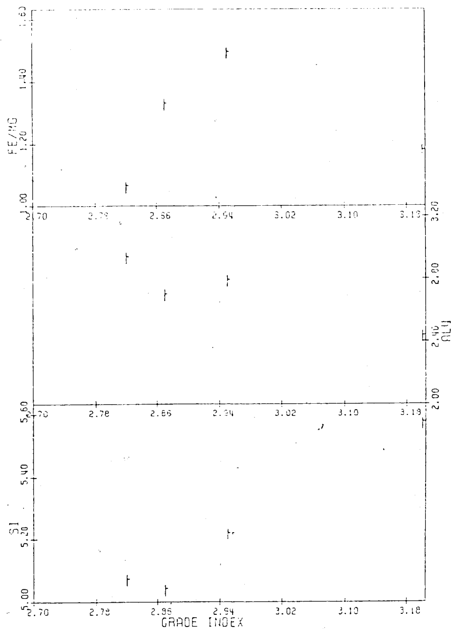
FIGURE 7a: Diagram illustrating the relationship of chlorite composition (atomic proportions) to grade index for chlorites from the biotite zone.
