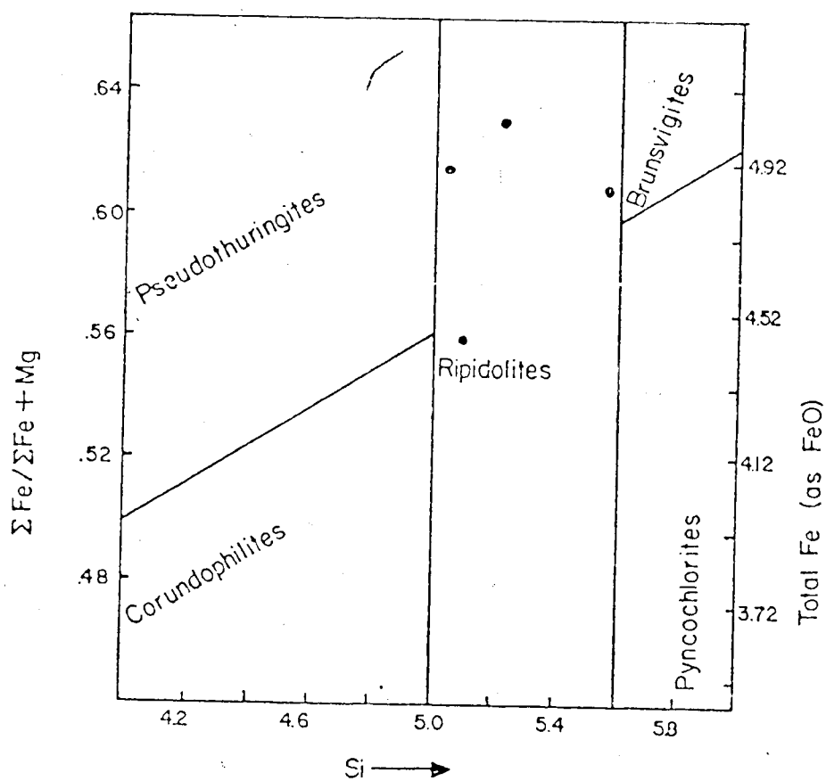
FIGURE 7b: Diagram showing that all of the biotite zone chlorites are ripidolites. (Modified after Hey, 1954)
