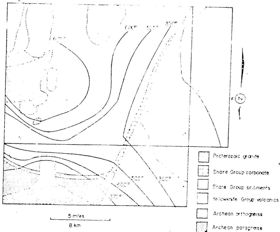
FIGURE 2. Block diagram showing the hypothetical distribution of lithologies and isotherms for the Arsen Lake area. Vertical exaggeration is \times 1.5 .
