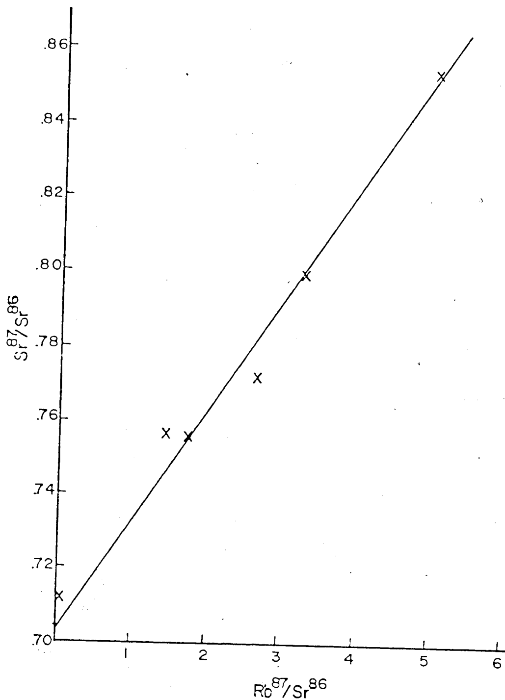
FIGURE 3: Diagram showing the Rb/Sr data available for the remobilised Archean paragneiss. The line shown is a 2110 m.y. reference isochron.
