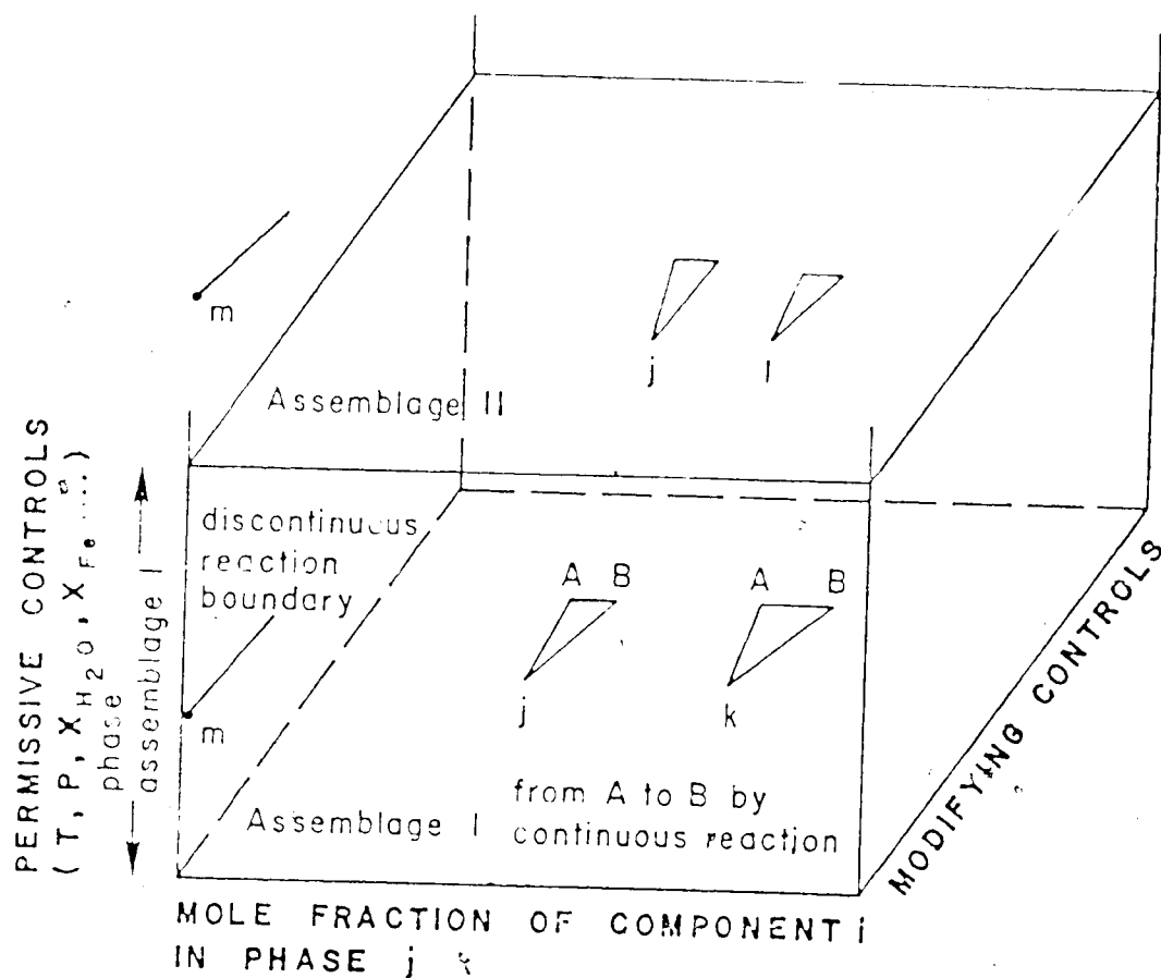
FIGURE 8: Diagram illustrating the relative roles of permissive and modifying controls on mineral composition. See text for discussion of the modifying controls. Points m, j, k, and i all lie on one vertical plane and represent mineral compositions that would be attained at perfect equilibrium (i.e., the chemical potential for any given species is identical in all phases containing that species). Where perfect equilibrium is not attained due to kinetic restrictions or limited intergranular diffusion, then a mineral's composition may vary along the area KAB. The exact location in the area KAB can be related to the cumulative effects of all of the modifying controls.
