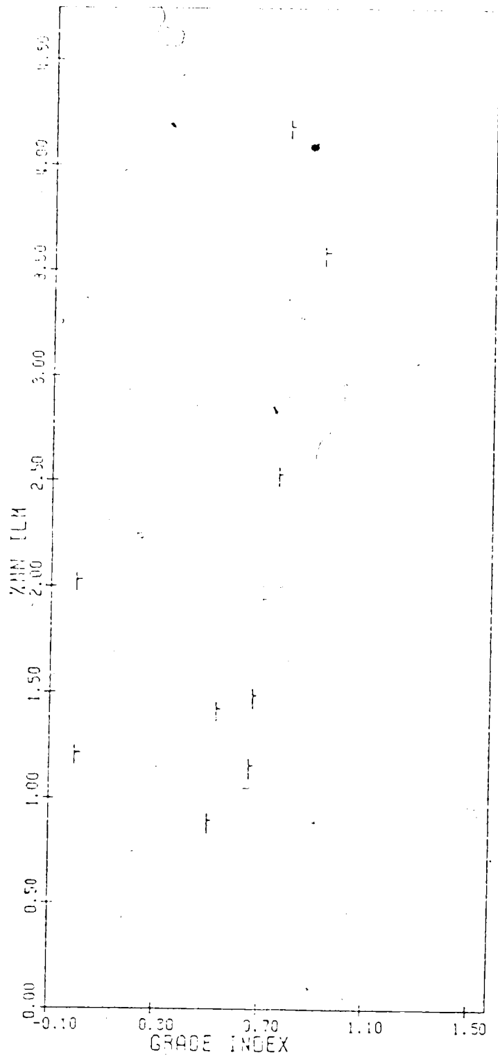
FIGURE 5b: Diagram illustrating the relationship between pyrophanite content of ilmenite and grade index for ilmenite from the almandine-cordierite-K-feldspar zone.
