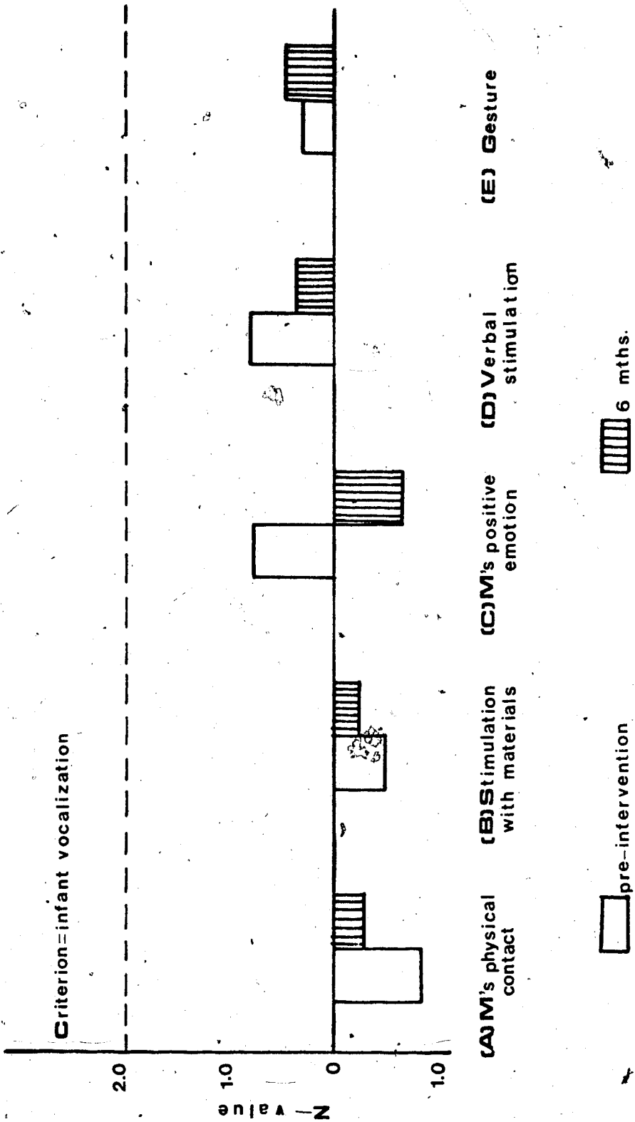
FIGURE 12: SEQUENTIAL DEPENDENCIES (2)
