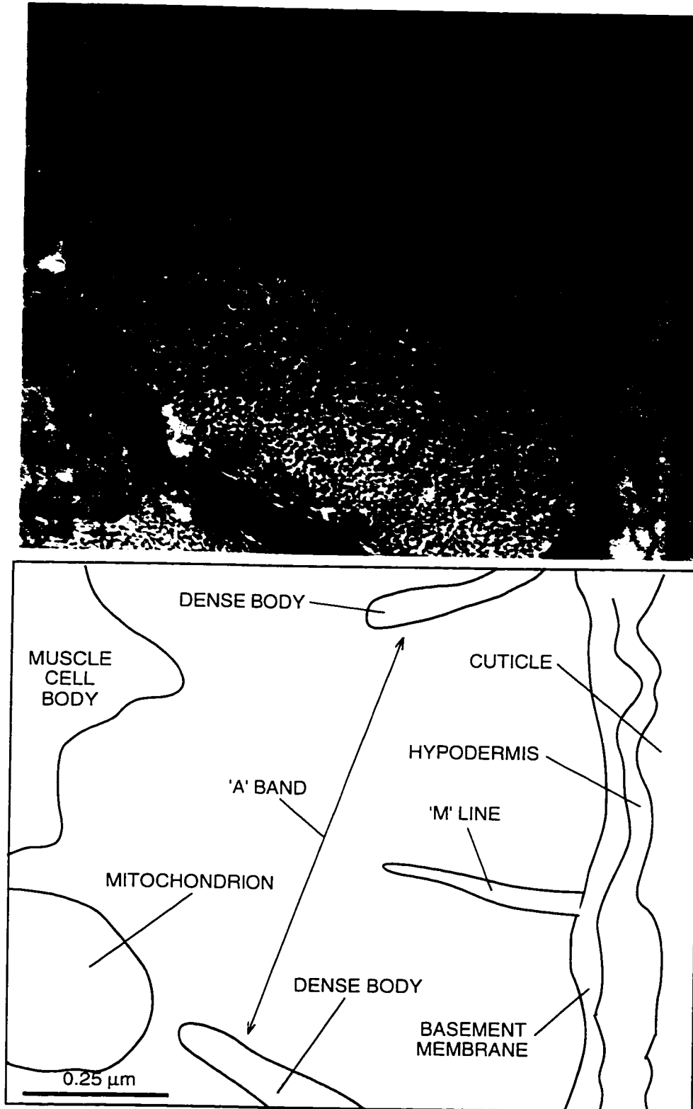
Figure 2.12 Electron micrograph of unc-119(e2498) muscle sarcomere (top). A line representation of the micrograph is shown below, to indicate particular structures.
