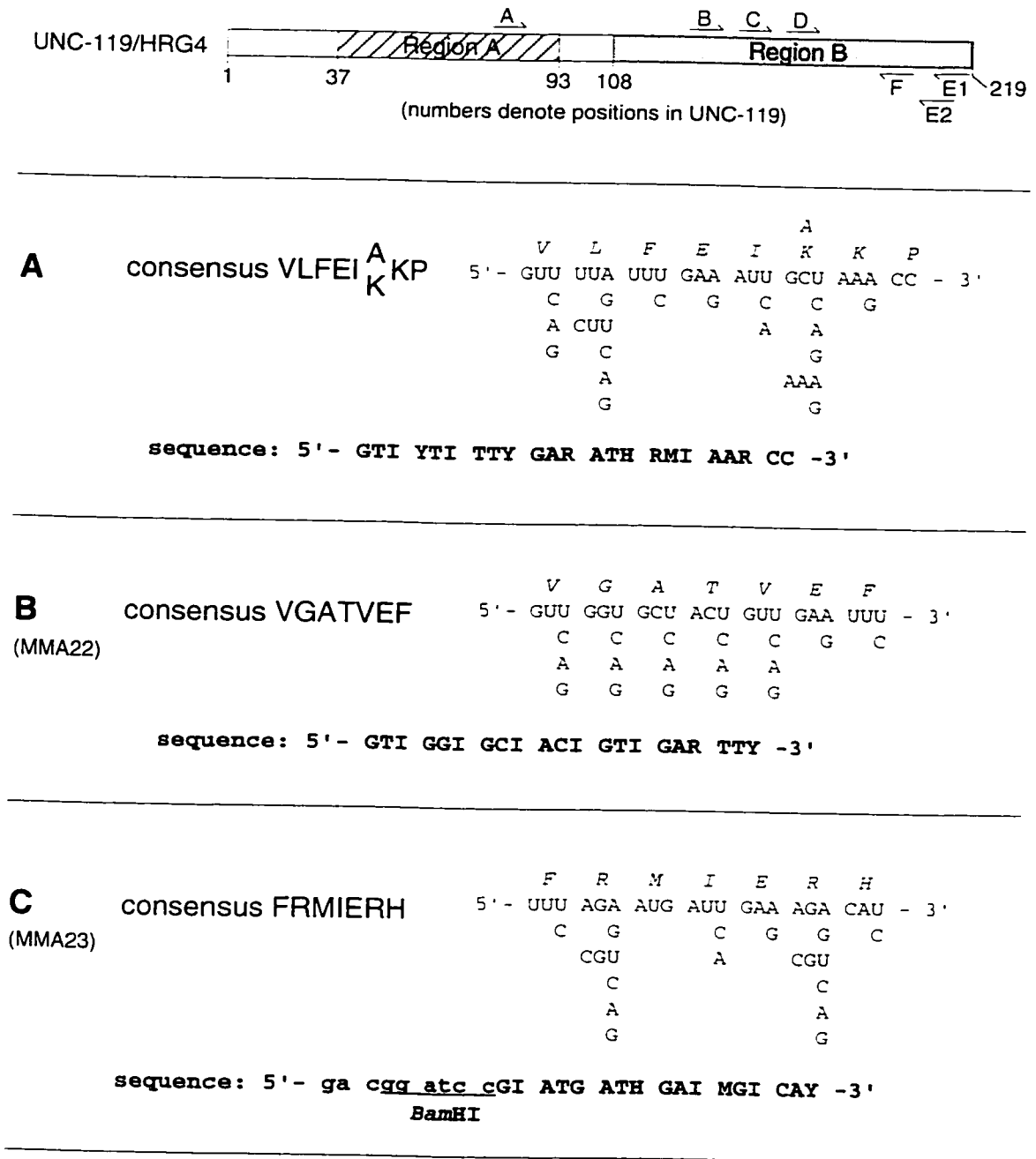
Figure 4.10 Design of degenerate PCR primers to amplify putative homologues of UNC-119/HRG4 (continued on next page). The top figure shows the locations of the various primers within the UNC-119 coding region. Only the B, C, E2 and F primers were synthesized. The Bam HI sites used for cloning are indicated. Nucleotide abbreviations: I = inosine; R = A or G; Y = C or T; S = G or C; W = A or T; H = A or C or T; N = A or C or G or T.
