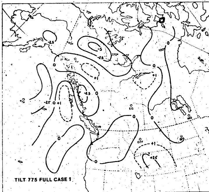
Fig. 11. Test areas and an analysis of the tilting term (TILT) at 775 mb for the full lower boundary condition. Units of the tilting term are 1.25 \times 10^{-10} \text{ sec}^{-2} . The dotted line in the test area diagram is part of row 9 of the grid from which sample omega values were taken (Table 2).
