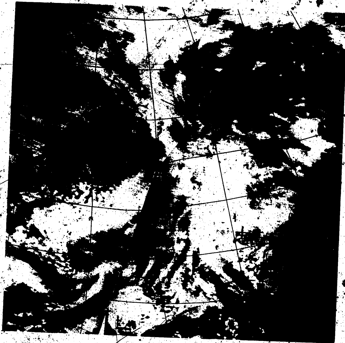
Fig. 24. Satellite photograph mosaic of the meteorological conditions for Case 3. This photograph was available in specially prepared gridded format, thanks to Mr. D. L. Orcheski, a graduate student at the University of Alberta. Longitude lines are every 10^{\circ} and latitude lines every 5^{\circ} . 60^{\circ}\text{N} , 120^{\circ}\text{W} is just southwest of Great Slave Lake (plainly visible).
