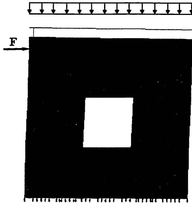
(b) Deformed mesh for W2 (DSF=10)
