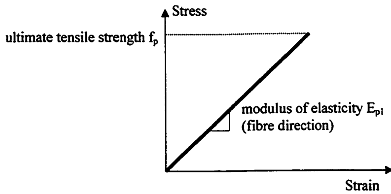
Figure 3-10 CFRP Behaviour
