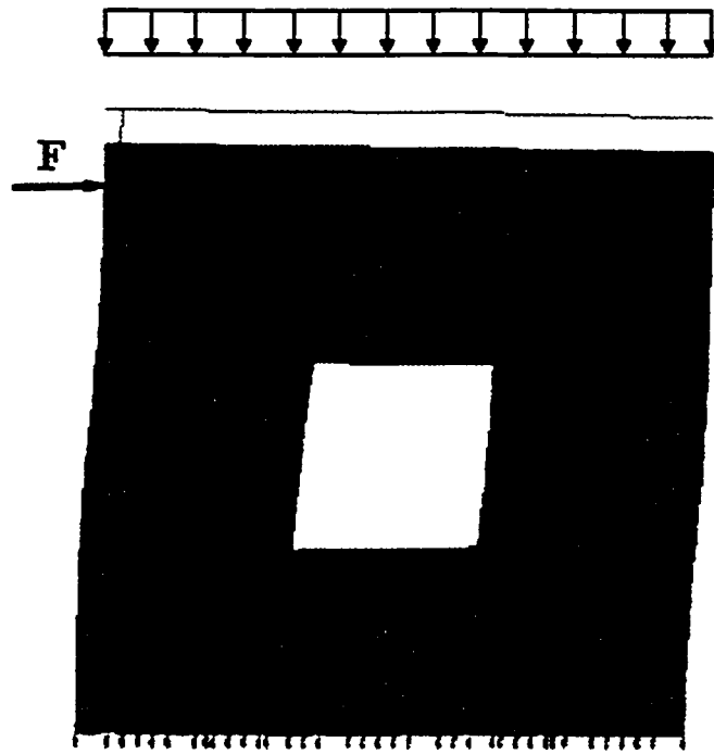
(a) Deformed mesh for W1 (DSF=10)
