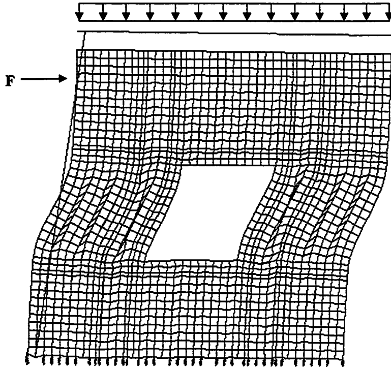
Figure 4-46 Deformed Mesh for Specimen W4 (DSF = 10)
