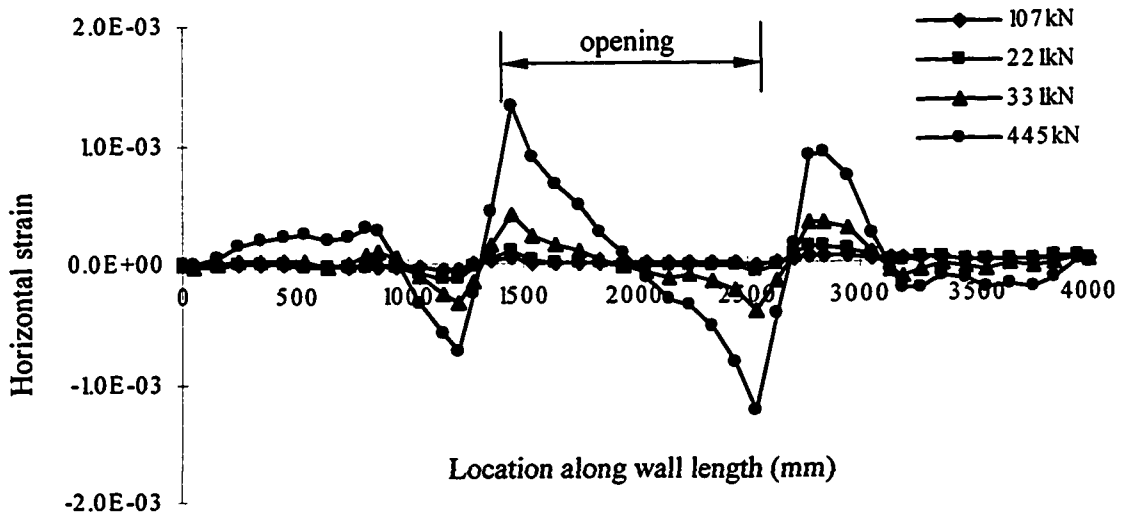
Figure 4-14 H1 Strain Distribution of Horizontal CFRP for W2
