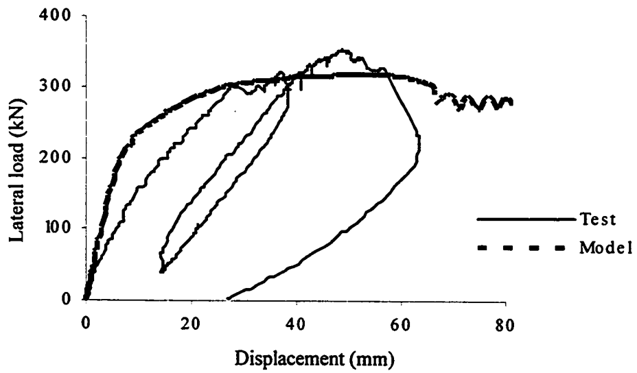
Figure 4-47 Lateral Load - Displacement Curves for W4
