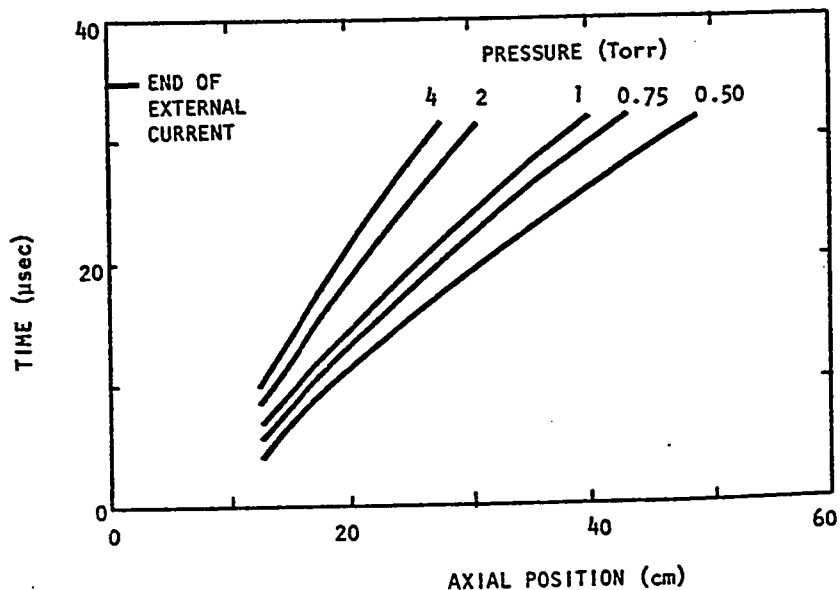
Fig.6.13 Current front position of CPA with Insulator II; V_0 = +10 kV.
