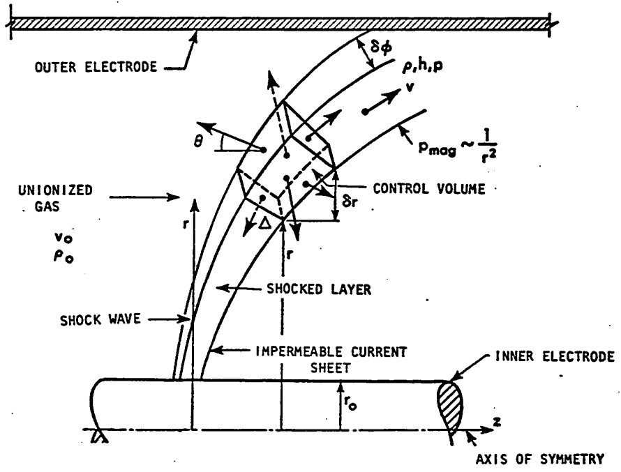
Fig.3.1 Sketch of part of a long CPA with the control volume just between the current sheet and the shock wave; notation used in the quasi-one-dimensional model in the cylindrical coordinates (r, z, \phi) .
