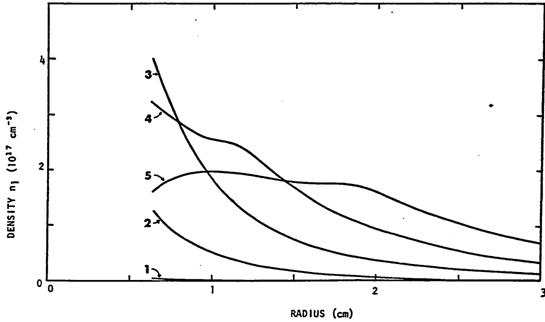
Fig.4.8 Calculated number density n_1 = n_{\text{He}^+} versus radius;quasi-one-dimensional-model. See also Fig.4.5
