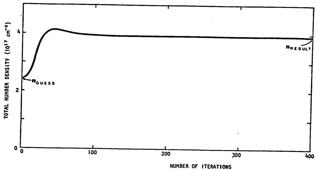
Fig.4.6 Iterative improvement of the guess value. The resulting value is one point on the n = n(v_0) curve of Fig.3.4 ( v_0 = 4.5 \text{ cm/sec} ).
