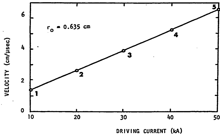
Fig.4.5 Ideal steady-state current sheet velocity versus driving current; points #1, ..., #5 are of the same meaning as those in Figs. 4.7 to 4.14 .
