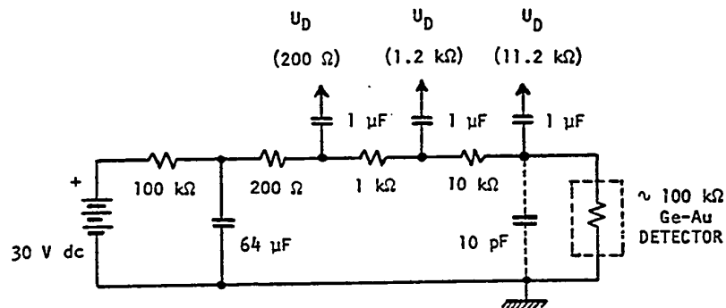
Fig.5.16 Schematic diagram of the Ge-Au detector.
