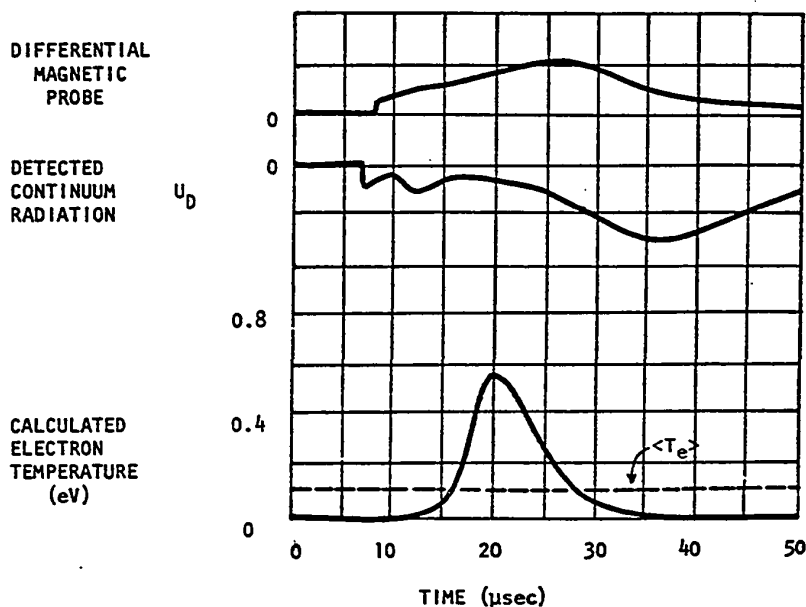
Fig.6.8 Oscillograms of local current, detected ir continuum radiation, and calculated electron temperature for known electron density (Fig.5.15) and known average temperature \langle T_e \rangle .
