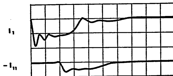
Fig.5.8 Oscillogram of the currents I_1 and I_{11} ; R_2 \sim Z_0/1.8 , V_0 = -8 kV, I_1:50 kA/div, I_{11} is not calibrated, 10 \mu sec/div.
