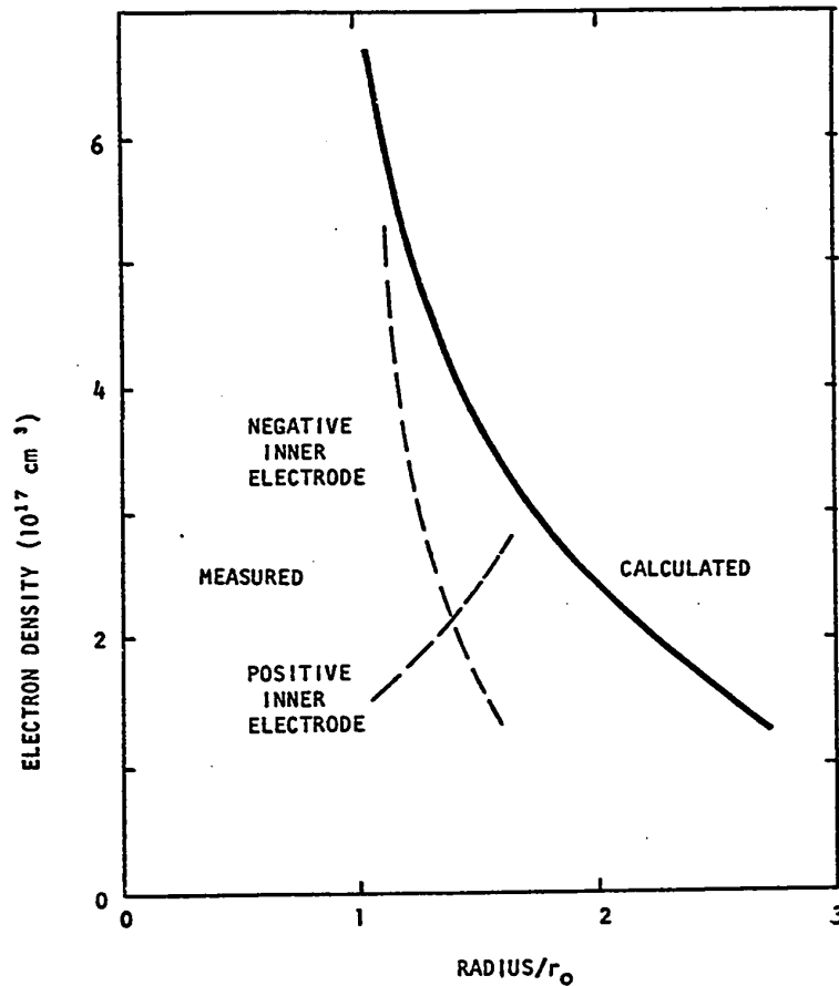
Fig.4.15 Calculated and experimental electron number densities; v_0 = 6 \text{ cm}/\mu\text{sec} ; experimental data of Lie et al.(1967).
