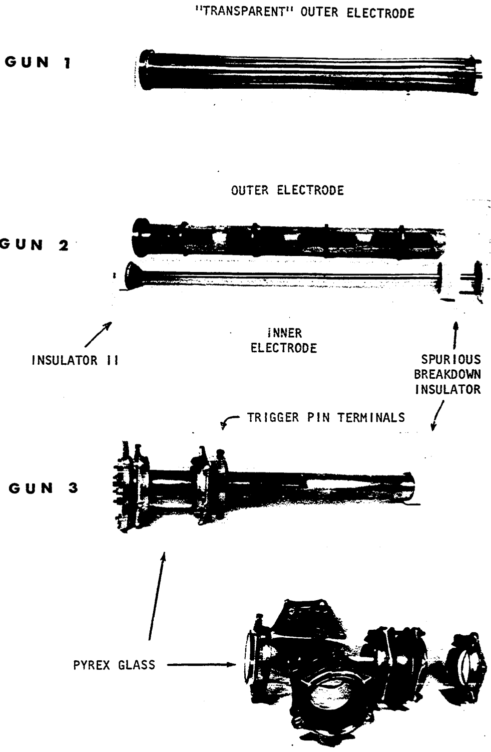
Fig.5.3 Three versions of the CPA.
