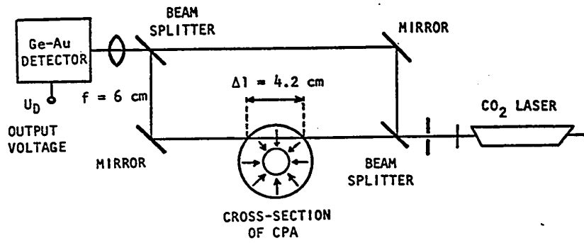
Fig.5.14 Mach-Zehnder interferometer arrangement.
