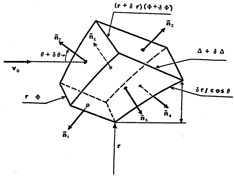
Fig.3.2 The control volume of steady shocked layer model. The surface of this volume is divided into six parts with unit normal vectors \bar{n}_1, \dots, \bar{n}_6 ; (r, z, \phi) are cylindrical coordinates, v_0 is the axial velocity of the undisturbed gas relative to the current sheet, \Delta and \theta are defined by Fig.3.1
