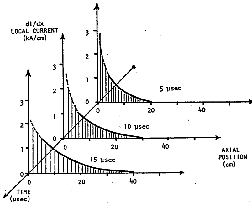
Fig.6.4 Typical time development of the discharge current inside CPA with Insulator I; P_0 = 1 \text{ Torr} .
