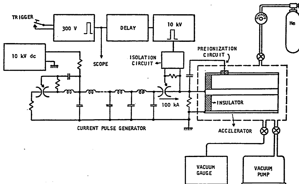
Fig.5.1 Schematic layout of the CPA apparatus.
