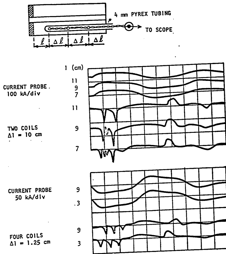
Fig.5.12 Current sheet velocity measurement; schematic and typical oscillograms for two and four coils nonintegrated magnetic probes (10 V/div); horizontal scale: 5 \mu\text{sec/div} .
