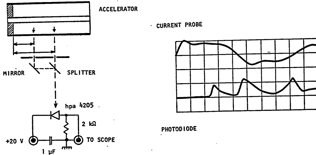
Fig. 5.10 Luminous layer position measurement; experimental set-up and typical oscillograms; V_0 = -10 kV, I = 100 kA/div, photodiode: 10 v/div, horizontal scale: 10 \mu sec/div. One photodiode and six exposures were used.
