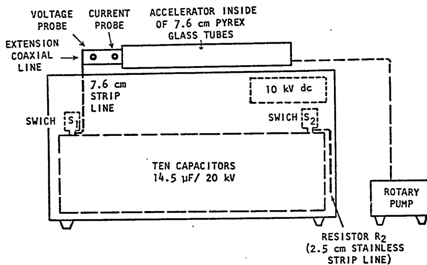
Fig.5.2 Sketch of the mechanical set-up. Notation according Fig.5.4
