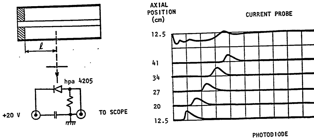
Fig. 5.11 Luminous layer velocity measurement; experimental set-up and typical oscillogram, I = 100 kA/div, photodiode: 0.2 V/div, horizontal scale: 5 \mu sec/div.
