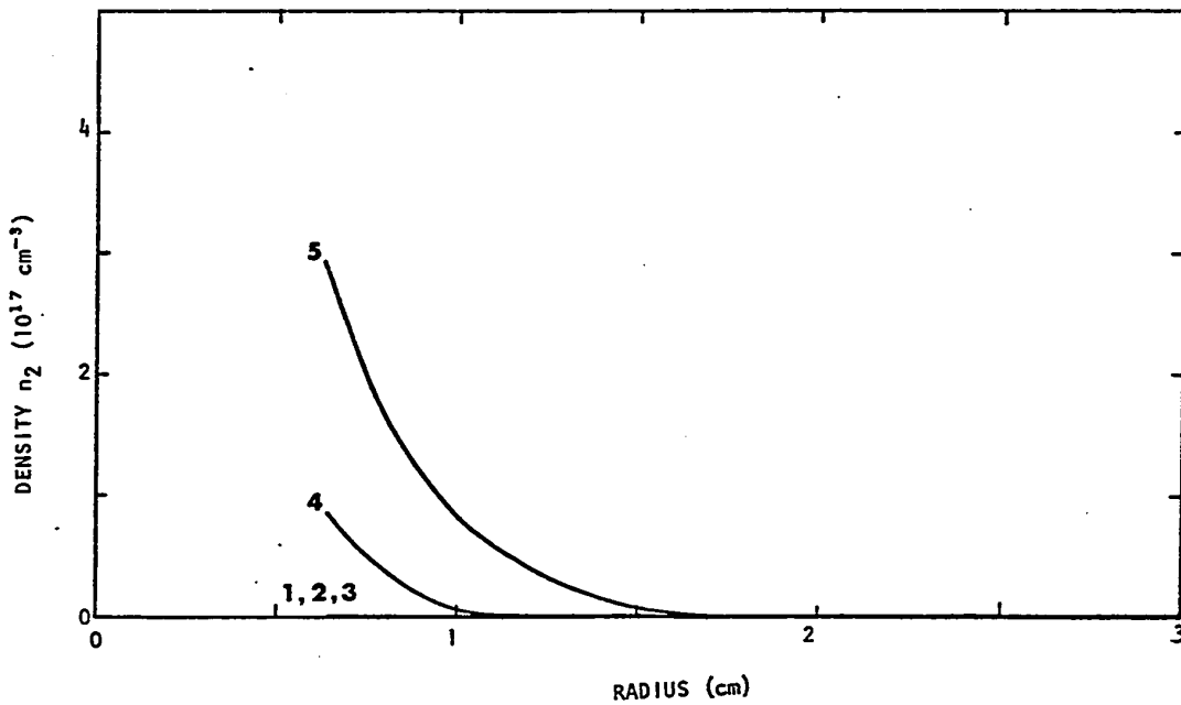
Fig.4.9 Calculated number density n_2 = n_{\text{He}^{++}} versus radius;quasi-one-dimensional model. See also Fig.4.5
