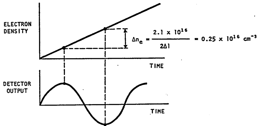
Fig.5.15 Evaluation of the interferogram for a linear electron density change and path \Delta l \sim 4.2 \text{ cm} . One fringe shift corresponds to 2\Delta n_e .
