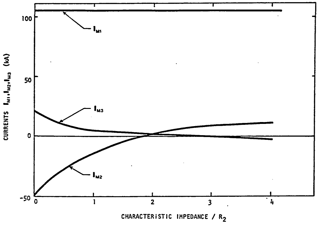
Fig.5.6 Variation of currents I_{M1} , I_{M2} , and I_{M3} with Z_o/R_2 , for experimental parameters as above. These currents are defined in Fig.5.5 .
