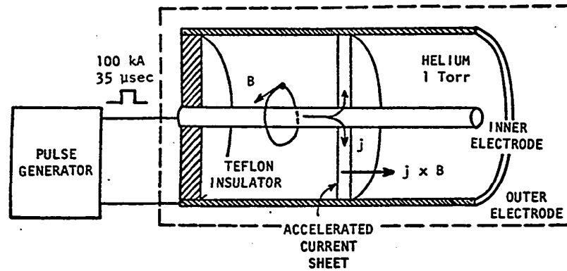
Fig.1.1 Coaxial plasma accelerator.
