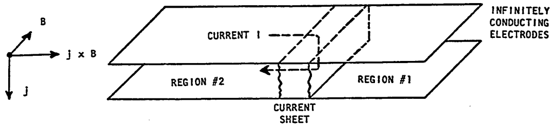
Fig.2.3 Diagram of current sheet motion.
