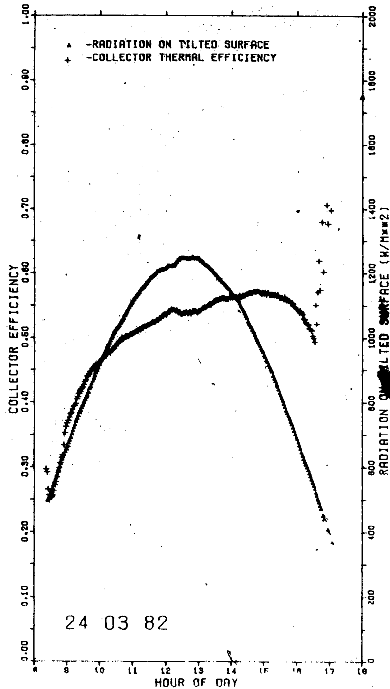
Figure 5.3 Instantaneous Solar Radiation And Collector Thermal Efficiency For 24 March 1982
