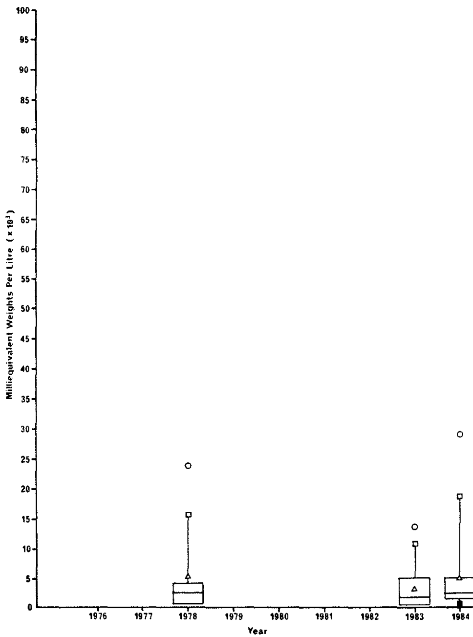
Figure 38. Box plots for the annual distribution of Mg 2+ in snow samples in the AOSERP network.
