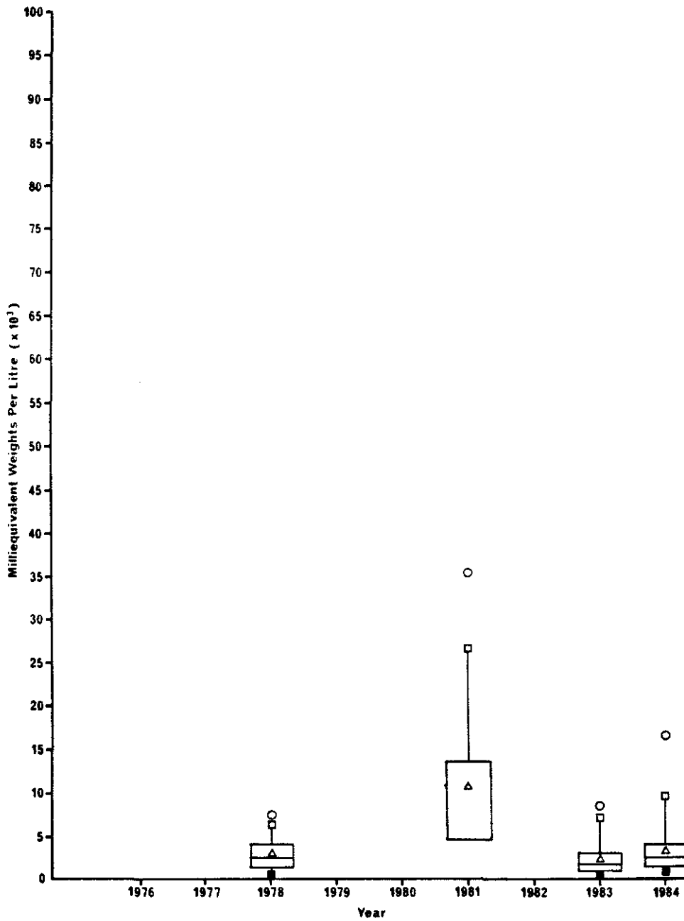
Figure 35. Box plots for the annual distribution of Na + in snow samples in the AOSERP network.
