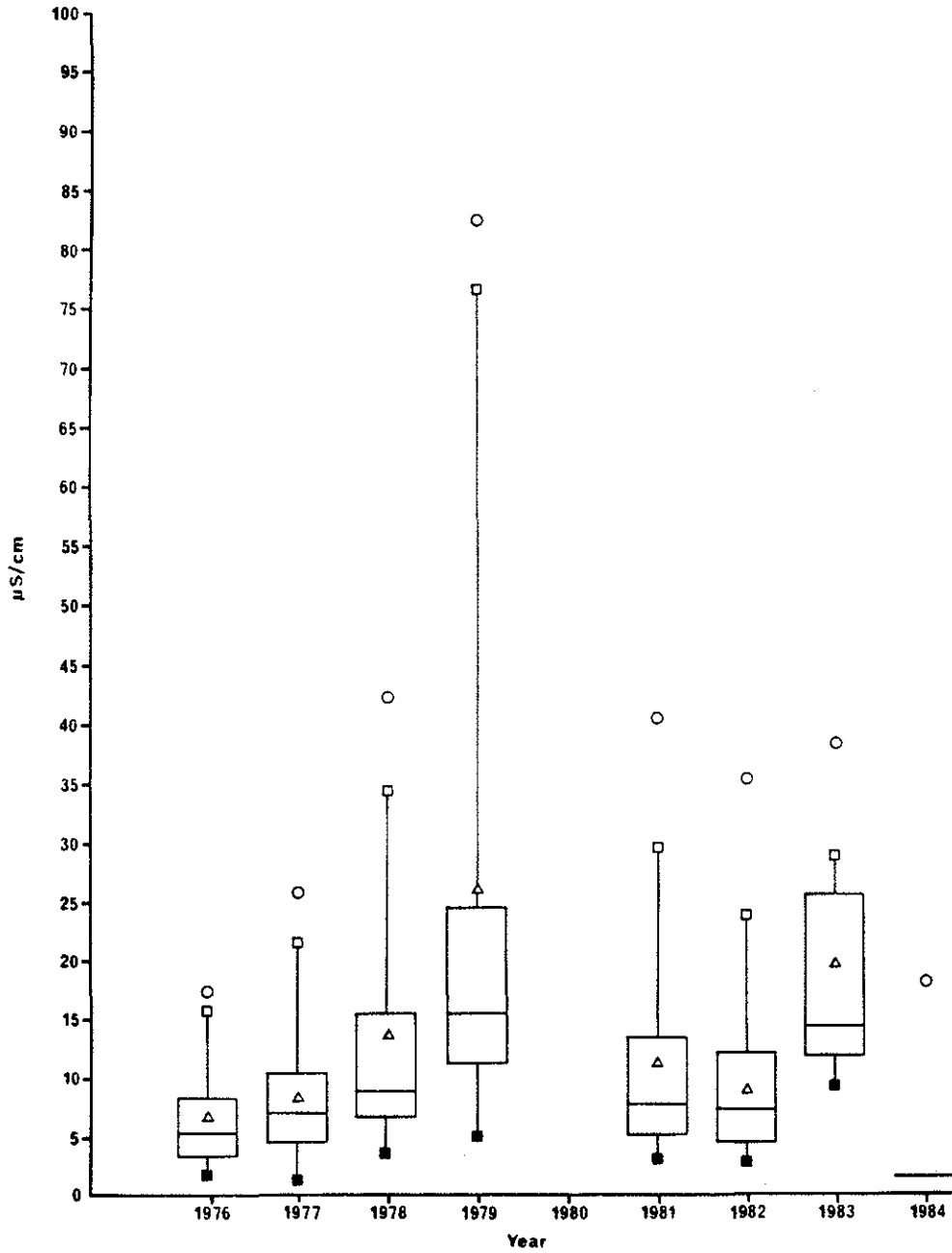
Figure 18. Box plots for the annual distribution of conductance in rain samples in the AOSERP network.
