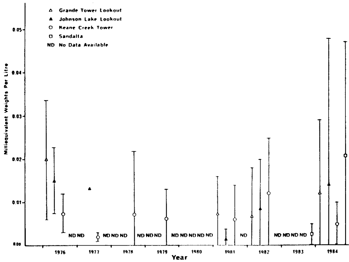
Figure 23. Annual mean calcium ion concentrations at selected stations in the AOSERP network.
