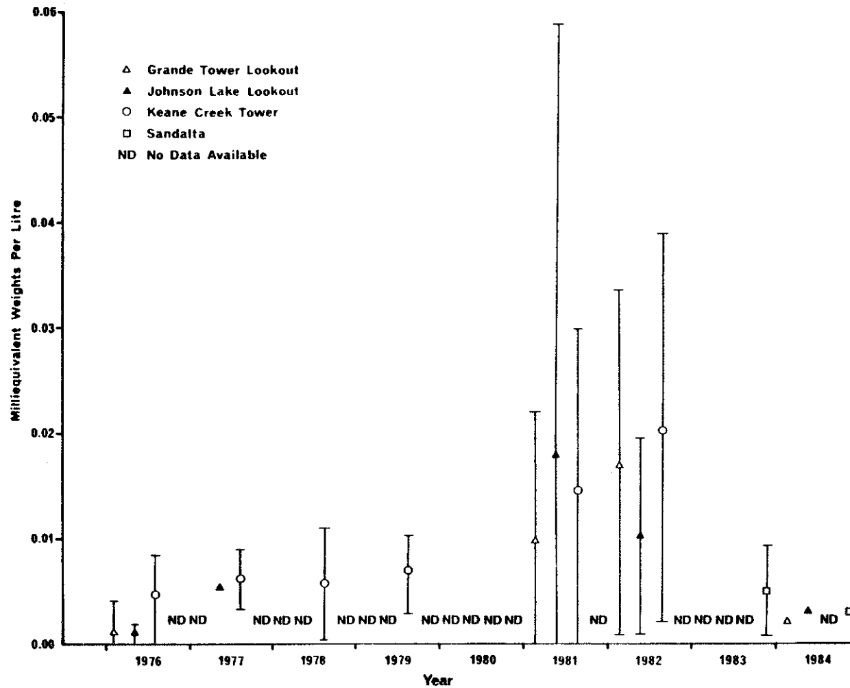
Figure 22. Annual mean ammonium ion concentrations at selected stations in the AOSERP network.
