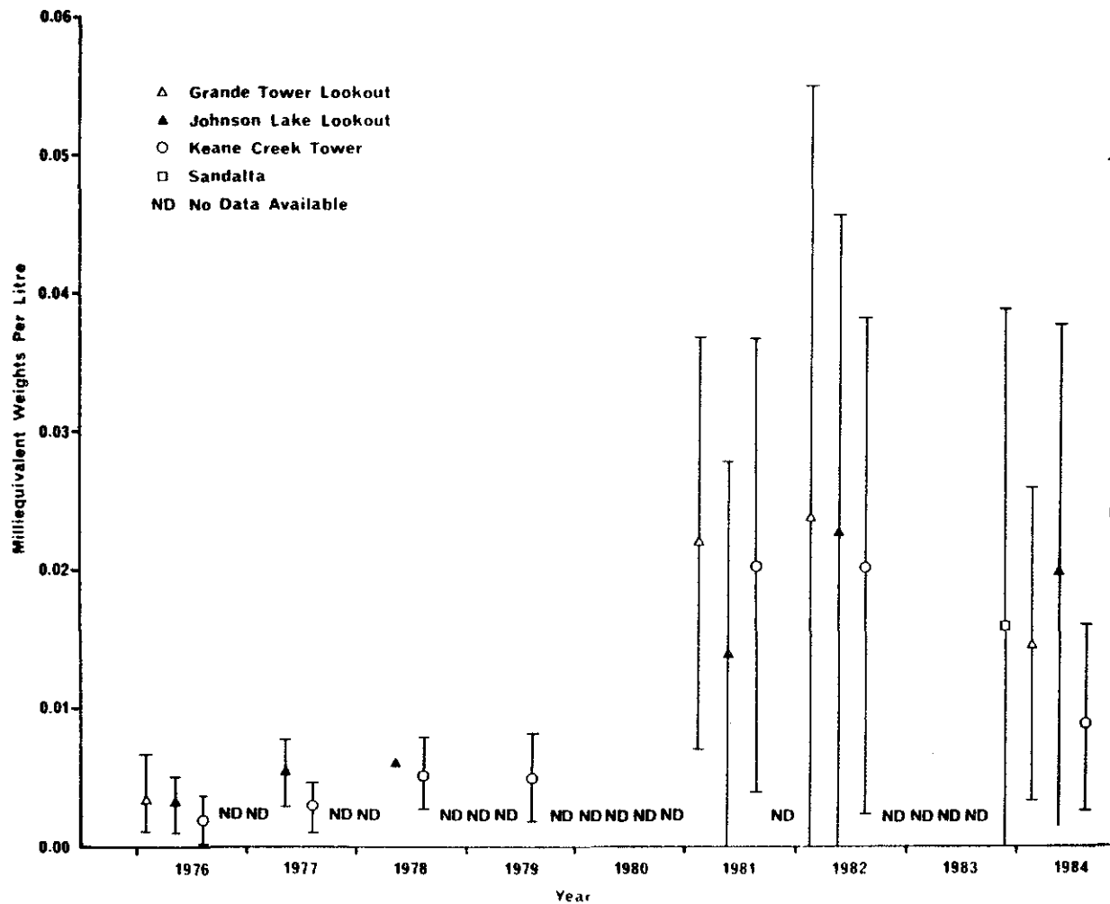
Figure 20. Annual mean sulphate ion concentrations at selected stations in the AOSERP network.
