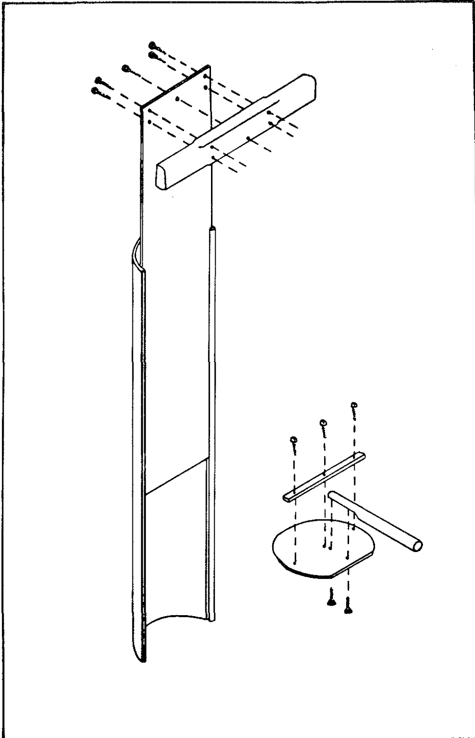
Figure 6. Snow corer.
