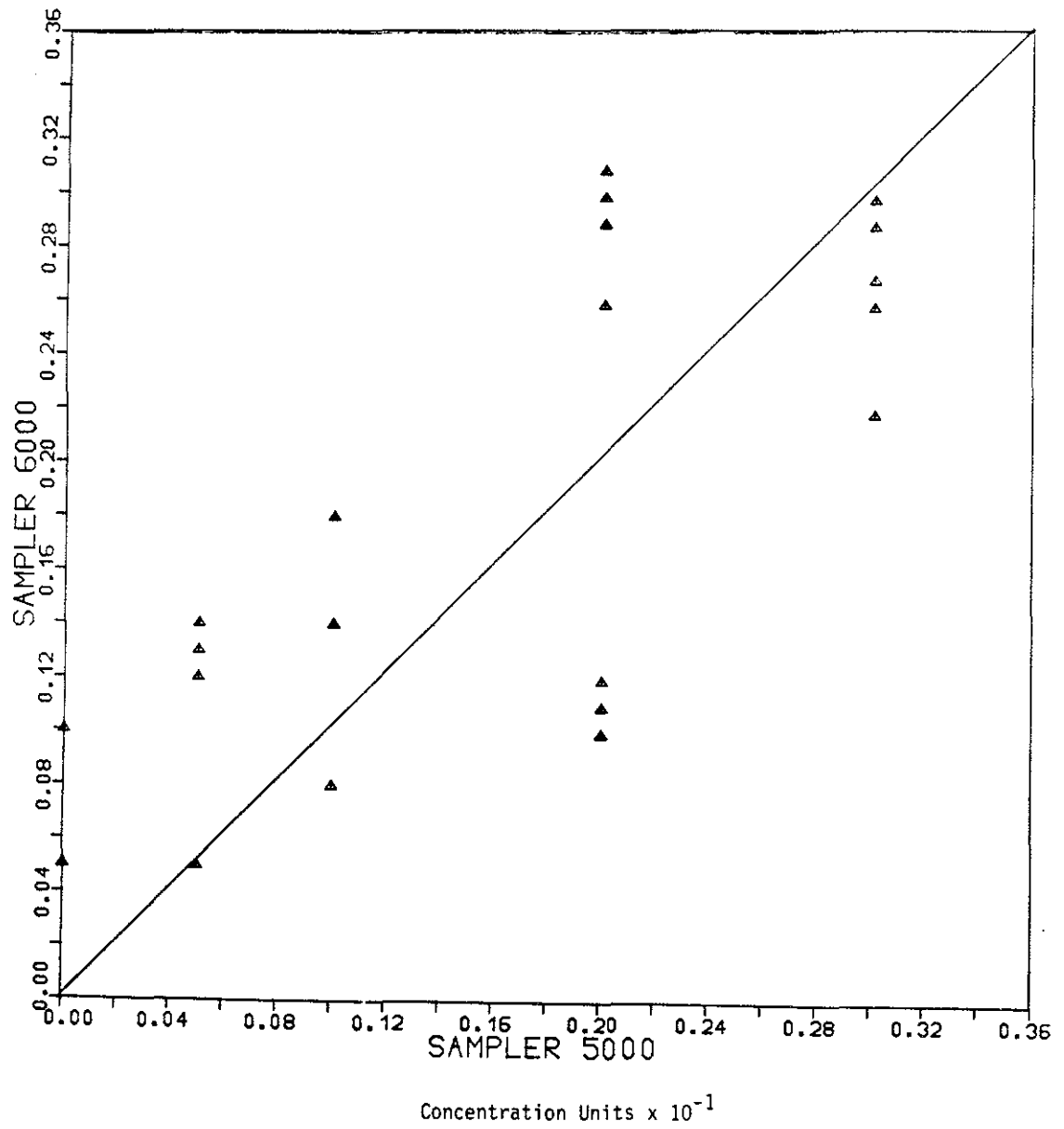
Figure 67. Plot of 1983 co-located sampling data for Mg^{2+} .
