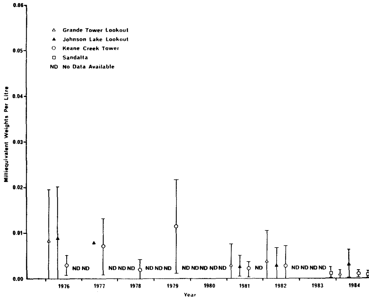
Figure 24. Annual mean sodium ion concentrations at selected stations in the AOSERP network.
