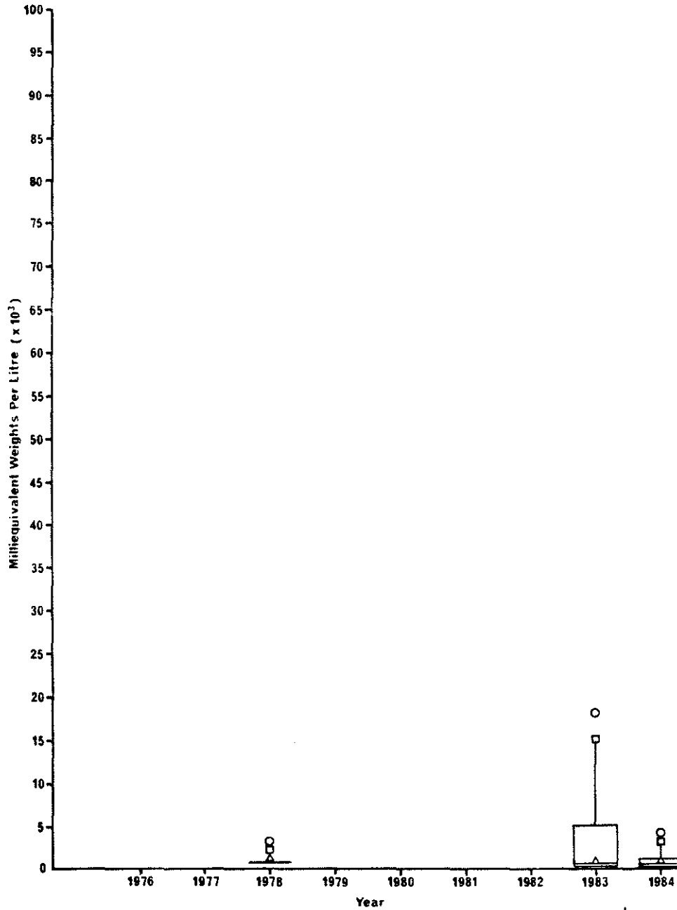
Figure 36. Box plots for the annual distribution of K^+ in snow samples in the AOSERP network.
