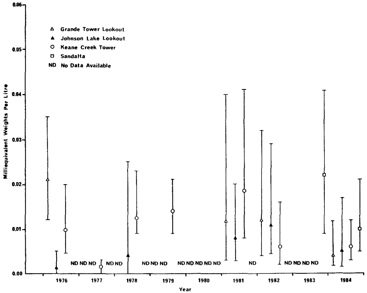
Figure 21. Annual mean hydrogen ion concentrations at selected stations in the AOSERP network.
