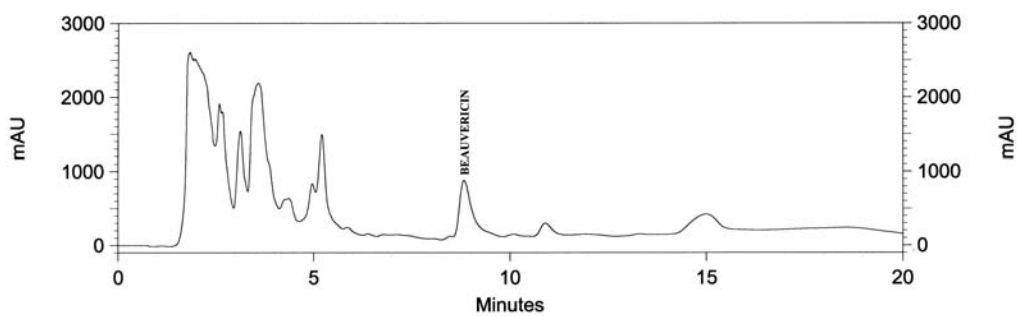
Figure 3.12. Chromatogram representing signal generated at 205 nm by injecting 20 µl of SR-25 methanol extraction. Signal measured in milliabsorbance units (mAU).
