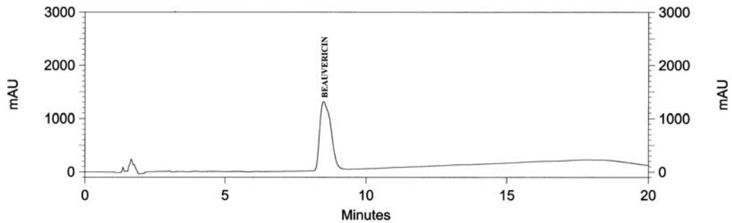
Figure 3.4. Chromatogram representing signal generated at 205 nm by injecting 20 \mu l of 1000 \mu M standard beauvericin. Signal measured in milliabsorbance units (mAU).
