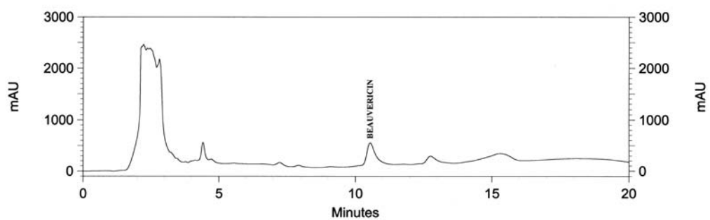
Figure 3.14. Chromatogram representing signal generated at 205 nm by injecting 20 µl of SR-35 methanol extraction. Signal measured in milliabsorbance units (mAU).
