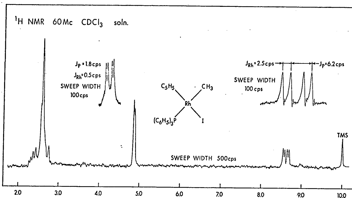
FIGURE 22: The ^1\text{H} NMR Spectrum of \text{CpRhP}(\text{C}_6\text{H}_5)_3\text{CH}_3\text{I} .
