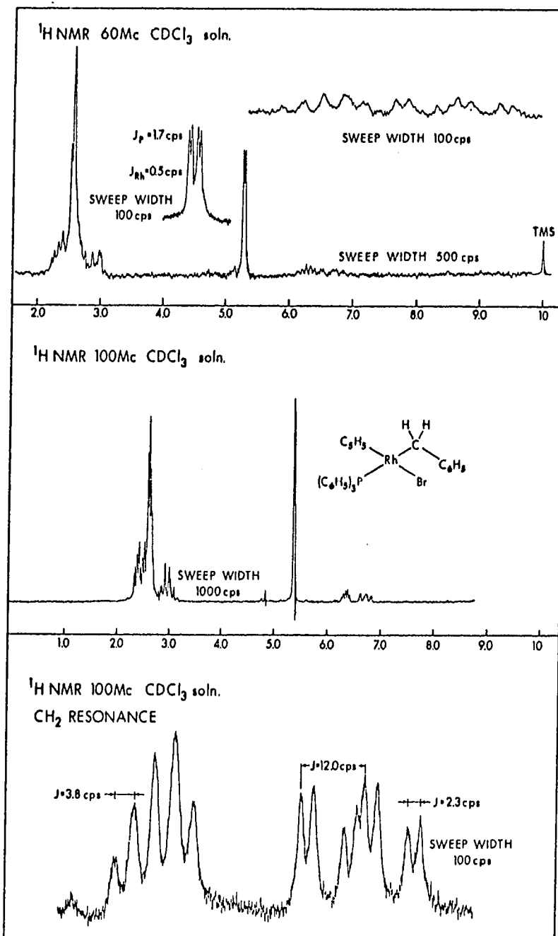
FIGURE 24: The ^1\text{H} NMR Spectrum of \text{CpRhP}(\text{C}_6\text{H}_5)_3(\text{CH}_2\text{C}_6\text{H}_5)\text{Br} .
