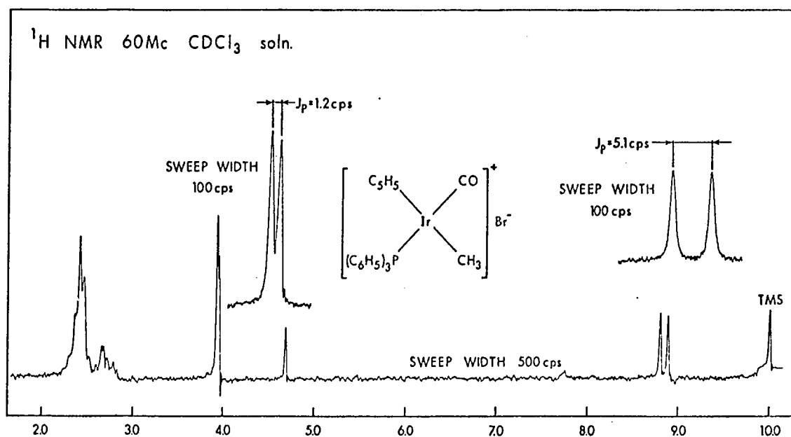
FIGURE 21: The ^1\text{H} NMR Spectrum of [\text{CpIrP}(\text{C}_6\text{H}_5)_3(\text{CO})\text{CH}_3]^+ \text{Br}^- .
