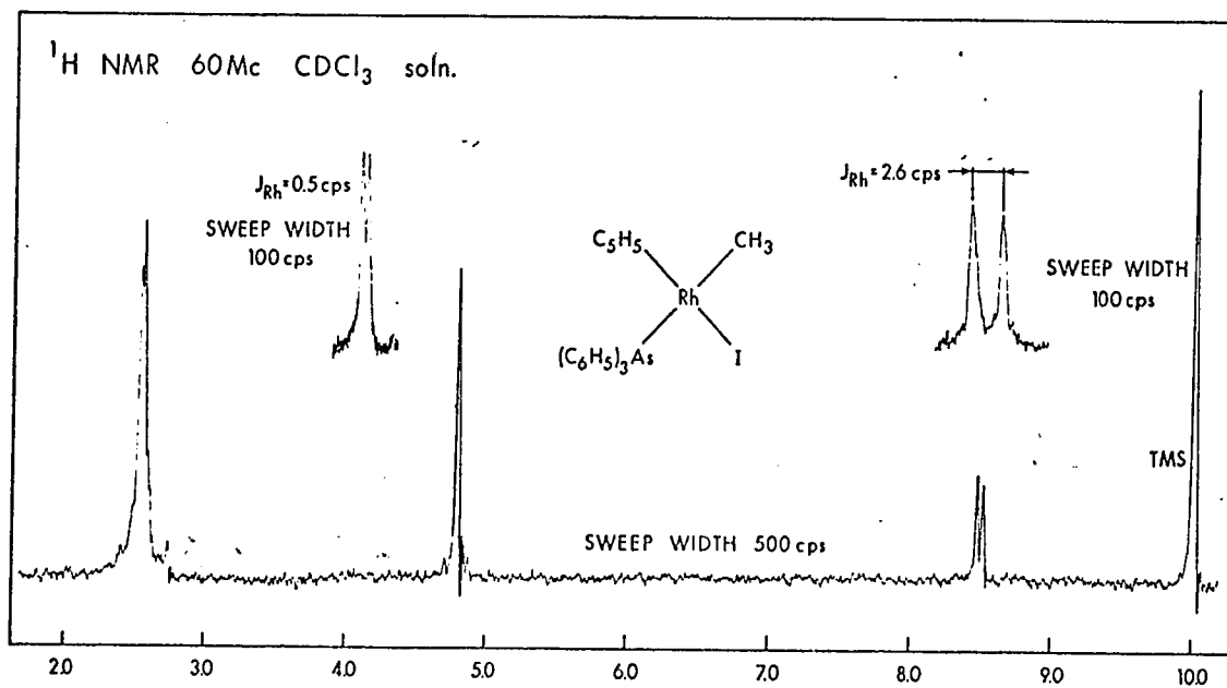
FIGURE 23: The ^1\text{H} NMR Spectrum of \text{CpRhAs}(\text{C}_6\text{H}_5)_3\text{CH}_3\text{I} .
