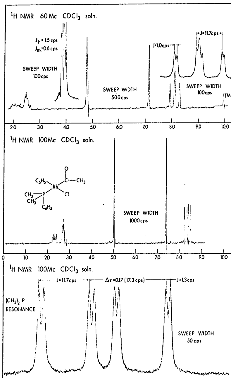
FIGURE 17: The ^1\text{H} NMR Spectrum of \text{CpRhP}-(\text{CH}_3)_2\text{C}_6\text{H}_5(\text{COCH}_3)\text{Cl} .
