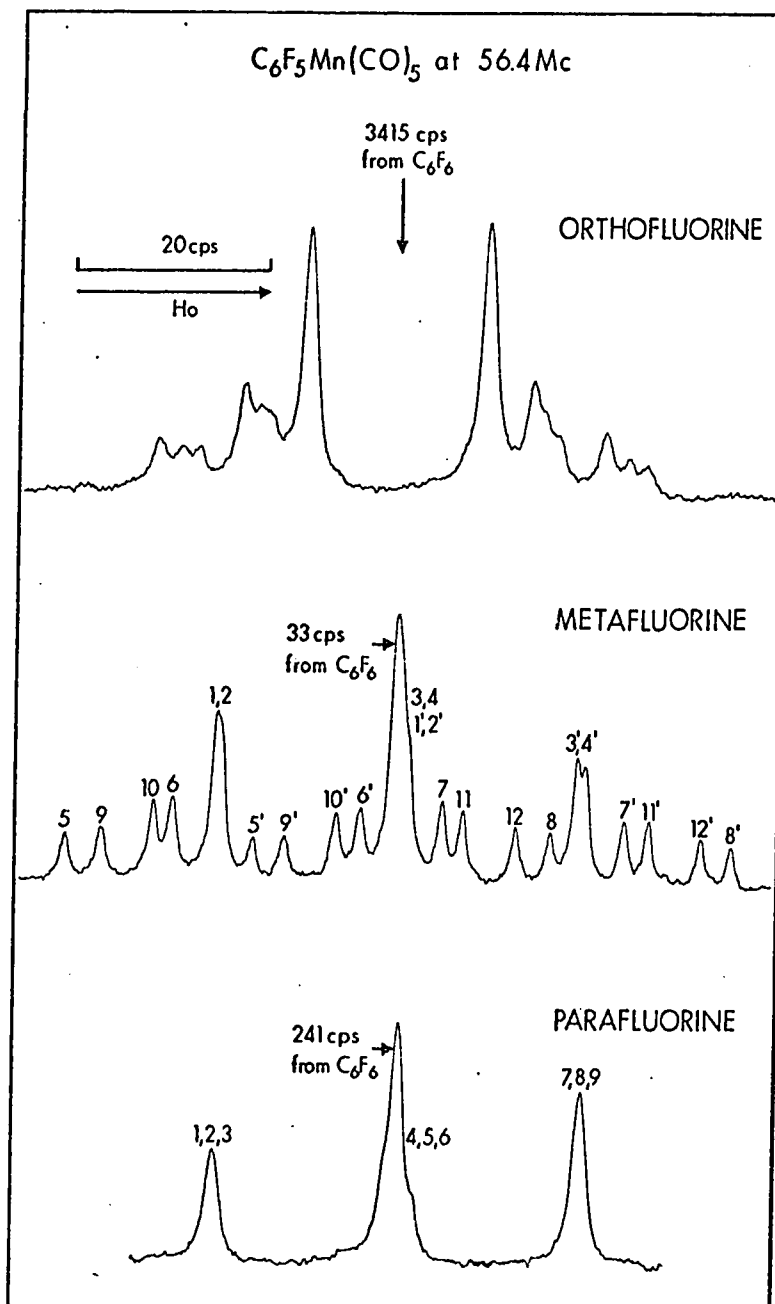
FIGURE 16. The ^{19}F NMR Spectrum of C_6F_5Mn(CO)_5 in acetone solution.
