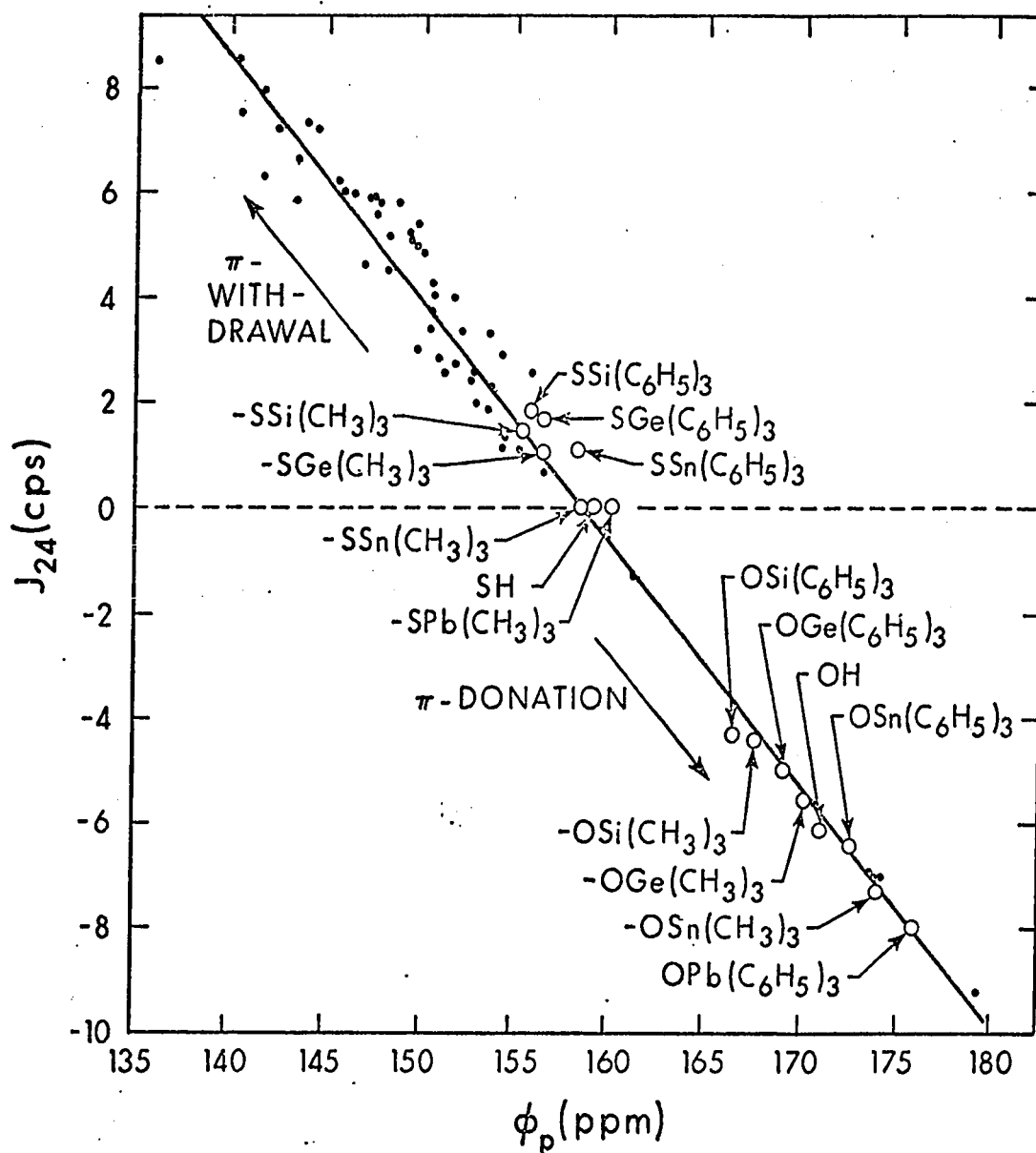
FIGURE 5. The J_{24} - \phi_p relationship for compounds of the type \text{C}_6\text{F}_5\text{-XMR}_3 where \text{X}=\text{O} or \text{S} , \text{M}=\text{Si} , \text{Ge} , \text{Sn} and \text{Pb} , \text{R}=\text{CH}_3 or \text{C}_6\text{H}_5 .
