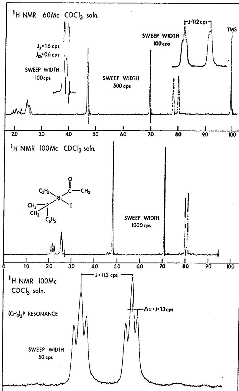
FIGURE 19: The ^1\text{H} NMR Spectrum of \text{CpRhP}(\text{CH}_3)_2\text{C}_6\text{H}_5(\text{COCH}_3)\text{I} .
