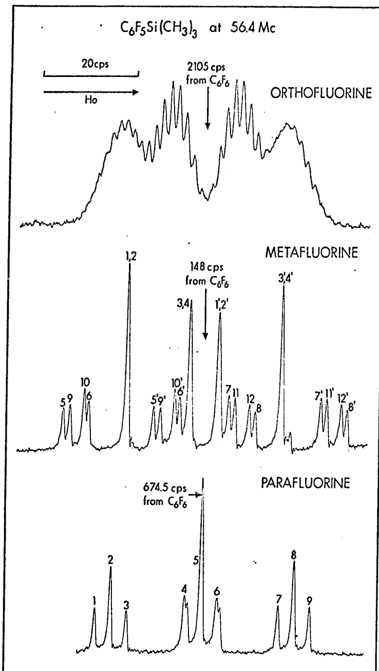
FIGURE 7. The ^{19}F nmr spectrum of C_6F_5Si(CH_3)_3 .
