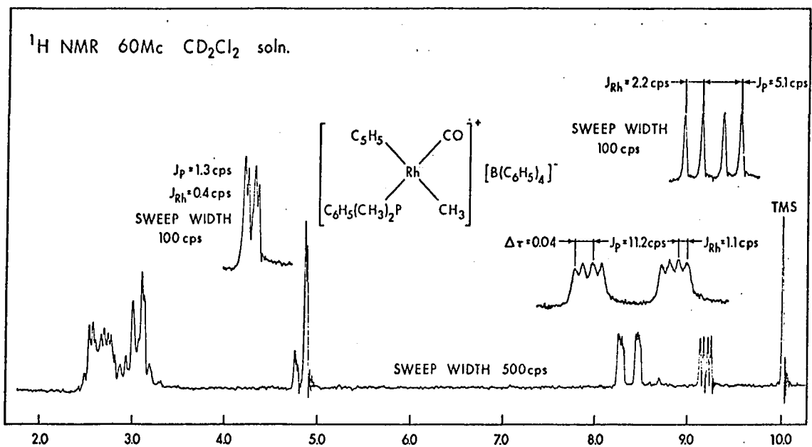
FIGURE 20: The ^1\text{H} NMR Spectrum of [\text{CpRhP}(\text{CH}_3)_2\text{C}_6\text{H}_5(\text{CO})\text{CH}_3]^+ [\text{B}(\text{C}_6\text{H}_5)_4]^-
