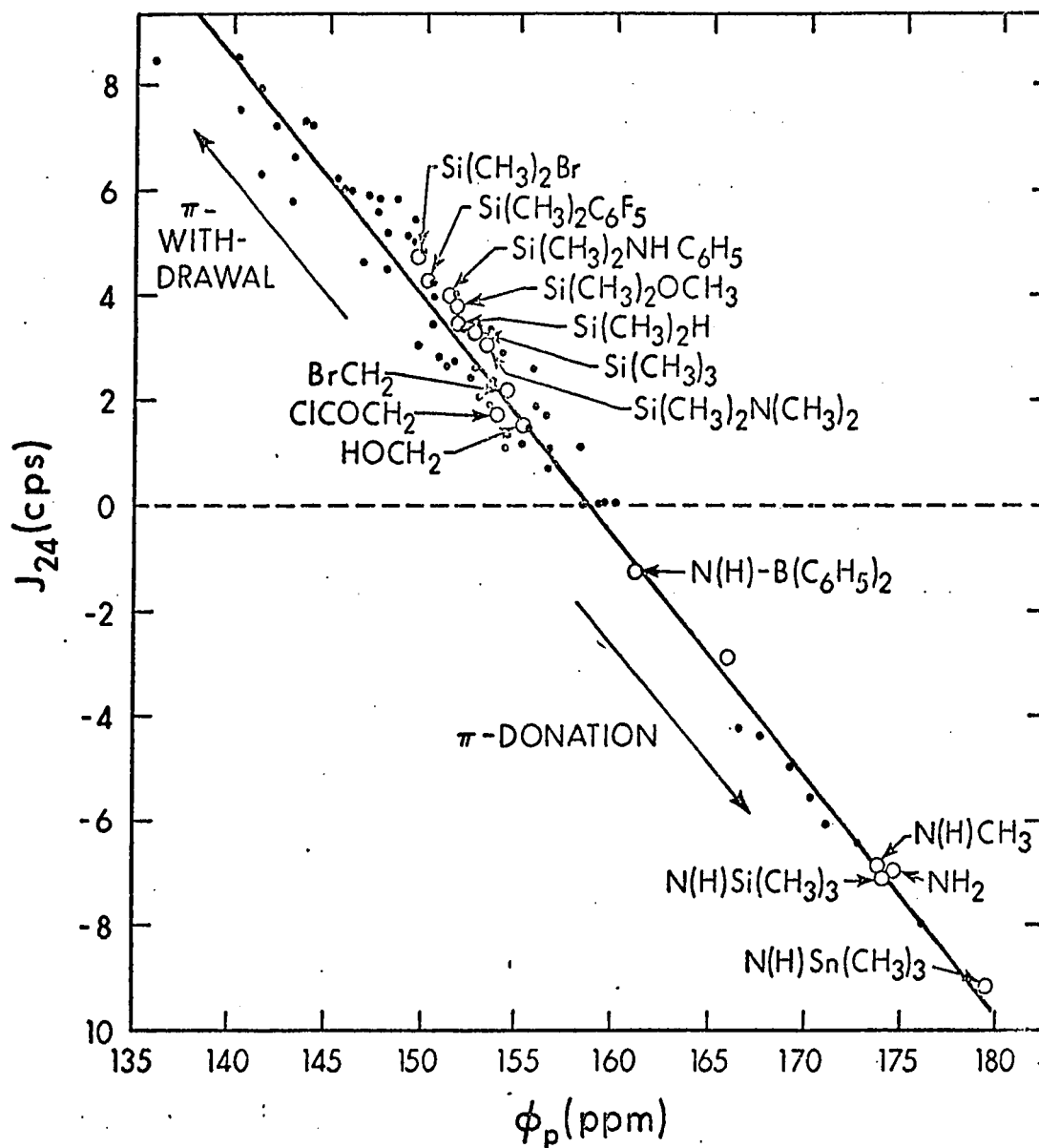
FIGURE 6. The J_{24} - \phi_p relationship for some pentafluorobenzyl and pentafluoroaniline derivatives and the compounds \text{C}_6\text{F}_5(\text{CH}_3)_2\text{SiX} where \text{X} = \text{H}, \text{CH}_3, \text{C}_6\text{H}_5, \text{OCH}_3, \text{N}(\text{CH}_3)_2 or \text{N}(\text{H})\text{C}_6\text{H}_5 .
