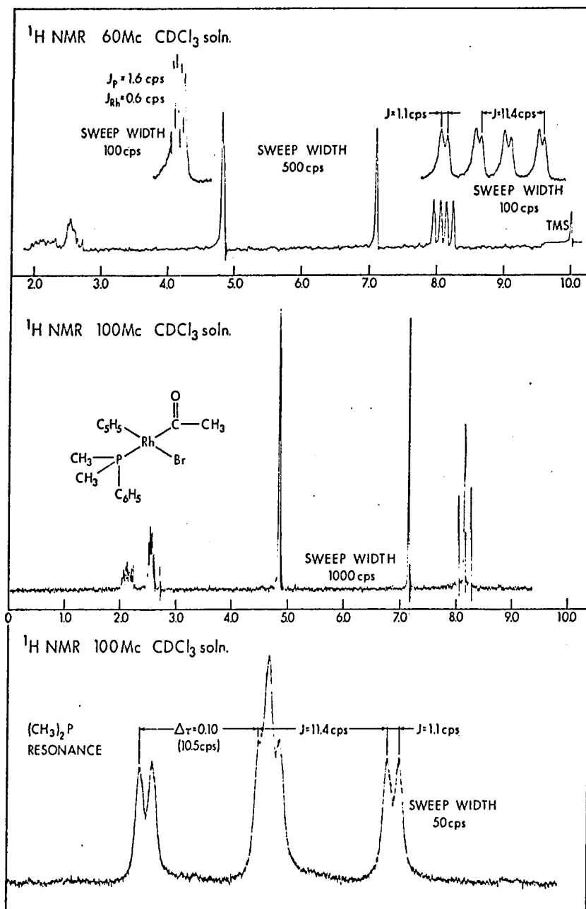
FIGURE 18. The ^1\text{H} NMR Spectrum of \text{CpRhP}(\text{CH}_3)_2\text{C}_6\text{H}_5(\text{COCH}_3)\text{Br} .
