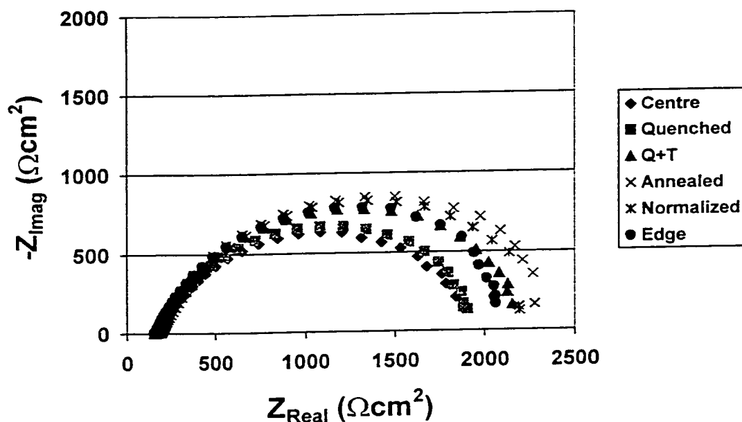
Figure 5-9: Comparison of the various X-70 microstructures using EIS without the low frequency data
