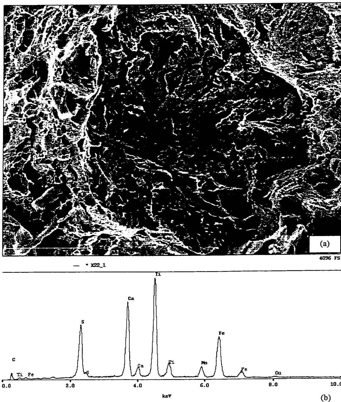
Figure 6-11: (a) Quasi-cleavage fracture surface, (b) EDX analysis of the centrally located precipitate
