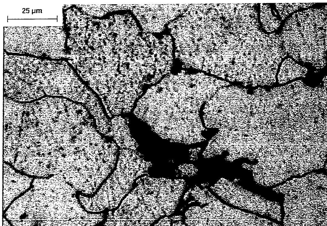
Figure 4-12: Annealed X-70 microstructure
