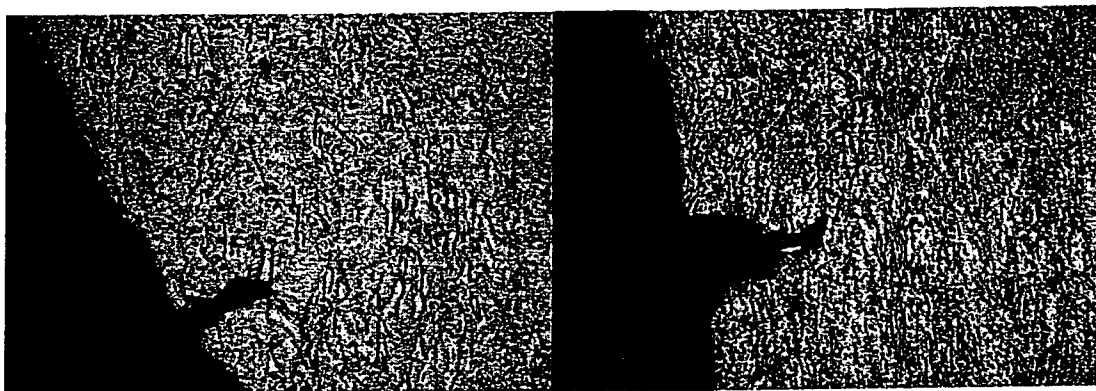
Figure 6-7: Shallow cracks in as-received X-70
