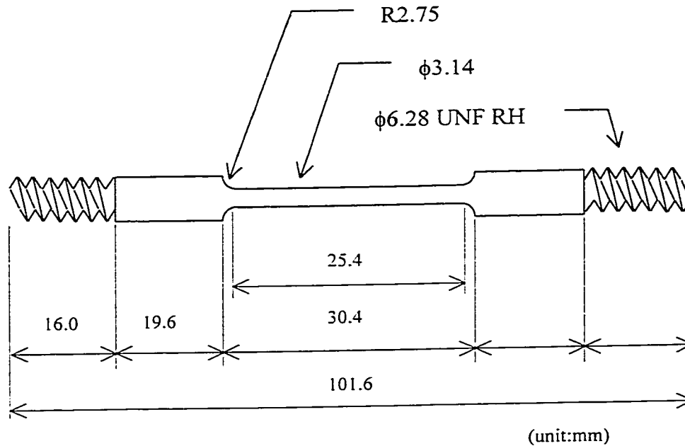
Figure 3-1: SSRT specimen
