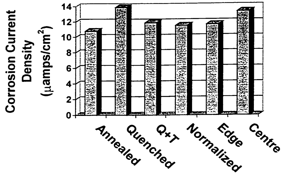
Figure 5-5: Corrosion current of various X-70 microstructures as determined from the polarization resistance
