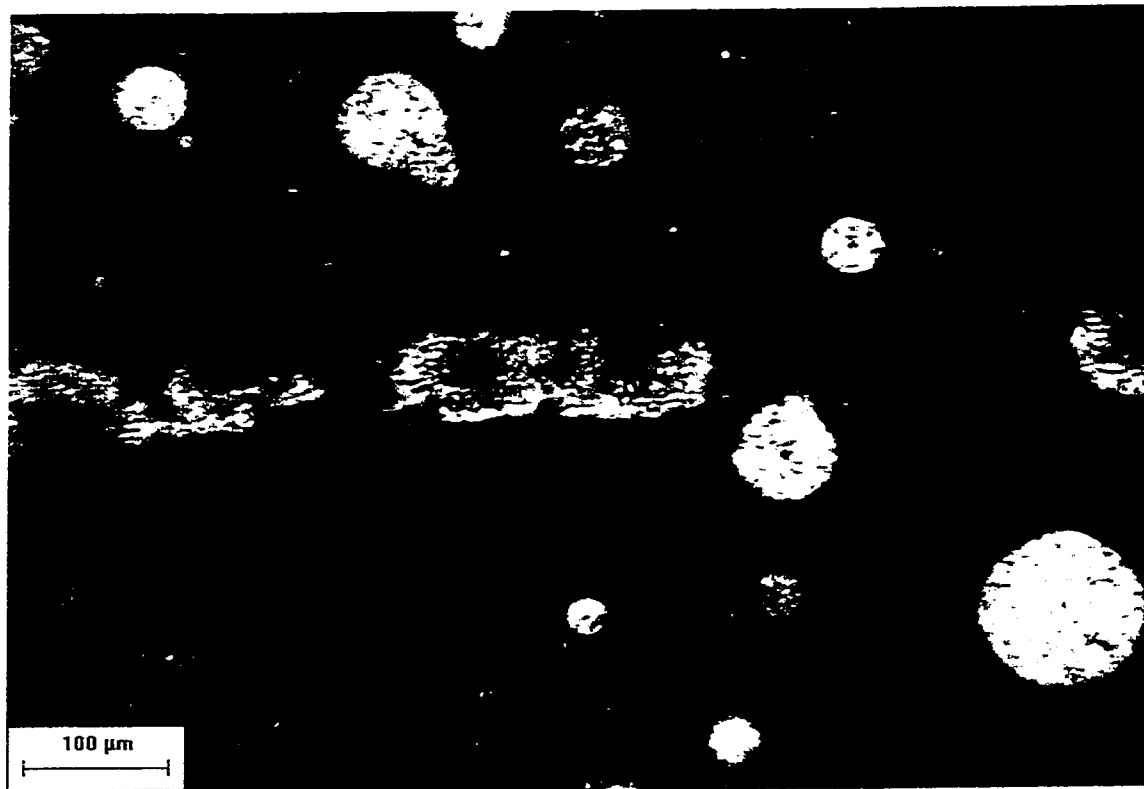
Figure 5-11: X-70 corrosion surface after being exposed to NS4 for 7 days
