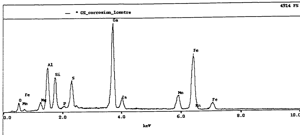
Figure 5-24: Composition of inclusion in the previous figure
