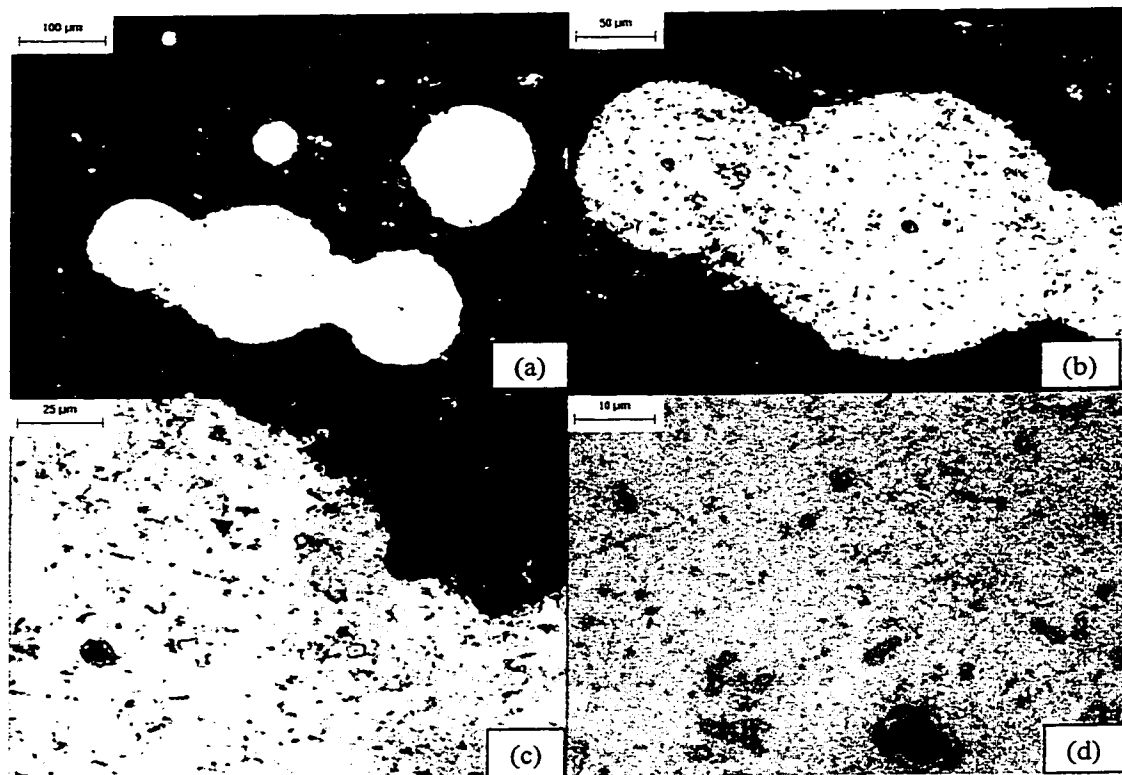
Figure 5-17: Irregular shaped cathodic area, (a) 200x, (b) 400x, (c) 800x, (d) 2000x
