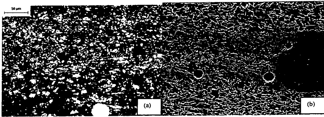
Figure 5-19: Influence of the calcium sulphide inclusion on the corrosion surface (a) optical microscope view, the four dark spots across the middle are the original locations of inclusions (b) SEM view and the dark spots are the original location of the inclusions
