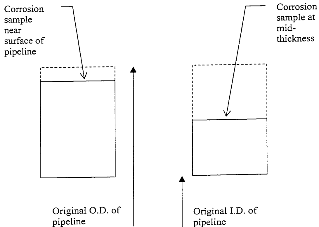
Figure 5-27: Schematic showing the sectioning of the pipeline to get samples with varying amounts of retained austenite and inclusions
