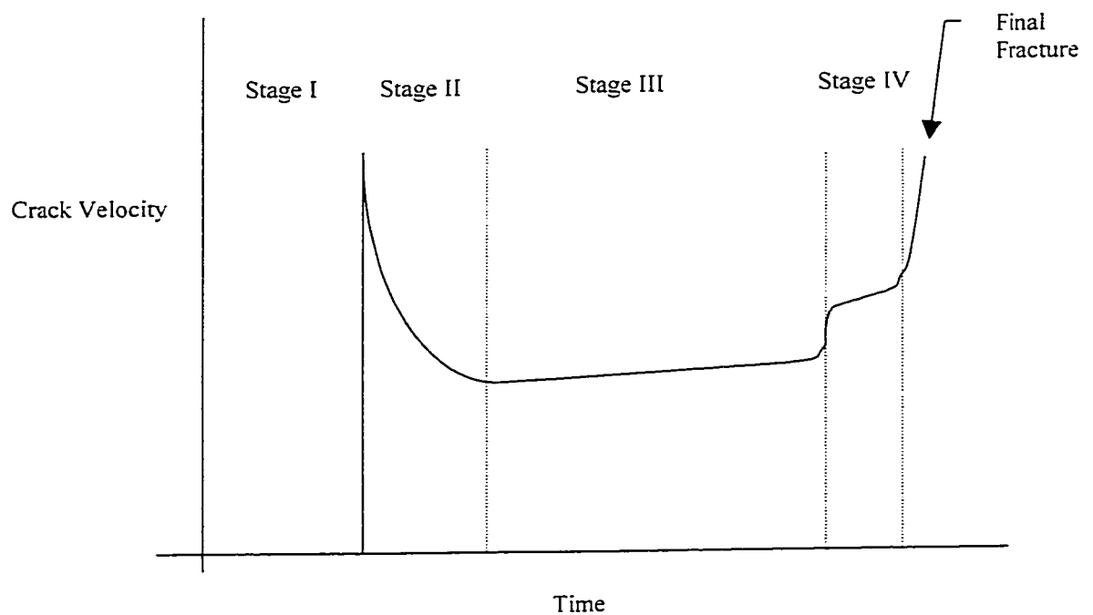
Figure 2-1: Sequence of events for SCC as a function of time
