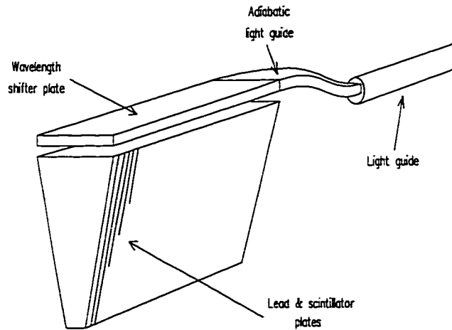
Figure 26: The construction of one end cap module.
