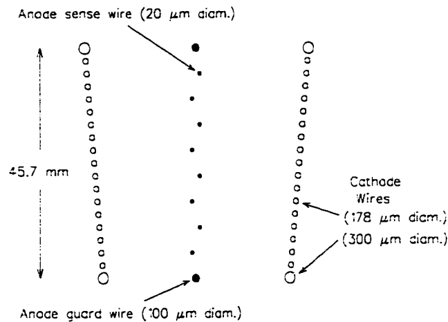
Figure 23: View of a single drift chamber cell.
