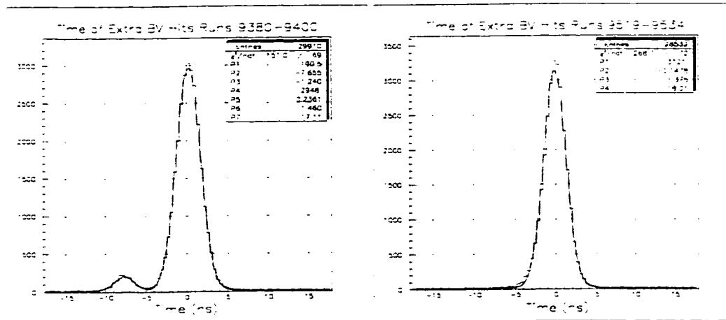
Figure 53: Timing of excess BV energy at two different portions of the run.
