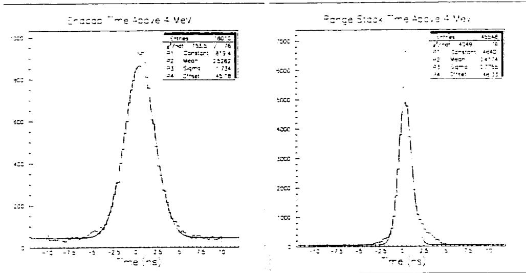
Figure 43: INTIME time distribution for events above 4MeV visible energy. The fit is to the equation y = p_4 + p_1 e^{-(x-p_2)^2/2p_3^2}
