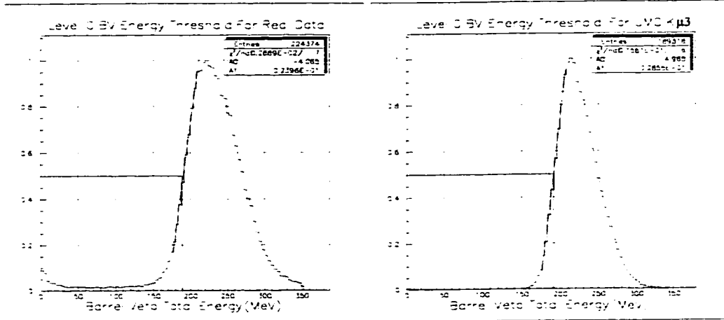
Figure 32: Total BV energy within \pm 6.3 ns of prompt for real \pi\gamma\gamma(2) level 0 data and UMC level 0 K\mu 3 data. (Distribution normalized to unit height).
