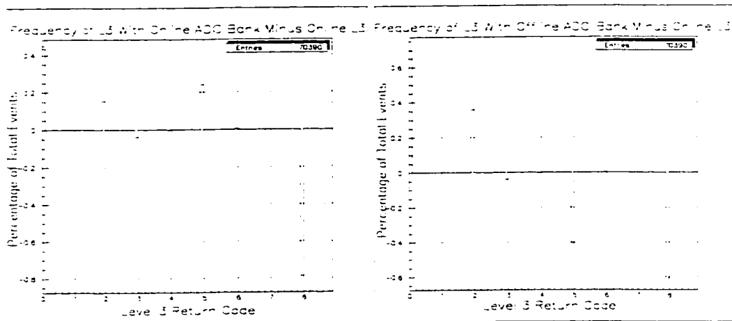
Figure 39: Difference in frequency of level 3 return codes expressed as a percentage of total number of events for online or offline BV ADC banks compared to actual online return codes.
