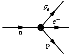
Figure 3: Nuclear beta decay in terms of nucleons.
