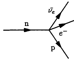
Figure 4: Nuclear beta decay in the Fermi theory.
