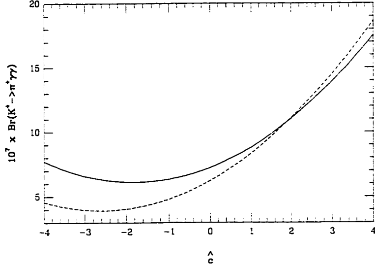
Figure 10: K^+ \rightarrow \pi^+ \gamma \gamma branching ratio prediction as a function of \hat{c} at O(p^4) (dashed line) and including the O(p^6) unitarity correction (solid line).
