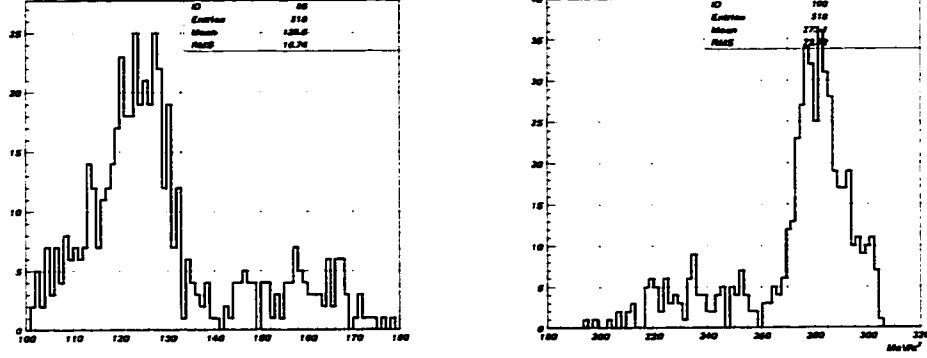
Figure 69: \pi^+ momentum (left) and photon invariant mass (right) distributions for the events which passed all cuts except for PHICUT and ZCUT. K\pi 3 background dominates in the region of P_{\pi^+} < 133 \text{ MeV}/c , or equivalently, in the region of M_{\gamma\gamma} > 270 \text{ MeV}/c^2 .
