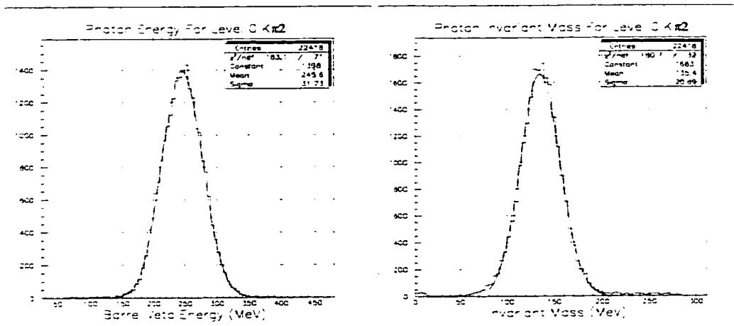
Figure 31: K\pi 2 photon energy and invariant mass using a BV visible fraction of 0.308.
