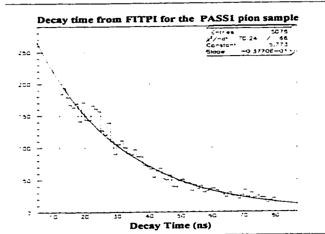
Figure 92: Pion decay time for PASS1 pion sample.
