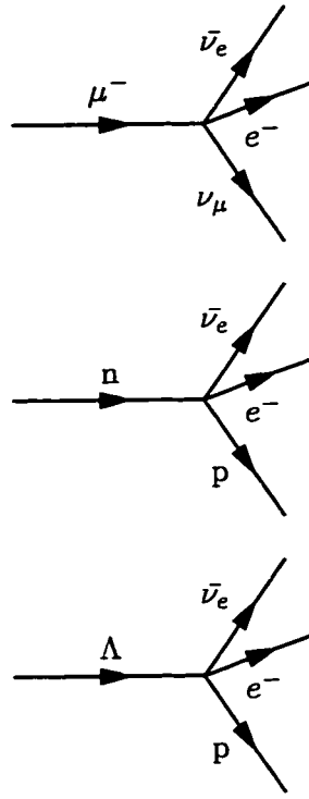
Figure 5: Fermi theory diagrams for muon decay, nuclear beta decay and \Lambda beta decay.
