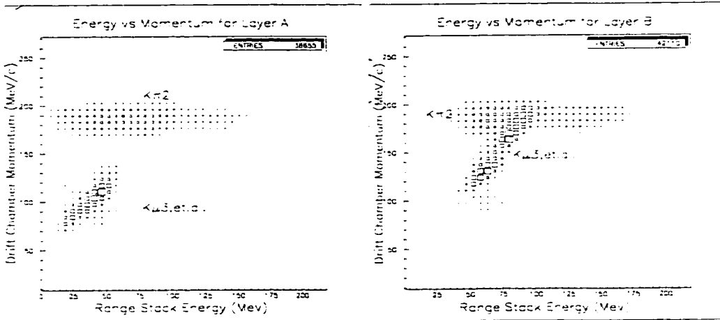
Figure 90: Range stack energy versus DC momentum in \pi\gamma\gamma(2) level 0 data
