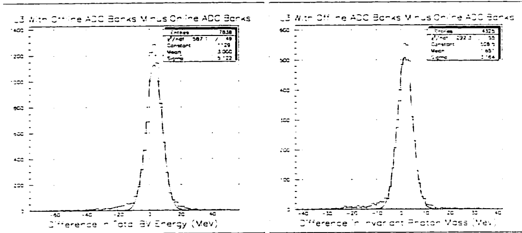
Figure 40: Level 3 BV energy and M_{\gamma\gamma} found using the new ADC banks minus those found using the online calibrated ADC banks.
