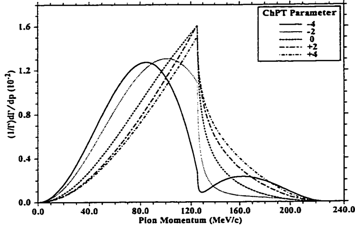
Figure 97: The theoretical \pi^+ momentum distribution for various values of \hat{c} .
