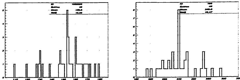
Figure 82: The \pi^+ momentum of the non-overlapping gamma background (left) and two photon invariant mass calculated using the \pi^+ momentum (right). All Set-II cuts were applied except that for the \cos(\theta_{\pi X}) cut which was reversed.
