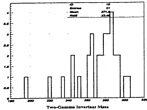
Figure 99: The KINFIT-returned invariant photon mass of the final event sample.
