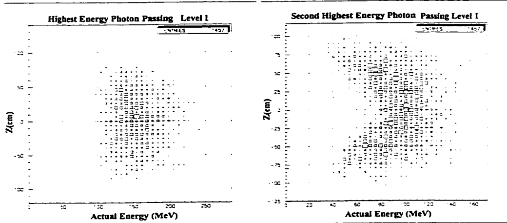
Figure 38: Z distribution versus photon energy for the highest and second highest energy photon clusters in the BV from UMC data.
