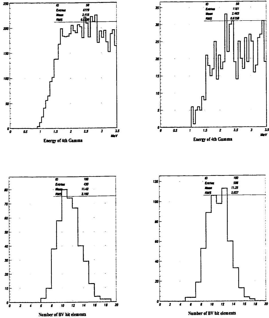
Figure 74: The energy distribution of the 4th photon cluster in PASS2 data (top left) and UMC generated K\pi 3 data (top right) and the total number of hit BV elements in real data below the K\pi 3 threshold which failed PHICUT (bottom left) and UMC-generated K\pi 3 (bottom right).
