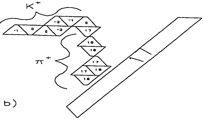
Figure 21: A typical K^+ \rightarrow \pi^+ decay in the target showing ADC (top) and TDC (bottom) information.
