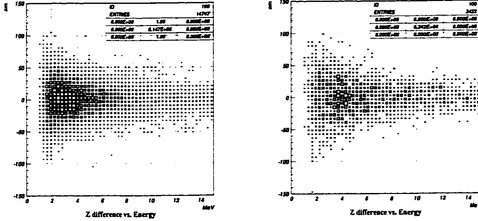
Figure 73: The difference between the ADC and TDC based z measurements in the BV ( z_{ADC} - z_{TDC} ) as a function of photon energy for real data (left) and UMC data (right).
