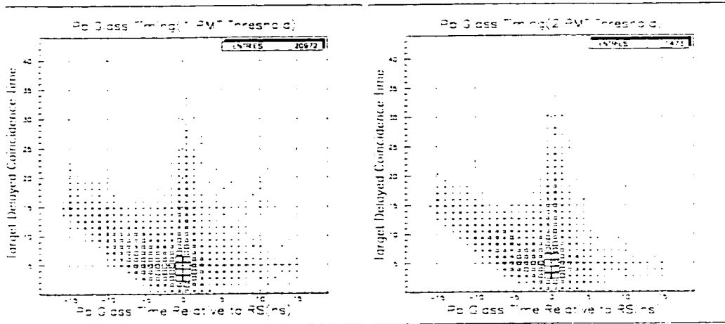
Figure 55: Time of Pb glass hits versus delayed coincidence time.
