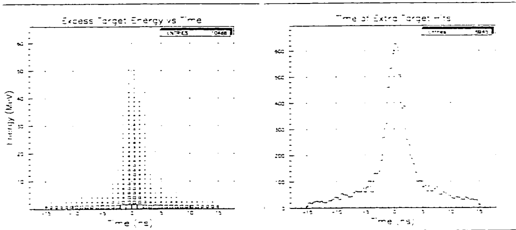
Figure 54: Excess energy in the target relative to target pion time.
