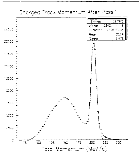
Figure 45: Total charged track momentum for events surviving PASS1.
