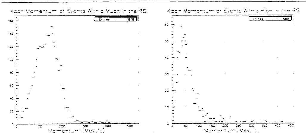
Figure 60: Missing kaon momentum in \pi\gamma\gamma(2) events selected to contain either muons or pions.
