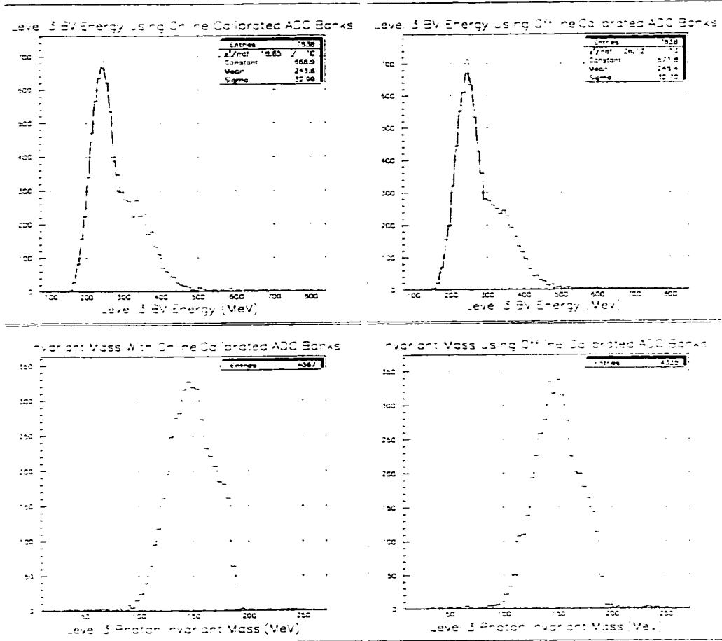
Figure 41: Level 3 BV energy and M_{\gamma\gamma} for K\pi 2 events calculated using the new ADC banks and using the online calibrated ADC banks.
