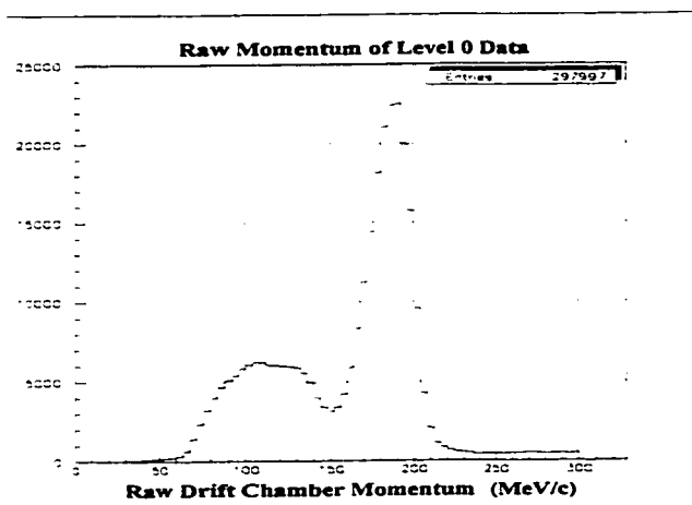
Figure 83: Raw DC momentum in \pi\gamma\gamma(2) level 0 data
