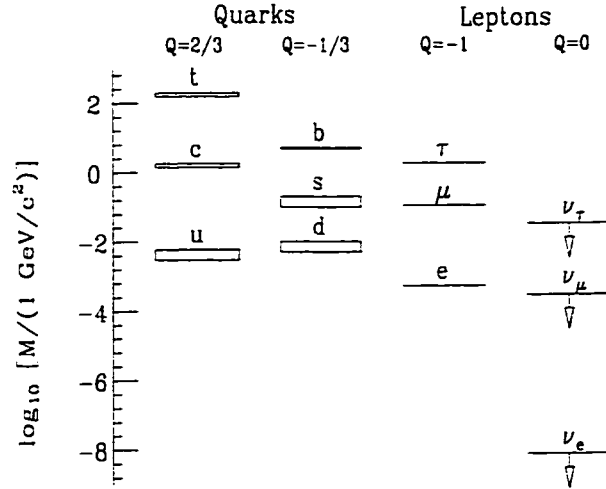
Figure 6: Quark masses on a logarithmic scale, widths indicate uncertainties in the values.
