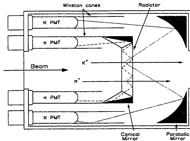
Figure 17: Schematic showing the design of the Cherenkov counter and a typical light path for both pion and kaon Cherenkov light.
