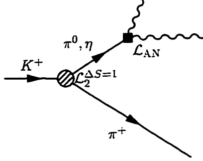
Figure 8: The anomalous diagram contributing at O(p^4) to K^+ \rightarrow \pi^+ \gamma \gamma .
