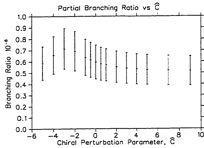
Figure 98: The \pi\gamma\gamma(2) partial branching ratio as a function of \hat{c} . Only statistical errors are shown.
