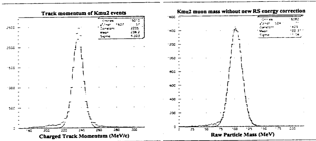
Figure 89: Charged track momentum and mass for the K\mu 2 sample.
