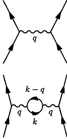
Figure 1: A tree level Feynman graph showing exchange of a virtual photon between two fermions and the same graph with a virtual loop on the photon line.
