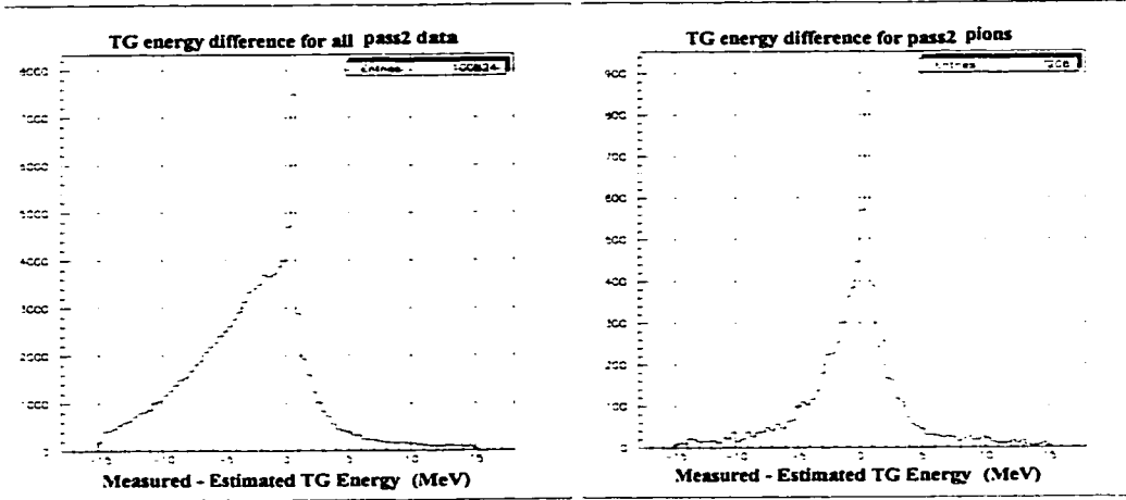
Figure 48: \Delta E_{TG} energy difference for all PASS2 data and PASS2 pions selected using TD cuts.
