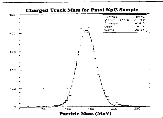
Figure 87: Charged track mass in K\pi^3 sample.
