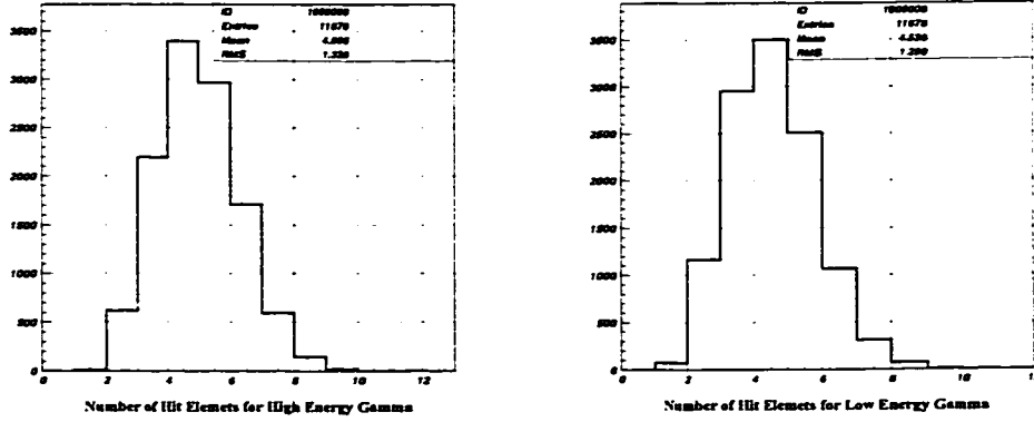
Figure 63: The number of hit BV elements in UMC generated \pi\gamma\gamma(2) data.
