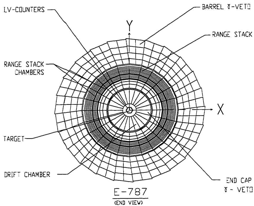
Figure 14: Schematic end view of the E787 detector showing the active elements in the center plane ( z=0 ) of the apparatus.
