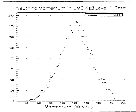
Figure 57: K\mu 3 neutrino momentum after passing the level 1 trigger (UMC data).
