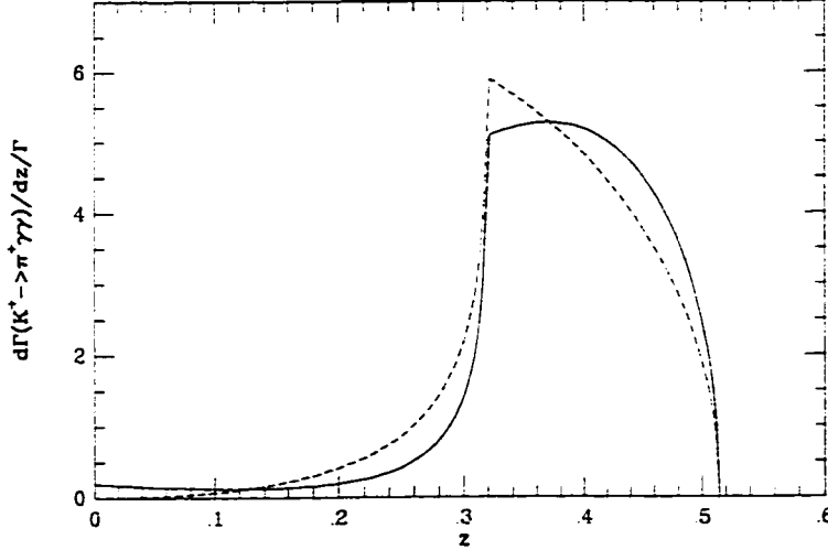
Figure 11: K^+ \rightarrow \pi^+ \gamma \gamma invariant photon mass spectrum at \hat{c} = 0 calculated to O(p^4) (dashed line) and with the inclusion of the O(p^6) unitarity correction (solid line).
