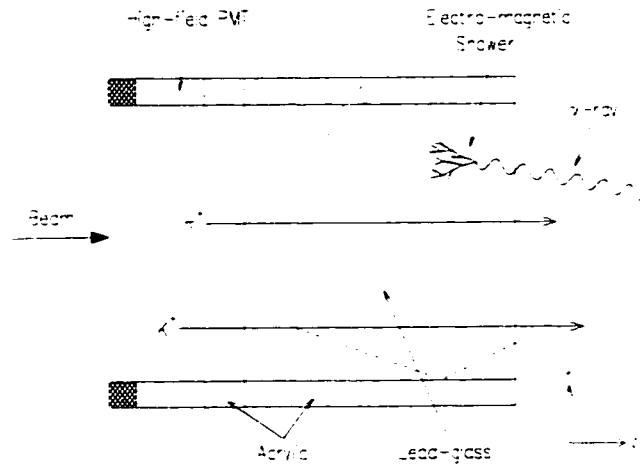
Figure 19: The typical effect of kaons, pions or high energy photons on the lead glass Cherenkov counter
