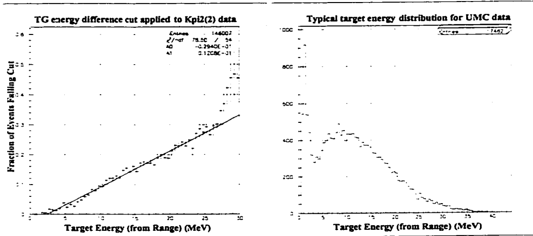
Figure 91: Fraction failing TG-energy-difference cut as a function of TG energy (from range) for K\pi 2(2) data and a typical UMC \pi\gamma\gamma(2) TG energy distribution.
