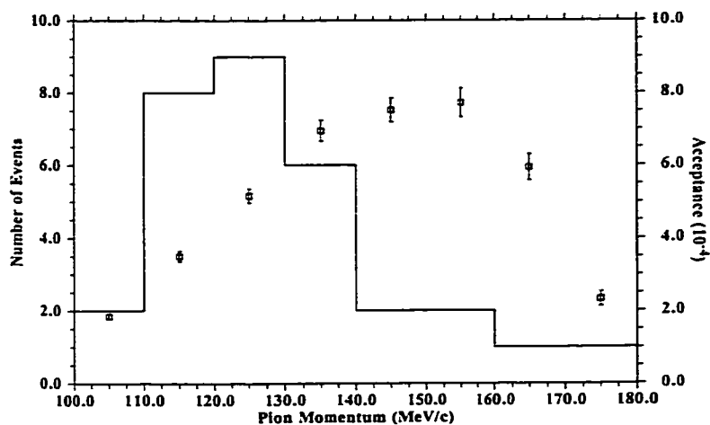
Figure 96: The measured total \pi^+ momentum of the final event sample (solid line) and the \hat{c} independent portion of the acceptance. The background (not shown) was 0.6 \pm 1.0 events per bin assuming a flat background.
