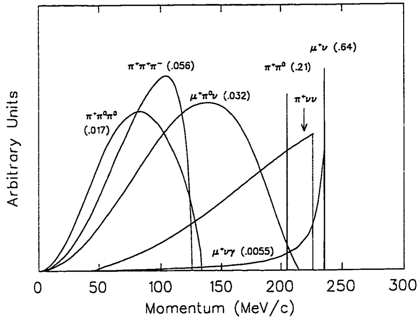
Figure 30: The charged particle momentum spectrum of the six most probable kaon decay modes excluding Ke3 and including \pi\nu\bar{\nu} .
