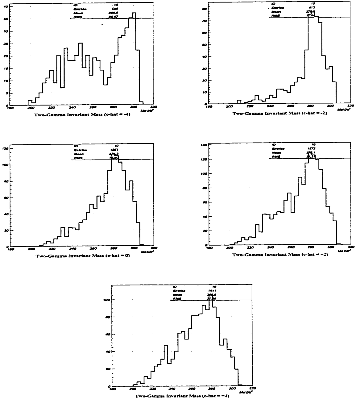
Figure 100: The KINFIT-returned invariant photon mass of UMC events using various \hat{c} values.
