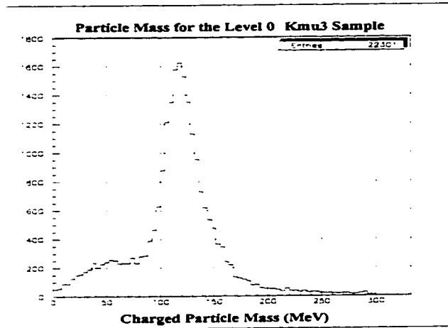
Figure 85: Charged track mass in K\mu 3 decays selected from \pi\gamma\gamma(2) level 0 data
