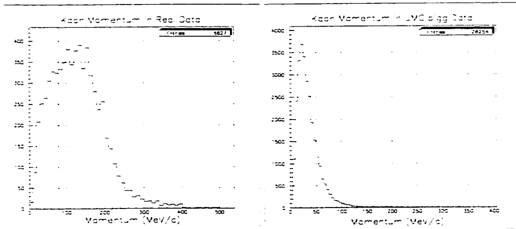
Figure 59: Missing kaon momentum in real \pi\gamma\gamma(2) data (left) and UMC \pi\gamma\gamma(2) data (right) after PASS1, photon veto, P_{\pi^+} and M_{\gamma\gamma} cuts. The solid vertical line in the left figure shows the missing momentum cut position at 86.6 MeV/c.
