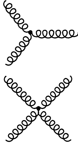
Figure 2: Gluon self interaction diagrams.
