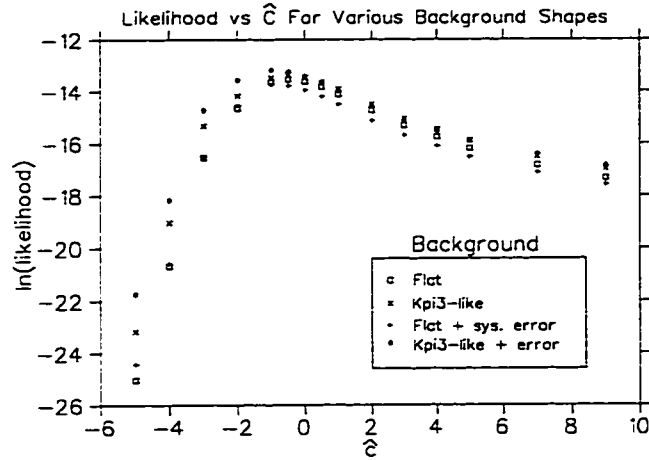
Figure 101: \ln \mathcal{L} vs \hat{c} for flat or K\pi 3 -like background shapes with and without systematic error in the background estimate.
