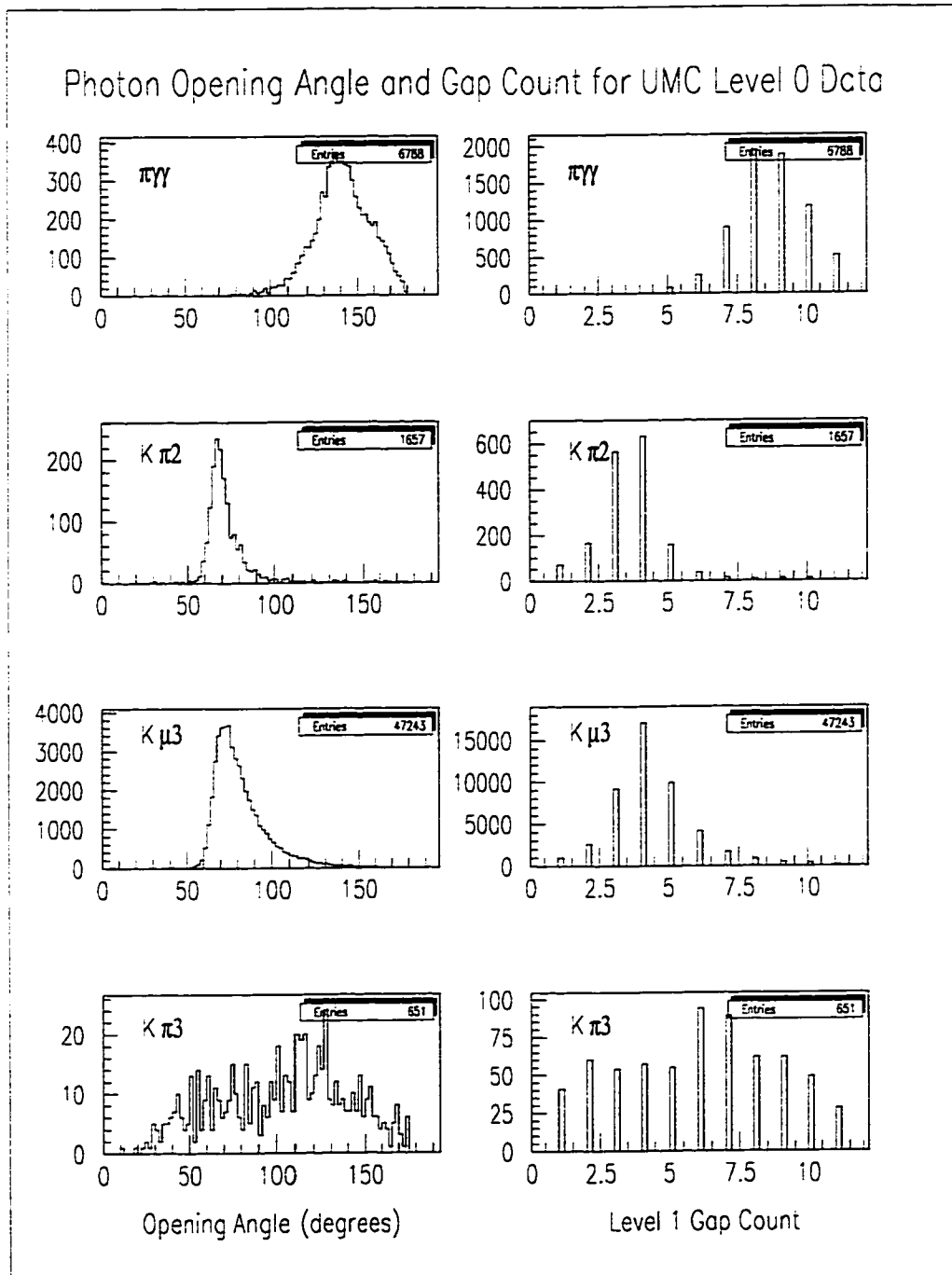
Figure 34: UMC-generated photon opening angle and gap count for various triggers.
