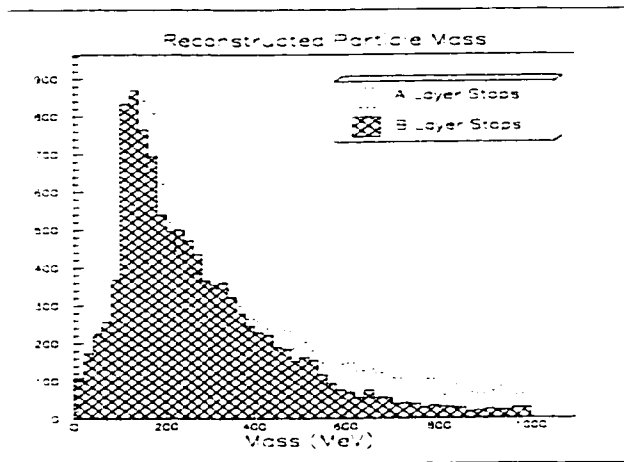
Figure 44: Charged track mass for A and B layer stops in \pi\gamma\gamma(2) after EC and RS photon vetoes.
