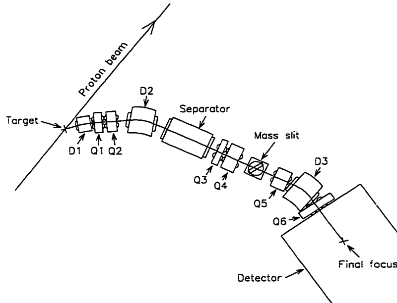
Figure 12: A schematic of the LESB 1 beamline used by E787 from 1988-1991.
