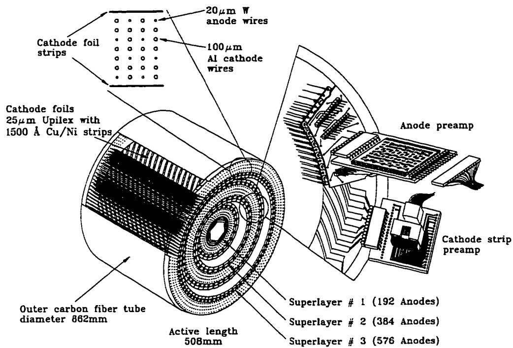
Figure 27: Schematic of the UTC showing the inside of the outer superlayer.
