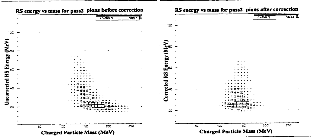
Figure 49: Mass vs RS energy for pions selected from PASS2 data using TD cuts, before and after the RS energy correction.
