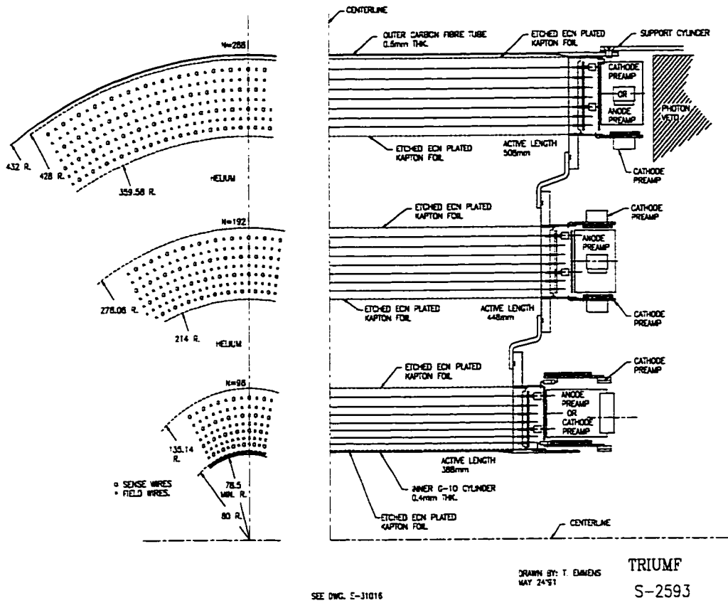
Figure 28: Schematic side view of the downstream end of the UTC and a portion of the wire layout.
