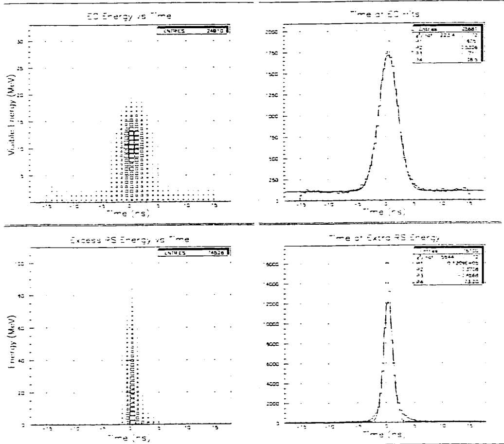
Figure 51: INTIME energy in the endcap and range stack (the corresponding PASS1 photon veto cuts have not been applied).
