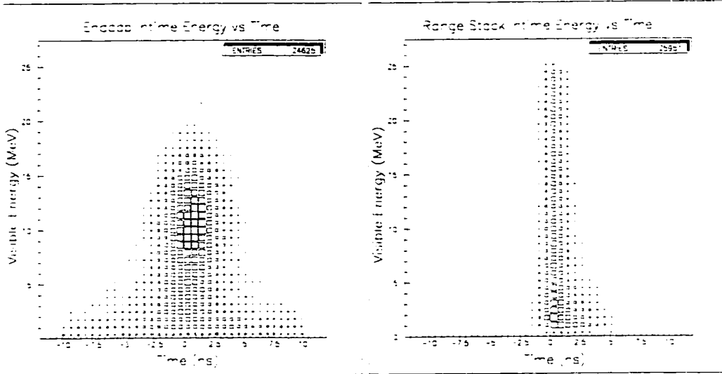
Figure 42: Typical INTIME energy/time distributions for raw \pi\gamma\gamma(2) data
