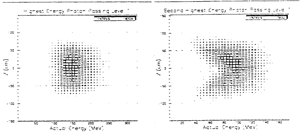
Figure 33: Z distribution versus real photon energy for the most energetic and second most energetic photon clusters in the BV.
