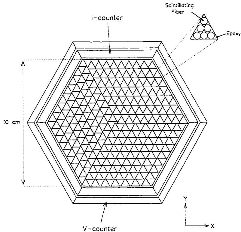
Figure 20: Cross section of the scintillating fiber target
