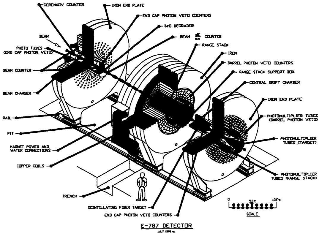
Figure 15: Isometric view of the E787 detector with the magnet sections separated.
