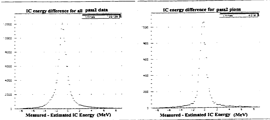
Figure 47: \Delta E_{IC} energy difference for all PASS2 data and PASS2 pions selected using TD cuts.
