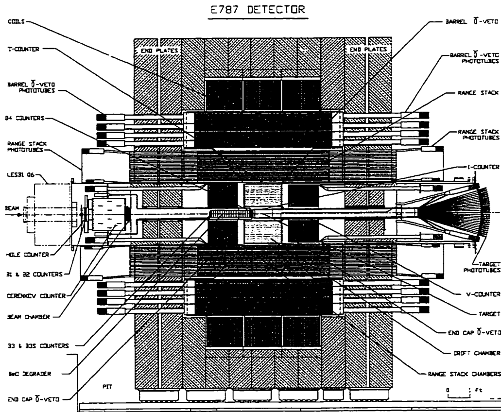
Figure 13: Cross sectional schematic side view of the E787 detector.
