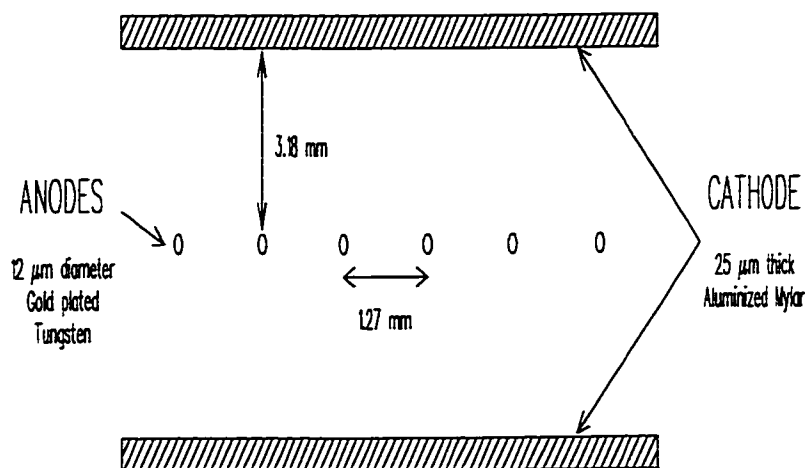
Figure 18: The layout of the beam proportional chamber
