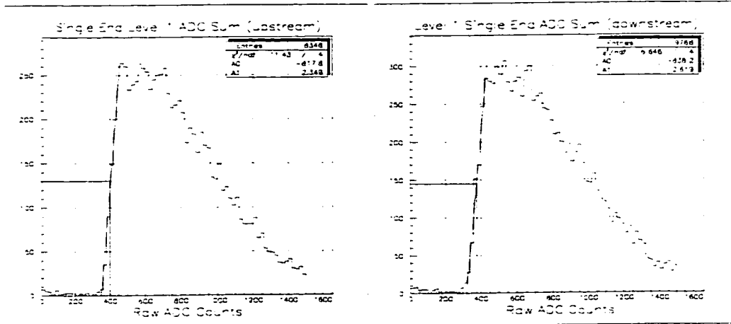
Figure 37: Raw ADC spectrum averaged over all sectors for the upstream and downstream end of the BV in \pi\gamma\gamma(2) data passing level 1.
