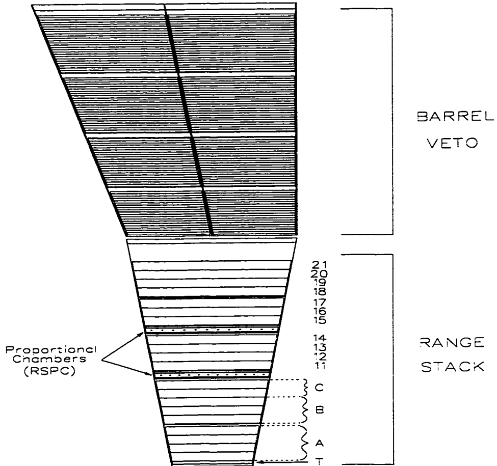
Figure 24: Design of a single range stack (and two barrel veto) sectors.
