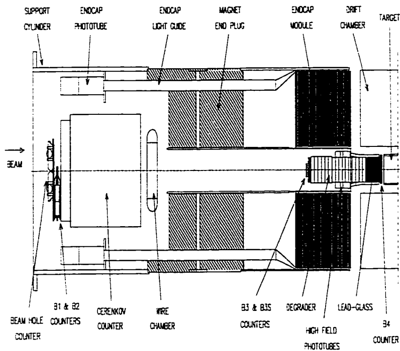
Figure 16: Detailed section of figure 13 showing the beam counters. Note that the B3 counters were removed for the 1991 run.
