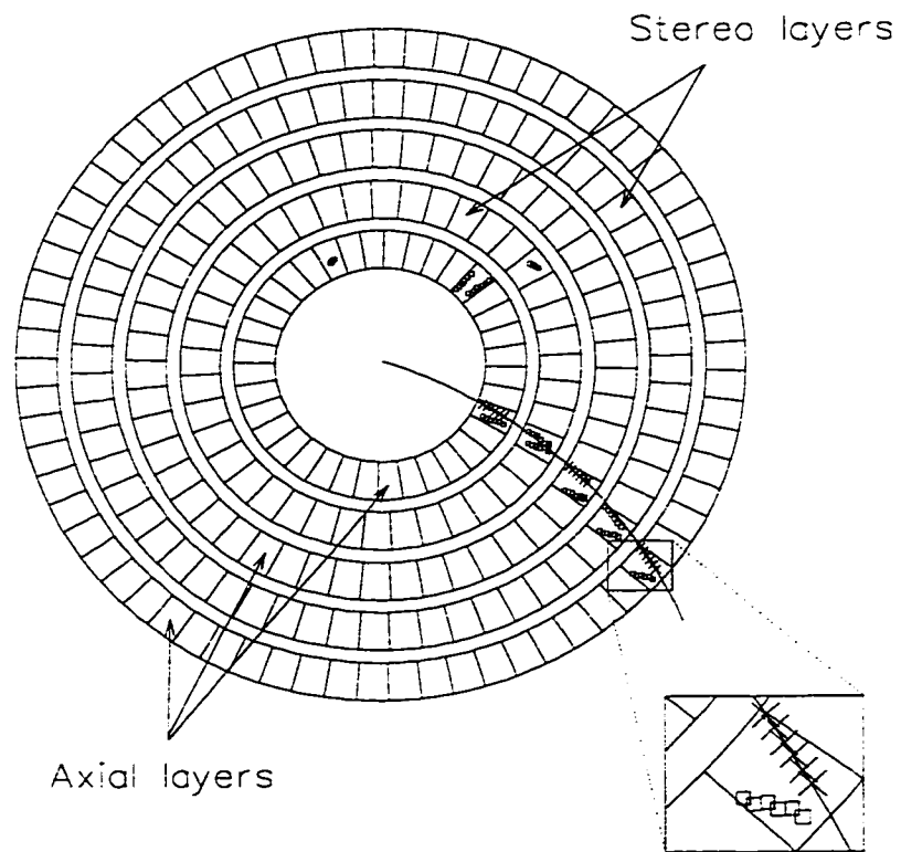
Figure 22: Cross section of the drift chamber showing the 5 layers of drift cells and a typical charged track including the two possible locations each single wire hit could correspond to (crosses and squares).
