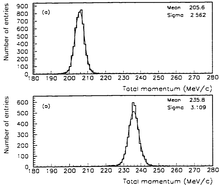
Figure 29: Total momentum resolutions for K\mu 2 and K\pi 2 found using the UTC and including target energy.
