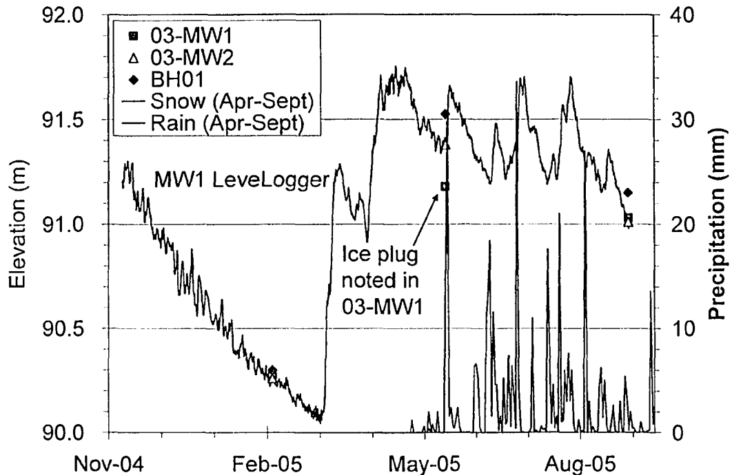
Figure AII-10 Annual groundwater surface elevation at Site B
