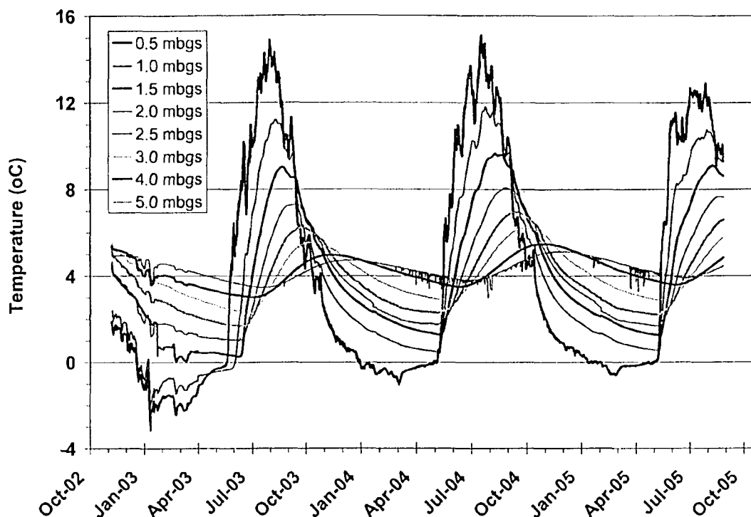
Figure AII-13 Subsurface temperature range with depth at Site B
