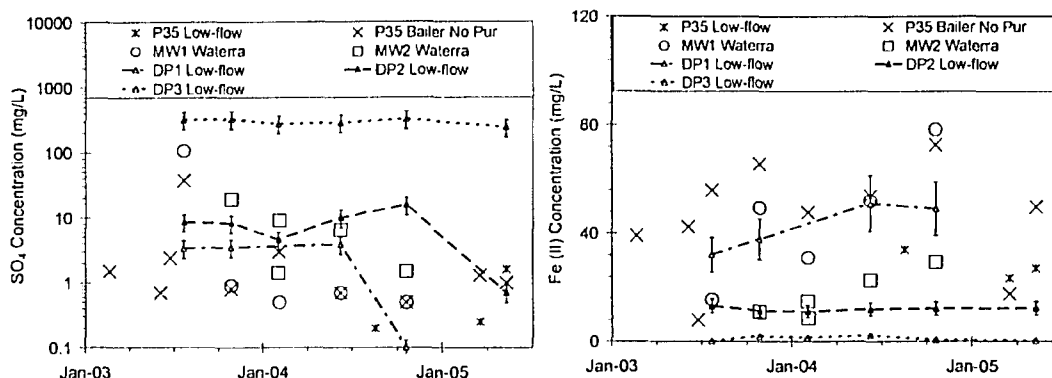
Figure 3-16 Sulphate (a, log-scale) and iron (II) (b) concentrations from selected monitoring wells at P35 cluster: lines connect DP data to show depth-discrete samples (0.7 m screen lengths); 30% error bars for sulphate and 20% for iron (II)
