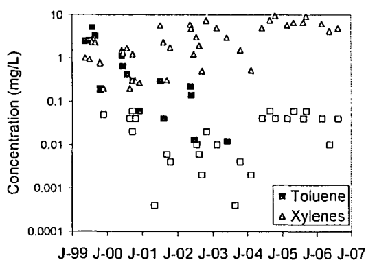
Figure 5-3 Trends at 98-17A: for T (decrease) and X (increase); hollow symbol = compound not detected
