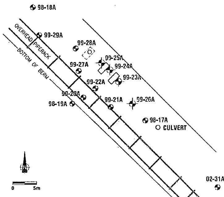
Figure AII-15 Site plan and monitoring wells at Site C
