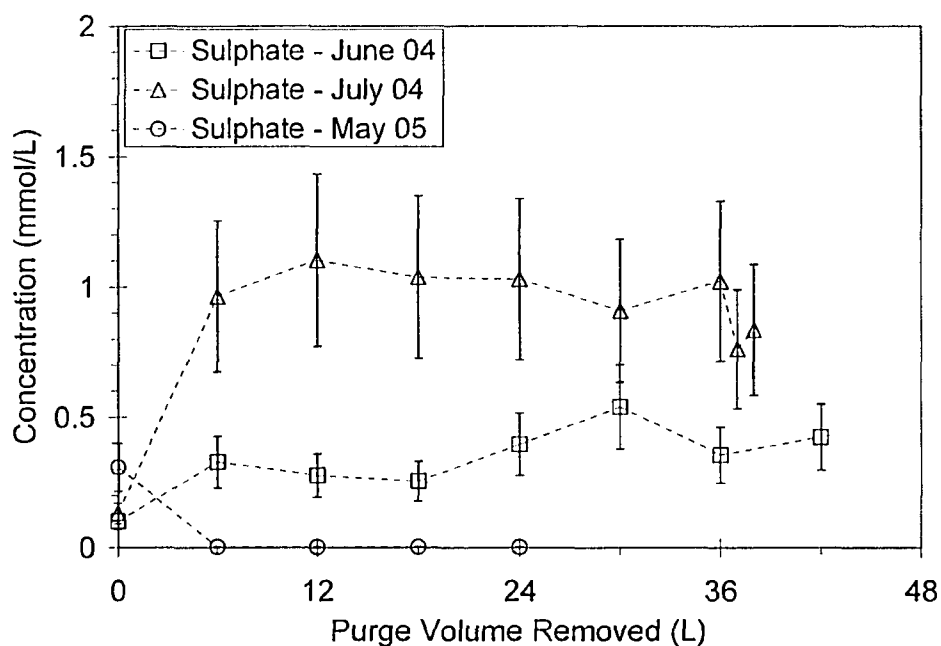
Figure 4-10 Sulphate concentrations for consecutive low-flow purge samples from P34 (1 borehole volume = 6 L)
