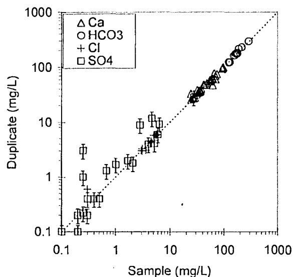
Figure 3-9 Cross-plot of selected analytes from duplicate samples at Site B. Symbol size includes 10% error; 30% error bar for \text{SO}_4 ; Dotted line shows theoretical 1:1 ratio.
