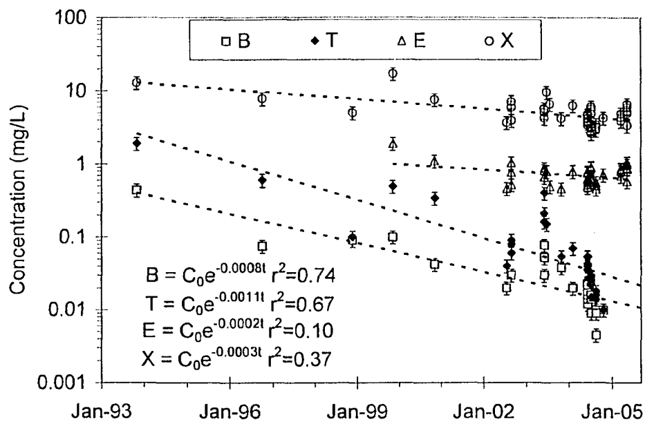
Figure 4-7 Temporal trends for BTEX at P34 (B, T in 2005 <0.04 mg/L)
