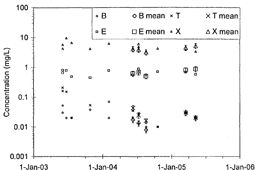
Figure 3-36 Historical variation compared to mean values of replicate samples for BTEX analytes sampled from well P34: (20% error bars)
