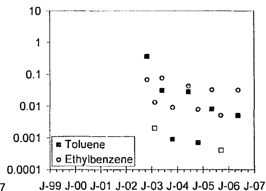
Figure 5-4 Trends at 02-31A for E (no trend) and T (decrease); hollow symbol = compound not detected
