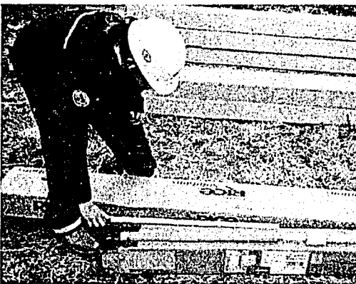
DP-pre-pack well screen, foam seal and paper wrapped bentonite seal to be placed inside driven steel pipe
