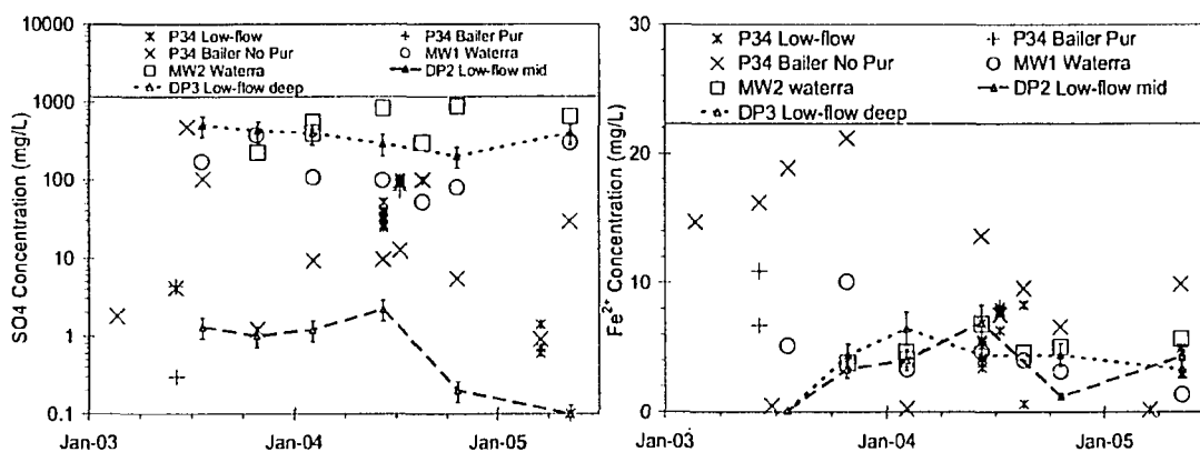
Figure 3-13 Sulphate (a) (log scale) and iron (II) (b) concentrations from selected monitoring wells and sampling strategies at P34 cluster: lines connect DP data to show data range for depth-discrete samples (0.7 m screen lengths). Error bars (30% \text{SO}_4 , 20% \text{Fe}(\text{II}) ) shown for DP wells.
