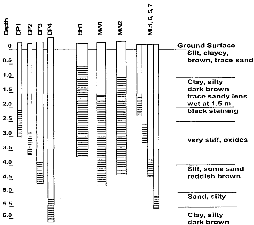
Figure 3-5. Site B Well Cluster Schematic Cross-section
