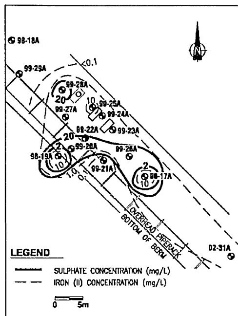
Figure AII-16b Iron(II) and sulphate concentrations (mg/L)
