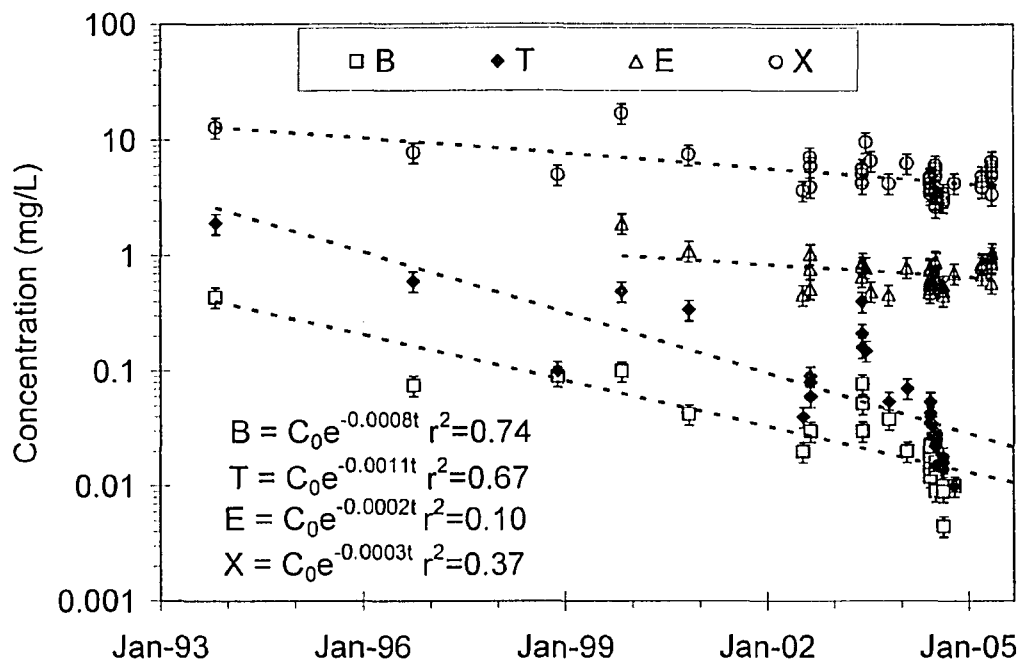
Figure 3-28 Temporal concentration trends for BTEX over time in P34, Site A; dashed lines follow exponential fit to the data with equations provided; suspected analytical problems with pre-1999 data for E
