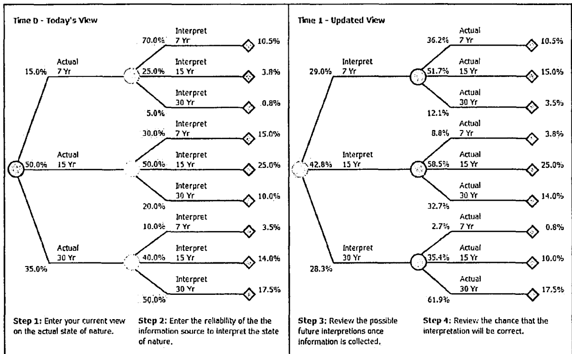
Figure 5-9 Decision tree modification using Bayes Law (interpret 7 year project after 2 years of monitoring) values rounded to 1 decimal place.
