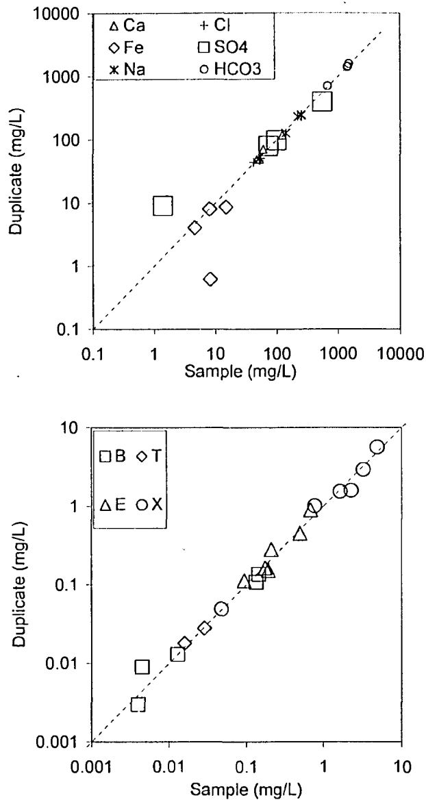
Figure 3-6 Cross-plots (log-scale) of selected analytes from duplicate samples at Site A. Symbol size includes error bar; dotted line shows the theoretical 1:1 ratio.
